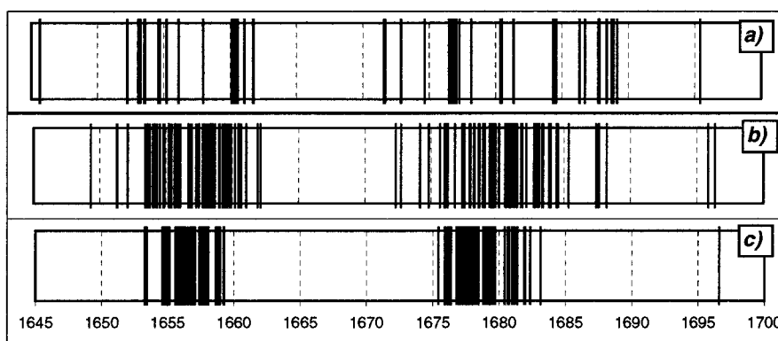
Figure 2. Days with sunspots during the deep Maunder minimum. (a) Actual observations according to the GSN series. (b) A sample of simulation for case I with B_0 = 0.05 , \sigma_0 = 3 , A_{11} = 0.05 . (c) A sample of simulation for case II with B_0 = 0.05 , \sigma_0 = 3 , A_{11} = 0.1
