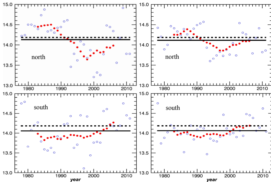
Fig. 1. Left-hand panels: yearly values of \Omega_{17} in units of deg/day in the north ( top ) and south ( bottom ) for X-ray flares. Open circles stand for the yearly best-fit values, filled circles demonstrate the 11-point running mean values. The solid horizontal line denotes the average \Omega_{17} over the entire study period, the dashed line the sidereal Carrington rotation rate. Right-hand panels: the same as in the left-hand panels , but for sunspots.
