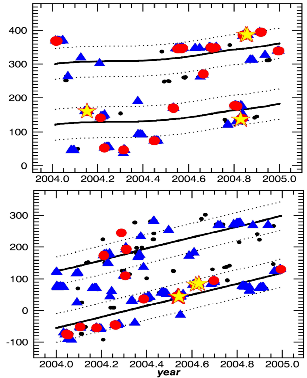
Fig. 3. Migration of ALs in units of degrees in the Carrington reference frame in the north (top) and south (bottom) in 2004. Black dots stand for B-flares, triangles for C-flares, red dots for M-flares, and stars for X-flares. The two solid lines depict the migration of the two ALs from the beginning to the end of 2004 with 45^\circ extensions on each side denoted by dotted lines.
