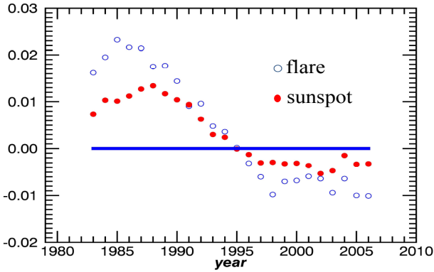
Fig. 2. Yearly values of the N-S asymmetry ((N-S)/(N+S)) of the solar rotation at latitude 17^\circ obtained from Fig. 1 for X-ray flares (open circles) and for sunspots (filled circles).
