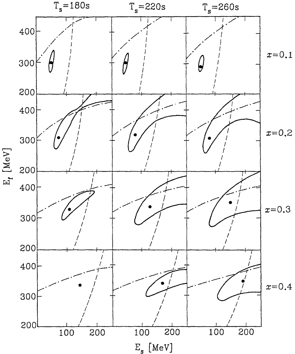
Fig. 6. Results of parameter fitting of Climax neutron monitor counting rate. Each contour represents the 90% confidence level in the (E_f, E_s) plane, for given values of the decay time of the slow component of neutron emission, T_s , and the fast-to-slow components ratio, x . The solid circles in each frame represent the best fit-parameter points. Additional restrictions are denoted by dash-dotted and dashed lines (see text).
