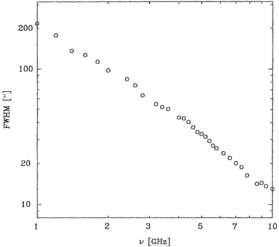
Fig. 2. Full width at half maximum of microwave brightness as a function of observing frequency. Full widths at half maximum are derived from the relative visibility of one baseline at Owens Valley Radio Observatory at the time 20:49 UT on 1990 May 24.
