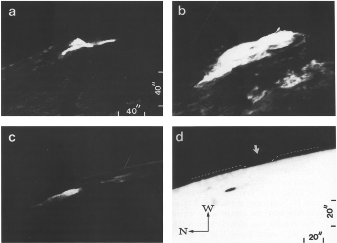
Fig. 1. (a) H\alpha center line picture of the active region NOAA 6063 at 19:40 UT on 1990 May 24. (b) The same as (a) at 20:49 UT. (c) A magnetogram of the region at 20:50 UT. (d) A white-light picture of the active region showing a hole in the limb profile before the flare. Note that (a), (b), and (c) are in the same scale and (d) is in a different scale as specified.
