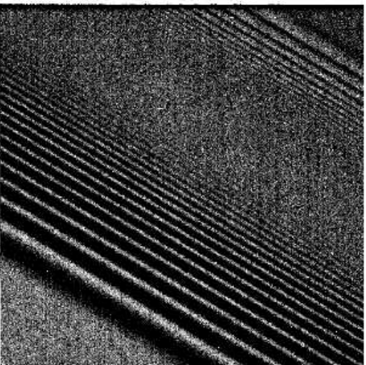
MIMAS 5:3 RESONANCE Density wave and bending wave
