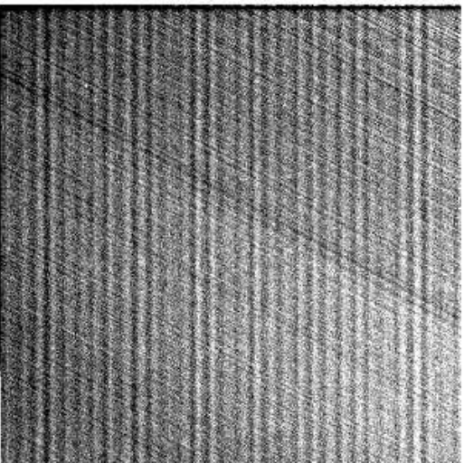
B RING ? (Cassini image with missing caption)
