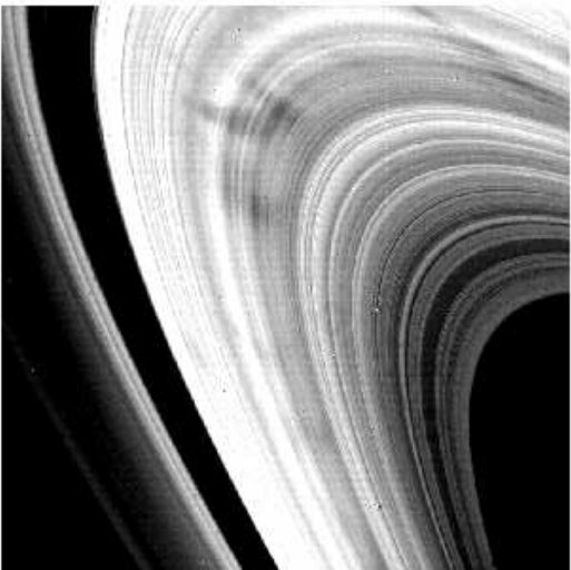
B RING SPOKES (Voyager image)
