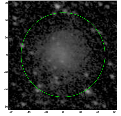
S4G: pa,inc= 154.3 40.3
