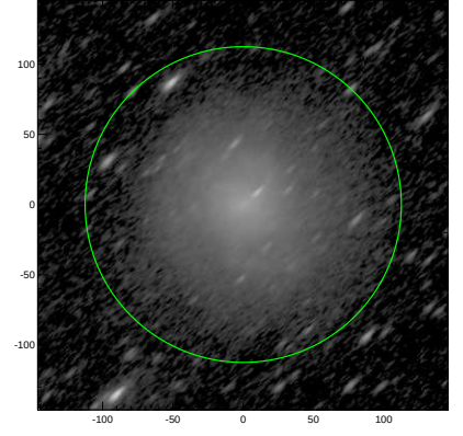
S4G: pa,inc= 42.6 69.5
