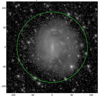
S4G: pa,inc= 124.4 25.7
