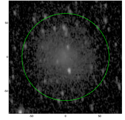
S4G: pa,inc= 96.9 54.3
