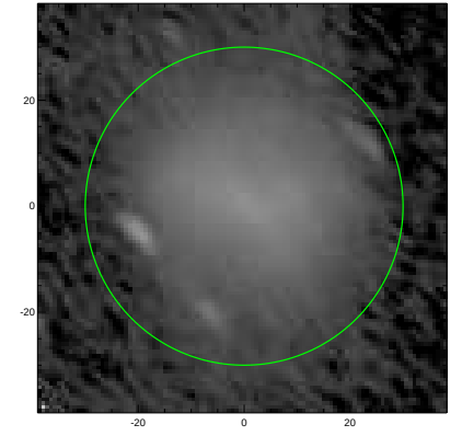
S4G: pa,inc= 134.5 64.5
