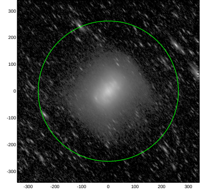
S4G: pa,inc= 130.5 73.2
