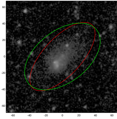
ESO409-015
