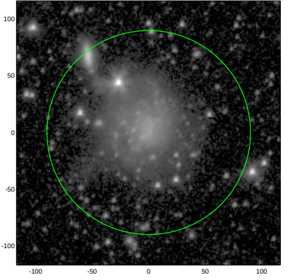
S4G: pa,inc= 78.2 22.3
