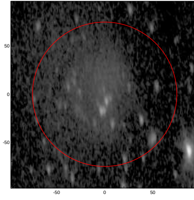
LEDA: pa,inc= 95.5 66.3
