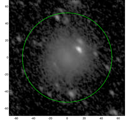
S4G: pa,inc= 132.2 55.1
