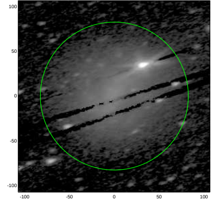
S4G: pa,inc= 17.0 63.0
