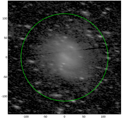
S4G: pa,inc= -11.2 67.9
