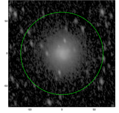
S4G: pa,inc= 104.3 59.0
