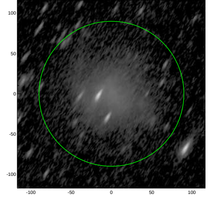
S4G: pa,inc= 58.4 71.0
