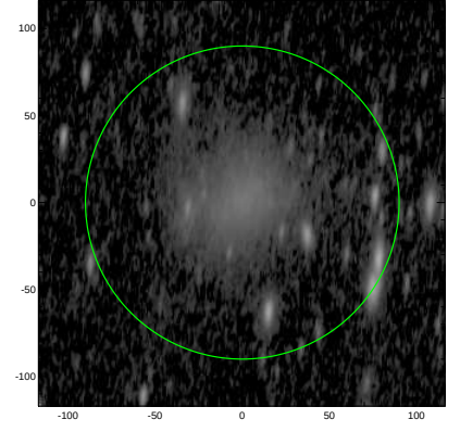
S4G: pa,inc= 85.3 70.6
