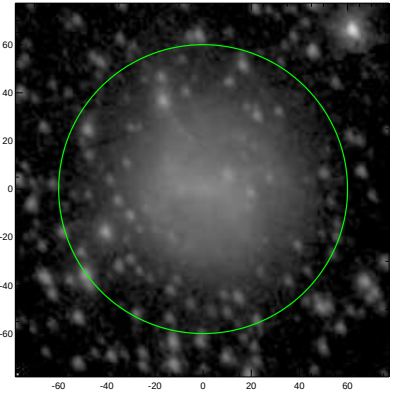
S4G: pa,inc= 116.7 37.2
