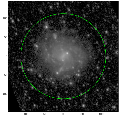
S4G: pa,inc= 117.5 33.3
