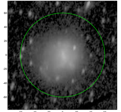
S4G: pa,inc= 78.8 55.6
