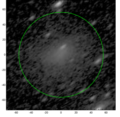
S4G: pa,inc= 36.8 65.1
