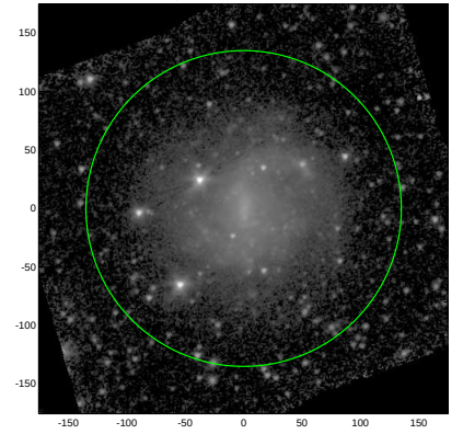
S4G: pa,inc= 32.8 25.7
