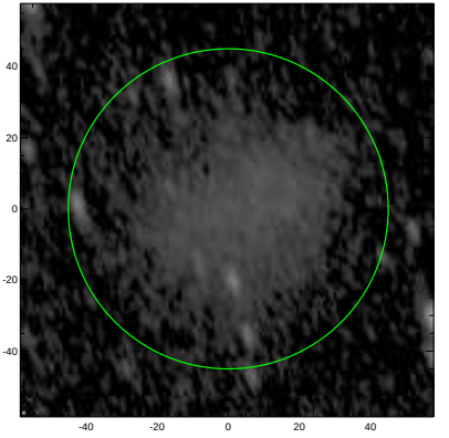
S4G: pa,inc= 109.1 63.3
