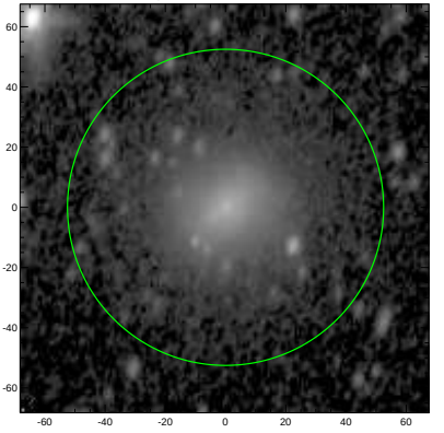
S4G: pa,inc= 73.5 47.6
