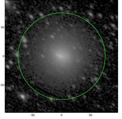
S4G: pa,inc= 138.3 52.8
