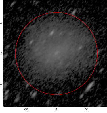
LEDA: pa,inc= 50.3 64.4
