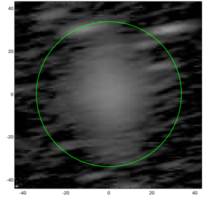
S4G: pa,inc= 10.3 77.7
