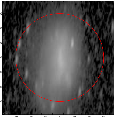
LEDA: pa,inc= 83.9 73.3
