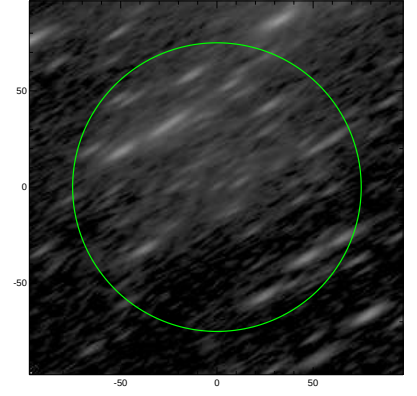
S4G: pa,inc= 30.3 75.7
