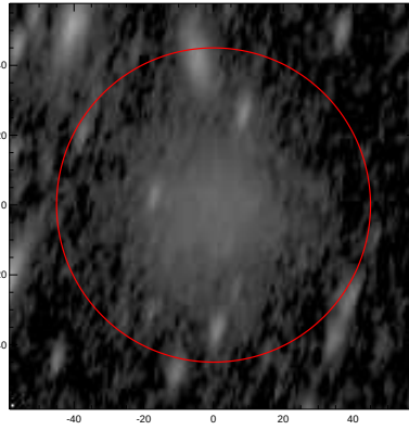
LEDA: pa,inc= 76.6 68.1
