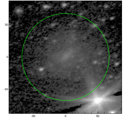
S4G: pa,inc= 18.1 50.4
