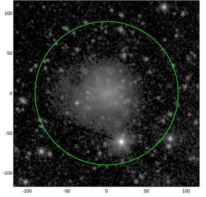
S4G: pa,inc= 127.5 21.2
