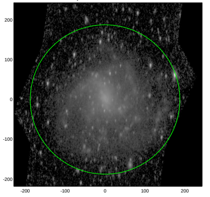
S4G: pa,inc= 88.4 60.9
