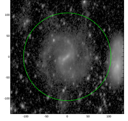
S4G: pa,inc= 80.9 51.0
