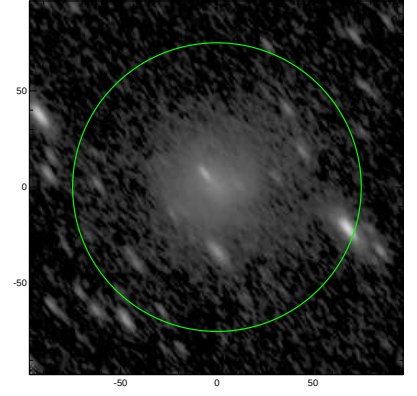
S4G: pa,inc= 127.7 67.9
