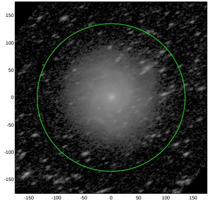
S4G: pa,inc= 24.3 62.5
