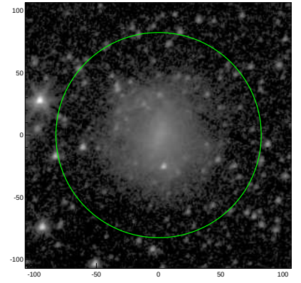
S4G: pa,inc= 49.6 26.3
