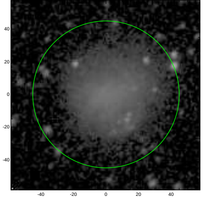
S4G: pa,inc= 43.2 24.5
