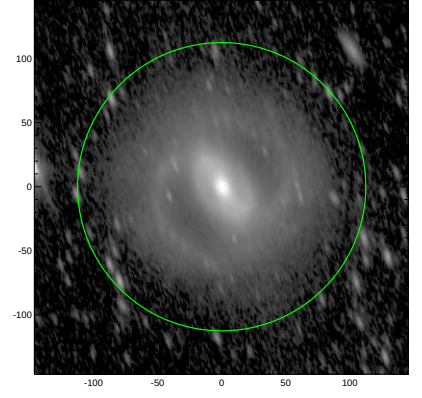
S4G: pa,inc= 109.1 69.1
