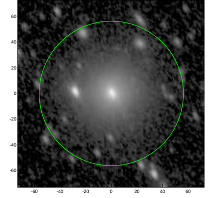
S4G: pa,inc= 121.0 52.7
