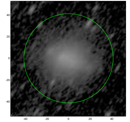
S4G: pa,inc= 52.9 62.9
