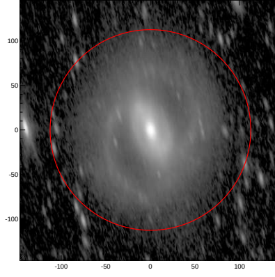
LEDA: pa,inc= 104.3 72.7
