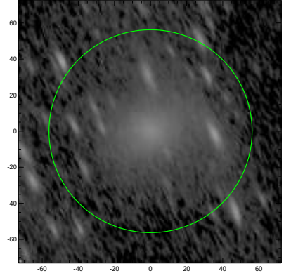
S4G: pa,inc= 114.4 69.4
