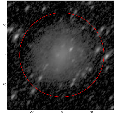
LEDA: pa,inc= 52.3 62.7
