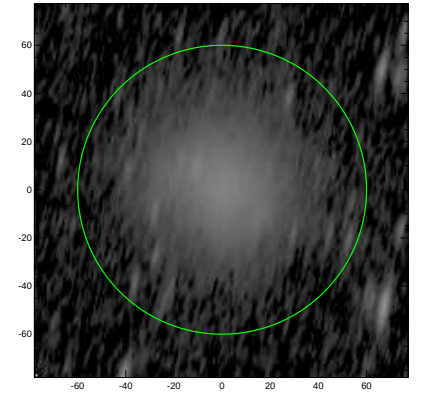
S4G: pa,inc= 77.6 75.1
