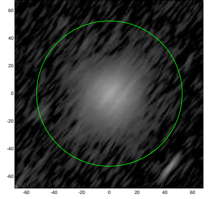
S4G: pa,inc= 51.9 78.6
