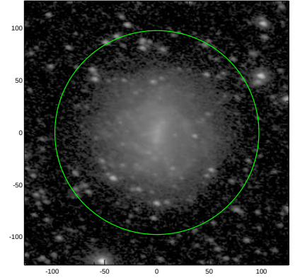
S4G: pa,inc= -14.3 49.0
