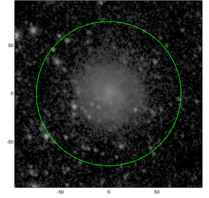
S4G: pa,inc= 112.0 25.0
