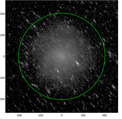
S4G: pa,inc= 128.4 67.4
