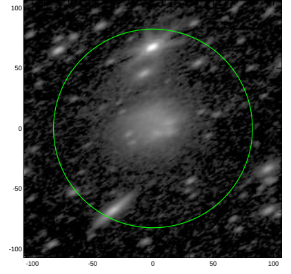
S4G: pa,inc= 28.2 61.6
