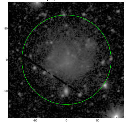
S4G: pa,inc= 26.6 27.1
