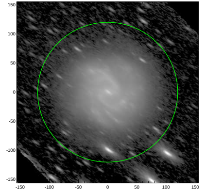
S4G: pa,inc= 145.1 70.5
