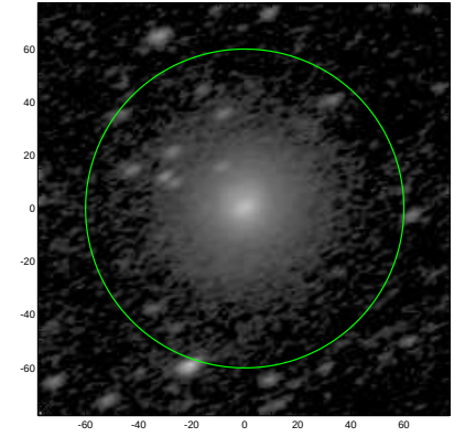
S4G: pa,inc= 23.8 58.6
