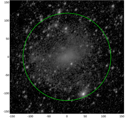
S4G: pa,inc= 53.8 41.8
