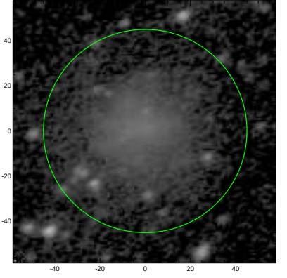
S4G: pa,inc= 22.5 43.7
