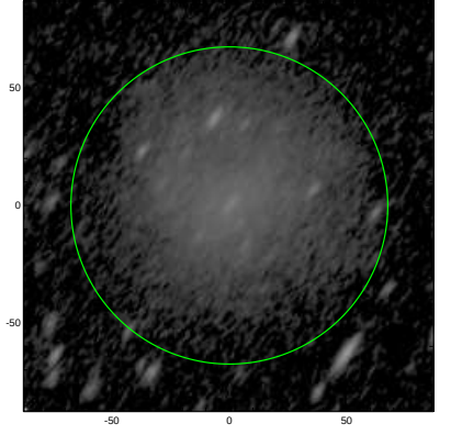
S4G: pa,inc= 56.4 64.1
