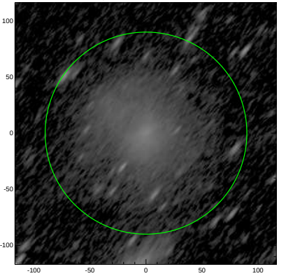
S4G: pa,inc= 50.0 72.5
