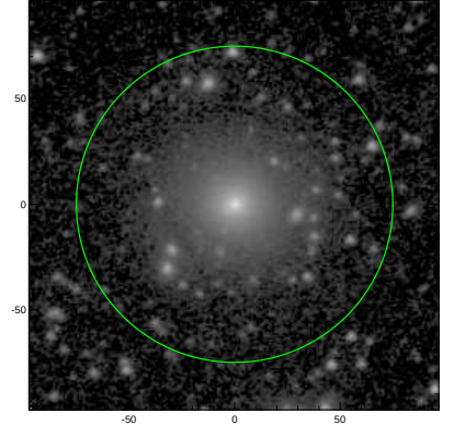
S4G: pa,inc= 16.6 24.4
