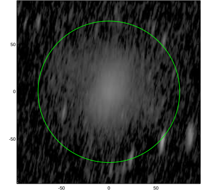
S4G: pa,inc= 79.9 78.2
