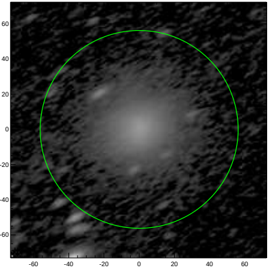
S4G: pa,inc= 28.1 65.8
