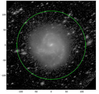
S4G: pa,inc= 25.7 50.2
