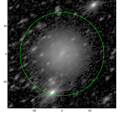
S4G: pa,inc= 38.3 59.8
