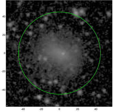
S4G: pa,inc= -13.1 22.8
