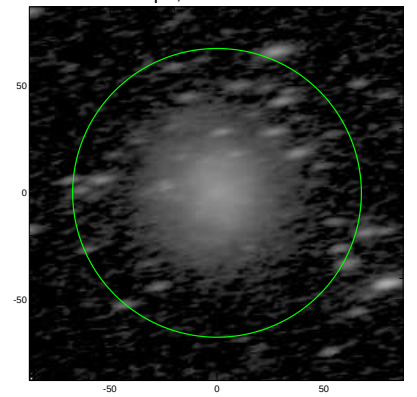
S4G: pa,inc= 12.0 70.1
