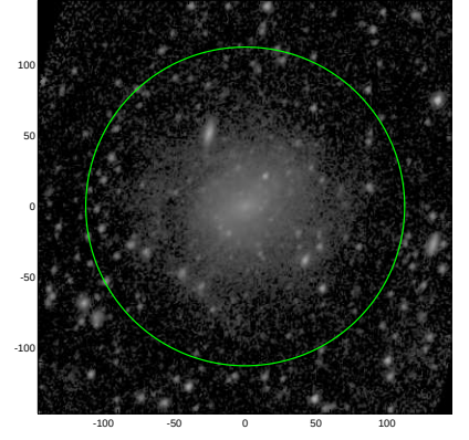
S4G: pa,inc= 66.9 29.4
