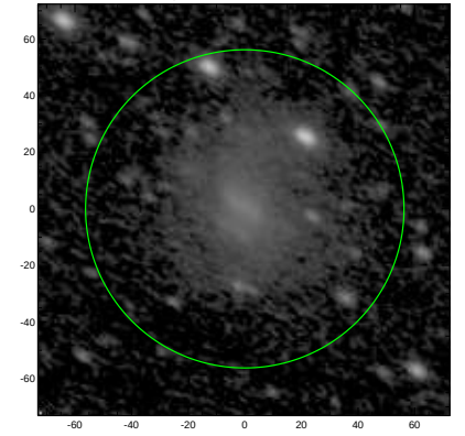
S4G: pa,inc= 148.2 52.6
