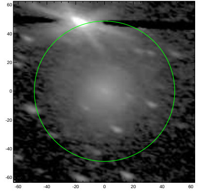
S4G: pa,inc= -19.6 63.5
