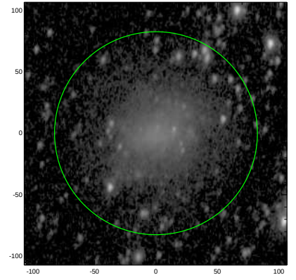
S4G: pa,inc= 86.4 47.5
