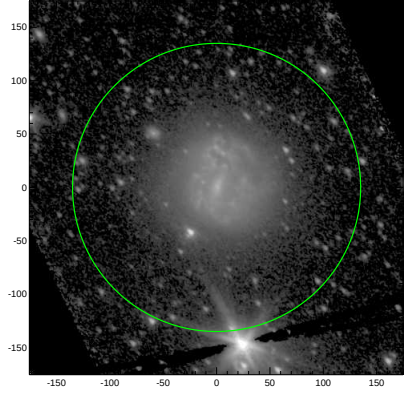
S4G: pa,inc= 134.6 44.8
