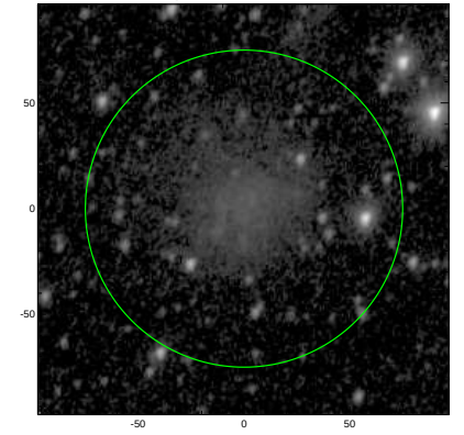
S4G: pa,inc= 71.6 38.0
