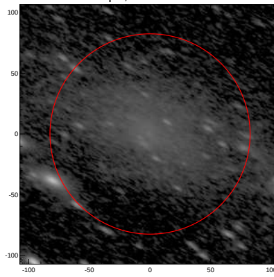
LEDA: pa,inc= 150.1 67.4
