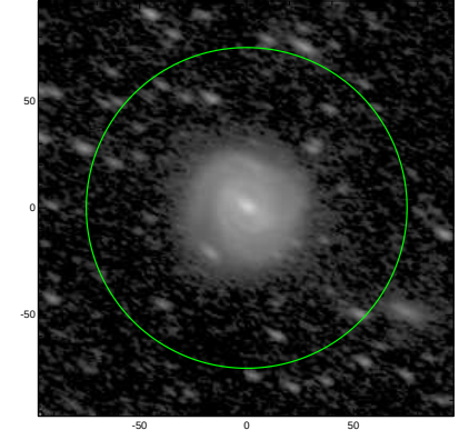
S4G: pa,inc= 155.7 59.4
