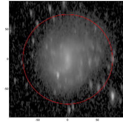
LEDA: pa,inc= 91.4 68.8
