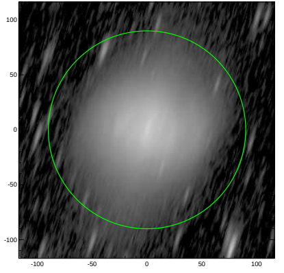
S4G: pa,inc= 72.8 79.9
