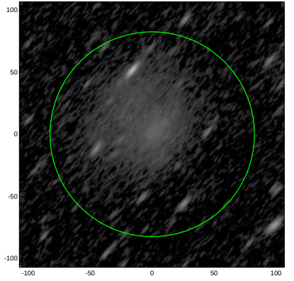
S4G: pa,inc= 49.2 71.2
