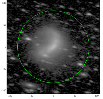
S4G: pa,inc= -13.0 66.3
