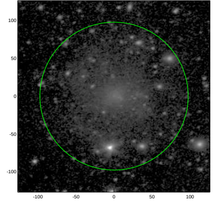
S4G: pa,inc= 12.2 34.9
