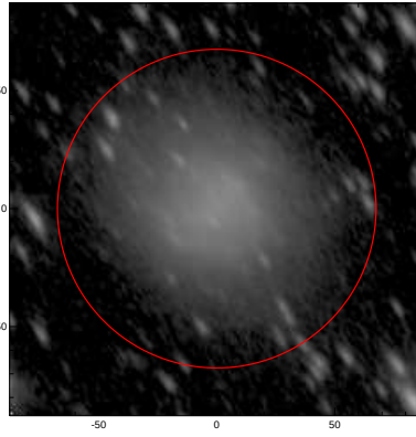
LEDA: pa,inc= 122.8 64.5
