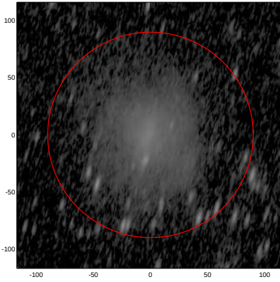
LEDA: pa,inc= 75.5 70.9
