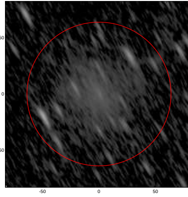
LEDA: pa,inc= 120.1 75.9
