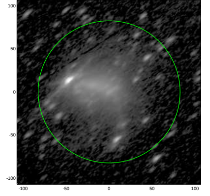
S4G: pa,inc= 39.1 65.8
