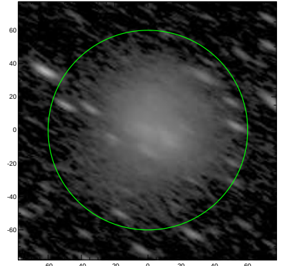
S4G: pa,inc= 151.9 71.1
