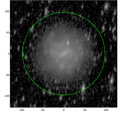
S4G: pa,inc= 81.8 64.8
