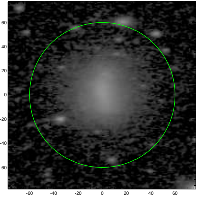
S4G: pa,inc= 2.1 58.8
