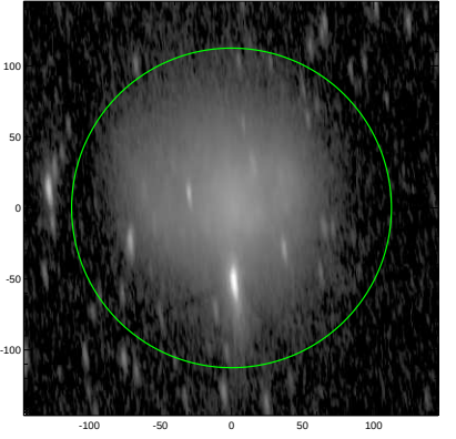
S4G: pa,inc= 95.3 76.5
