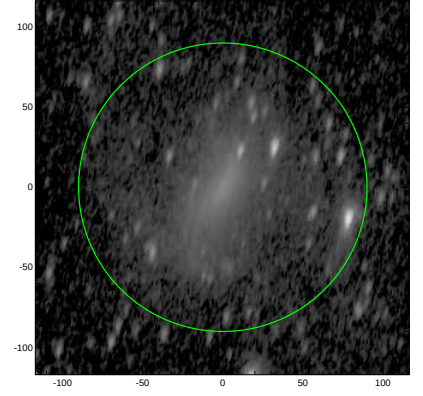
S4G: pa,inc= 76.9 65.3
