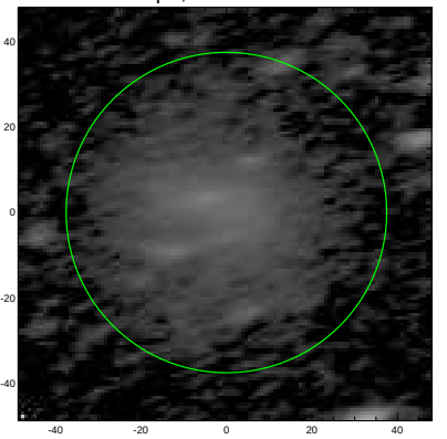
S4G: pa,inc= 15.4 67.5
