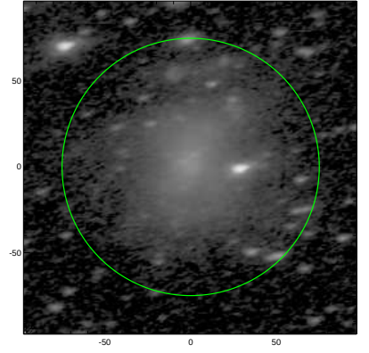
S4G: pa,inc= 13.1 60.9
