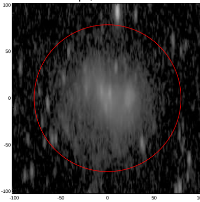
LEDA: pa,inc= 91.2 75.5
