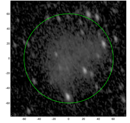
S4G: pa,inc= 111.2 60.0
