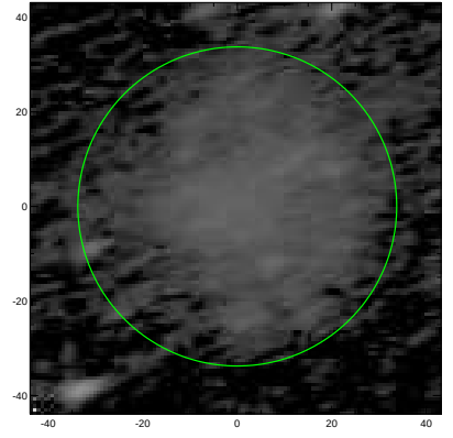
S4G: pa,inc= 16.0 64.5
