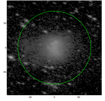
S4G: pa,inc= 159.8 55.8
