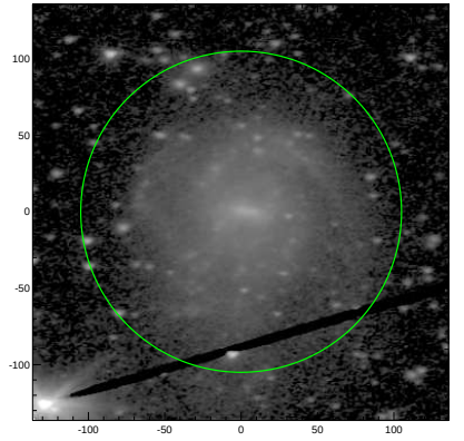
S4G: pa,inc= 5.2 50.7
