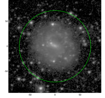
S4G: pa,inc= 19.3 20.0
