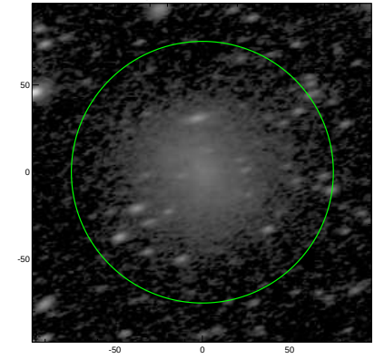
S4G: pa,inc= 16.8 59.6
