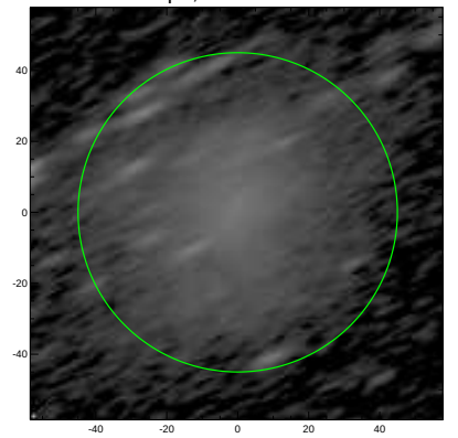
S4G: pa,inc= 25.3 73.1
