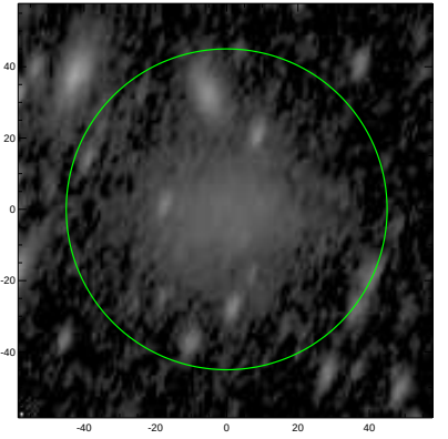
S4G: pa,inc= 71.1 62.3
