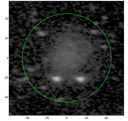
S4G: pa,inc= -7.8 57.2
