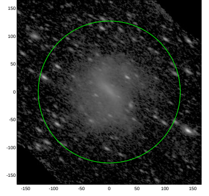
S4G: pa,inc= 146.2 62.7
