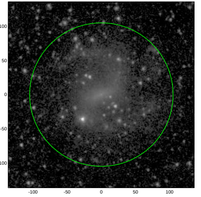
S4G: pa,inc= 124.8 10.3
