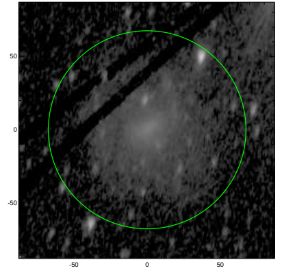
S4G: pa,inc= 77.9 58.3
