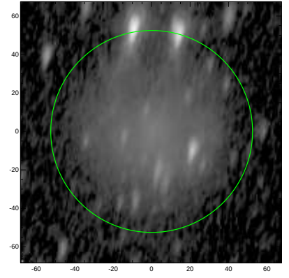
S4G: pa,inc= 78.2 68.5
