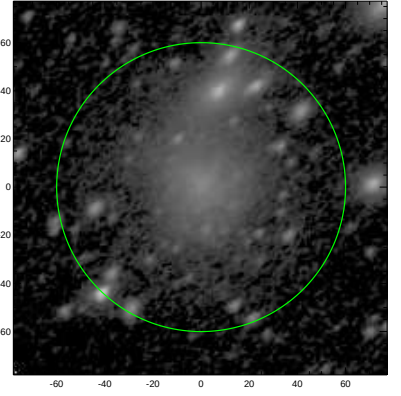
S4G: pa,inc= 39.7 47.6
