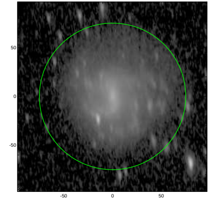
S4G: pa,inc= 96.3 67.5
