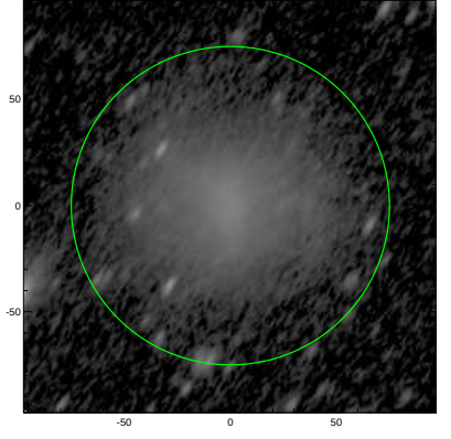
S4G: pa,inc= 57.1 65.7
