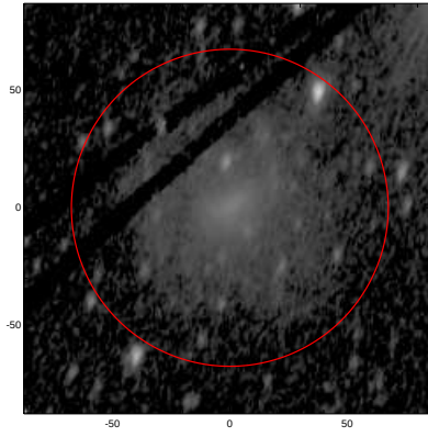
LEDA: pa,inc= 75.6 57.5
