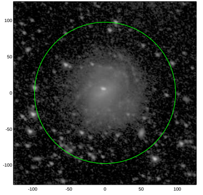
S4G: pa,inc= 151.7 40.2
