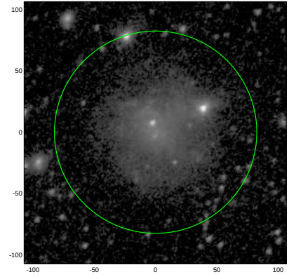
S4G: pa,inc= 45.3 31.7
