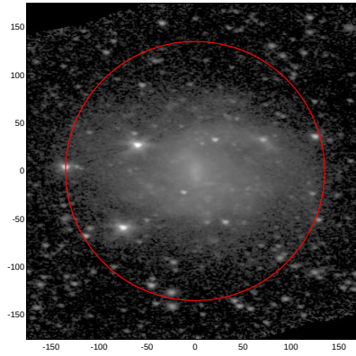
LEDA: pa,inc= 175.9 51.9
