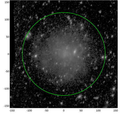
S4G: pa,inc= 69.3 40.5
