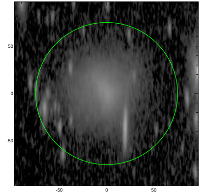
S4G: pa,inc= 90.9 74.5
