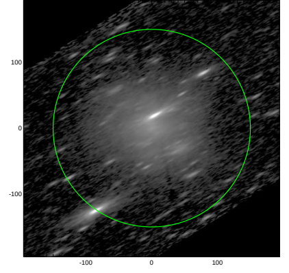
S4G: pa,inc= 27.7 75.5
