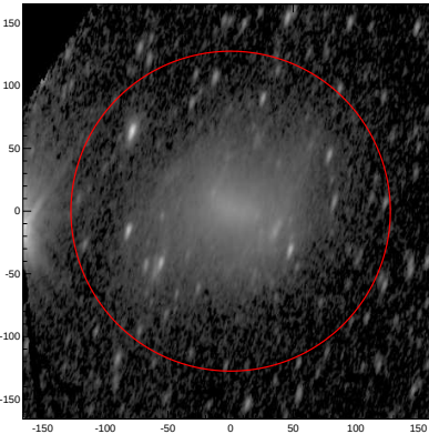
LEDA: pa,inc= 75.3 67.5
