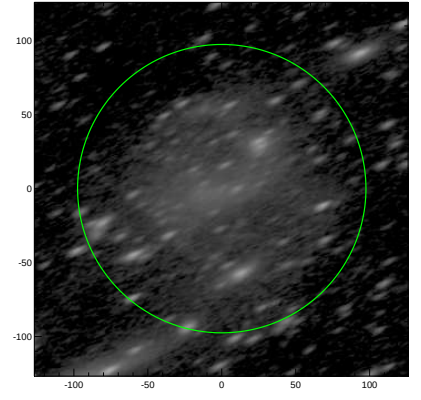
S4G: pa,inc= 25.3 68.8
