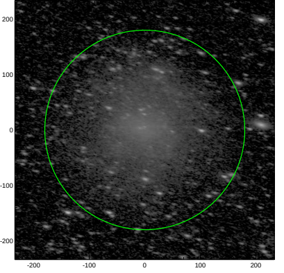
S4G: pa,inc= -14.1 64.2
