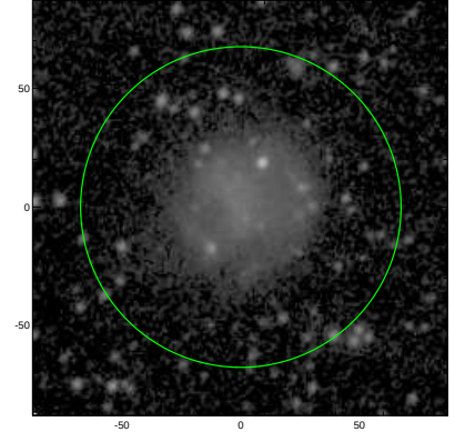
S4G: pa,inc= 67.0 20.7
