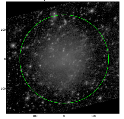
S4G: pa,inc= 35.2 40.8
