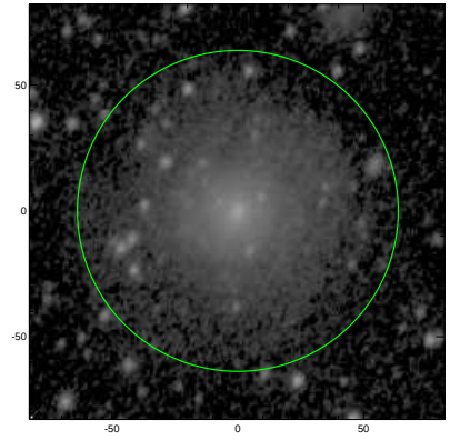
S4G: pa,inc= 63.1 38.0
