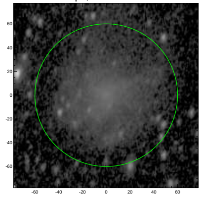
S4G: pa,inc= 80.1 50.6
