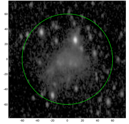
S4G: pa,inc= 97.0 53.2
