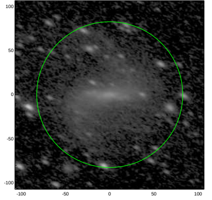
S4G: pa,inc= 153.2 60.0
