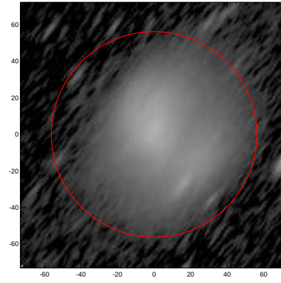
LEDA: pa,inc= 52.9 75.4
