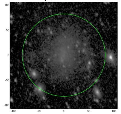
S4G: pa,inc= 111.6 48.3
