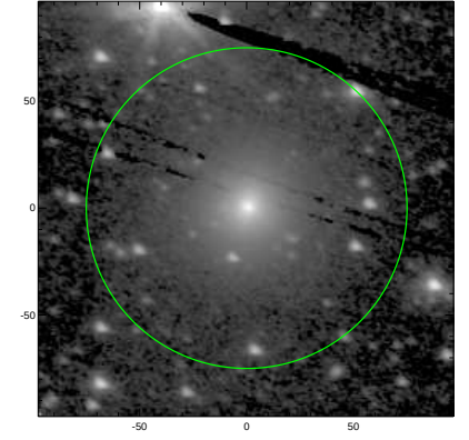
S4G: pa,inc= 158.2 44.6
