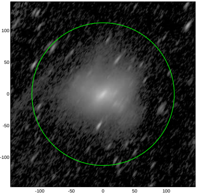
S4G: pa,inc= 56.3 71.2
