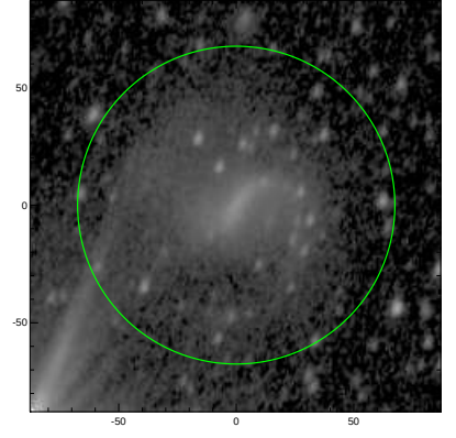
S4G: pa,inc= 71.9 46.6
