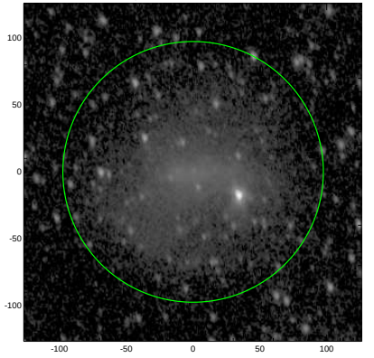
S4G: pa,inc= 102.7 47.1
