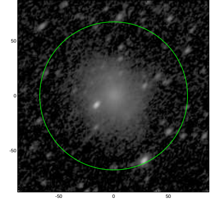
S4G: pa,inc= 46.5 51.3
