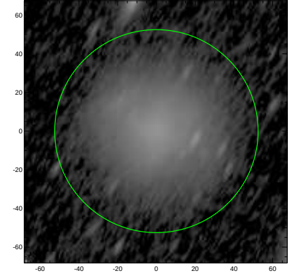
S4G: pa,inc= 61.5 69.8
