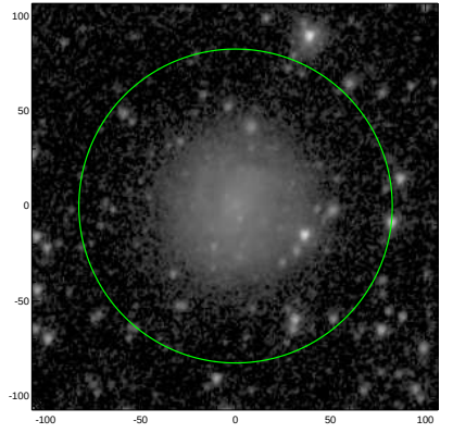
S4G: pa,inc= 68.2 31.0
