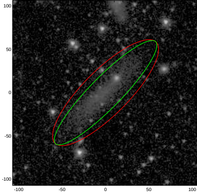
ESO508-030
