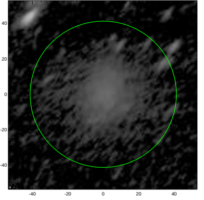
S4G: pa,inc= 46.0 64.8
