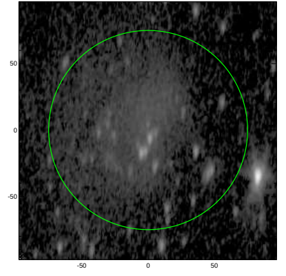
S4G: pa,inc= 85.2 64.5
