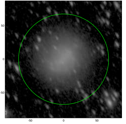
S4G: pa,inc= 118.2 58.7
