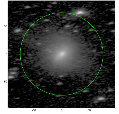
S4G: pa,inc= 5.6 65.7
