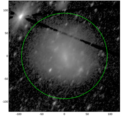
S4G: pa,inc= 56.1 57.0
