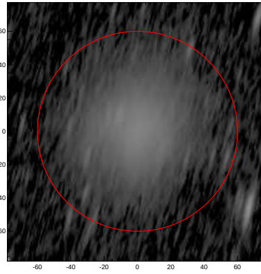
LEDA: pa,inc= 75.7 77.8
