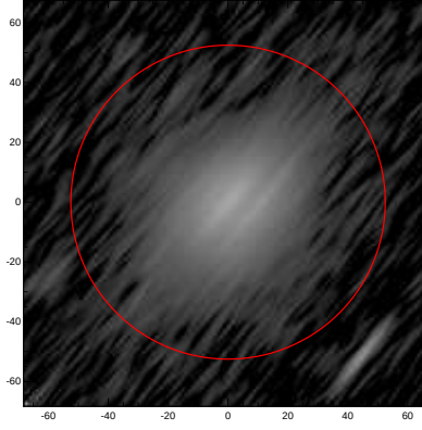
LEDA: pa,inc= 50.8 81.2
