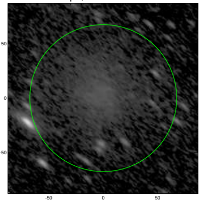
S4G: pa,inc= 139.4 67.7
