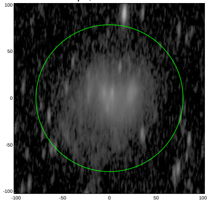
S4G: pa,inc= 87.0 74.7
