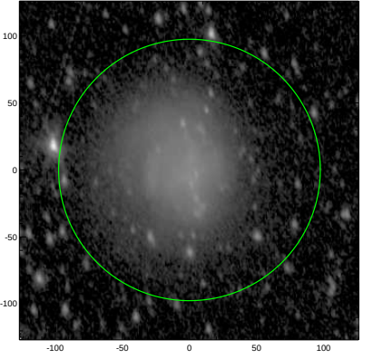
S4G: pa,inc= 102.9 55.1
