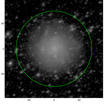
S4G: pa,inc= 31.8 39.5
