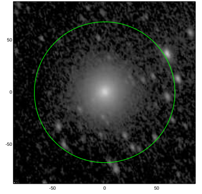
S4G: pa,inc= 117.6 53.1
