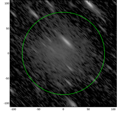
S4G: pa,inc= 135.6 77.3
