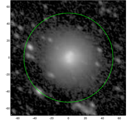
S4G: pa,inc= 137.9 51.5
