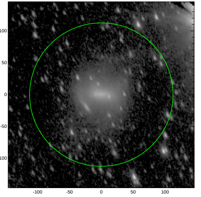
S4G: pa,inc= 114.1 59.0
