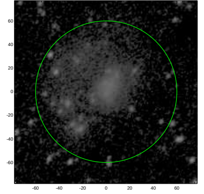
S4G: pa,inc= 46.2 37.4
