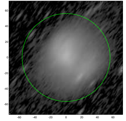
S4G: pa,inc= 51.6 74.8
