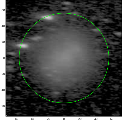
S4G: pa,inc= -4.2 69.8
