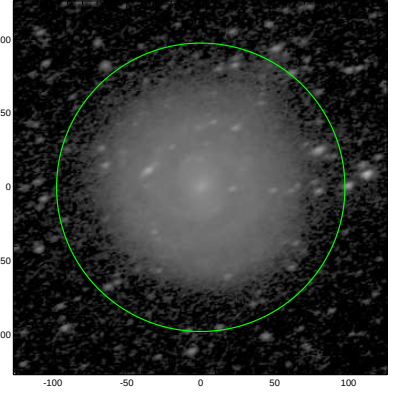
S4G: pa,inc= 19.1 52.6
