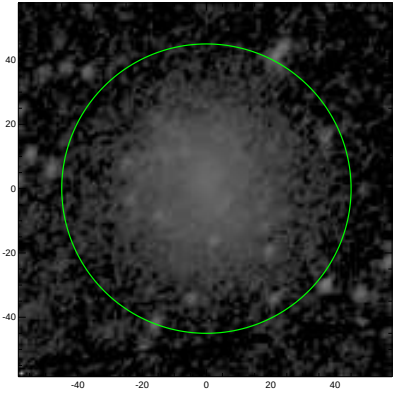
S4G: pa,inc= 49.8 42.3
