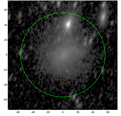
S4G: pa,inc= 74.4 56.8
