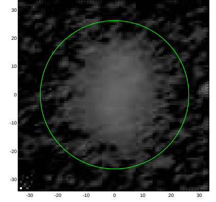
S4G: pa,inc= 26.3 59.9
