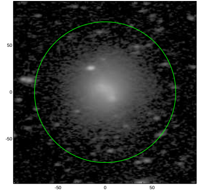
S4G: pa,inc= 2.4 59.7
