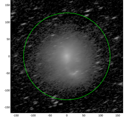
S4G: pa,inc= 19.8 70.4
