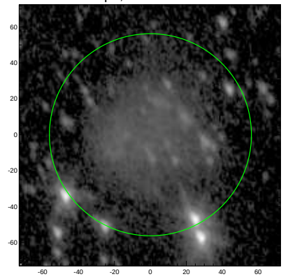
S4G: pa,inc= 111.4 48.4
