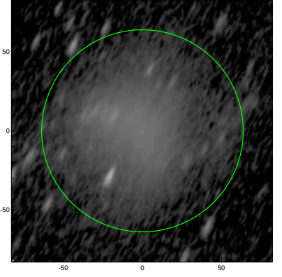
S4G: pa,inc= 63.3 70.5
