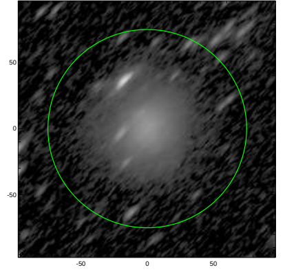
S4G: pa,inc= 45.9 71.6
