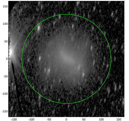
S4G: pa,inc= 83.6 68.3
