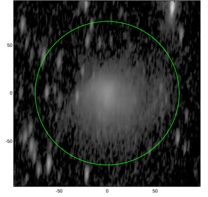
S4G: pa,inc= 85.2 74.0
