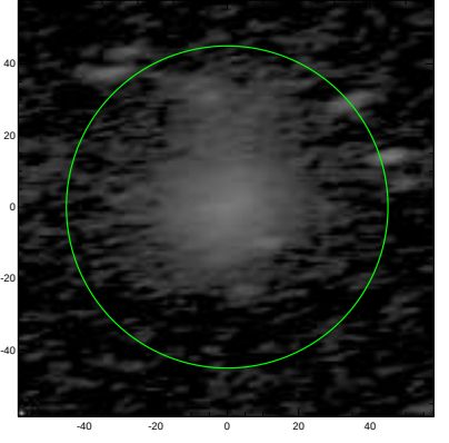
S4G: pa,inc= 8.3 71.2
