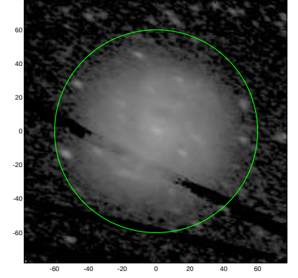
S4G: pa,inc= 155.9 56.9
