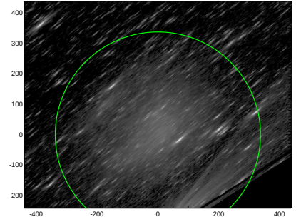
S4G: pa,inc= 39.8 80.7
