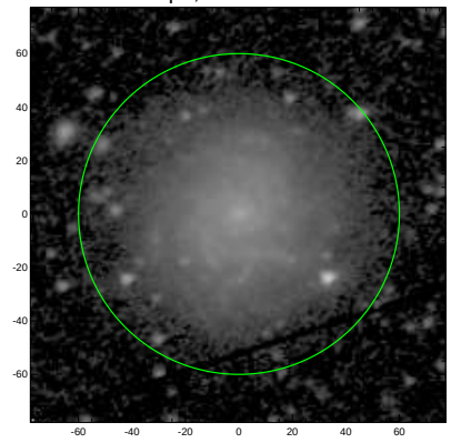
S4G: pa,inc= 19.9 35.6
