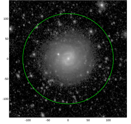
S4G: pa,inc= 118.8 31.8
