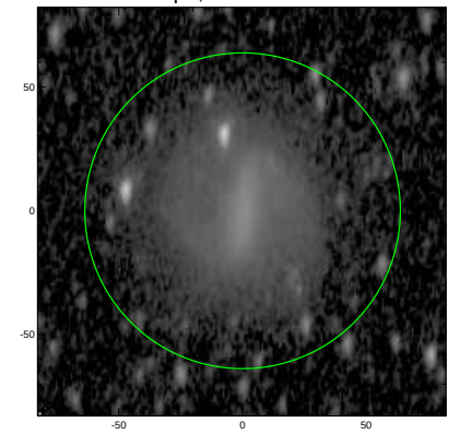
S4G: pa,inc= 86.4 58.2
