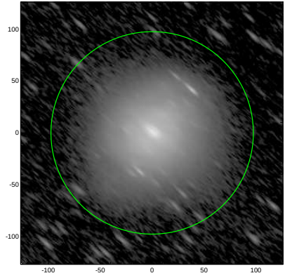
S4G: pa,inc= 138.4 74.9
