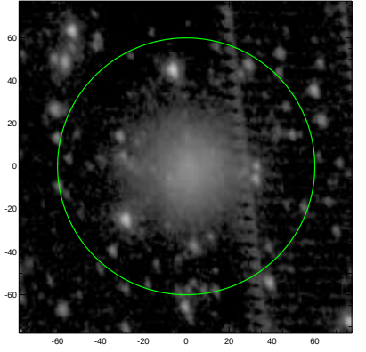
S4G: pa,inc= 107.2 40.4
