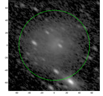
S4G: pa,inc= 142.4 61.2
