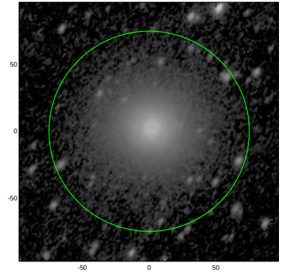
S4G: pa,inc= 55.6 51.6
