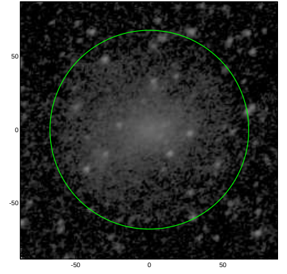
S4G: pa,inc= 36.2 39.1
