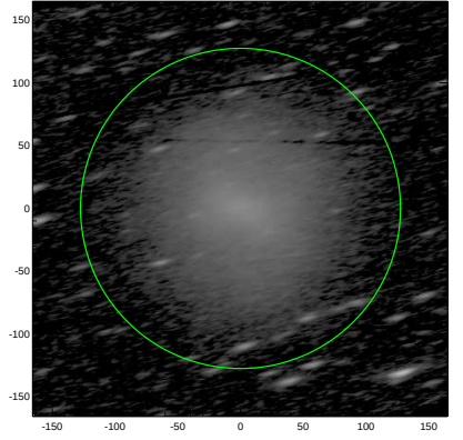
S4G: pa,inc= 14.6 75.9
