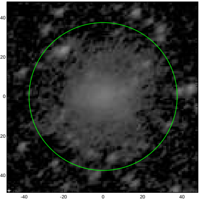
S4G: pa,inc= 36.6 50.3
