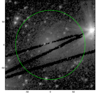
S4G: pa,inc= 44.0 36.3
