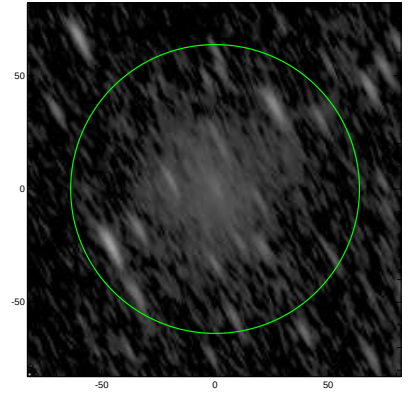
S4G: pa,inc= 118.2 75.4
