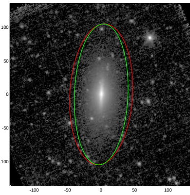
ESO506-033
