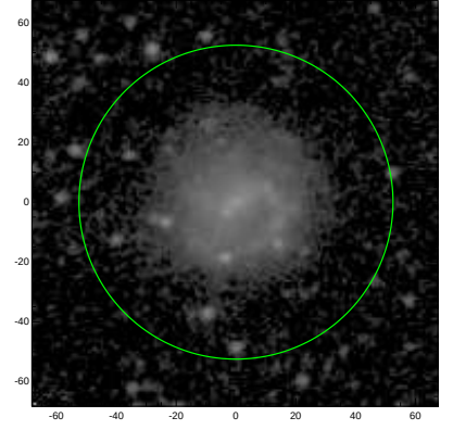
S4G: pa,inc= 7.5 24.5
