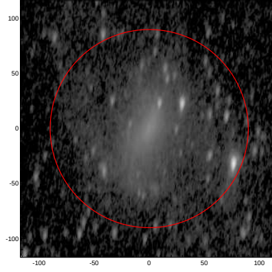
LEDA: pa,inc= 82.6 66.5
