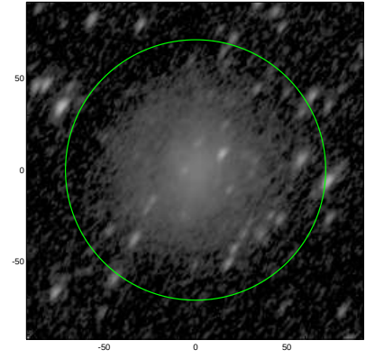
S4G: pa,inc= 54.8 61.2
