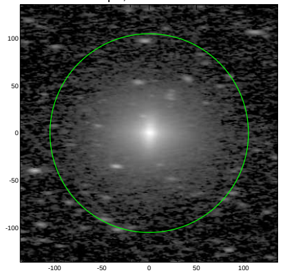
S4G: pa,inc= -2.3 67.6
