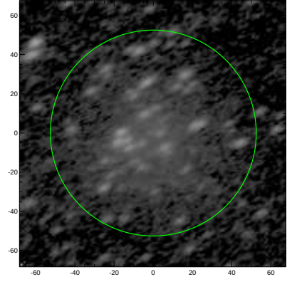
S4G: pa,inc= 29.2 58.6
