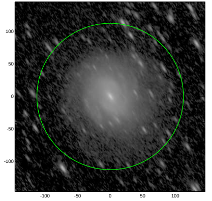
S4G: pa,inc= 125.2 69.0
