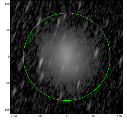
S4G: pa,inc= 71.5 76.1
