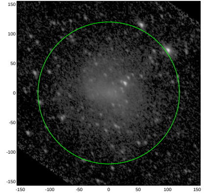
S4G: pa,inc= 129.4 51.5
