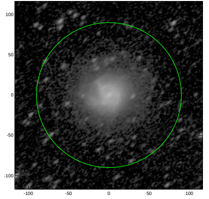
S4G: pa,inc= 40.1 56.5
