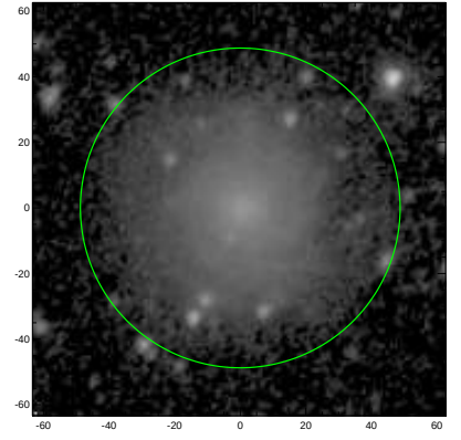
S4G: pa,inc= 57.5 32.9
