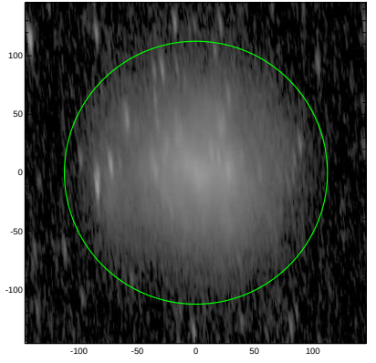
S4G: pa,inc= 94.8 80.6
