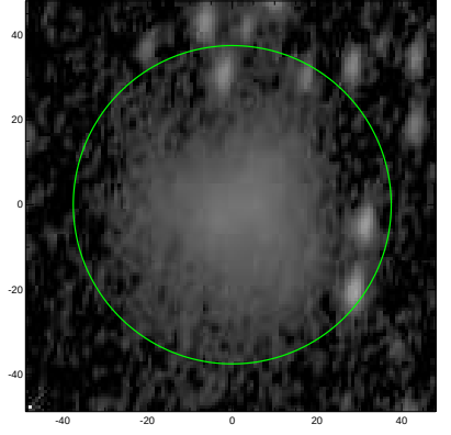
S4G: pa,inc= 83.7 62.3
