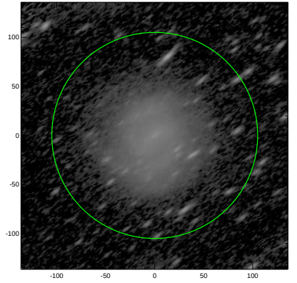
S4G: pa,inc= 35.6 67.7
