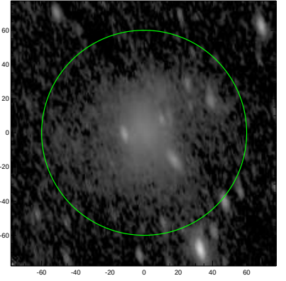
S4G: pa,inc= 105.3 64.1
