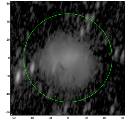
S4G: pa,inc= 80.4 67.7
