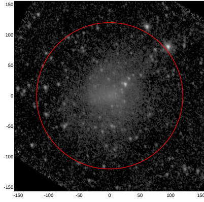
LEDA: pa,inc= 115.6 37.4
