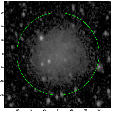
S4G: pa,inc= 92.8 42.5
