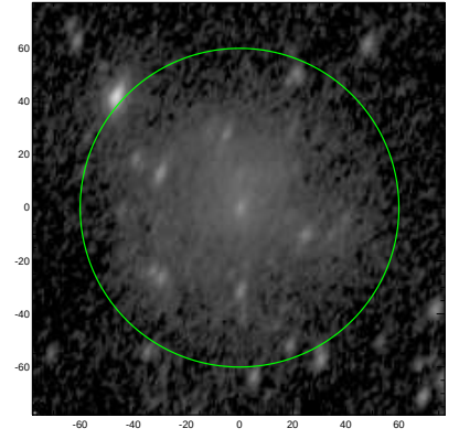
S4G: pa,inc= 69.3 55.8
