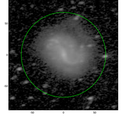
S4G: pa,inc= 9.0 58.1
