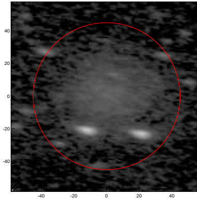
LEDA: pa,inc= 170.2 67.0
