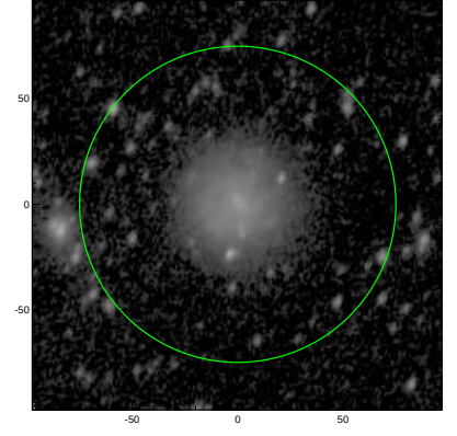
S4G: pa,inc= 70.9 41.7
