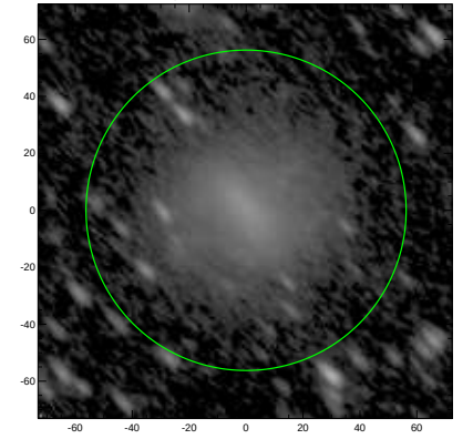
S4G: pa,inc= 133.7 62.7
