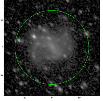
S4G: pa,inc= 136.2 47.8
