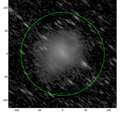
S4G: pa,inc= 141.4 72.1
