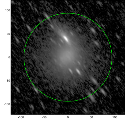
S4G: pa,inc= 127.1 70.6
