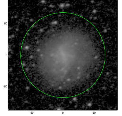
S4G: pa,inc= 18.3 36.1
