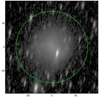
S4G: pa,inc= 79.5 69.9
