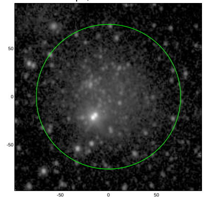
S4G: pa,inc= 106.0 26.0
