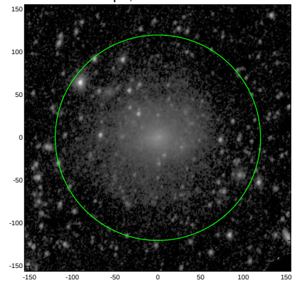
S4G: pa,inc= 75.9 35.1
