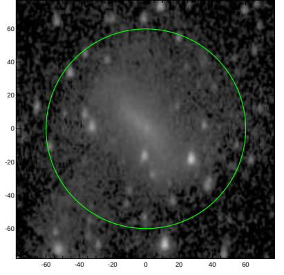
S4G: pa,inc= 91.3 48.0
