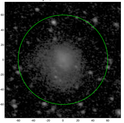
S4G: pa,inc= 158.4 40.5
