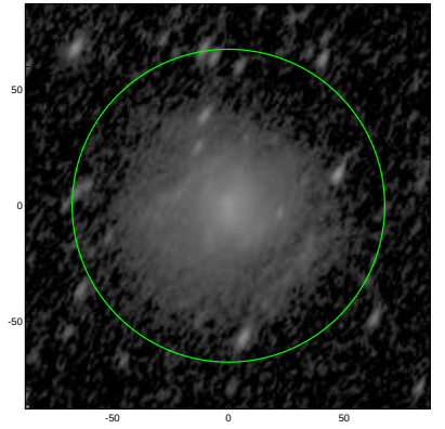
S4G: pa,inc= 59.7 61.0
