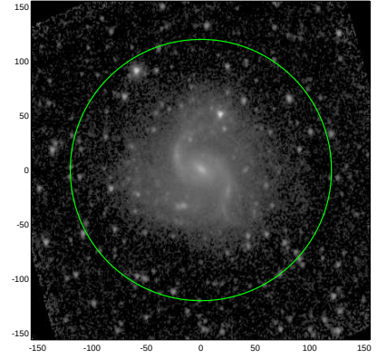
S4G: pa,inc= 81.6 31.5
