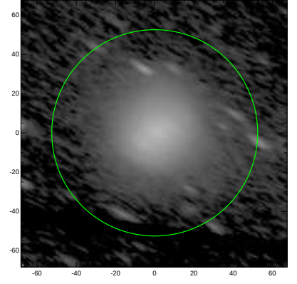
S4G: pa,inc= 151.3 70.3
