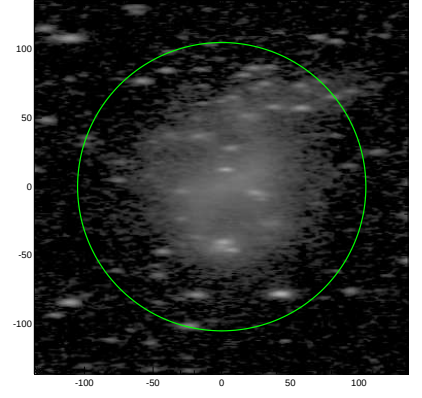
S4G: pa,inc= 0.4 72.0
