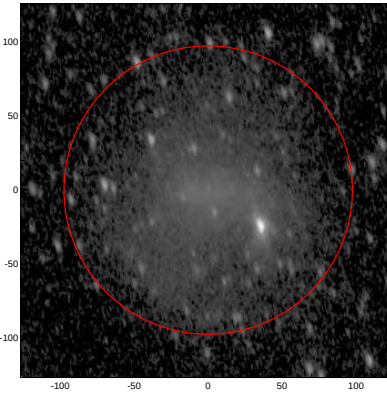
LEDA: pa,inc= 102.8 57.8
