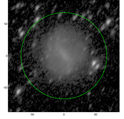
S4G: pa,inc= 56.8 58.0
