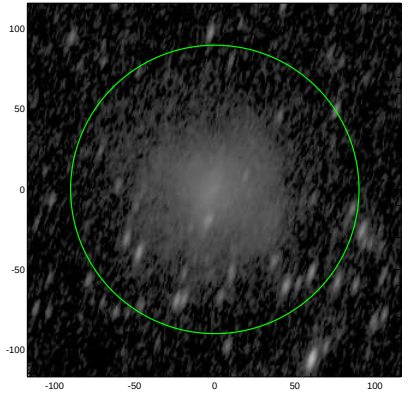
S4G: pa,inc= 72.4 68.1
