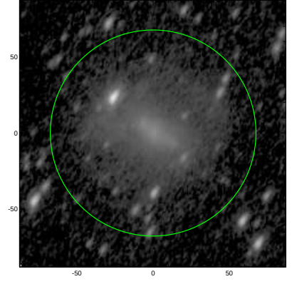
S4G: pa,inc= 63.0 58.0
