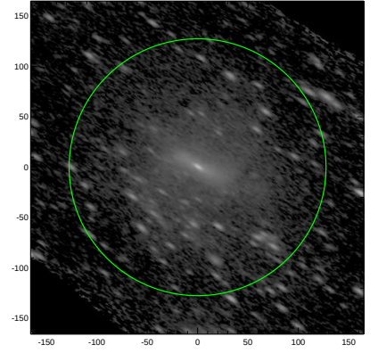
S4G: pa,inc= 146.7 68.9
