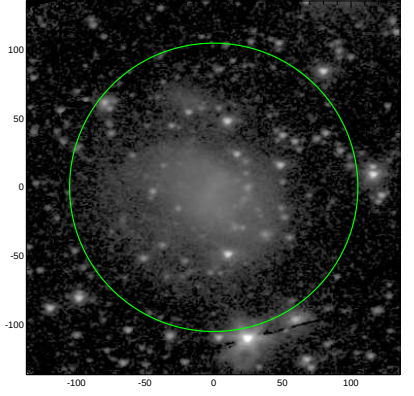
S4G: pa,inc= 6.6 38.6
