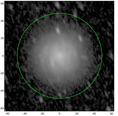
S4G: pa,inc= 113.8 58.3
