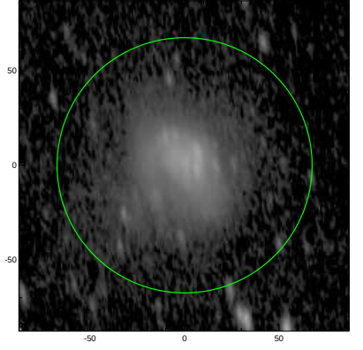
S4G: pa,inc= 100.0 67.5
