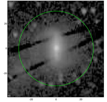
S4G: pa,inc= 91.9 25.5
