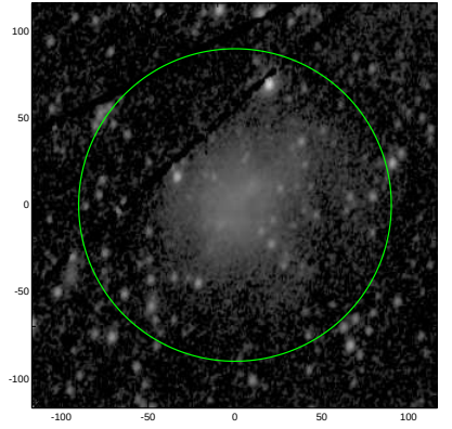
S4G: pa,inc= 75.8 42.2
