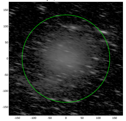
S4G: pa,inc= -14.9 77.2
