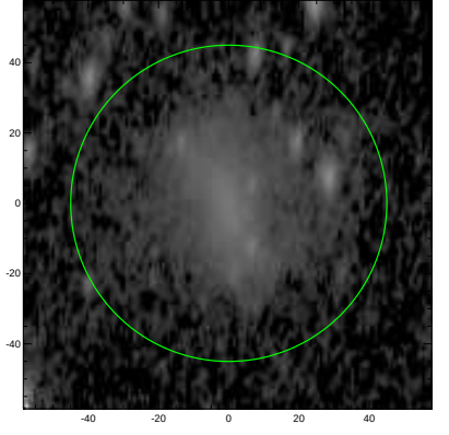
S4G: pa,inc= 85.8 61.6
