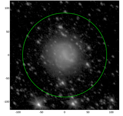
S4G: pa,inc= 136.7 47.0
