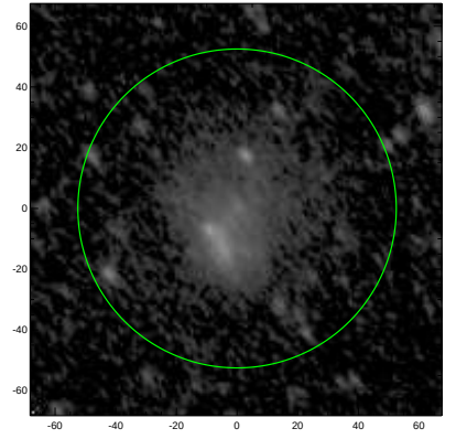
S4G: pa,inc= 127.7 53.4
