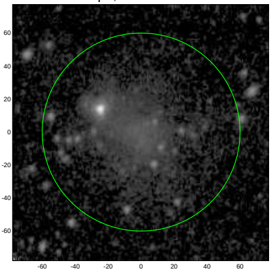
S4G: pa,inc= 77.7 29.3
