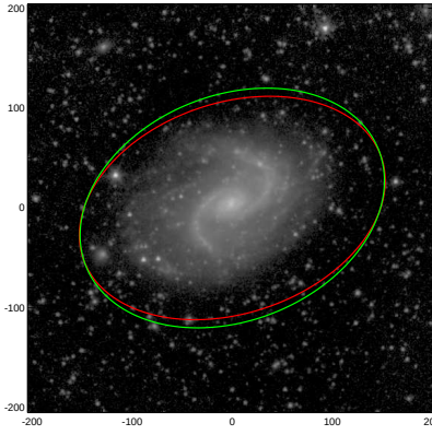
NGC0895
