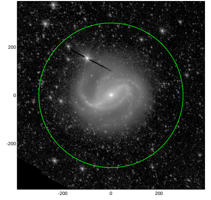
S4G: pa,inc= 125.9 38.9
