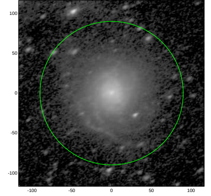
S4G: pa,inc= 27.5 54.1
