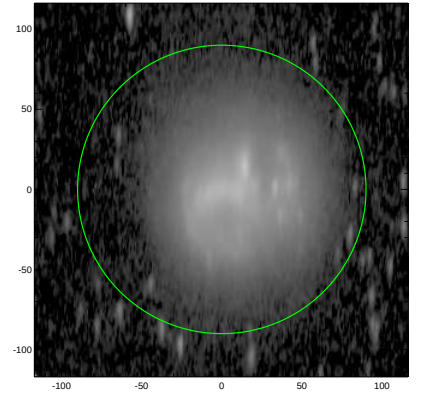
S4G: pa,inc= 88.6 72.9
