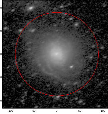
LEDA: pa,inc= 21.2 52.8
