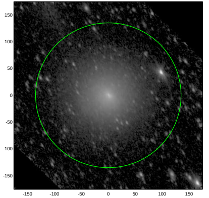
S4G: pa,inc= 121.8 56.8
