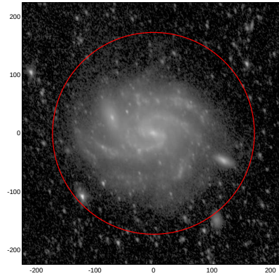
LEDA: pa,inc= 113.9 52.7
