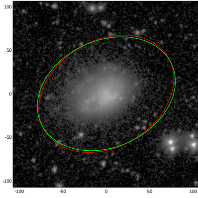
NGC0899
