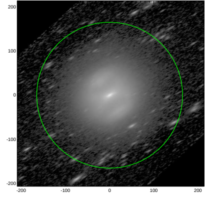
S4G: pa,inc= 29.2 73.6
