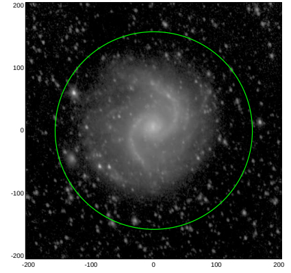
S4G: pa,inc= 111.7 44.3
