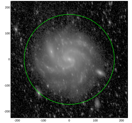
S4G: pa,inc= 107.6 57.6
