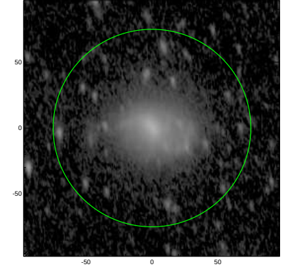
S4G: pa,inc= 101.0 60.6
