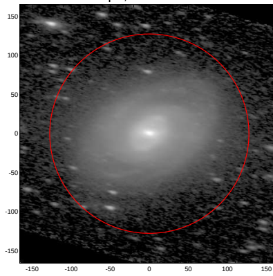
LEDA: pa,inc= 167.8 68.6
