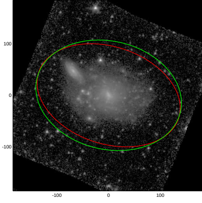
NGC0450
