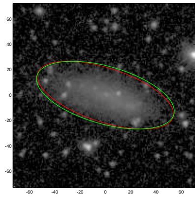
NGC0986A
