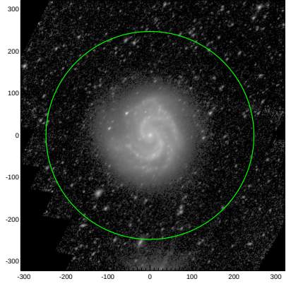
S4G: pa,inc= 44.0 48.0
