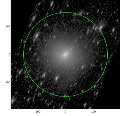
S4G: pa,inc= 65.7 63.2
