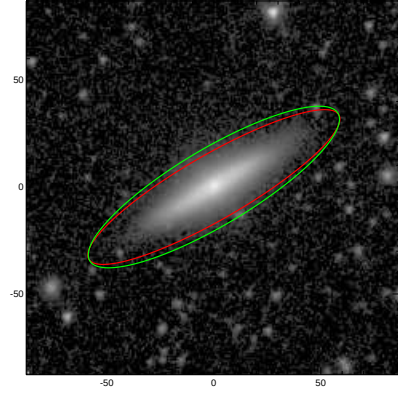
NGC0489
