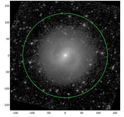
S4G: pa,inc= 14.8 32.2
