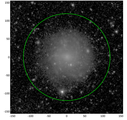
S4G: pa,inc= 118.3 19.0
