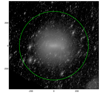
S4G: pa,inc= 68.9 62.8
