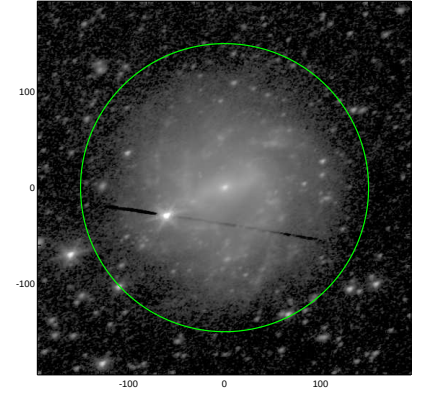
S4G: pa,inc= 26.1 47.0
