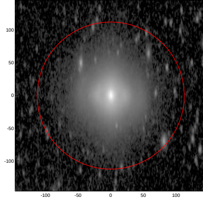
LEDA: pa,inc= 90.4 68.8
