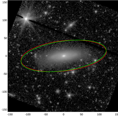
NGC0518
