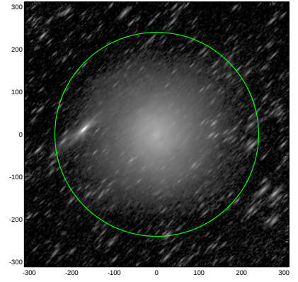
S4G: pa,inc= 44.7 75.1
