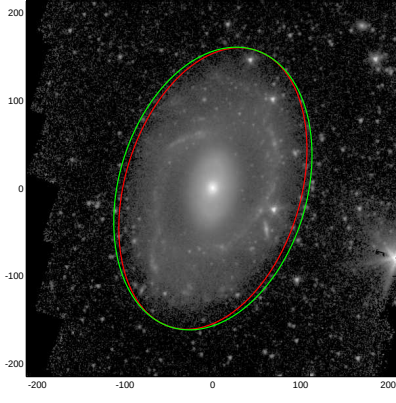
NGC0210
