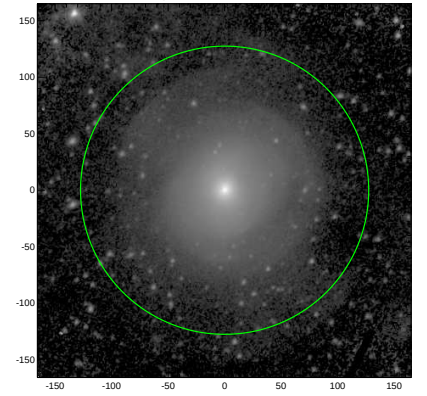
S4G: pa,inc= 56.5 23.0
