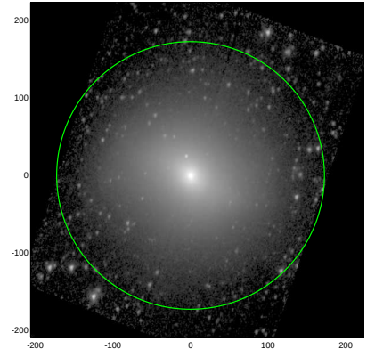
S4G: pa,inc= 76.3 39.2
