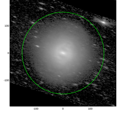
S4G: pa,inc= -19.3 70.3
