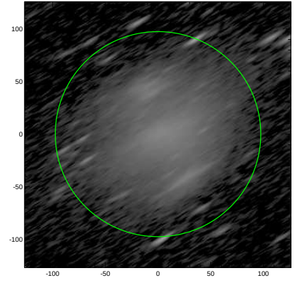
S4G: pa,inc= 31.0 79.0
