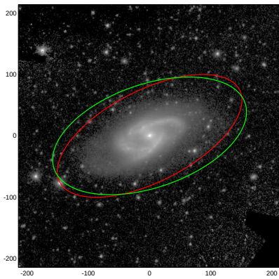
NGC0150
