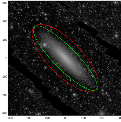
NGC0024
