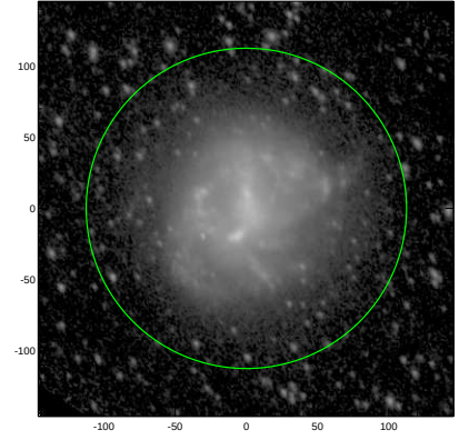
S4G: pa,inc= 119.6 44.5
