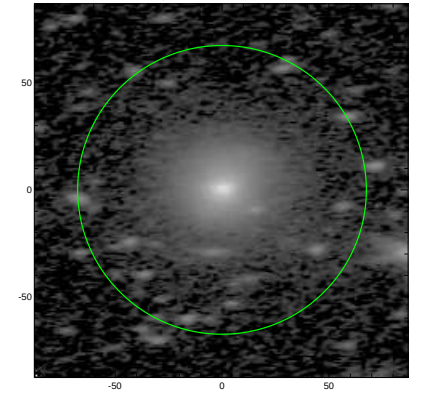
S4G: pa,inc= 4.5 65.0
