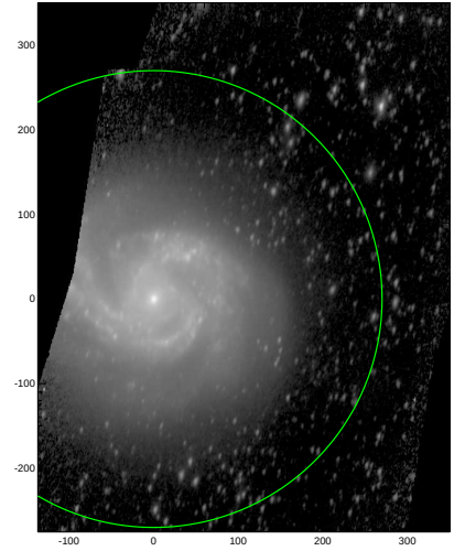
S4G: pa,inc= 77.3 58.1
