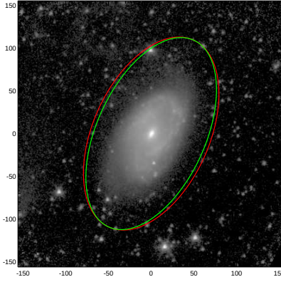
NGC0470
