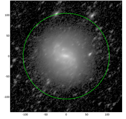
S4G: pa,inc= 44.7 58.6
