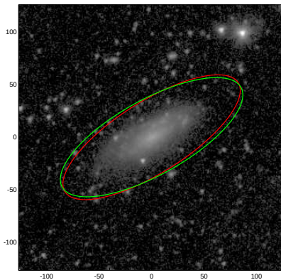
NGC0115
