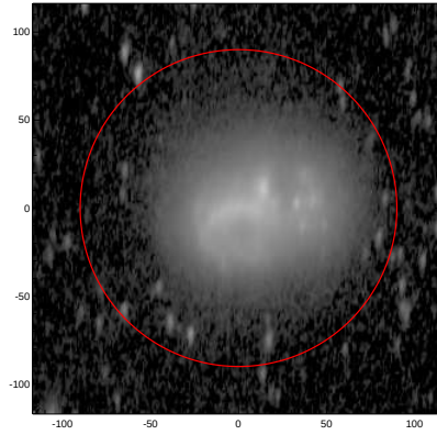
LEDA: pa,inc= 86.4 66.1
