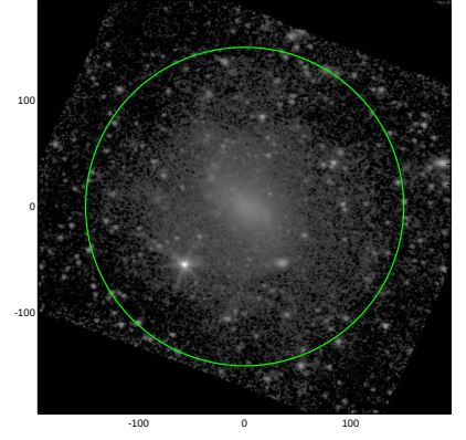
S4G: pa,inc= -14.2 33.5
