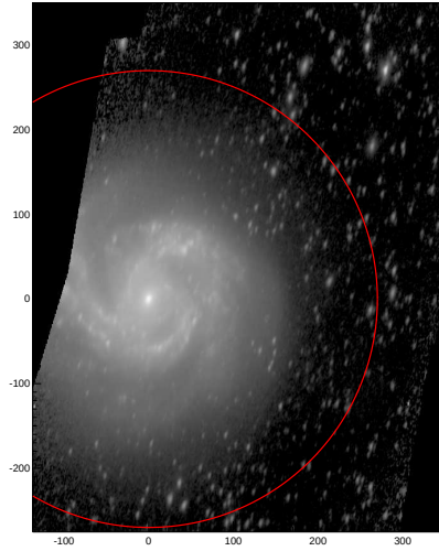
LEDA: pa,inc= 76.8 62.7
