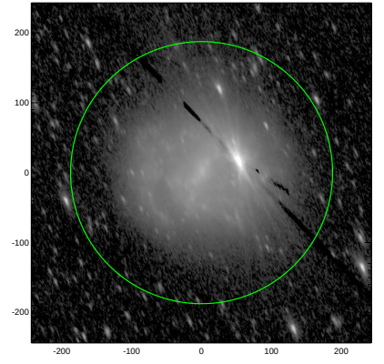
S4G: pa,inc= 114.8 67.9
