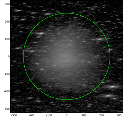
S4G: pa,inc= 1.4 76.1
