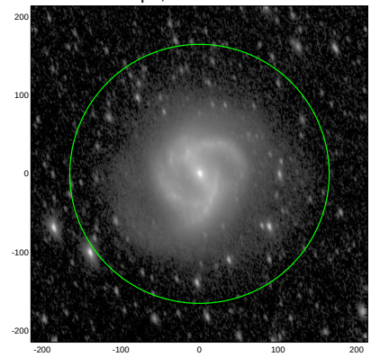
S4G: pa,inc= 108.9 59.3
