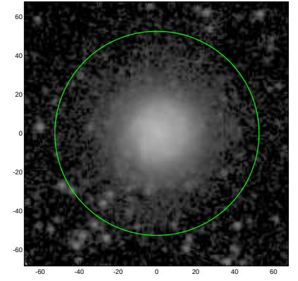
S4G: pa,inc= 151.9 14.8
