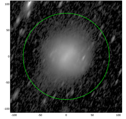
S4G: pa,inc= 63.1 68.8
