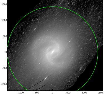
S4G: pa,inc= 51.3 78.9
