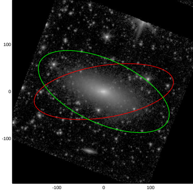
NGC0855
