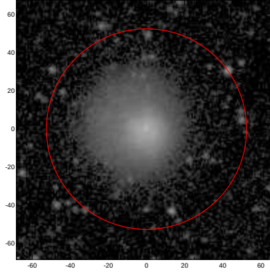
LEDA: pa,inc= 999.0 0.0
