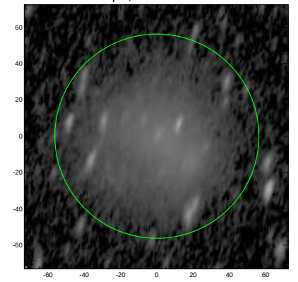
S4G: pa,inc= 74.2 66.2
