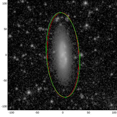
NGC0485
