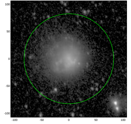
S4G: pa,inc= 114.4 42.0
