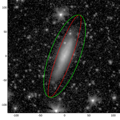
NGC0865
