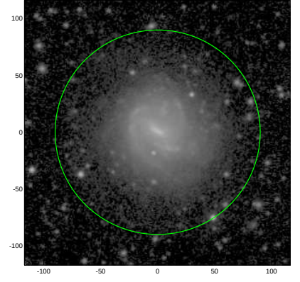
S4G: pa,inc= -4.8 24.2
