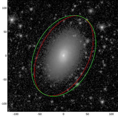
NGC0473
