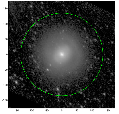
S4G: pa,inc= 131.4 48.5
