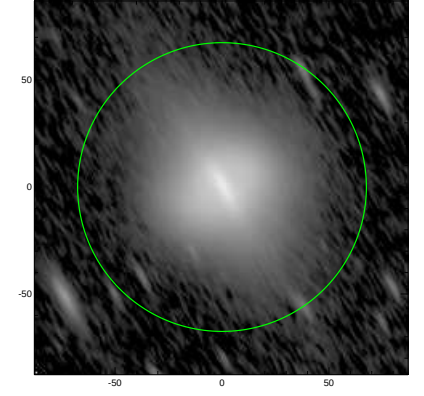
S4G: pa,inc= 120.8 74.6
