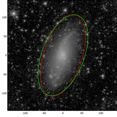
NGC0406
