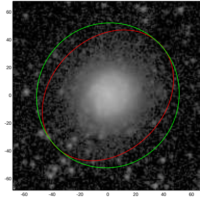
NGC0723
