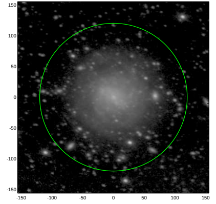
S4G: pa,inc= -13.4 44.2
