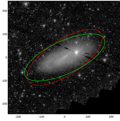
NGC0988
