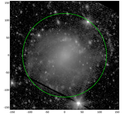
S4G: pa,inc= 111.2 29.6
