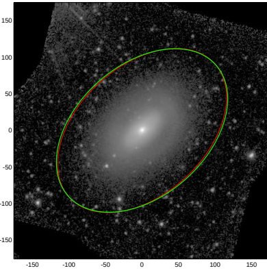
NGC0254
