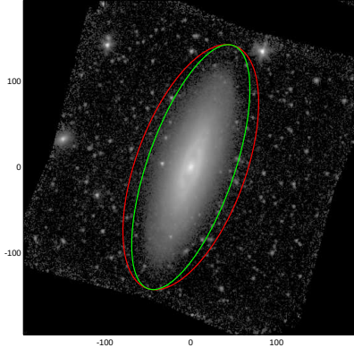
NGC0779
