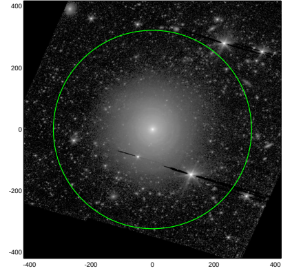
S4G: pa,inc= 10.9 32.3
