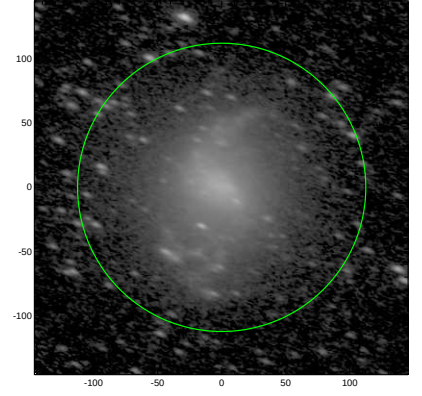
S4G: pa,inc= 159.0 60.4
