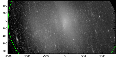
S4G: pa,inc= 108.0 79.0
