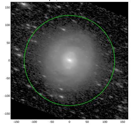
S4G: pa,inc= 158.3 66.0
