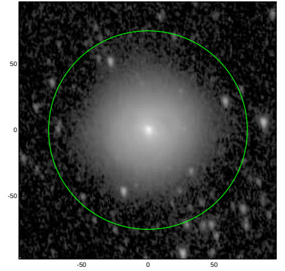
S4G: pa,inc= 102.9 49.6
