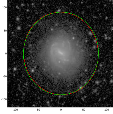
NGC0255
