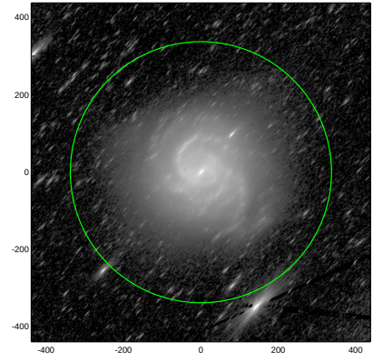
S4G: pa,inc= 46.9 73.8
