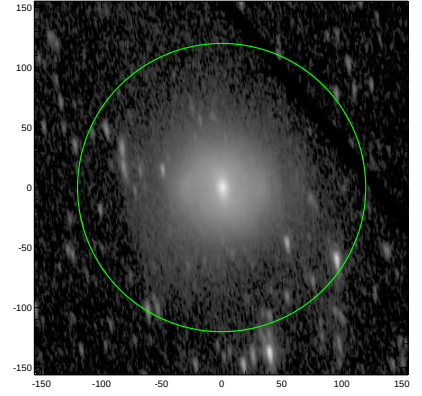
S4G: pa,inc= 98.3 69.9
