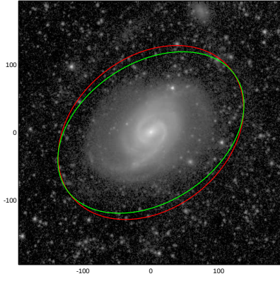
NGC0289
