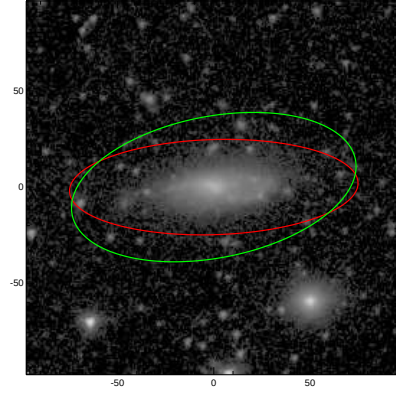
NGC0298
