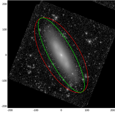
NGC0532
