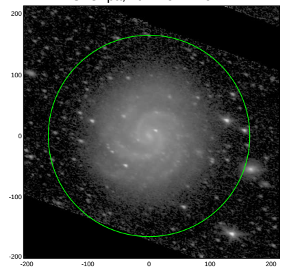
S4G: pa,inc= 157.7 54.1
