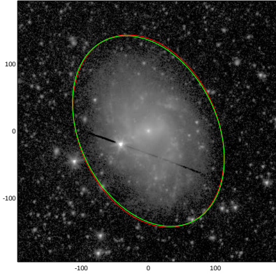
NGC0864
