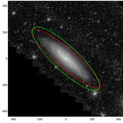
NGC0134
