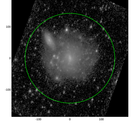
S4G: pa,inc= 76.8 42.6
