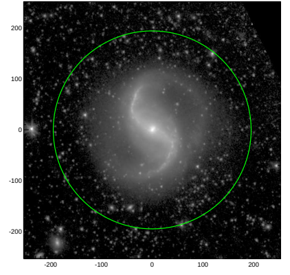
S4G: pa,inc= 107.6 26.0
