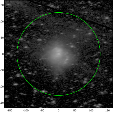
S4G: pa,inc= 1.3 58.9
