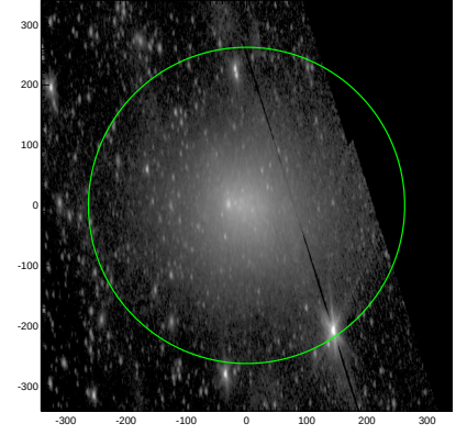
S4G: pa,inc= 94.2 68.1
