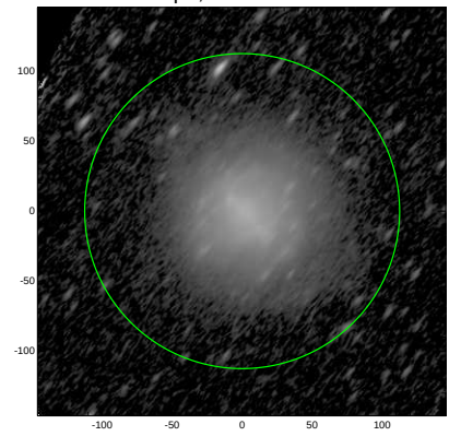
S4G: pa,inc= 49.8 68.3
