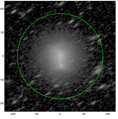
S4G: pa,inc= 29.4 66.8
