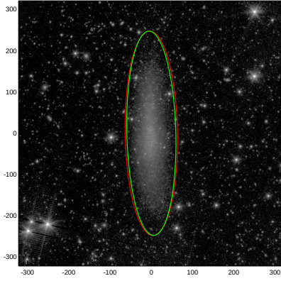
NGC0784
