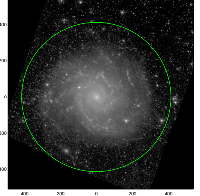
S4G: pa,inc= 141.1 30.9
