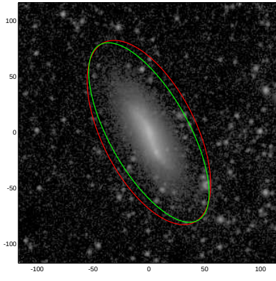
NGC0216
