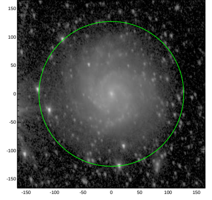
S4G: pa,inc= 104.4 48.6
