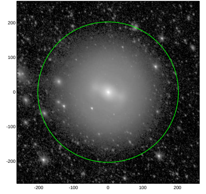
S4G: pa,inc= 126.6 42.4
