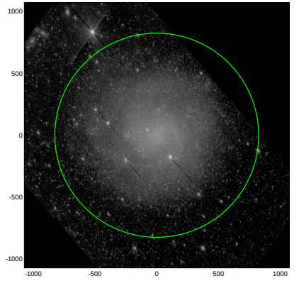
S4G: pa,inc= 115.5 44.9
