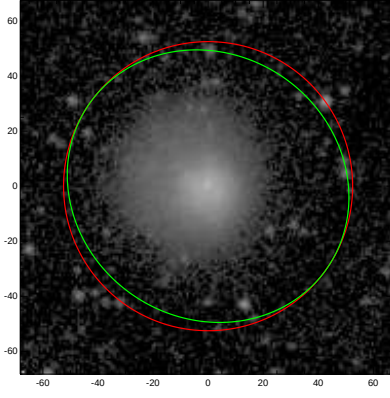
NGC0244
