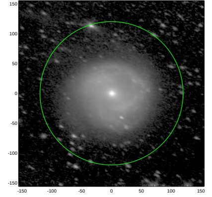
S4G: pa,inc= 155.4 58.0
