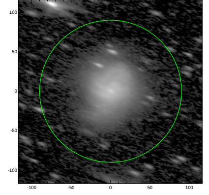
S4G: pa,inc= 159.2 70.0
