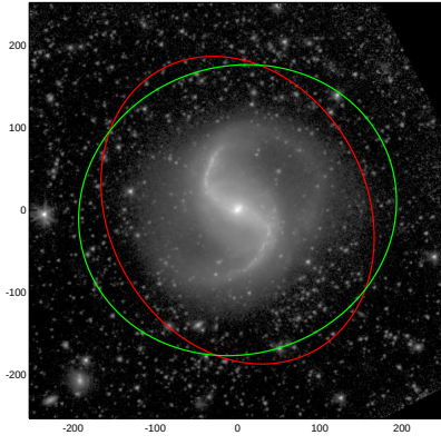
NGC0986
