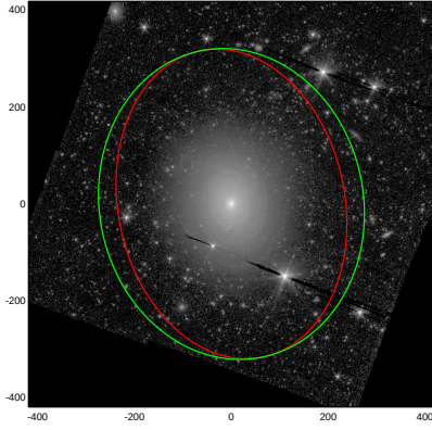
NGC0488
