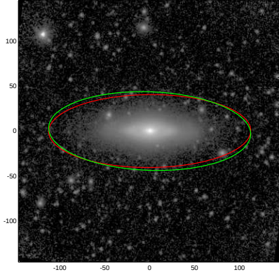
NGC0148
