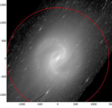
LEDA: pa,inc= 52.6 80.2
