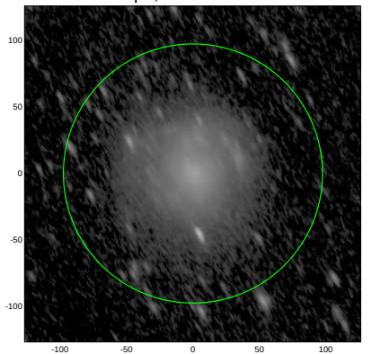
S4G: pa,inc= 119.1 68.6
