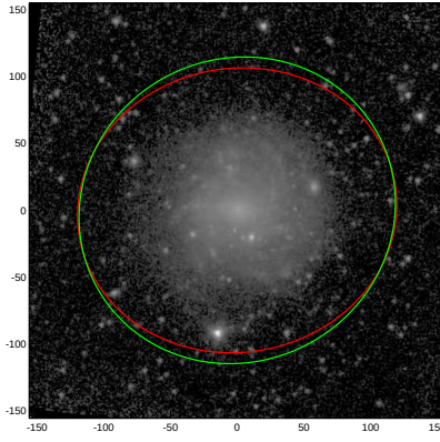
NGC0991
