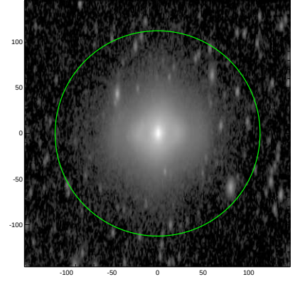
S4G: pa,inc= 87.9 67.1
