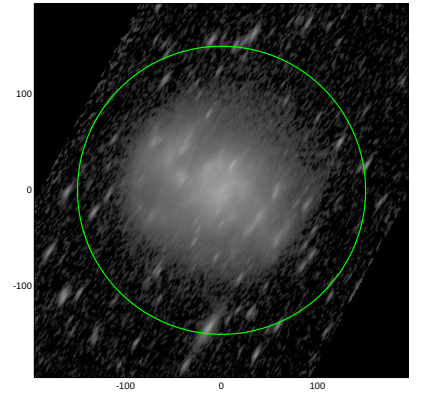
S4G: pa,inc= 57.4 72.7
