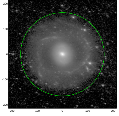
S4G: pa,inc= -16.6 49.5
