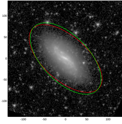
NGC0701
