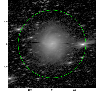
S4G: pa,inc= 10.4 67.2
