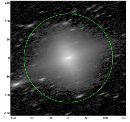
S4G: pa,inc= 18.8 73.1
