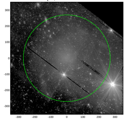
S4G: pa,inc= 129.3 34.4
