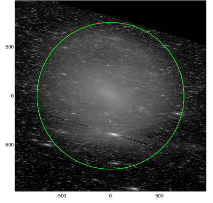
S4G: pa,inc= -9.2 75.5
