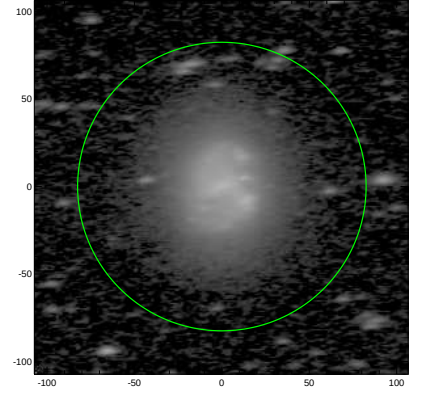
S4G: pa,inc= 4.1 67.0
