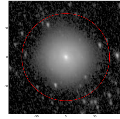
LEDA: pa,inc= 105.3 52.6
