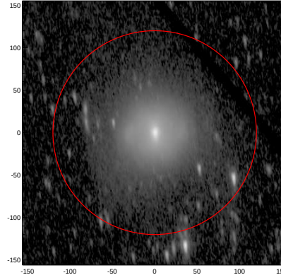
LEDA: pa,inc= 96.5 69.4
