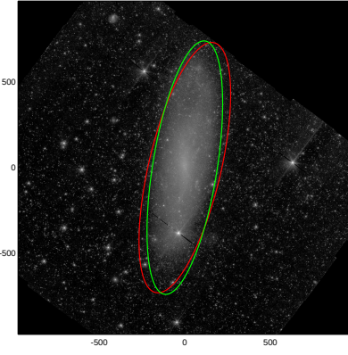
NGC0247
