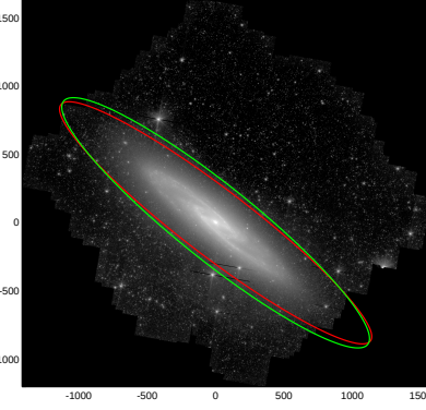
NGC0253
