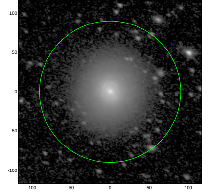
S4G: pa,inc= 153.2 48.2
