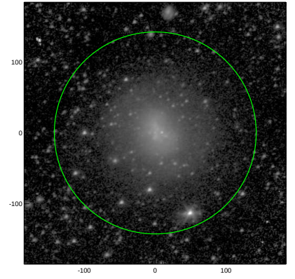
S4G: pa,inc= 23.4 32.4
