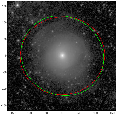
NGC0474
