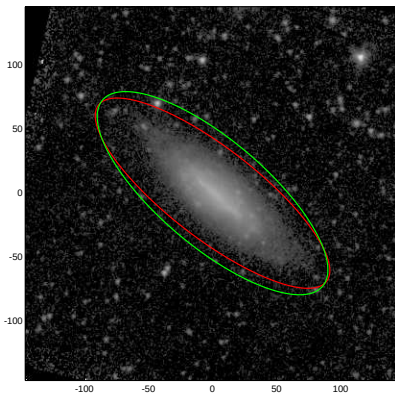
NGC0755
