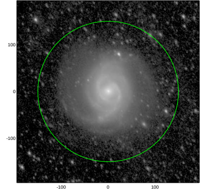
S4G: pa,inc= 123.7 47.0
