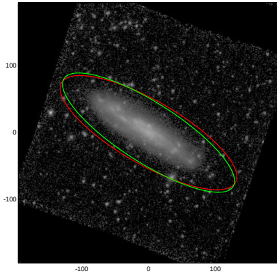
NGC0493
