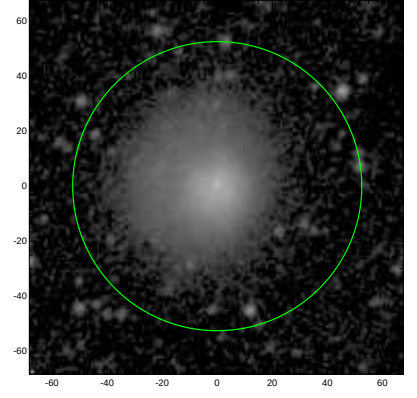
S4G: pa,inc= 55.9 23.7
