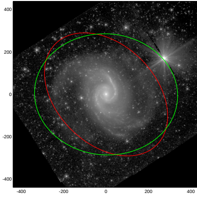
NGC1566
