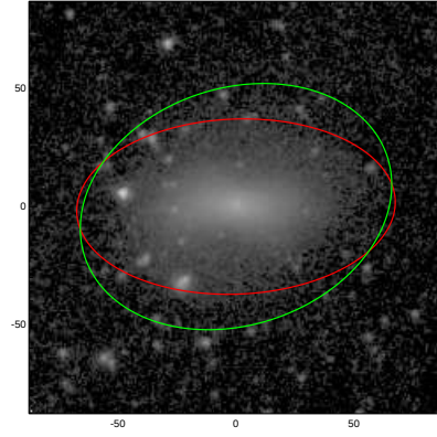
NGC1047
