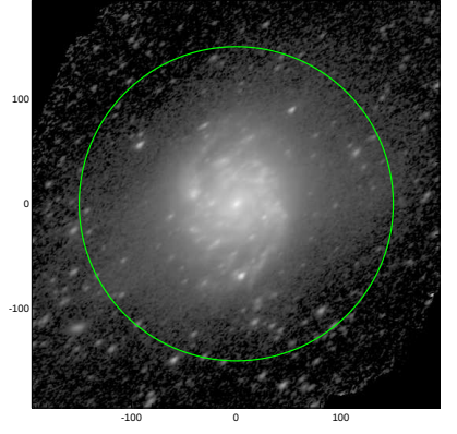
S4G: pa,inc= 38.4 57.2
