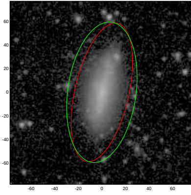
NGC1556
