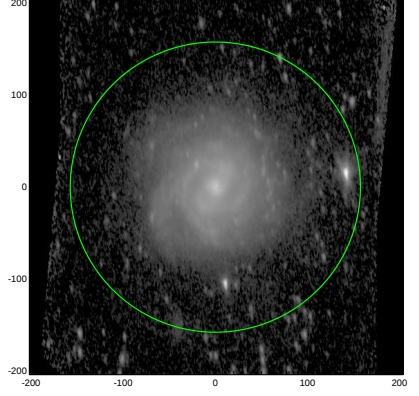
S4G: pa,inc= 98.0 63.8
