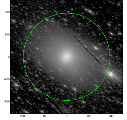
S4G: pa,inc= 147.4 63.9
