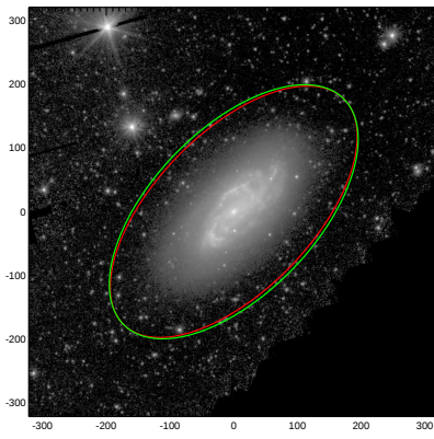
NGC1792
