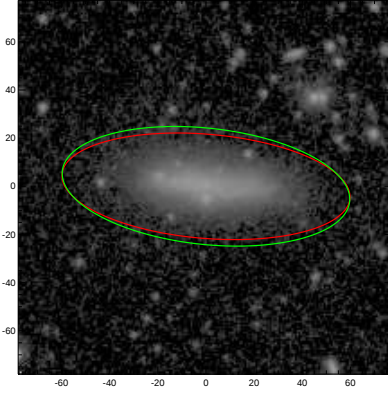
NGC1476
