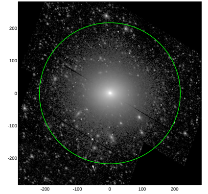
S4G: pa,inc= 131.5 40.9
