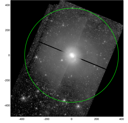
S4G: pa,inc= 61.6 16.3
