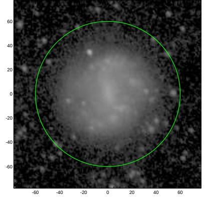
S4G: pa,inc= 125.7 36.0
