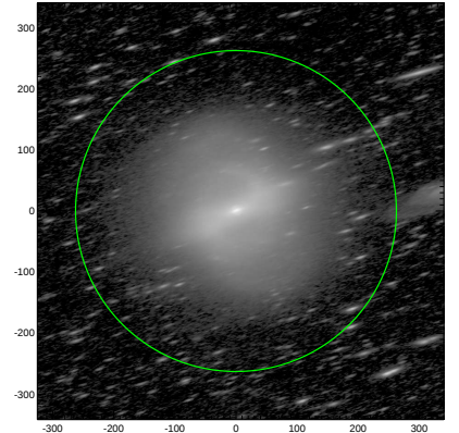
S4G: pa,inc= 17.7 75.1
