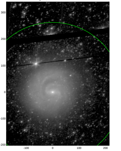
S4G: pa,inc= 32.7 38.8
