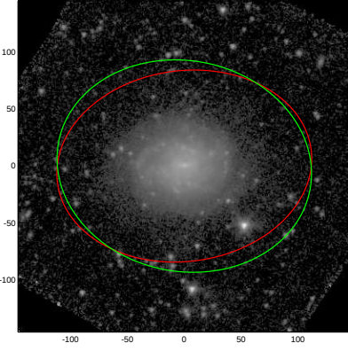
NGC1310
