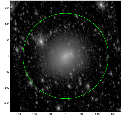
S4G: pa,inc= 105.0 51.9
