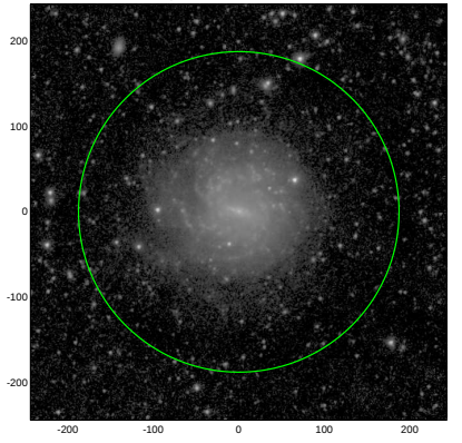
S4G: pa,inc= 49.5 10.2
