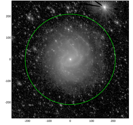
S4G: pa,inc= 122.6 42.5
