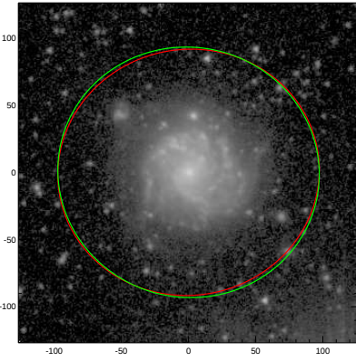
NGC1309
