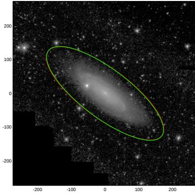
NGC1325
