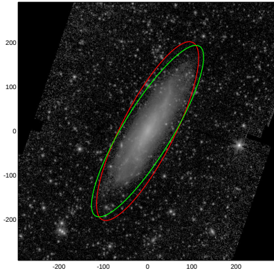
NGC1337
