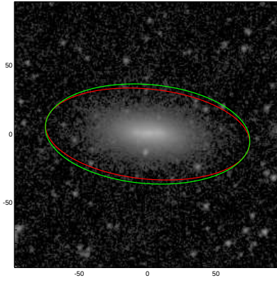
NGC1316C
