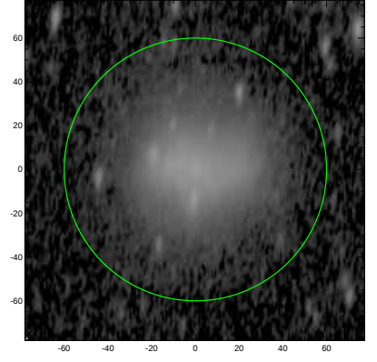
S4G: pa,inc= 83.9 66.3
