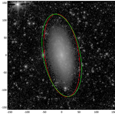
NGC1292
