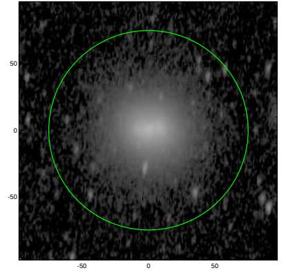
S4G: pa,inc= 85.1 61.2
