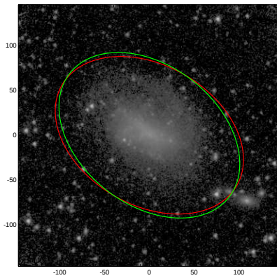
NGC1879
