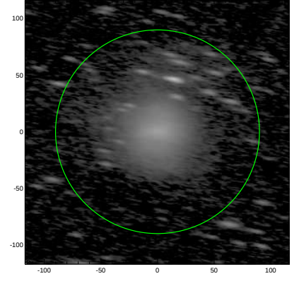
S4G: pa,inc= -10.2 74.6
