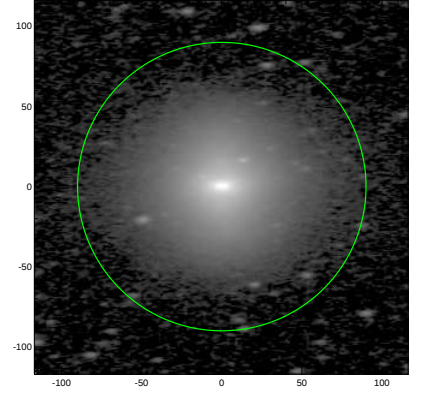
S4G: pa,inc= 2.2 64.1
