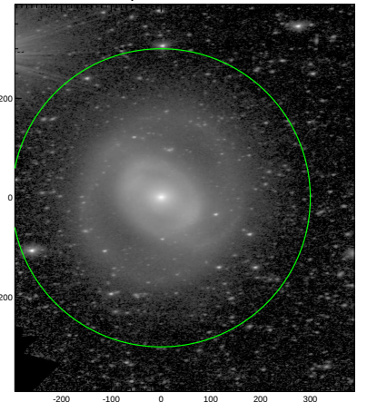
S4G: pa,inc= 4.7 58.2
