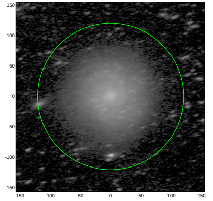
S4G: pa,inc= 11.2 63.6
