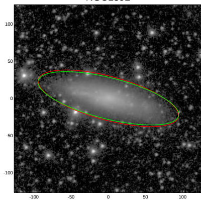
NGC1892
