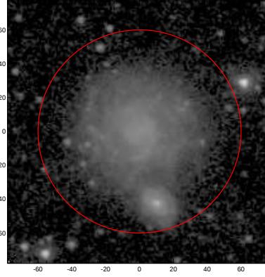
LEDA: pa,inc= 162.8 26.2
