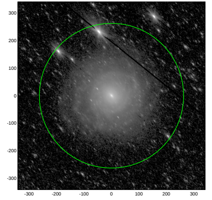
S4G: pa,inc= 131.5 63.7
