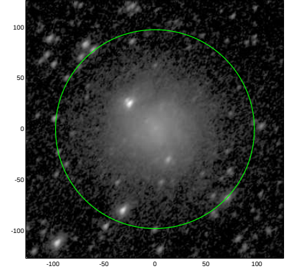
S4G: pa,inc= 49.2 50.7
