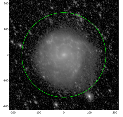
S4G: pa,inc= 123.2 52.0
