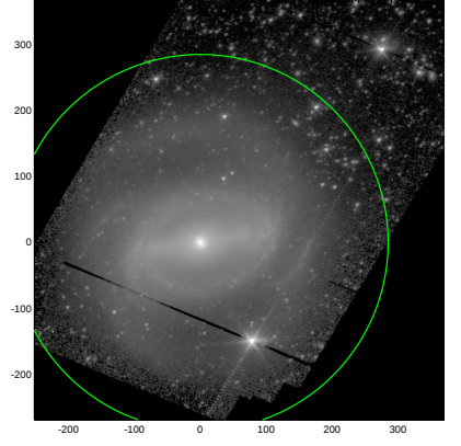
S4G: pa,inc= 24.3 30.6
