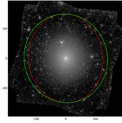
NGC1297
