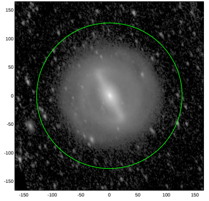
S4G: pa,inc= 113.7 53.3
