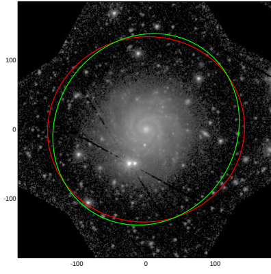
NGC1703
