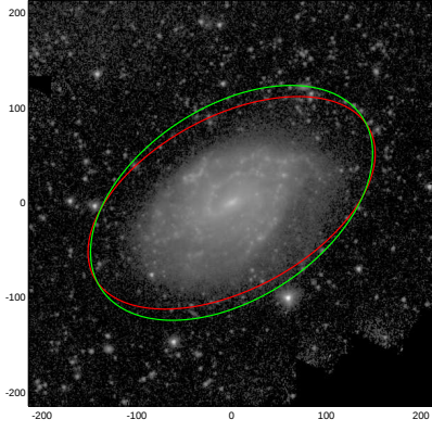
NGC1255
