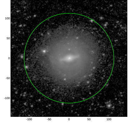
S4G: pa,inc= 12.5 30.5
