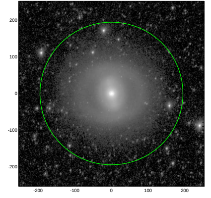
S4G: pa,inc= 80.4 37.2
