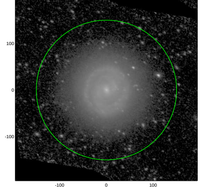
S4G: pa,inc= 148.2 45.1
