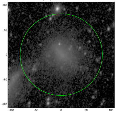
S4G: pa,inc= 76.0 40.1
