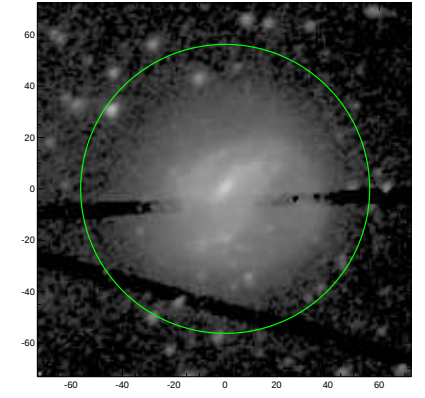
S4G: pa,inc= 40.5 30.0
