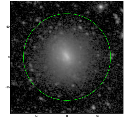
S4G: pa,inc= 158.9 31.4
