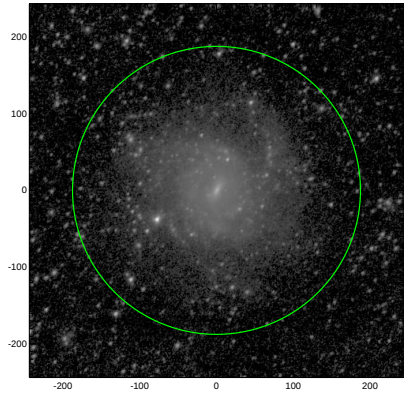
S4G: pa,inc= 49.0 34.4
