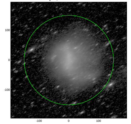
S4G: pa,inc= 32.1 65.3
