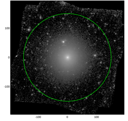
S4G: pa,inc= 13.6 20.6
