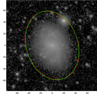
NGC1258
