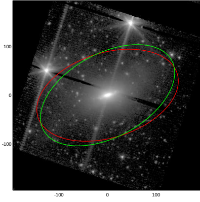
NGC1482
