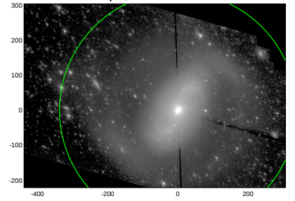
S4G: pa,inc= 125.8 43.0
