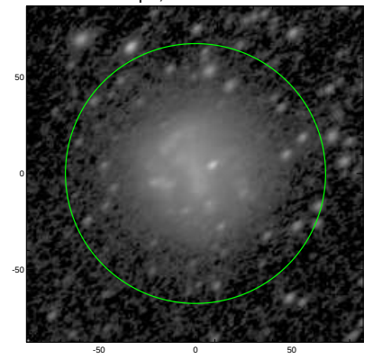
S4G: pa,inc= 40.7 49.9
