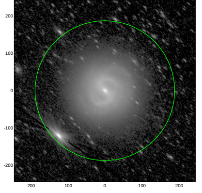
S4G: pa,inc= 137.3 65.2
