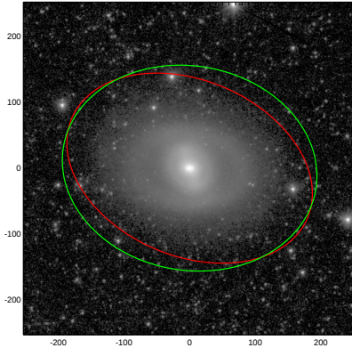
NGC1326
