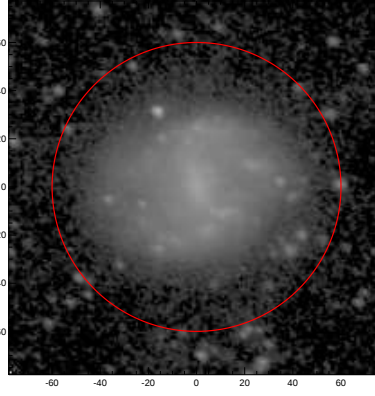
LEDA: pa,inc= 152.6 36.2
