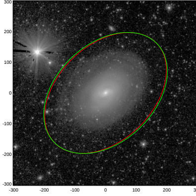
NGC1367
