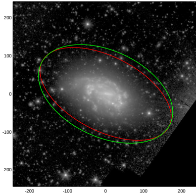
NGC1559
