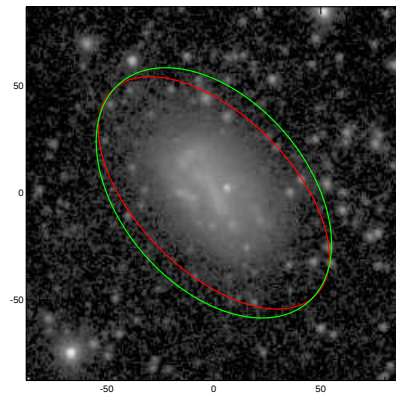
NGC1473
