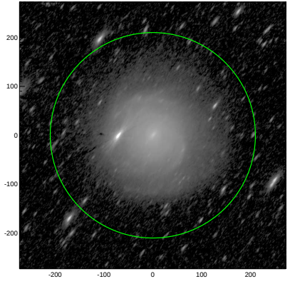
S4G: pa,inc= 53.0 69.8
