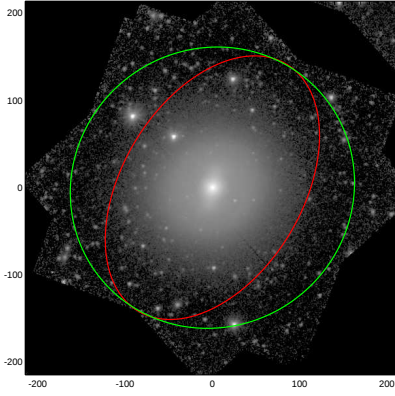
NGC1533
