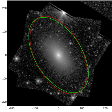
NGC1389
