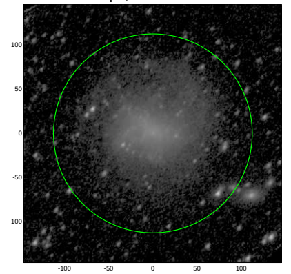
S4G: pa,inc= 52.3 46.3
