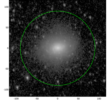
S4G: pa,inc= 101.1 42.3
