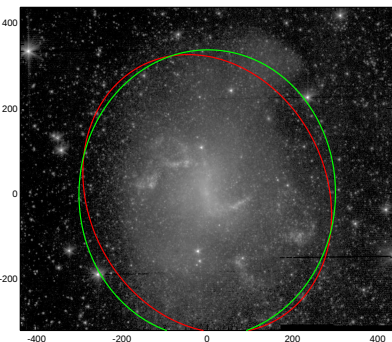
NGC1313
