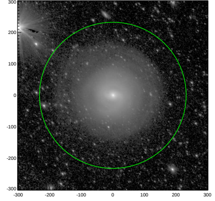
S4G: pa,inc= 133.4 46.5
