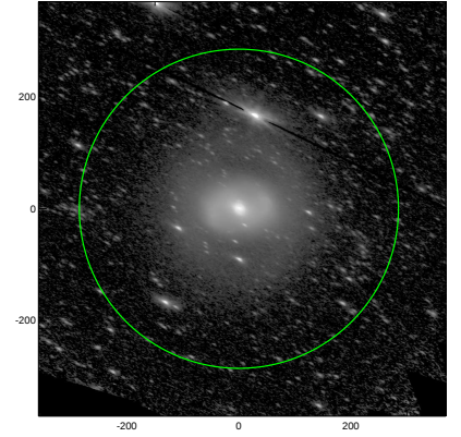
S4G: pa,inc= 152.3 66.3
