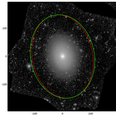
NGC1411
