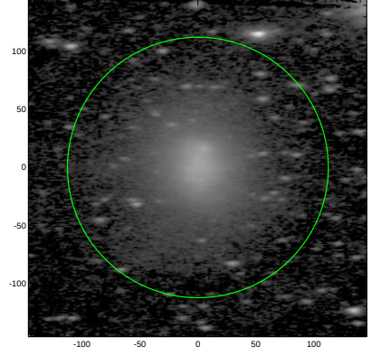
S4G: pa,inc= 1.2 66.2
