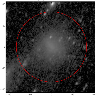
LEDA: pa,inc= 62.2 50.4
