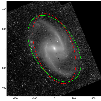
NGC1365
