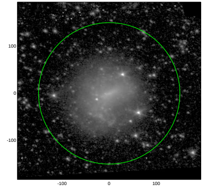
S4G: pa,inc= -13.1 35.9
