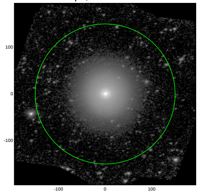
S4G: pa,inc= 11.0 41.0
