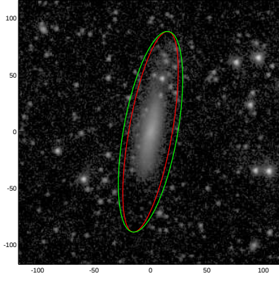
NGC1414
