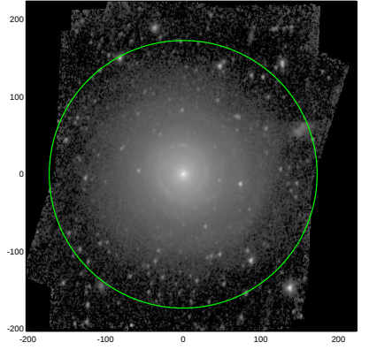
S4G: pa,inc= 81.0 37.8
