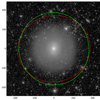
NGC1302
