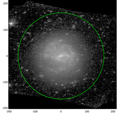
S4G: pa,inc= 1.4 50.5
