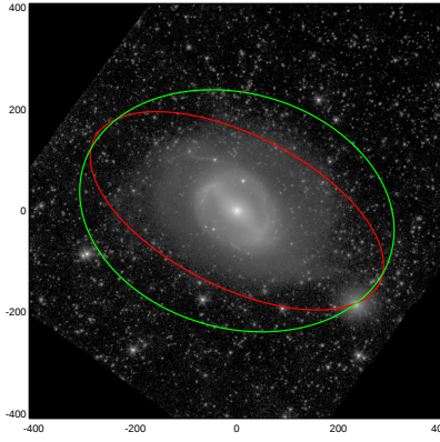
NGC1512
