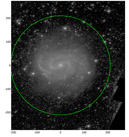
S4G: pa,inc= 6.7 38.8
