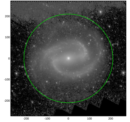
S4G: pa,inc= 106.1 33.4
