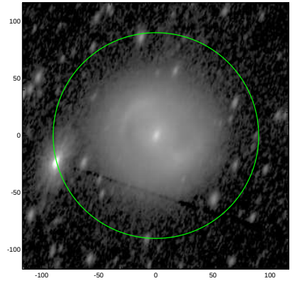
S4G: pa,inc= 69.4 61.4
