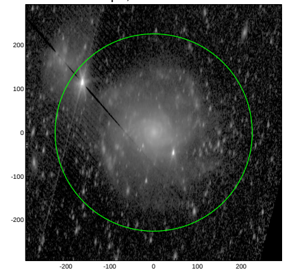
S4G: pa,inc= 84.5 66.1
