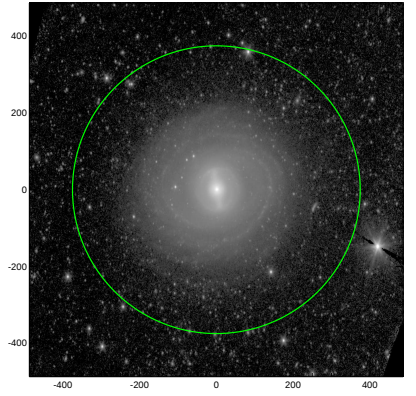
S4G: pa,inc= 93.4 42.2
