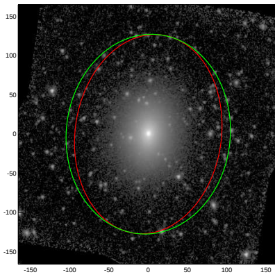
NGC1339
