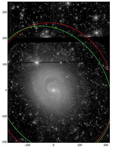
NGC1637
