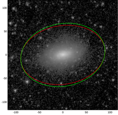
NGC1076
