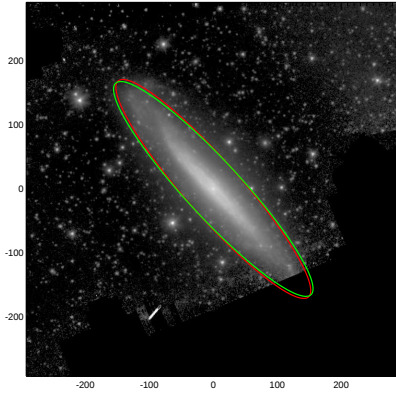
NGC1448
