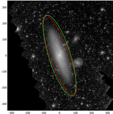
NGC1515
