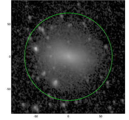
S4G: pa,inc= 108.4 42.0
