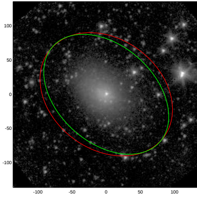
NGC1705
