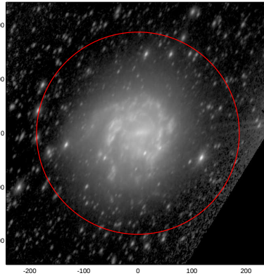
LEDA: pa,inc= 62.8 58.6
