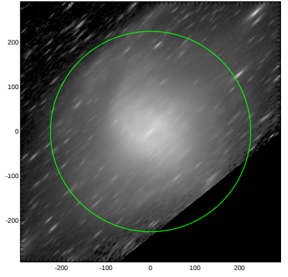
S4G: pa,inc= 42.7 78.9
