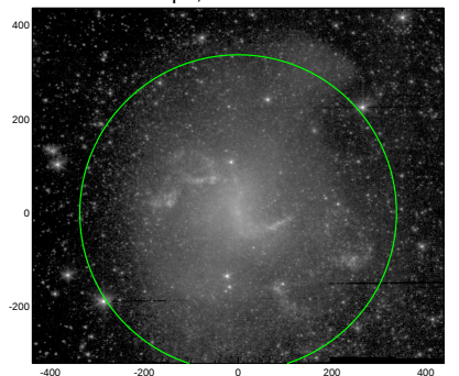
S4G: pa,inc= -1.5 27.0
