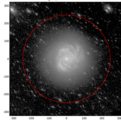
LEDA: pa,inc= 135.9 60.0
