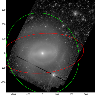
NGC1433
