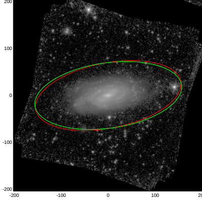
NGC1090
