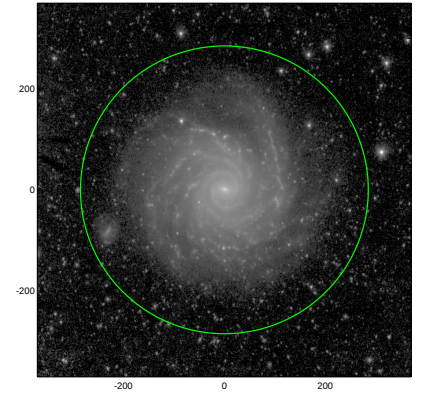
S4G: pa,inc= 94.1 31.4
