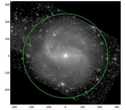
S4G: pa,inc= 148.5 26.6
