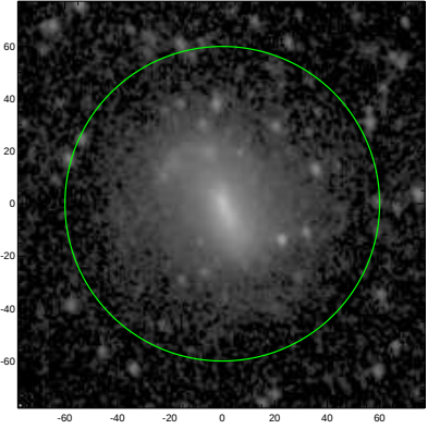
S4G: pa,inc= 105.9 32.2
