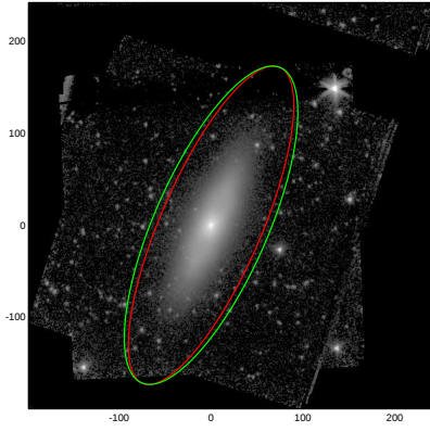
NGC1461
