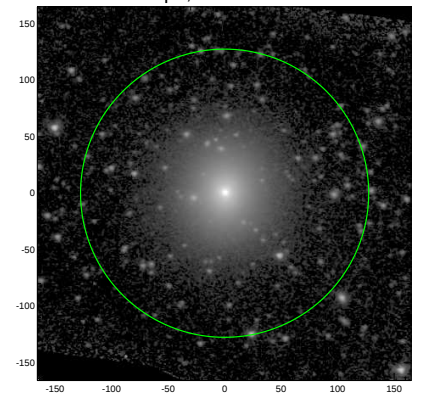
S4G: pa,inc= -5.6 34.9
