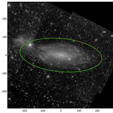
NGC1253
