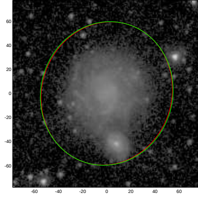
NGC1347
