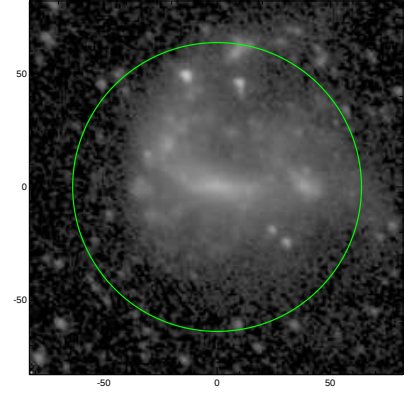
S4G: pa,inc= 135.2 36.3
