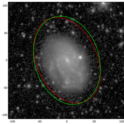
NGC2701
