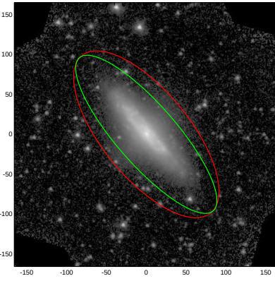
NGC2748
