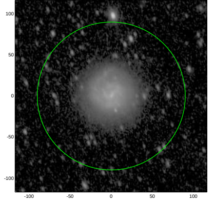
S4G: pa,inc= 107.4 49.2
