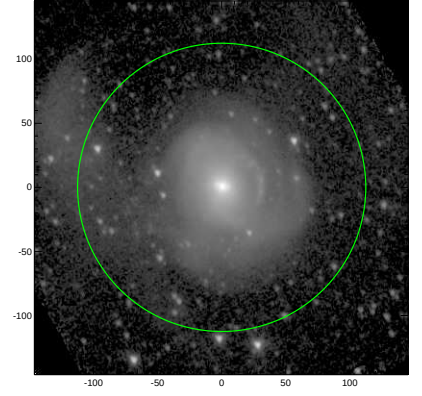
S4G: pa,inc= 108.9 33.0
