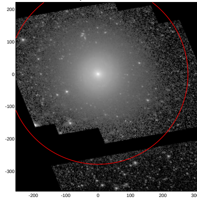
LEDA: pa,inc= 160.3 37.8
