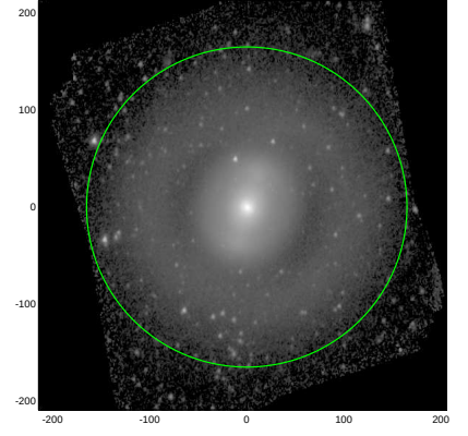
S4G: pa,inc= 81.8 37.2
