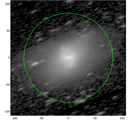
S4G: pa,inc= 22.0 70.7
