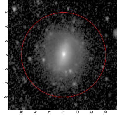
LEDA: pa,inc= 83.4 36.2
