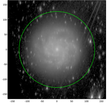
S4G: pa,inc= 86.5 60.0
