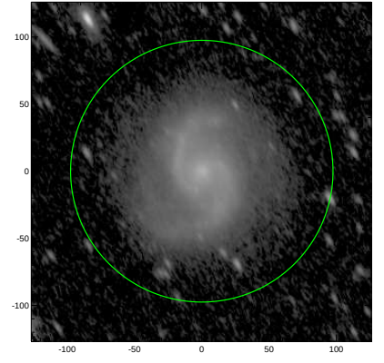
S4G: pa,inc= 118.6 63.9
