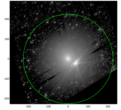
S4G: pa,inc= 47.2 45.8
