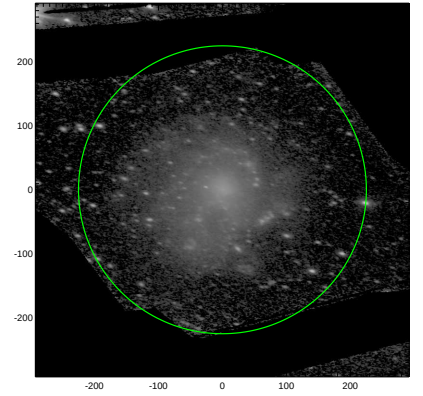
S4G: pa,inc= -12.2 59.2
