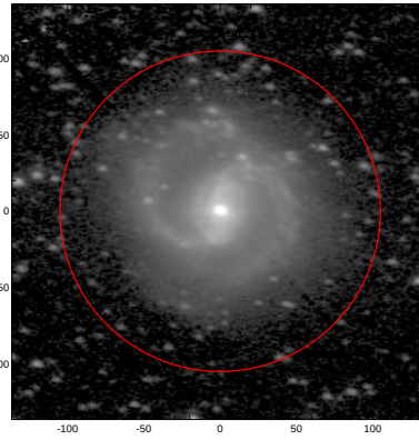
LEDA: pa,inc= 175.0 51.2
