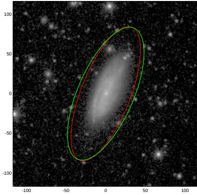
NGC2919
