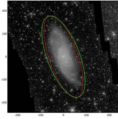
NGC2715
