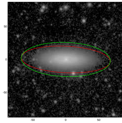
NGC2726
