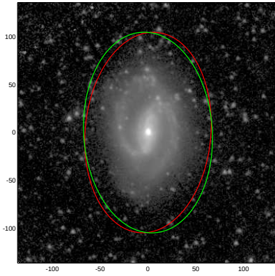
NGC2633
