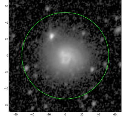
S4G: pa,inc= 70.3 41.9
