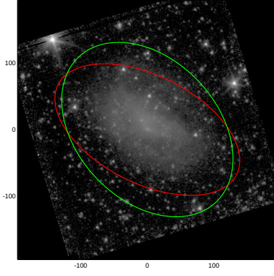
NGC2552
