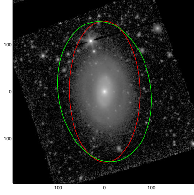
NGC2962
