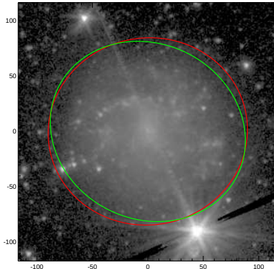
NGC2500
