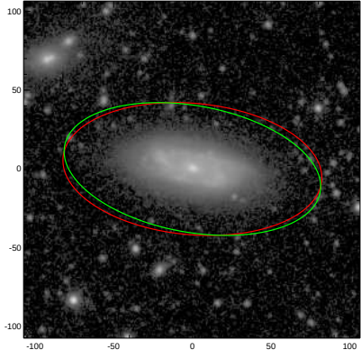
NGC2882
