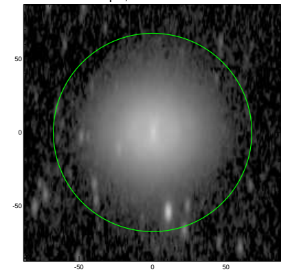
S4G: pa,inc= 88.2 67.4
