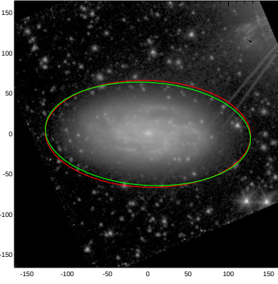
NGC2742
