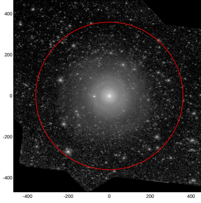
LEDA: pa,inc= 175.5 36.2
