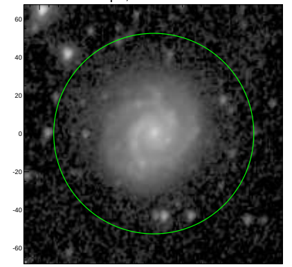
S4G: pa,inc= 70.4 32.9
