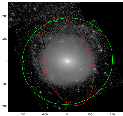
NGC2655
