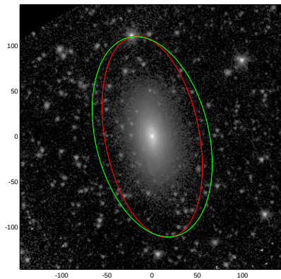
NGC2844
