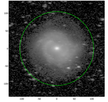
S4G: pa,inc= -0.5 60.6
