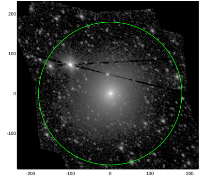
S4G: pa,inc= 136.3 44.2
