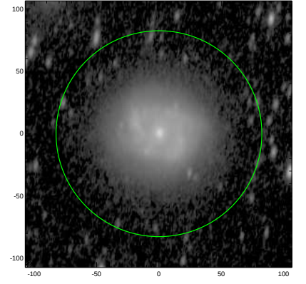
S4G: pa,inc= 79.8 60.9
