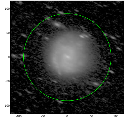
S4G: pa,inc= 156.6 66.9
