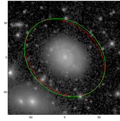
NGC2684
