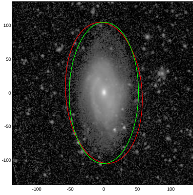
NGC2712
