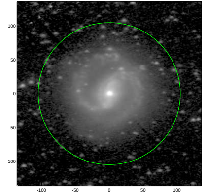
S4G: pa,inc= 3.7 50.1
