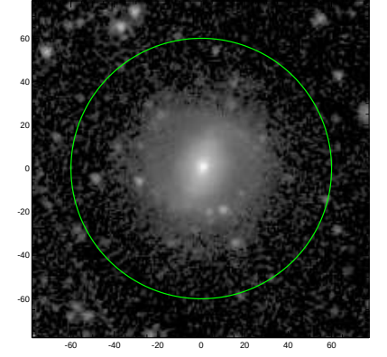
S4G: pa,inc= 49.1 17.4
