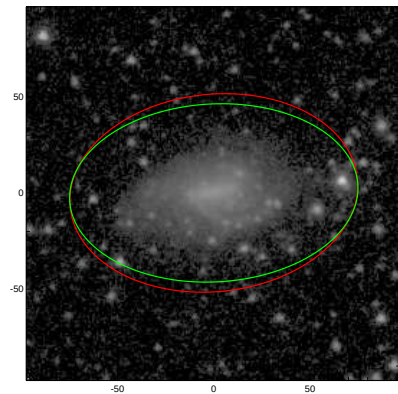
NGC2938
