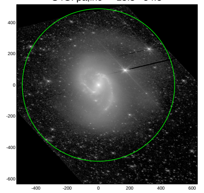
S4G: pa,inc= -13.8 54.3
