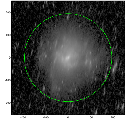
S4G: pa,inc= 78.5 76.1
