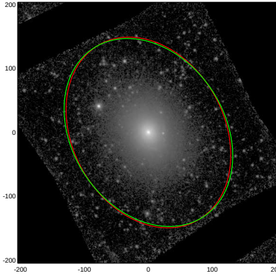
NGC3277
