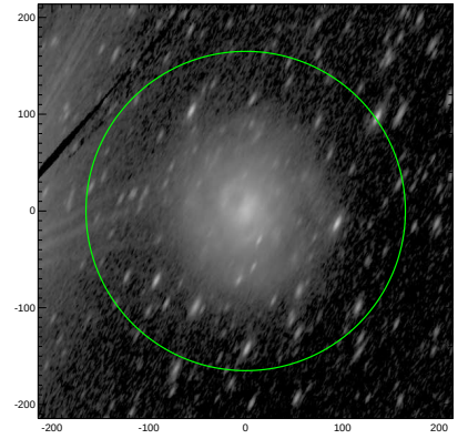
S4G: pa,inc= 63.6 71.7
