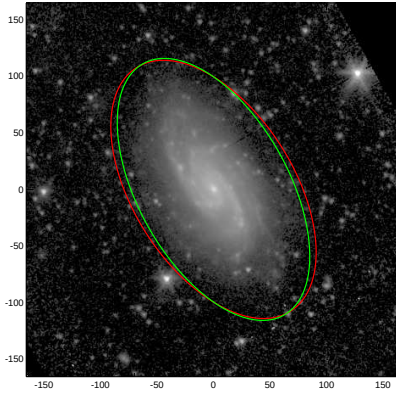
NGC3430
