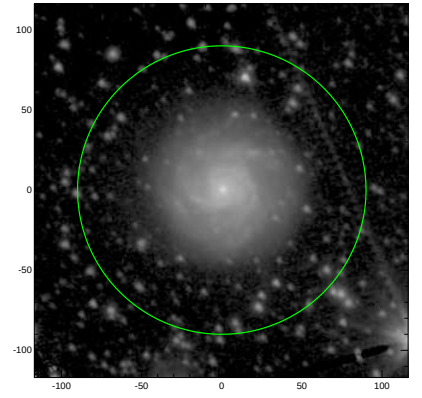
S4G: pa,inc= 135.5 31.3
