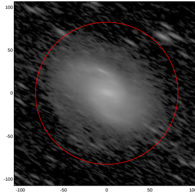
LEDA: pa,inc= 150.3 75.0
