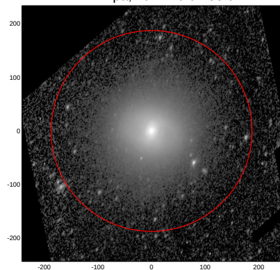
LEDA: pa,inc= 70.0 53.9
