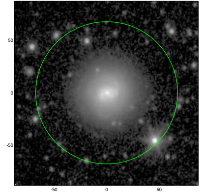
S4G: pa,inc= 79.2 24.7
