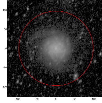
LEDA: pa,inc= 68.5 51.2
