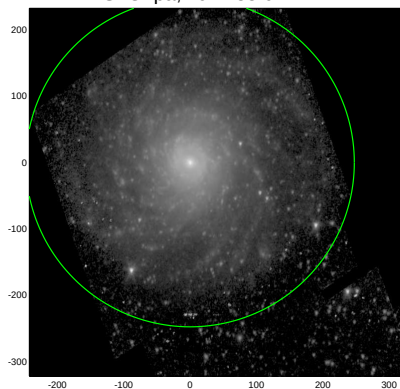
S4G: pa,inc= 83.6 42.1
