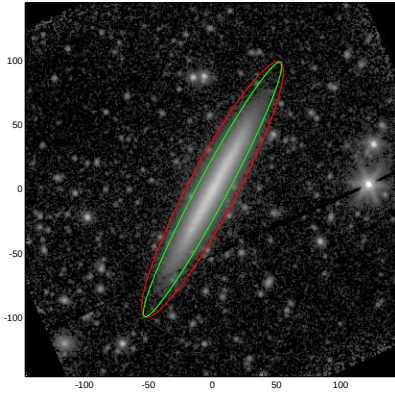
NGC3279
