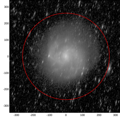
LEDA: pa,inc= 75.7 70.7
