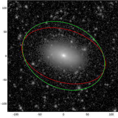
NGC3648
