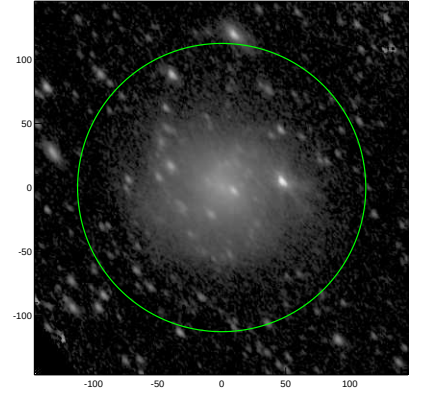
S4G: pa,inc= 124.8 54.2
