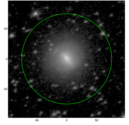
S4G: pa,inc= 22.9 43.9
