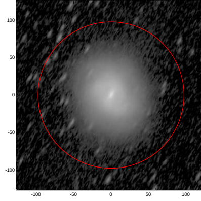
LEDA: pa,inc= 62.8 70.4
