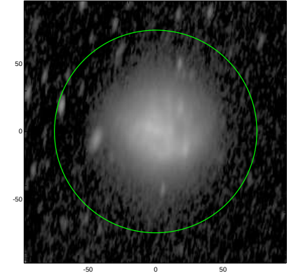
S4G: pa,inc= 80.3 69.9
