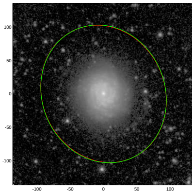
NGC3982
