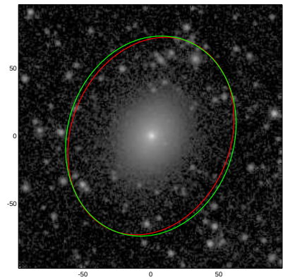
NGC3931
