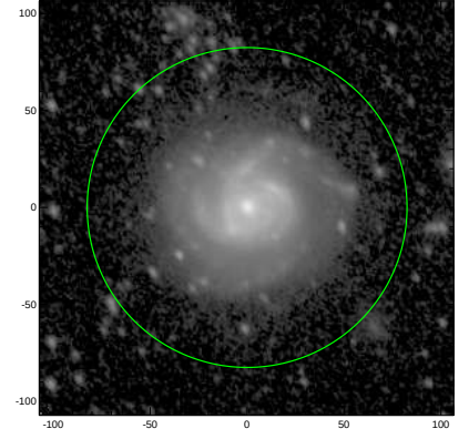
S4G: pa,inc= 121.2 41.8
