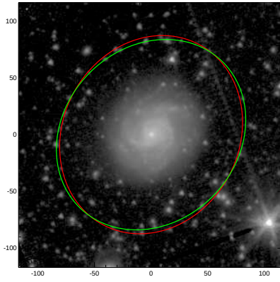
NGC3512
