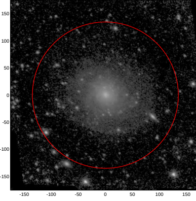
LEDA: pa,inc= 146.4 32.7
