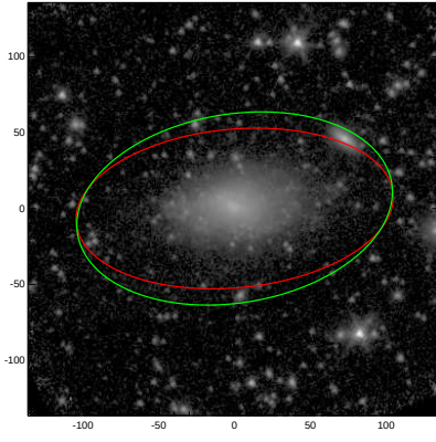
NGC3274
