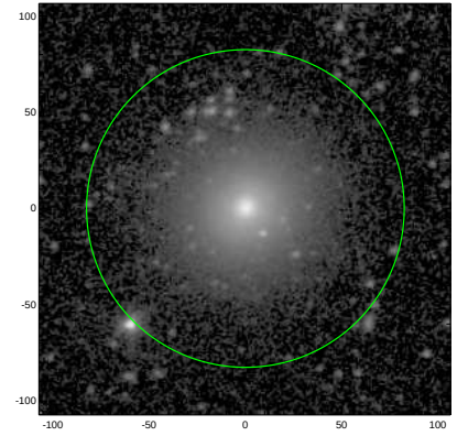
S4G: pa,inc= 30.9 25.9
