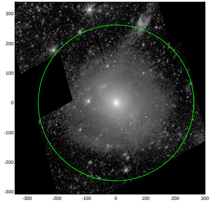
S4G: pa,inc= 56.3 39.0
