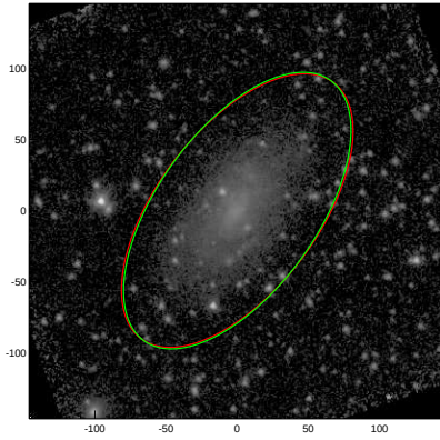
NGC3443
