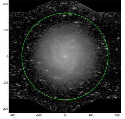
S4G: pa,inc= -0.9 59.2
