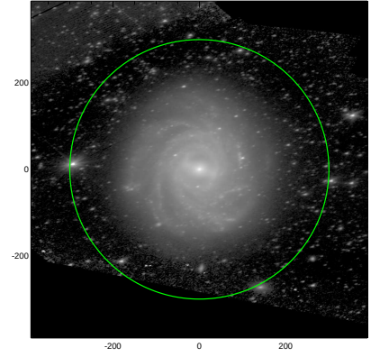
S4G: pa,inc= 14.0 58.4
