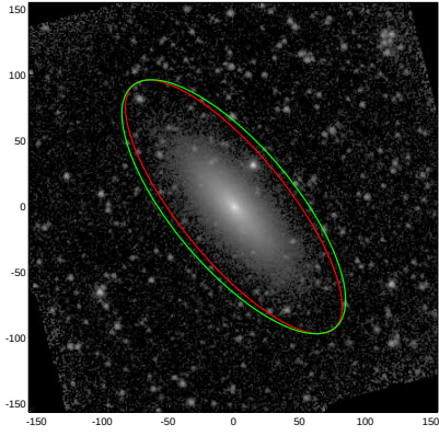
NGC3922
