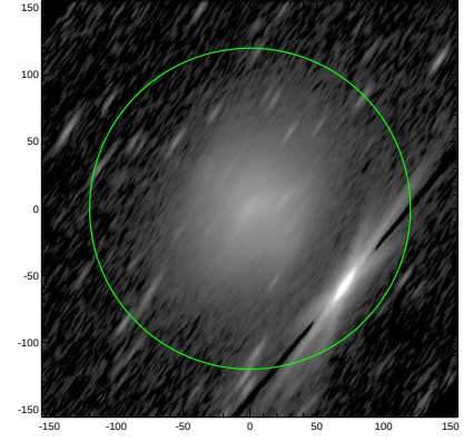
S4G: pa,inc= 56.6 79.5
