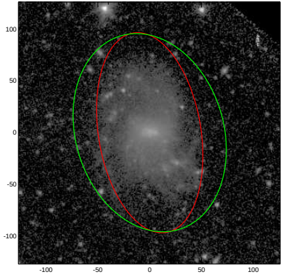
NGC3206
