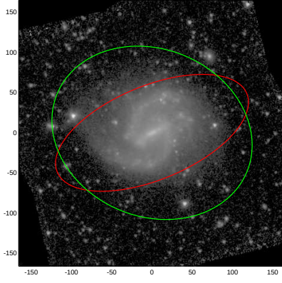
NGC3513
