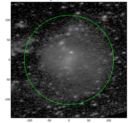
S4G: pa,inc= 9.7 57.6
