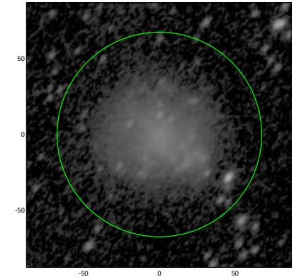
S4G: pa,inc= 51.5 54.4
