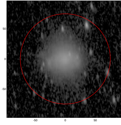
LEDA: pa,inc= 95.4 65.9
