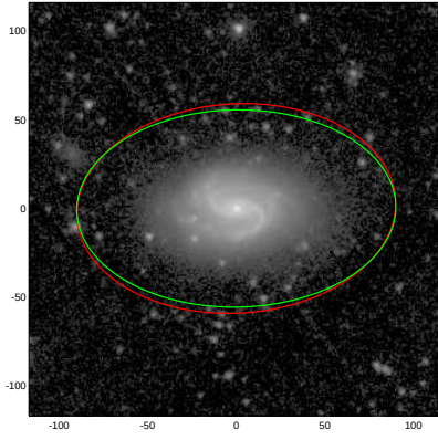
NGC3689
