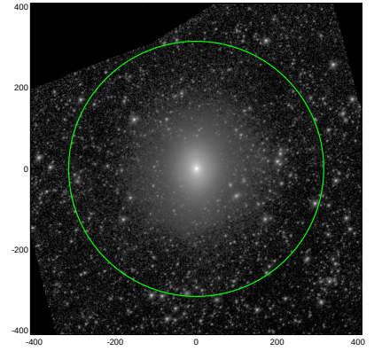
S4G: pa,inc= 40.3 30.3
