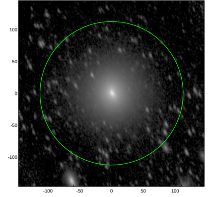
S4G: pa,inc= 111.9 60.3
