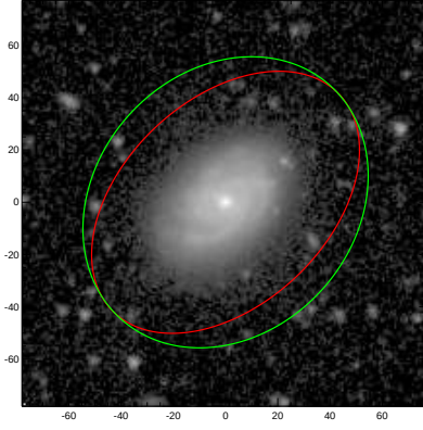
NGC3715
