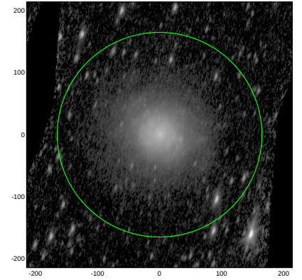
S4G: pa,inc= 75.4 66.2
