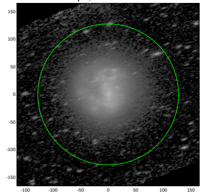
S4G: pa,inc= 19.3 64.6
