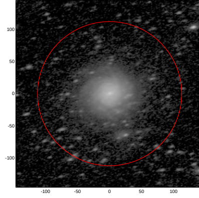
LEDA: pa,inc= 16.4 58.3
