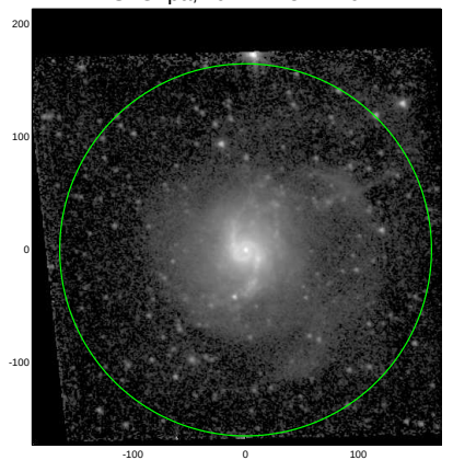
S4G: pa,inc= -17.8 27.9
