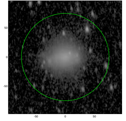
S4G: pa,inc= 93.6 60.0
