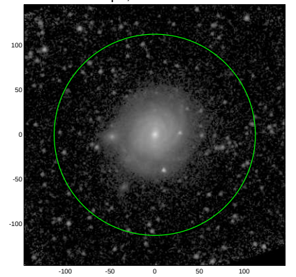
S4G: pa,inc= 42.0 18.1
