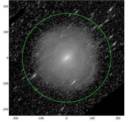
S4G: pa,inc= 45.9 73.3
