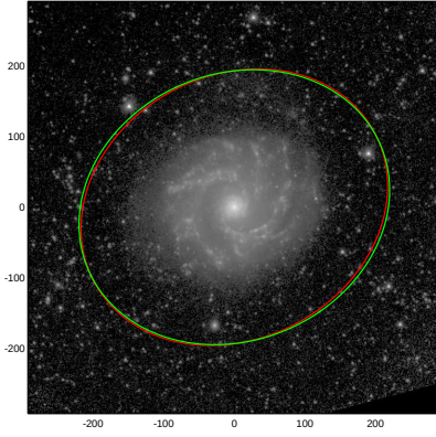
NGC3631
