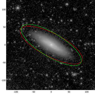
NGC3835
