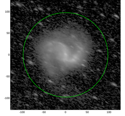
S4G: pa,inc= 152.4 66.7
