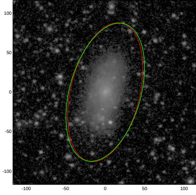
NGC3901
