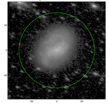
S4G: pa,inc= 154.6 52.6
