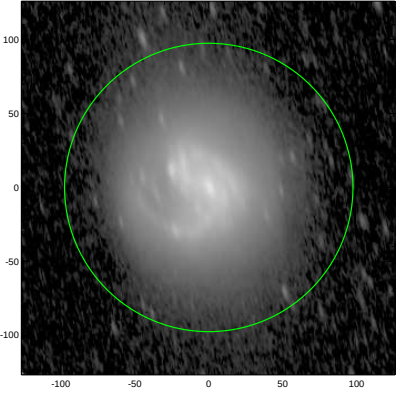
S4G: pa,inc= 103.2 70.9
