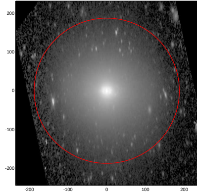
LEDA: pa,inc= 91.2 66.8
