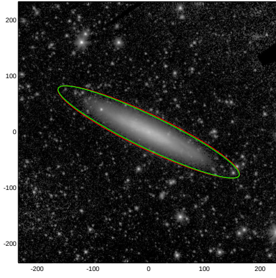
NGC3936
