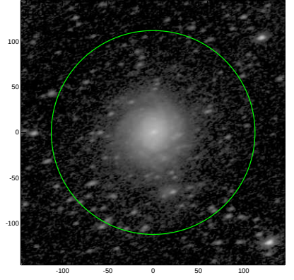
S4G: pa,inc= 20.1 54.8
