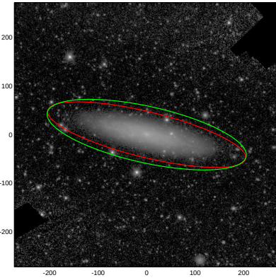
NGC3917
