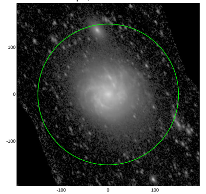
S4G: pa,inc= 121.8 52.9
