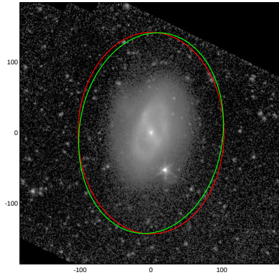
NGC3729
