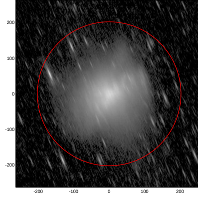
LEDA: pa,inc= 112.7 80.4
