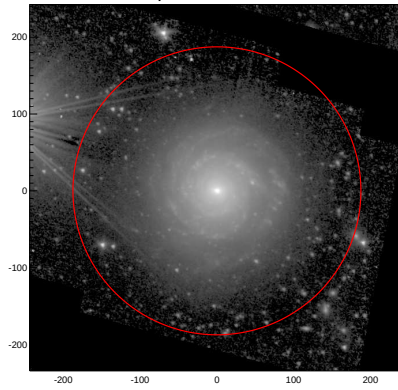
LEDA: pa,inc= 150.0 30.3
