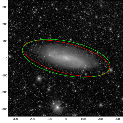
NGC3511
