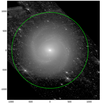
S4G: pa,inc= 156.3 57.1
