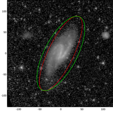
NGC3652
