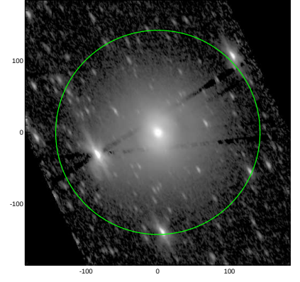
S4G: pa,inc= 120.4 64.4
