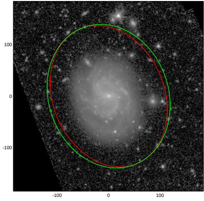
NGC3686
