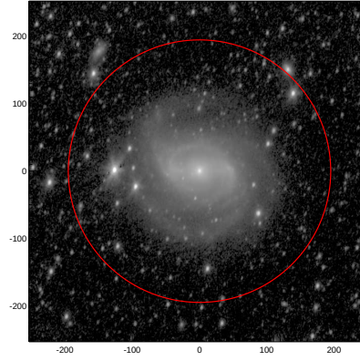
LEDA: pa,inc= 73.8 48.3
