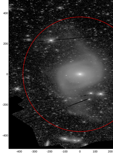
LEDA: pa,inc= 180.0 60.1
