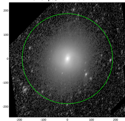
S4G: pa,inc= 70.9 60.1
