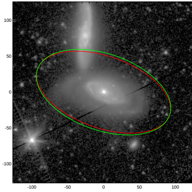
NGC3786
