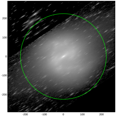
S4G: pa,inc= 34.7 78.0
