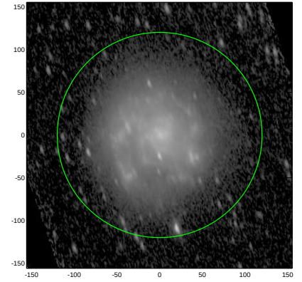
S4G: pa,inc= 107.0 64.4
