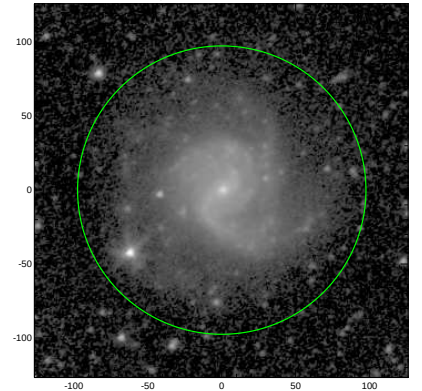
S4G: pa,inc= 29.2 30.7
