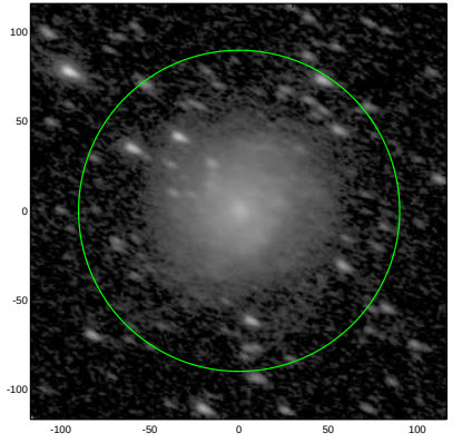
S4G: pa,inc= 154.8 59.0
