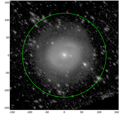
S4G: pa,inc= 136.3 49.5
