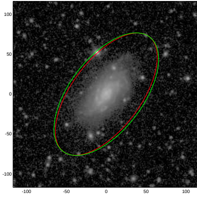
NGC3701
