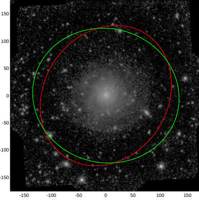
NGC3913
