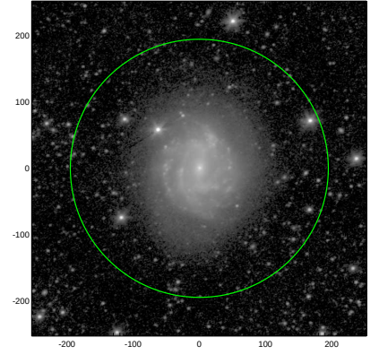
S4G: pa,inc= 21.9 32.9
