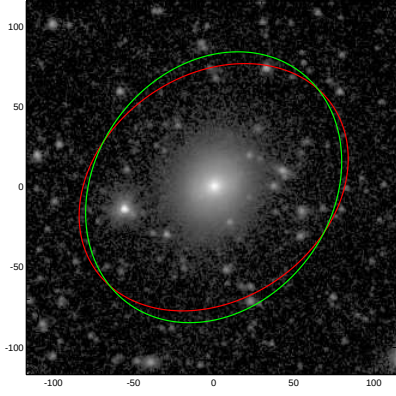
NGC3757
