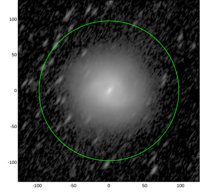
S4G: pa,inc= 58.5 70.2
