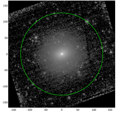
S4G: pa,inc= 41.9 23.0
