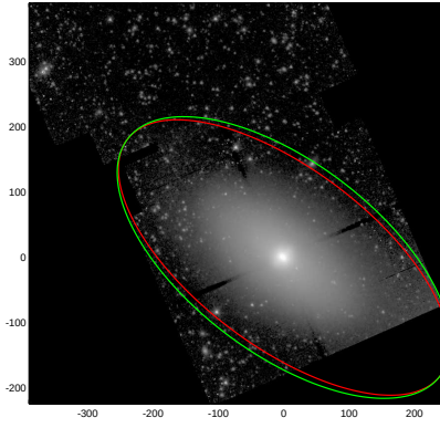
NGC3384
