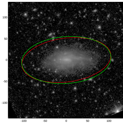
NGC3246
