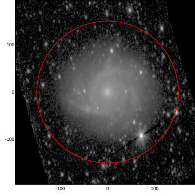
LEDA: pa,inc= 92.7 50.1
