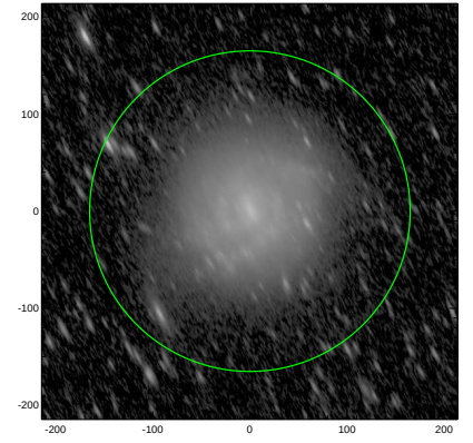
S4G: pa,inc= 116.7 72.9
