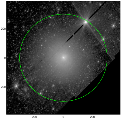
S4G: pa,inc= 63.8 38.9
