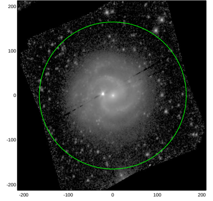
S4G: pa,inc= 80.1 29.7
