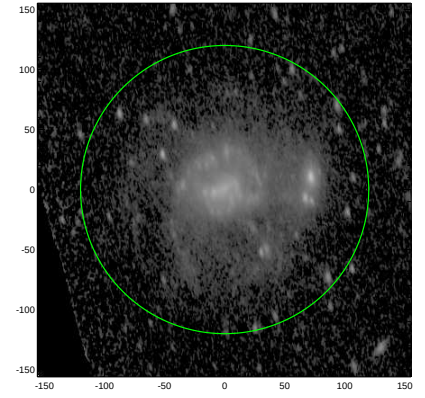
S4G: pa,inc= 99.3 60.2
