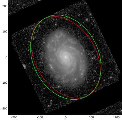
NGC3810
