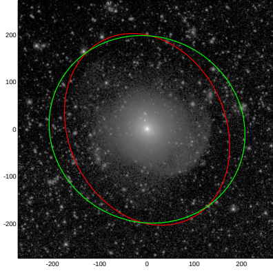
NGC3619
