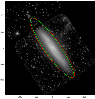
NGC3877
