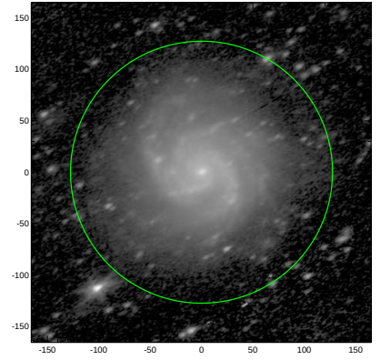
S4G: pa,inc= 29.3 58.5
