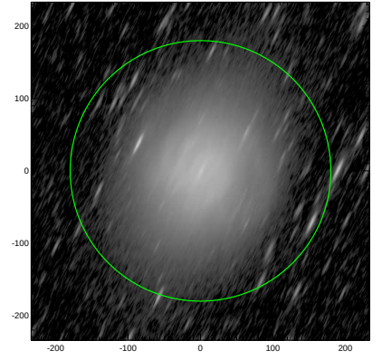
S4G: pa,inc= 64.2 80.7
