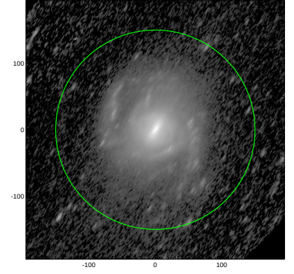
S4G: pa,inc= 57.6 71.4
