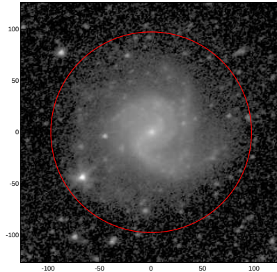
LEDA: pa,inc= 25.5 36.2
