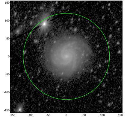
S4G: pa,inc= 64.7 47.8
