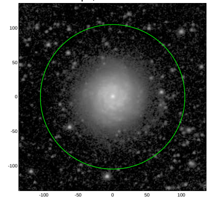
S4G: pa,inc= 22.8 28.5
