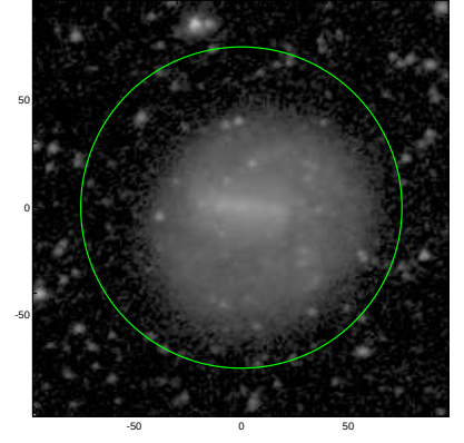
S4G: pa,inc= 28.1 29.6
