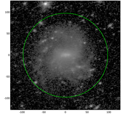
S4G: pa,inc= 16.8 42.9
