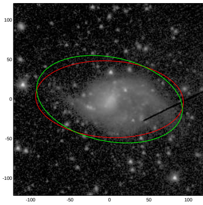
NGC3023
