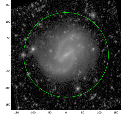
S4G: pa,inc= 67.6 35.2
