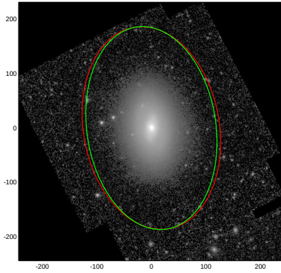
NGC3941
