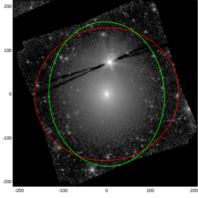
NGC3193
