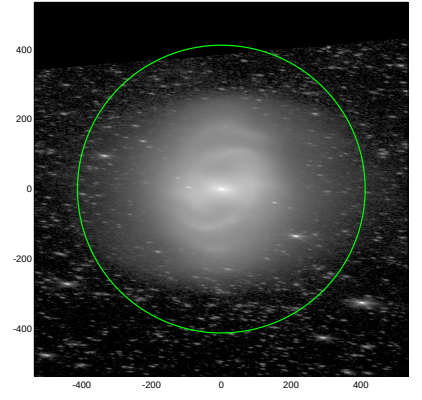
S4G: pa,inc= -6.0 73.7
