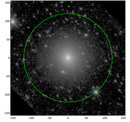
S4G: pa,inc= 133.1 38.6
