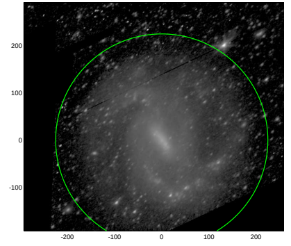
S4G: pa,inc= 43.0 55.6
