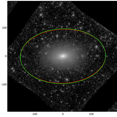
NGC3682
