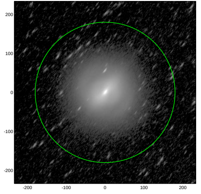
S4G: pa,inc= 51.6 71.7
