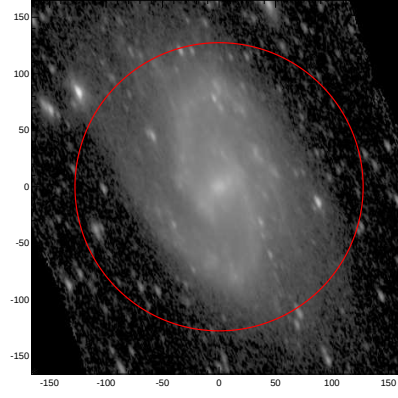
LEDA: pa,inc= 112.6 62.8
