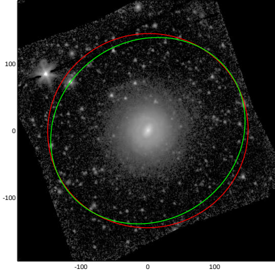
NGC3681
