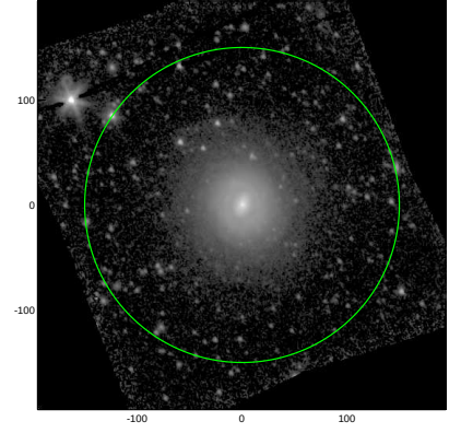
S4G: pa,inc= 123.5 26.5
