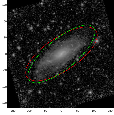
NGC3755
