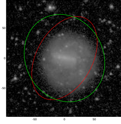
NGC3906
