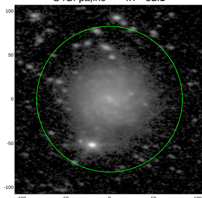
S4G: pa,inc= -4.7 52.1
