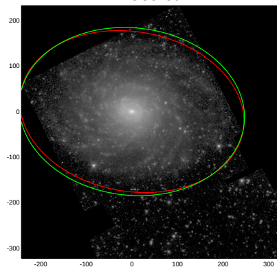
NGC3486
