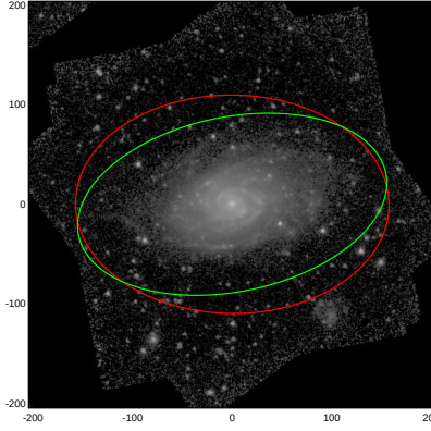
NGC3614
