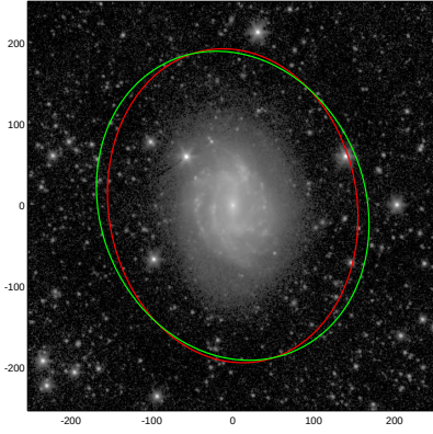
NGC3887
