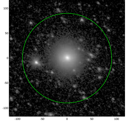
S4G: pa,inc= 143.2 35.1
