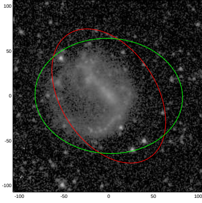
NGC3664
