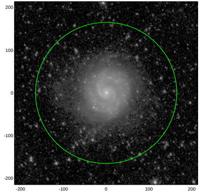
S4G: pa,inc= 108.2 21.4
