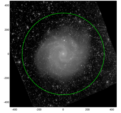
S4G: pa,inc= 45.2 16.2
