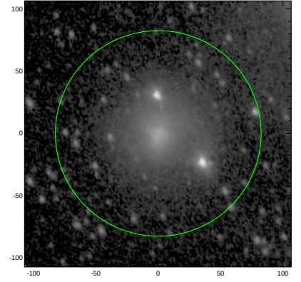
S4G: pa,inc= 121.5 44.7
