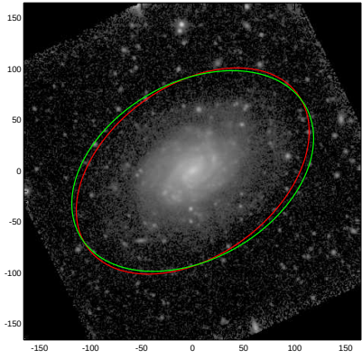
NGC3684
