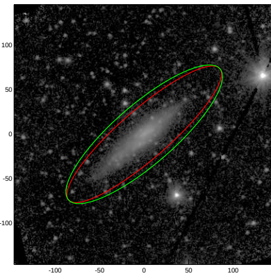
NGC3879
