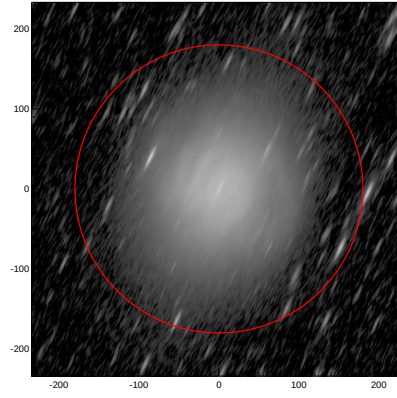
LEDA: pa,inc= 64.4 80.2
