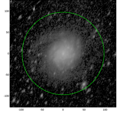
S4G: pa,inc= 62.4 58.4
