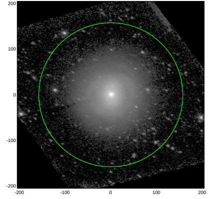
S4G: pa,inc= -16.8 46.3
