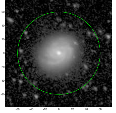
S4G: pa,inc= 138.0 33.9
