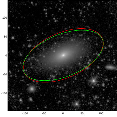
NGC3522
