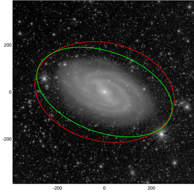
NGC3992
