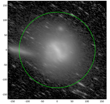
S4G: pa,inc= 149.4 71.5
