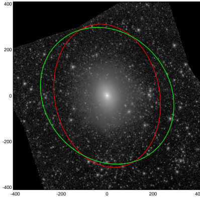
NGC3904
