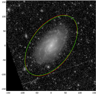
NGC3370
