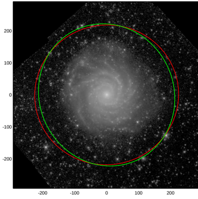
NGC3938
