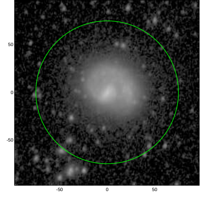
S4G: pa,inc= 75.2 39.1
