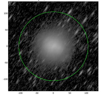
S4G: pa,inc= 54.4 73.8
