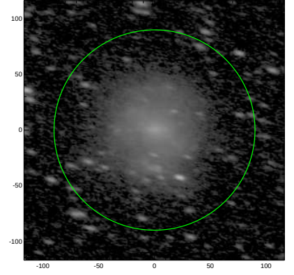
S4G: pa,inc= -15.5 59.9
