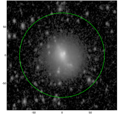
S4G: pa,inc= 83.1 42.7
