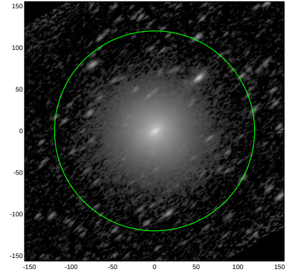
S4G: pa,inc= 40.1 67.2
