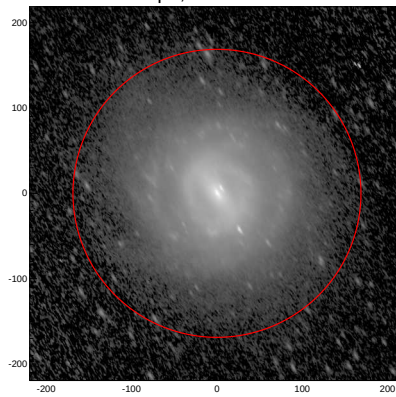
LEDA: pa,inc= 121.0 66.2
