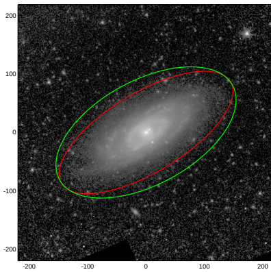
NGC3705
