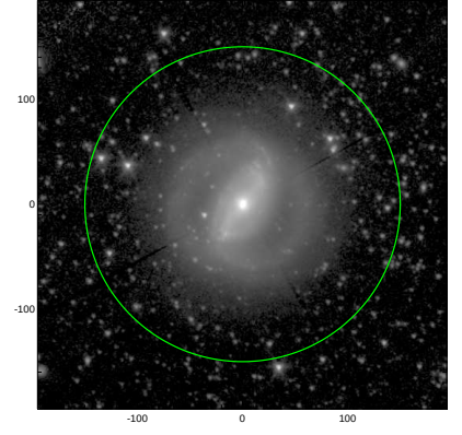
S4G: pa,inc= 131.1 12.8
