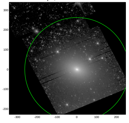
S4G: pa,inc= 138.6 28.6
