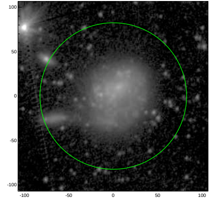
S4G: pa,inc= 67.8 28.1
