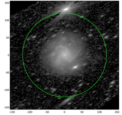
S4G: pa,inc= 25.8 63.4
