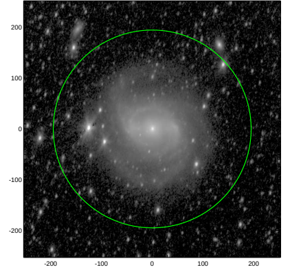
S4G: pa,inc= 76.7 52.6
