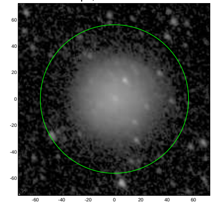
S4G: pa,inc= 128.3 38.5
