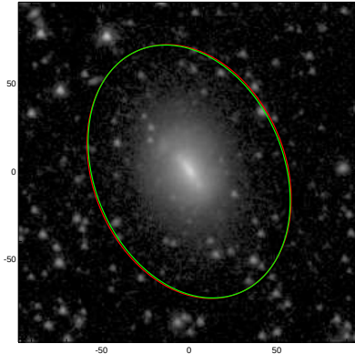
NGC3870
