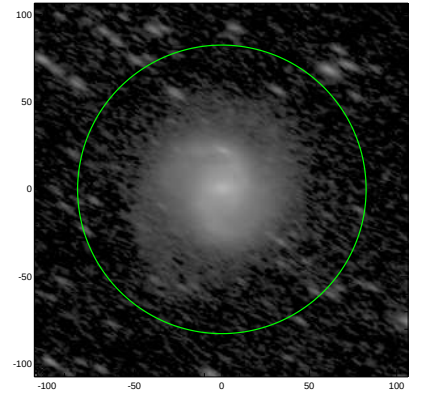
S4G: pa,inc= 151.9 66.5
