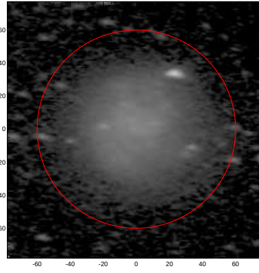
LEDA: pa,inc= 175.6 62.5
