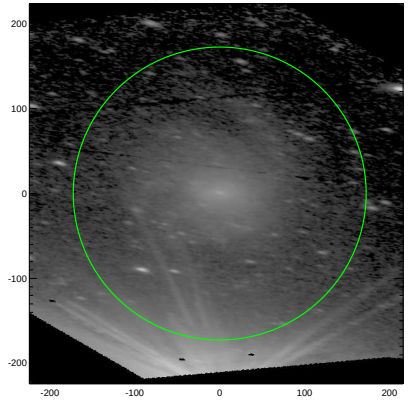
S4G: pa,inc= -10.6 71.5
