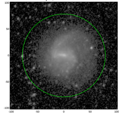
S4G: pa,inc= 57.0 32.7
