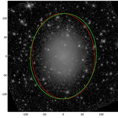
NGC3299
