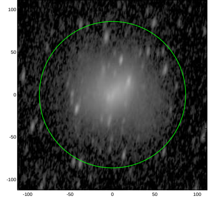
S4G: pa,inc= 81.1 69.4
