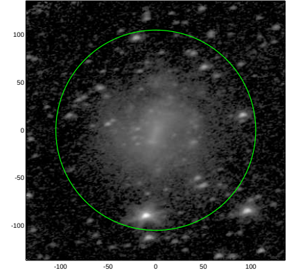
S4G: pa,inc= 13.0 53.0
