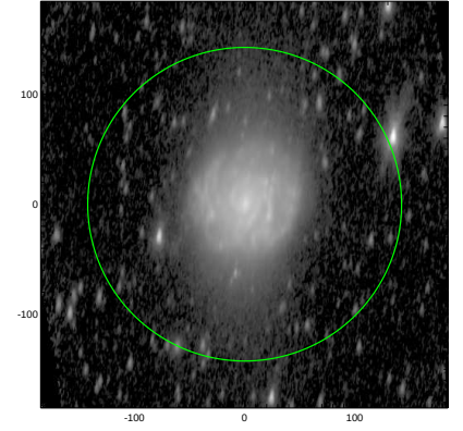
S4G: pa,inc= 83.1 68.2
