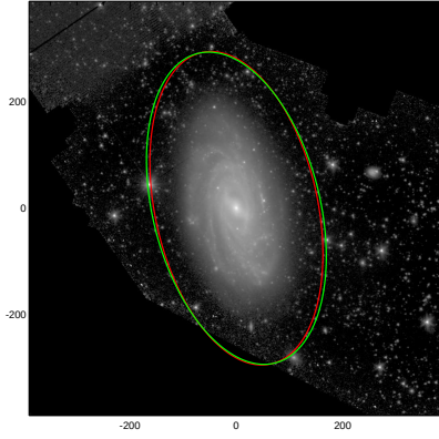
NGC3953
