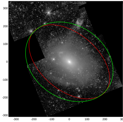
NGC3169
