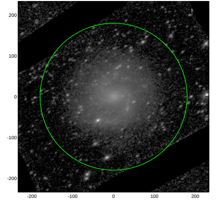
S4G: pa,inc= 33.8 52.4
