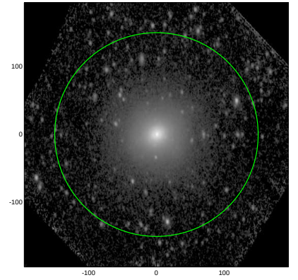
S4G: pa,inc= 91.9 49.9
