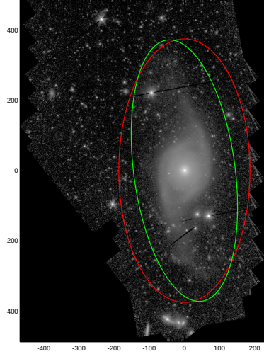
NGC3718
