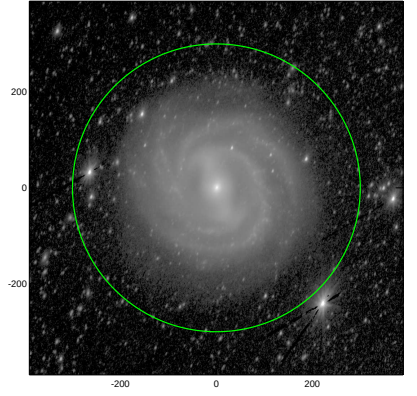
S4G: pa,inc= 70.1 55.1
