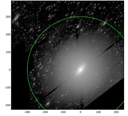
S4G: pa,inc= 52.9 60.8
