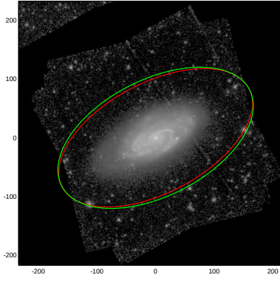
NGC3294
