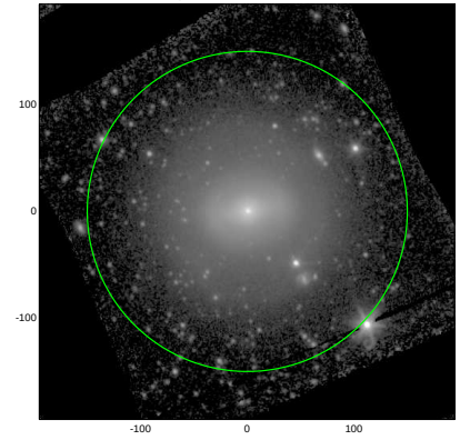
S4G: pa,inc= 99.7 16.5
