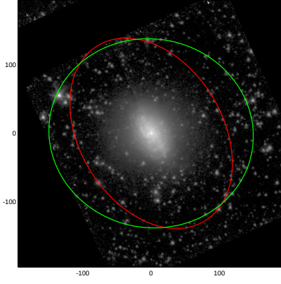
NGC3655
