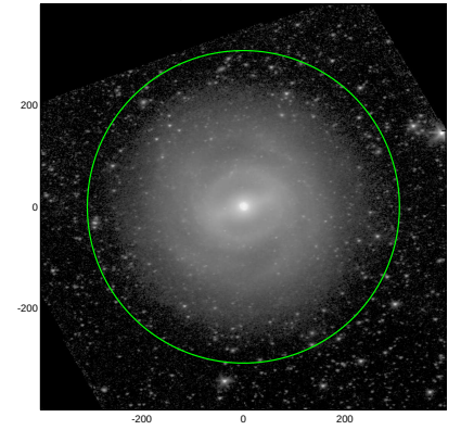
S4G: pa,inc= 8.4 45.0
