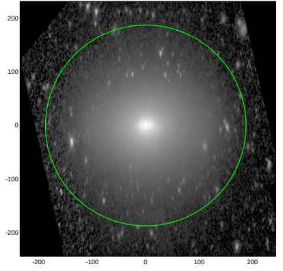
S4G: pa,inc= 89.3 63.7
