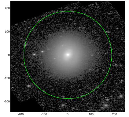
S4G: pa,inc= 8.5 50.8
