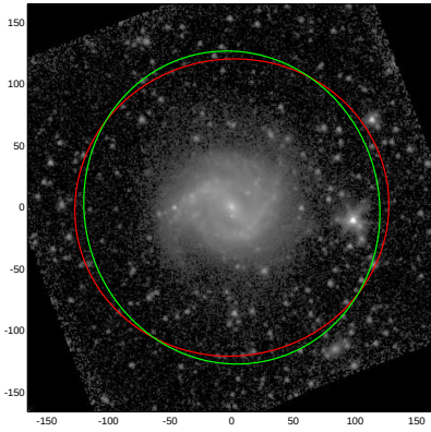
NGC3485
