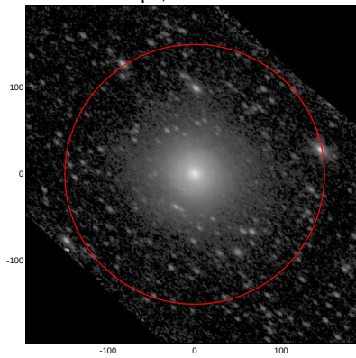
LEDA: pa,inc= 138.0 53.4
