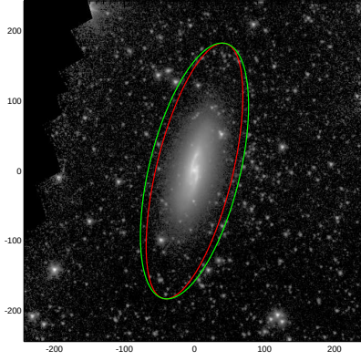
NGC3955
