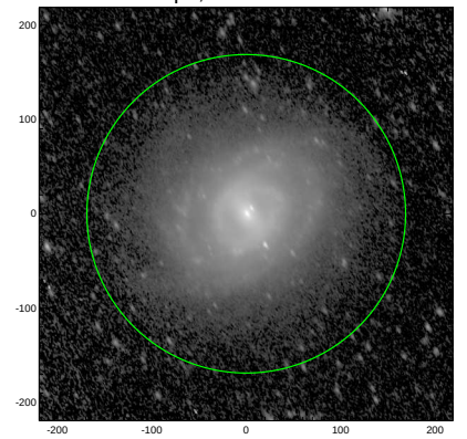
S4G: pa,inc= 118.5 58.2
