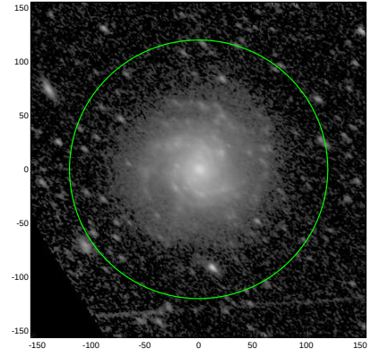
S4G: pa,inc= 141.9 55.1
