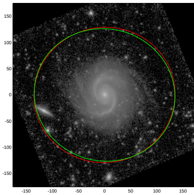
NGC3433
