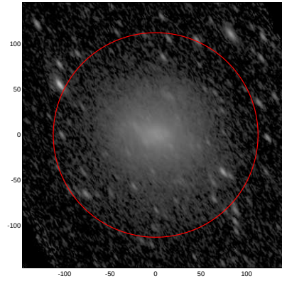
LEDA: pa,inc= 124.5 66.4
