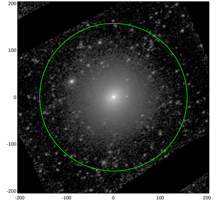
S4G: pa,inc= 33.1 40.7
