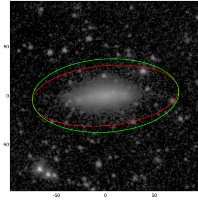
NGC3220
