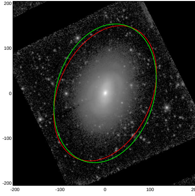
NGC3626
