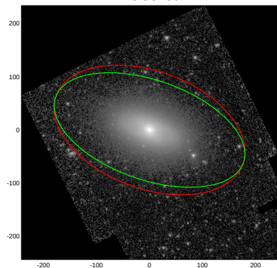
NGC3489
