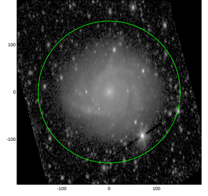
S4G: pa,inc= 90.0 51.2
