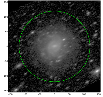
S4G: pa,inc= 29.7 61.3
