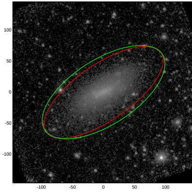
NGC3850
