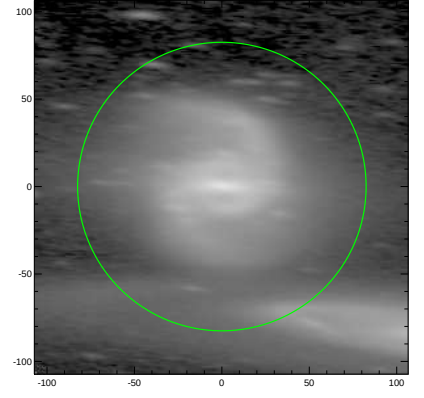
S4G: pa,inc= -4.2 76.3
