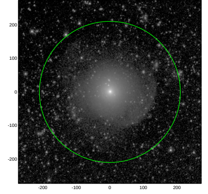
S4G: pa,inc= 63.5 21.5
