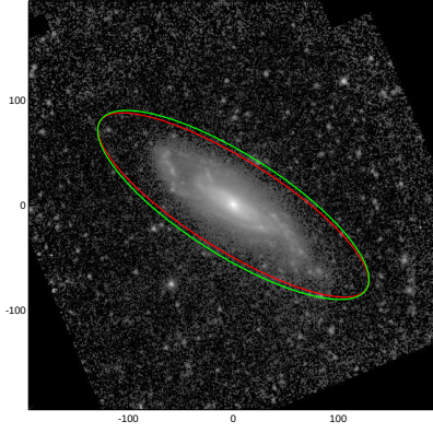
NGC3976
