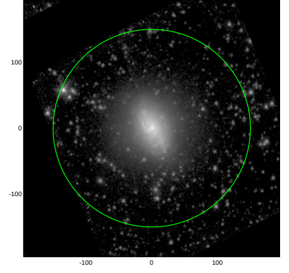
S4G: pa,inc= 79.7 23.5
