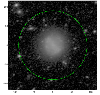
S4G: pa,inc= 21.6 40.8
