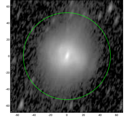
S4G: pa,inc= 71.6 68.1
