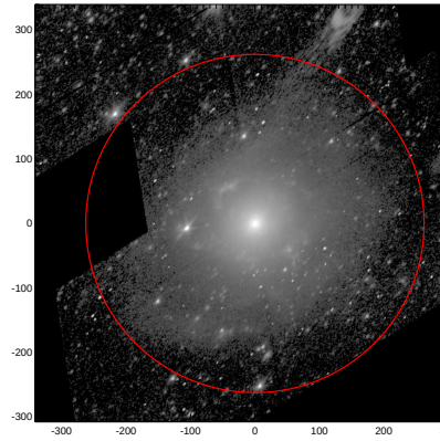
LEDA: pa,inc= 50.5 52.3
