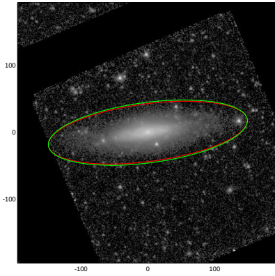
NGC3666
