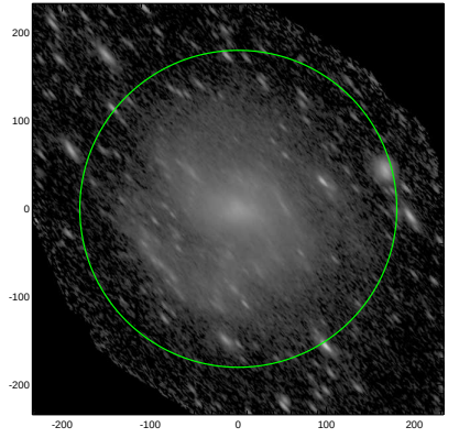
S4G: pa,inc= 130.4 71.3
