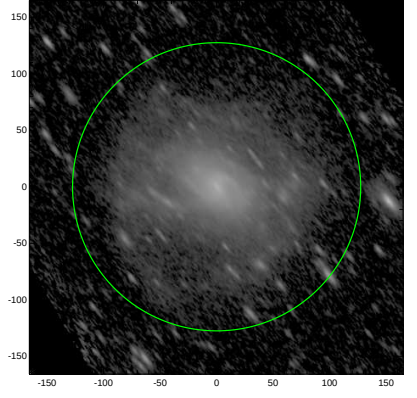
S4G: pa,inc= 129.3 68.7
