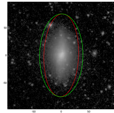
NGC3413
