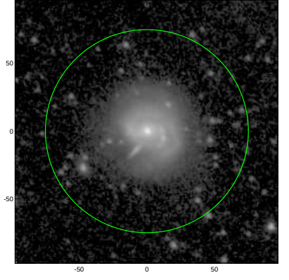
S4G: pa,inc= 132.0 25.7
