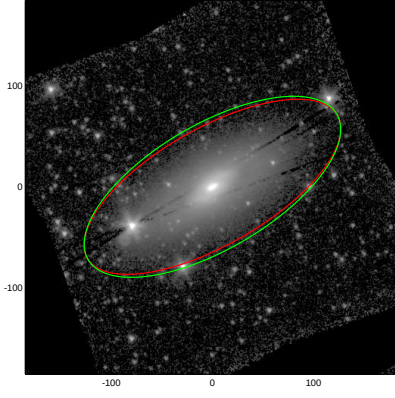
NGC3885
