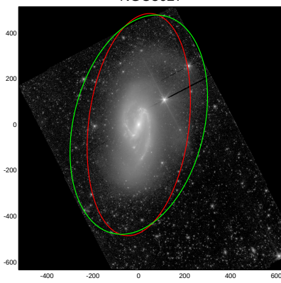
NGC3627
