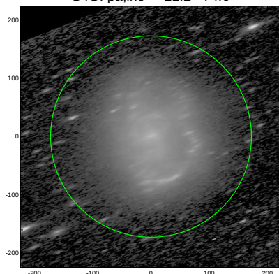
S4G: pa,inc= 21.2 74.6
