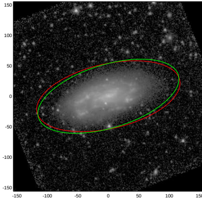
NGC3389
