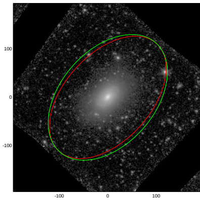
NGC3329
