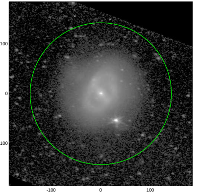
S4G: pa,inc= -7.7 44.7
