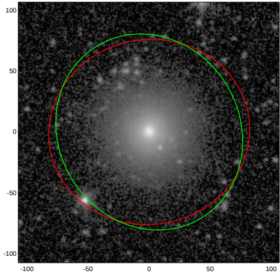
NGC3928
