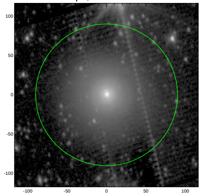
S4G: pa,inc= 96.6 37.4
