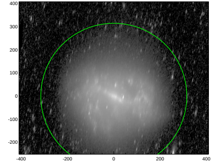
S4G: pa,inc= 80.7 73.0
