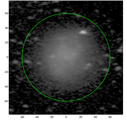
S4G: pa,inc= -2.1 60.0
