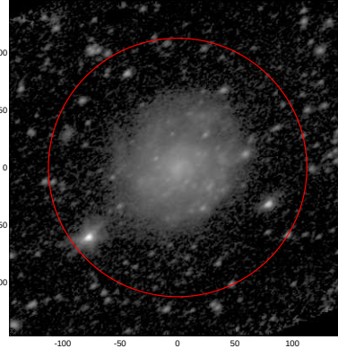
LEDA: pa,inc= 34.5 50.0
