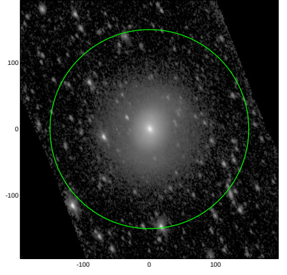
S4G: pa,inc= 118.6 52.0
