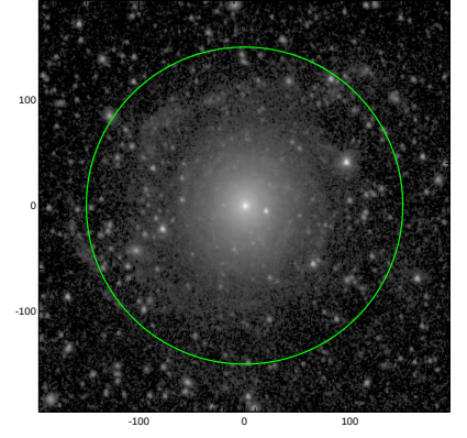
S4G: pa,inc= 98.0 25.1
