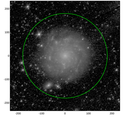
S4G: pa,inc= 36.1 35.2
