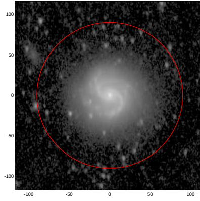
LEDA: pa,inc= 93.3 49.0
