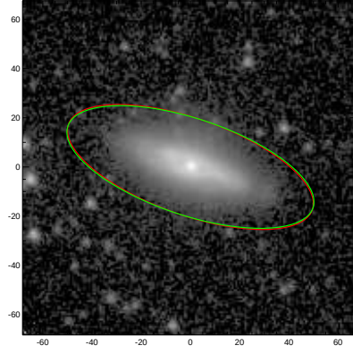
NGC3633
