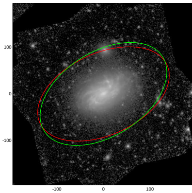
NGC3949
