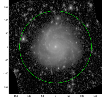
S4G: pa,inc= 81.9 39.8
