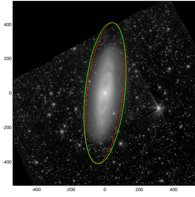
NGC3623
