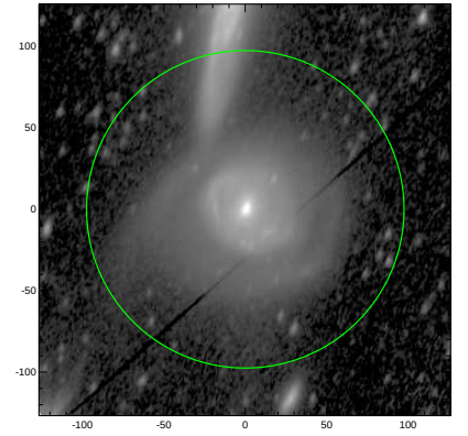
S4G: pa,inc= 70.9 56.8
