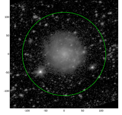
S4G: pa,inc= 25.1 38.9
