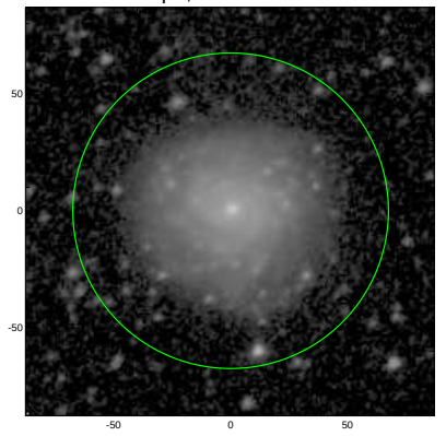
S4G: pa,inc= 50.5 28.2
