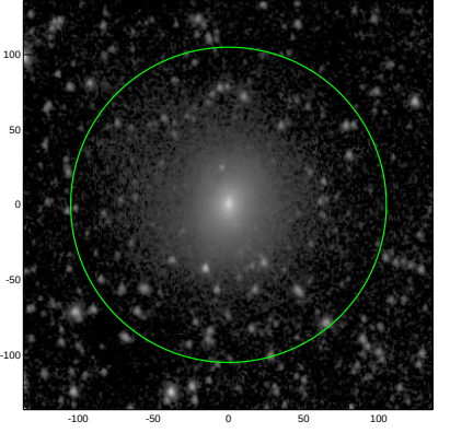
S4G: pa,inc= 91.6 32.5
