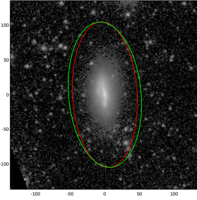
NGC3912
