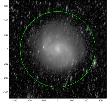
S4G: pa,inc= 78.4 67.6
