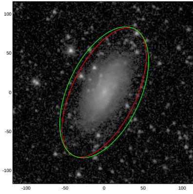
NGC3225
