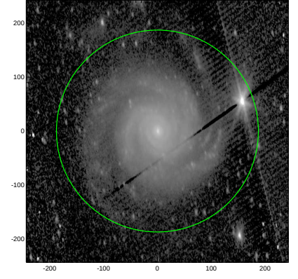
S4G: pa,inc= 97.1 60.9
