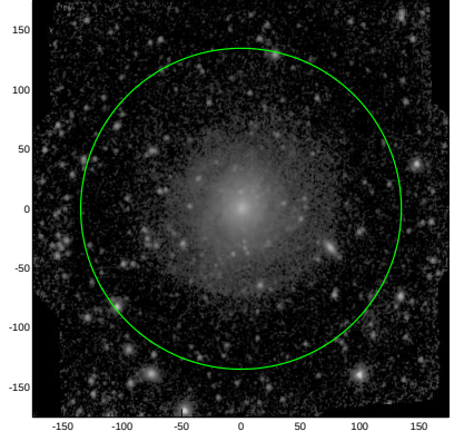
S4G: pa,inc= 76.9 24.1
