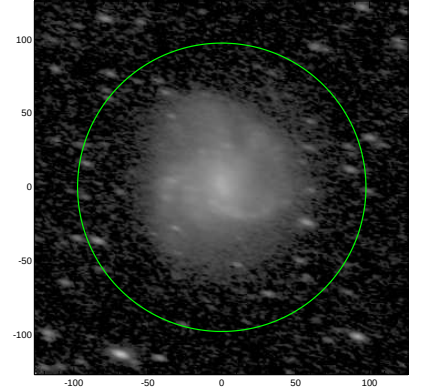
S4G: pa,inc= -15.4 62.8
