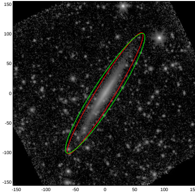
NGC3245A
