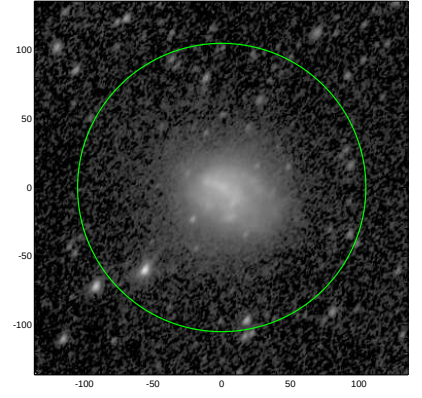
S4G: pa,inc= 55.3 53.1
