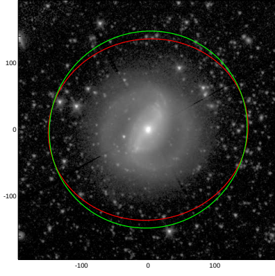
NGC3504
