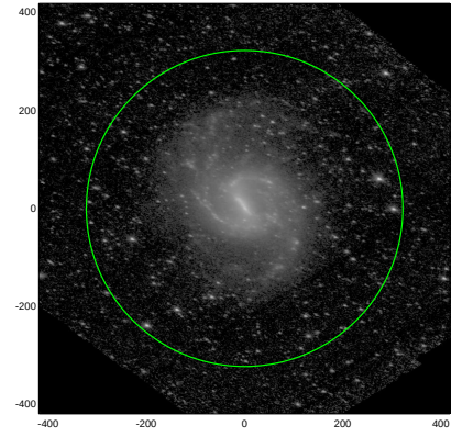
S4G: pa,inc= -15.8 53.8
