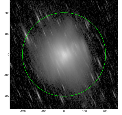
S4G: pa,inc= 113.4 82.3
