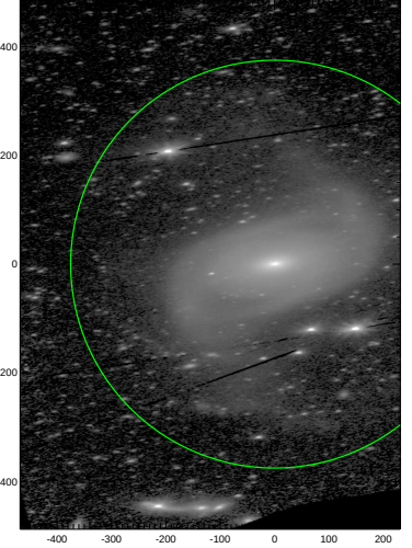
S4G: pa,inc= 7.6 67.4
