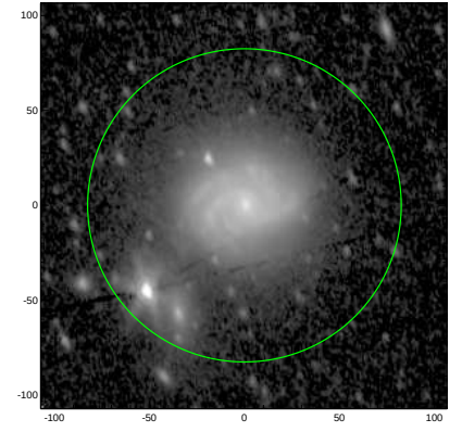
S4G: pa,inc= 106.5 47.9
