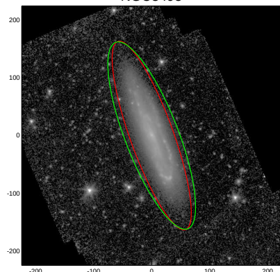
NGC3495
