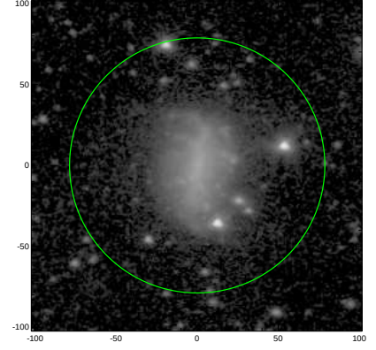
S4G: pa,inc= 2.0 34.2
