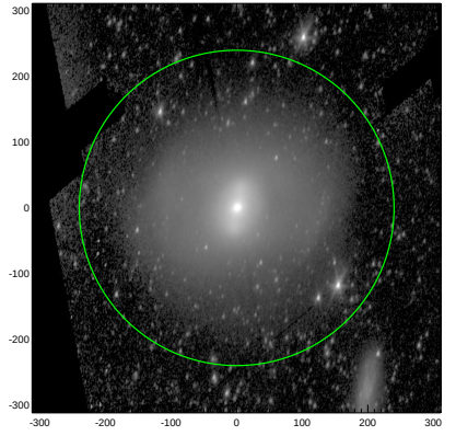
S4G: pa,inc= 79.6 55.8
