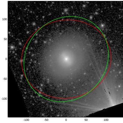
NGC3637
