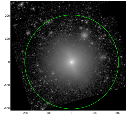
S4G: pa,inc= 12.6 33.2
