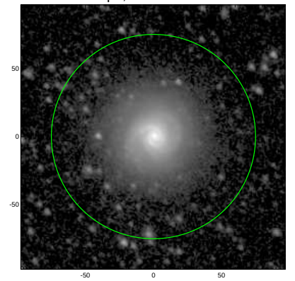
S4G: pa,inc= 137.5 28.9
