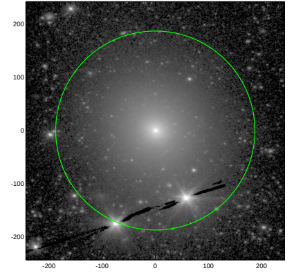
S4G: pa,inc= -1.5 36.6
