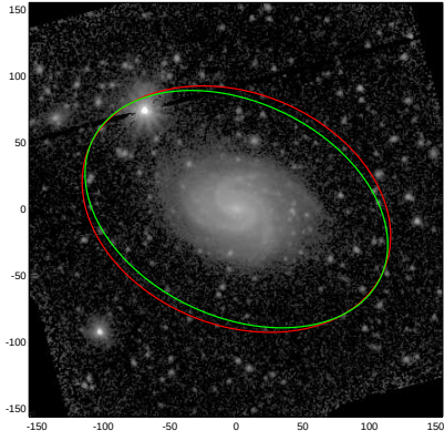
NGC3683A
