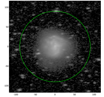
S4G: pa,inc= 5.5 59.6
