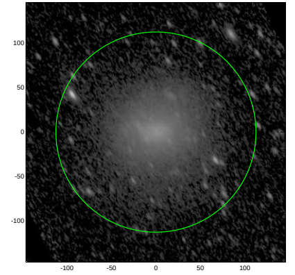
S4G: pa,inc= 122.7 62.2
