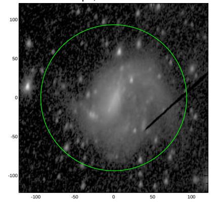
S4G: pa,inc= 78.2 55.6
