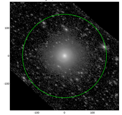
S4G: pa,inc= 138.9 49.6
