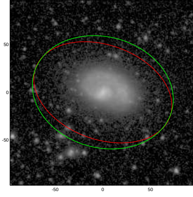
NGC3985
