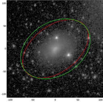
NGC3896
