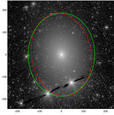
NGC3962
