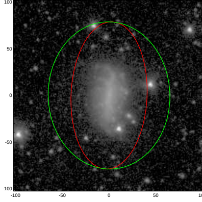
NGC3782
