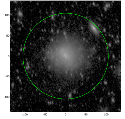
S4G: pa,inc= 99.2 53.7
