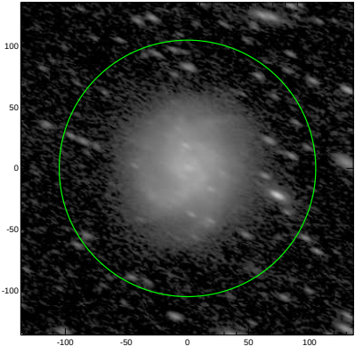
S4G: pa,inc= 154.0 65.6
