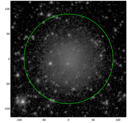
S4G: pa,inc= 56.4 24.0
