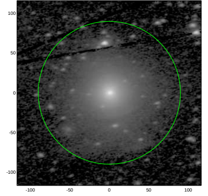
S4G: pa,inc= 9.4 54.9
