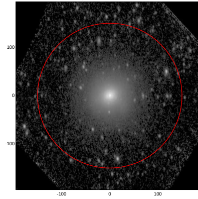
LEDA: pa,inc= 92.5 50.8
