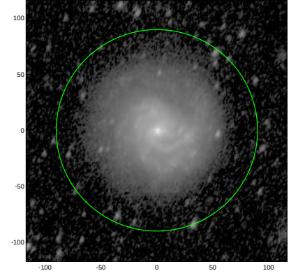
S4G: pa,inc= 63.8 54.4
