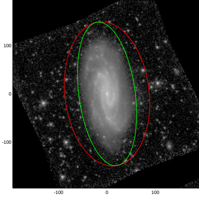
NGC3672
