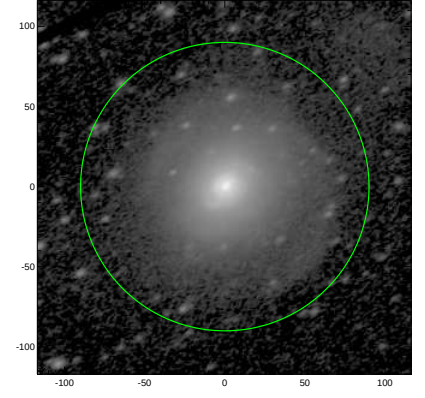
S4G: pa,inc= 29.4 51.3
