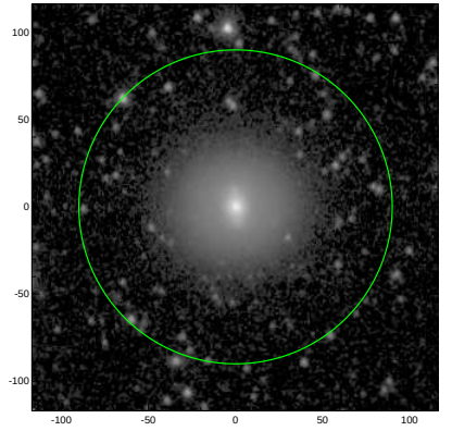
S4G: pa,inc= 91.9 25.6
