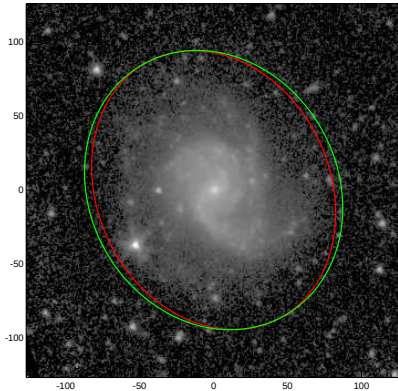
NGC3162
