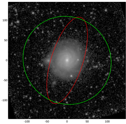
NGC3687
