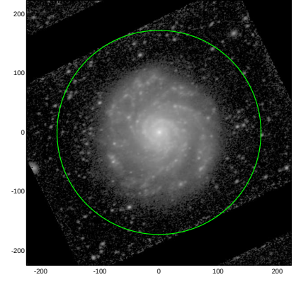
S4G: pa,inc= 25.7 42.2
