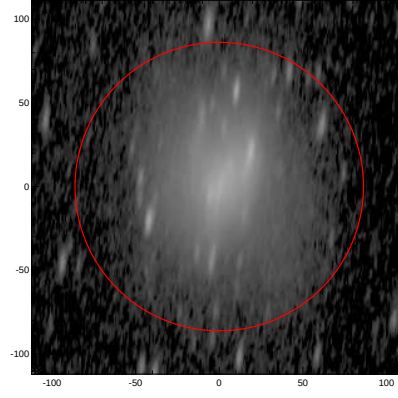
LEDA: pa,inc= 84.0 75.5
