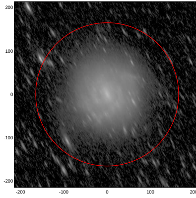
LEDA: pa,inc= 117.2 74.4
