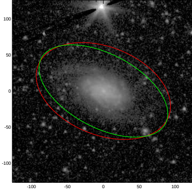
NGC3455
