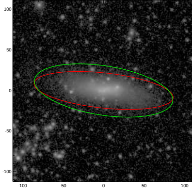
NGC3952
