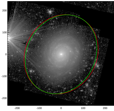
NGC3147
