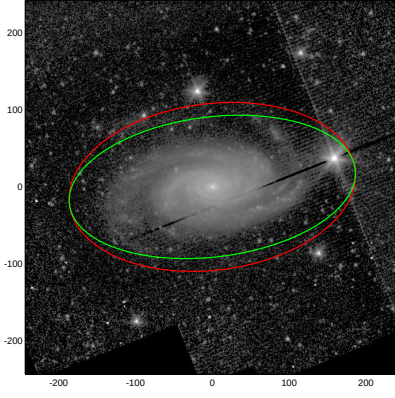
NGC3338
