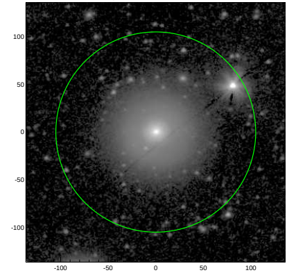
S4G: pa,inc= 12.7 24.6
