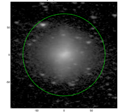
S4G: pa,inc= -0.6 58.4
