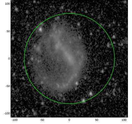
S4G: pa,inc= 87.1 38.9
