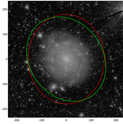
NGC3423
