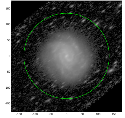
S4G: pa,inc= 38.0 66.9
