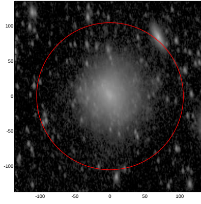
LEDA: pa,inc= 95.3 60.1
