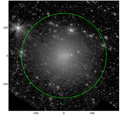
S4G: pa,inc= 158.0 40.5
