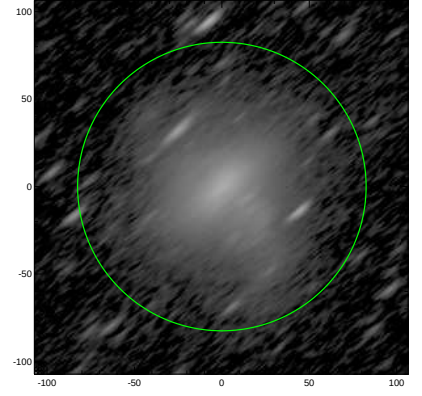
S4G: pa,inc= 39.2 75.6
