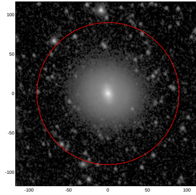
LEDA: pa,inc= 107.5 30.1
