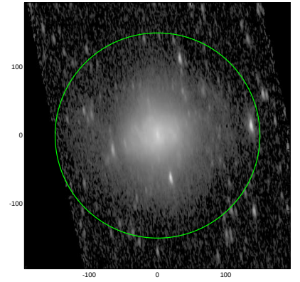
S4G: pa,inc= 97.5 72.5
