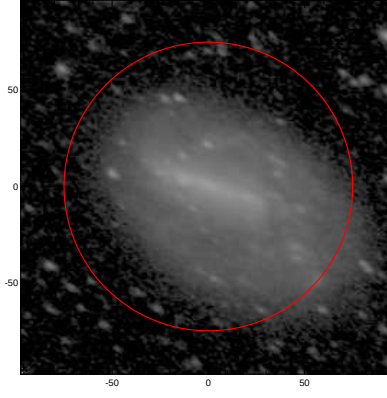
LEDA: pa,inc= 150.9 51.3
