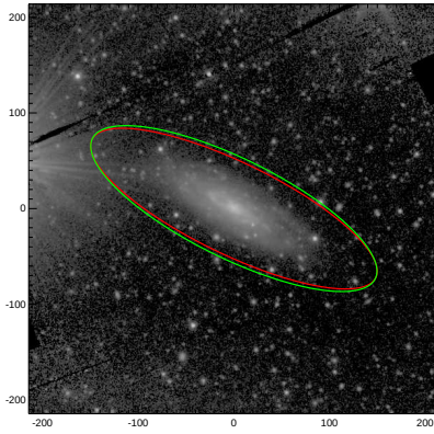
NGC3956
