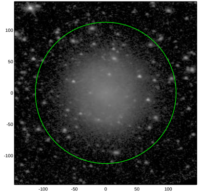
S4G: pa,inc= -4.9 39.5
