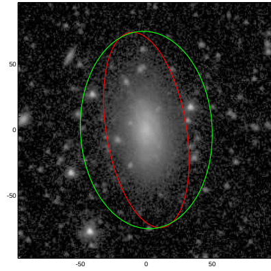
NGC3622
