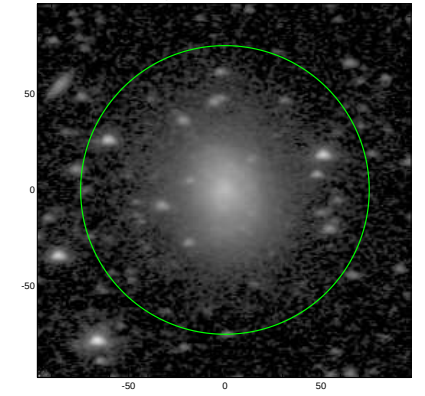
S4G: pa,inc= 3.0 48.2
