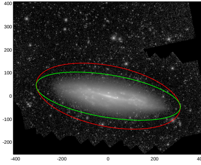
NGC3556
