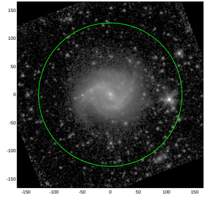
S4G: pa,inc= 15.7 20.4
