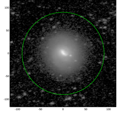
S4G: pa,inc= 10.5 48.6
