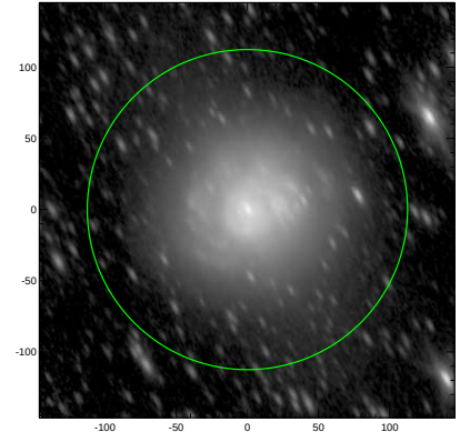
S4G: pa,inc= 118.5 65.9
