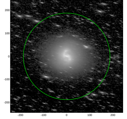
S4G: pa,inc= -13.8 69.8
