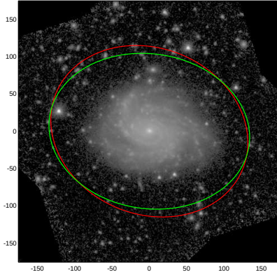
NGC3780
