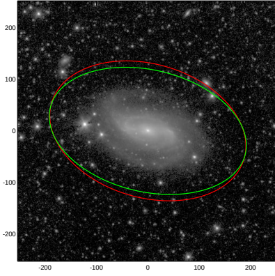
NGC3673
