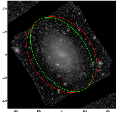
NGC3930
