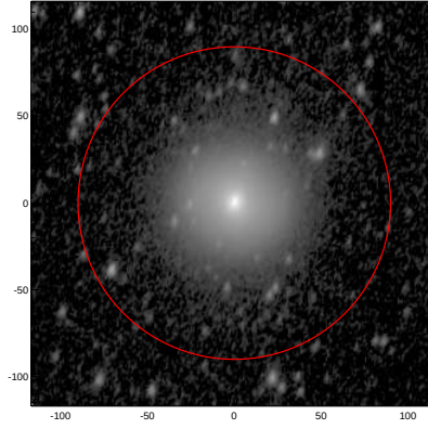
LEDA: pa,inc= 72.7 52.3
