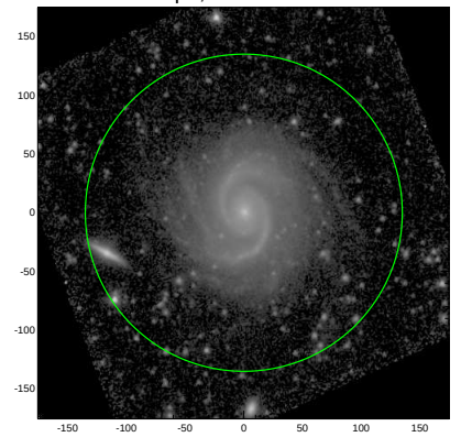
S4G: pa,inc= 77.3 21.0
