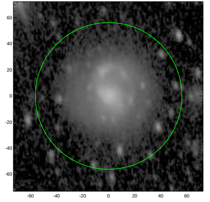
S4G: pa,inc= 100.8 53.6
