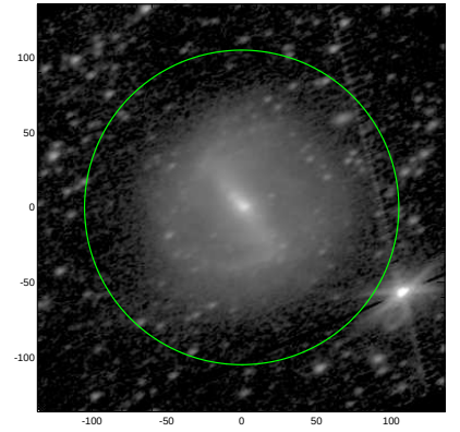
S4G: pa,inc= 28.6 53.4
