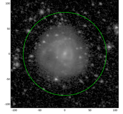
S4G: pa,inc= 162.8 34.1
