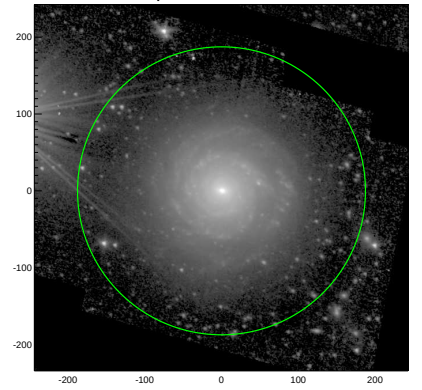
S4G: pa,inc= 151.7 34.3
