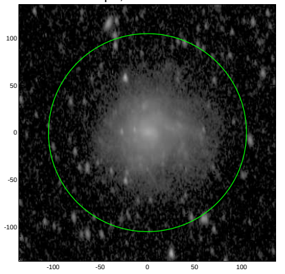
S4G: pa,inc= 94.2 58.5
