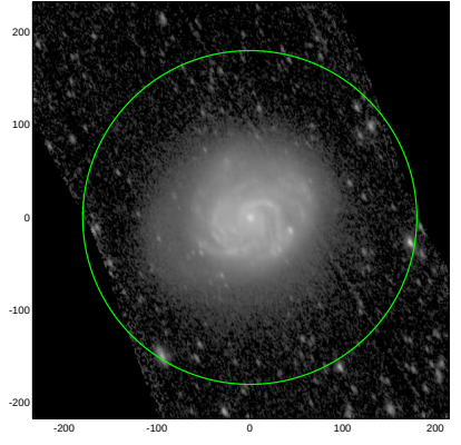
S4G: pa,inc= 116.9 56.6
