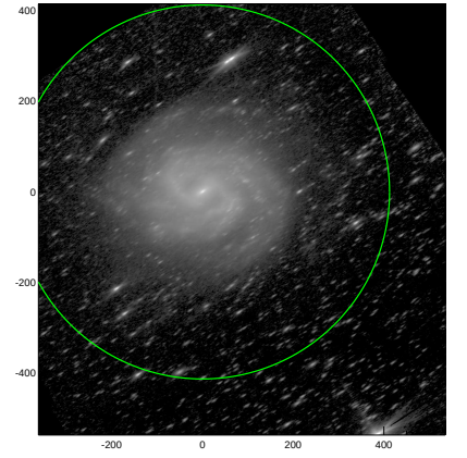
S4G: pa,inc= 33.6 70.5
