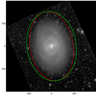
NGC3351
