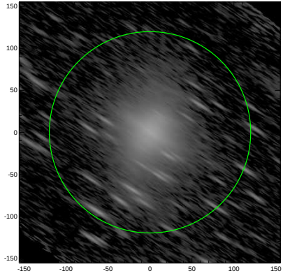
S4G: pa,inc= 147.1 80.4
