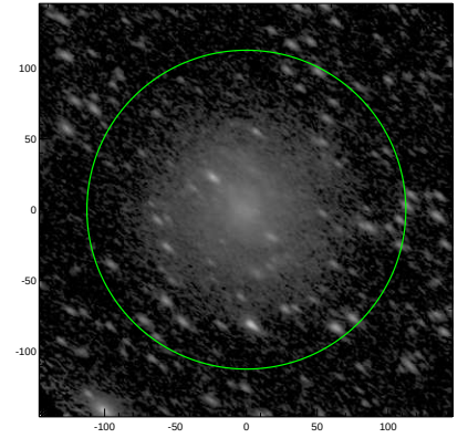
S4G: pa,inc= 144.4 60.1
