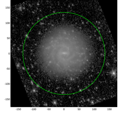
S4G: pa,inc= 116.3 32.6
