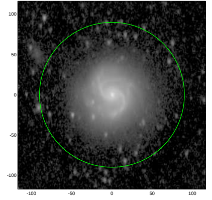
S4G: pa,inc= 90.9 51.8
