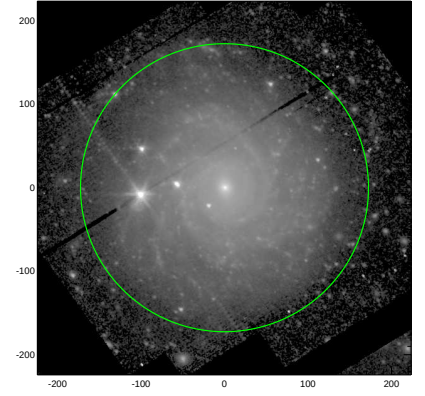
S4G: pa,inc= 142.7 27.0
