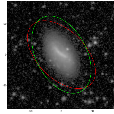
NGC3654
