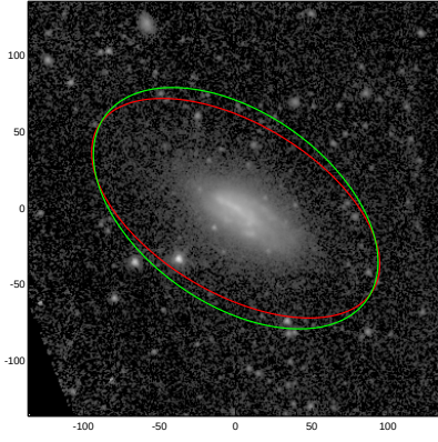
NGC3659
