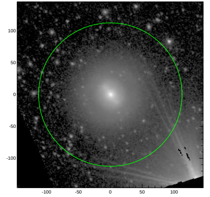
S4G: pa,inc= 138.1 27.0
