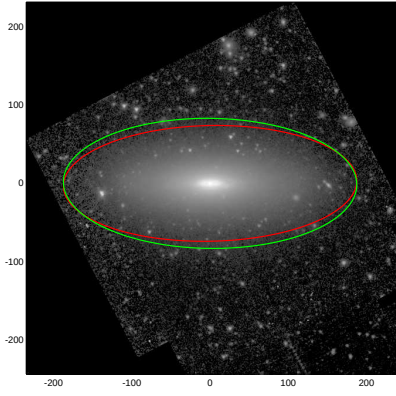
NGC3593
