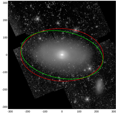
NGC3166
