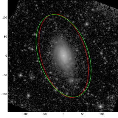
NGC3259
