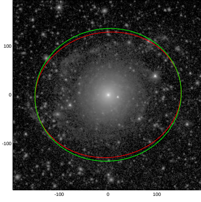
NGC3642
