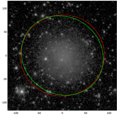
NGC3377A
