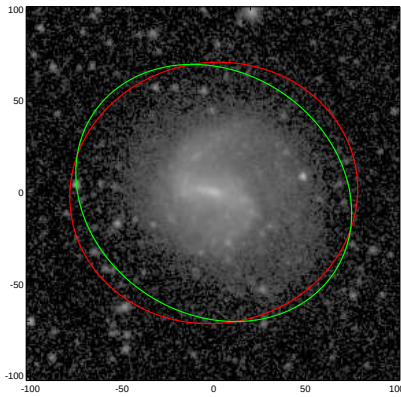
NGC3381
