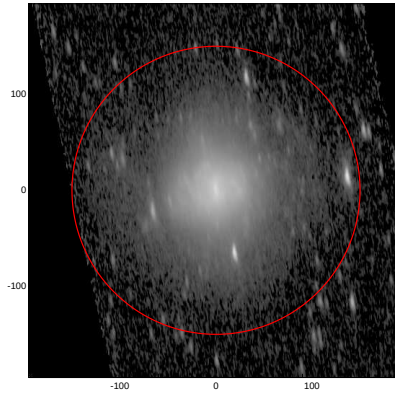
LEDA: pa,inc= 97.5 73.3
