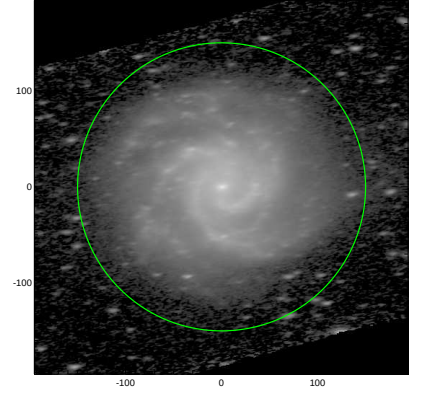
S4G: pa,inc= 7.8 67.2
