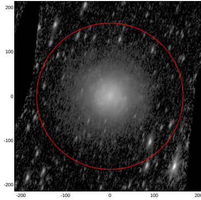
LEDA: pa,inc= 73.5 67.9
