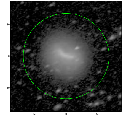
S4G: pa,inc= 27.7 52.6
