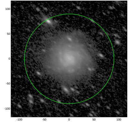
S4G: pa,inc= 142.8 59.3
