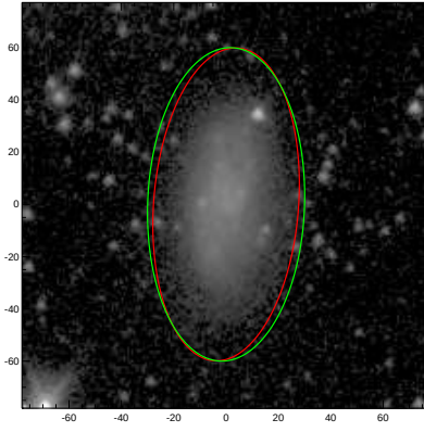
NGC3165
