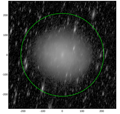
S4G: pa,inc= 77.5 73.9
