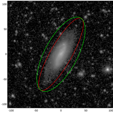
NGC3625
