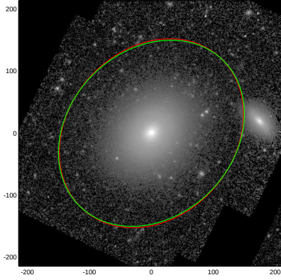
NGC3998
