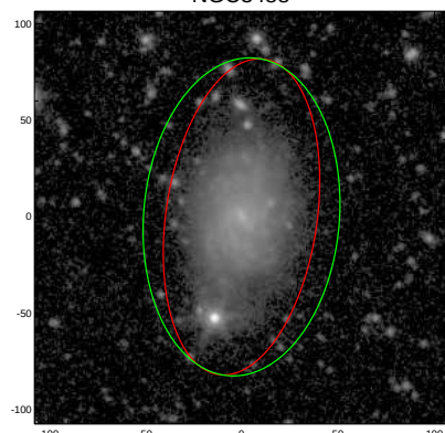
NGC3488
