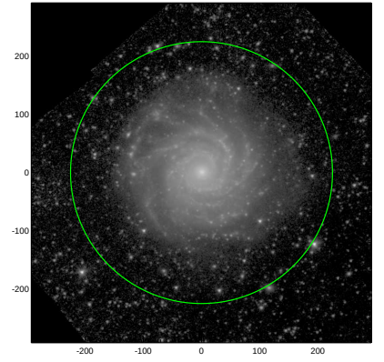
S4G: pa,inc= 26.0 20.9
