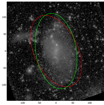
NGC3447
