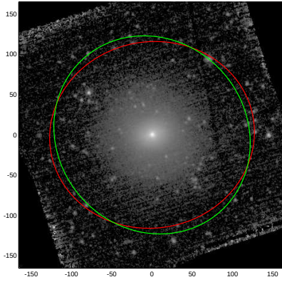
NGC3599
