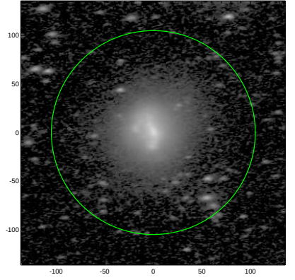
S4G: pa,inc= 5.0 60.1
