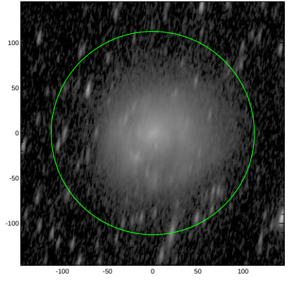
S4G: pa,inc= 79.5 73.4
