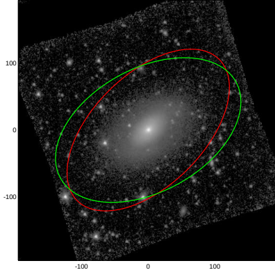
NGC3248
