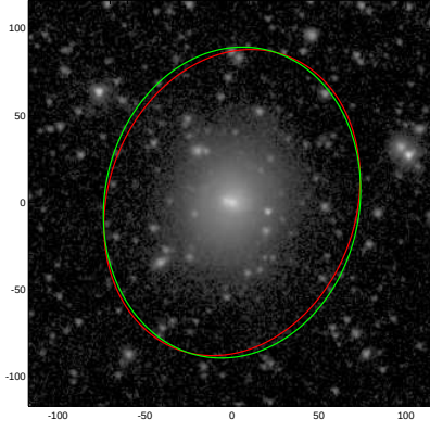
NGC3773
