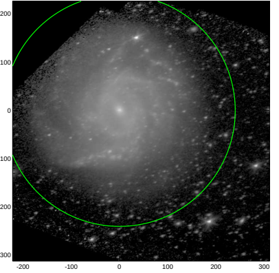
S4G: pa,inc= 18.1 51.0
