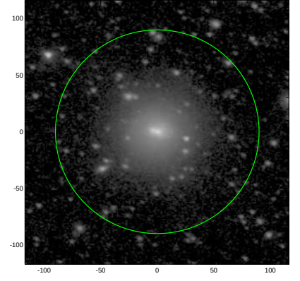
S4G: pa,inc= -11.7 35.7
