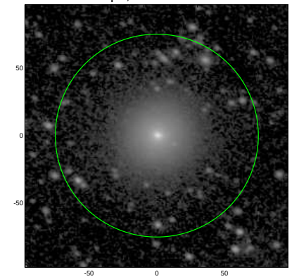
S4G: pa,inc= 161.5 35.3
