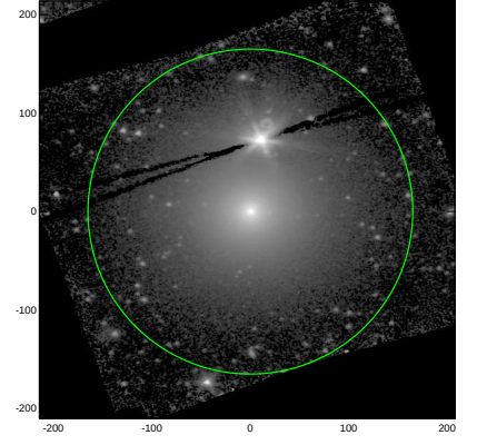
S4G: pa,inc= 3.7 36.9
