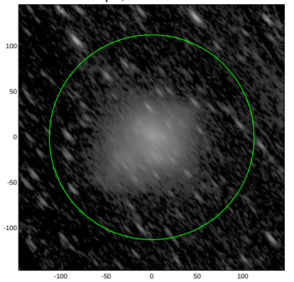
S4G: pa,inc= 130.8 72.6
