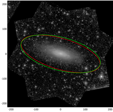
NGC3403
