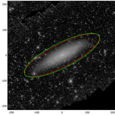
NGC3972
