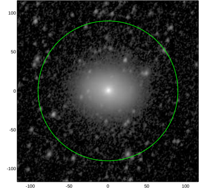
S4G: pa,inc= 63.8 41.9
