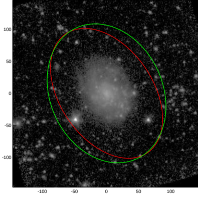
NGC3629
