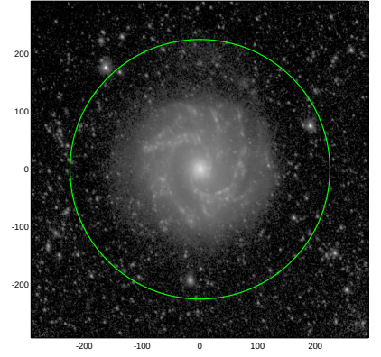
S4G: pa,inc= 112.9 32.9
