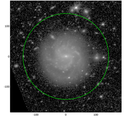
S4G: pa,inc= 19.5 35.2
