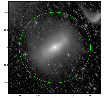
S4G: pa,inc= 111.1 46.9
