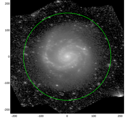
S4G: pa,inc= -8.3 50.8
