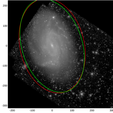
NGC3726
