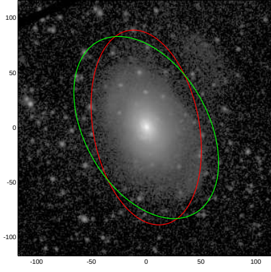
NGC3611
