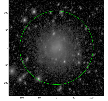
S4G: pa,inc= 76.2 34.6
