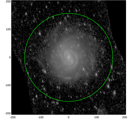
S4G: pa,inc= 101.4 56.1
