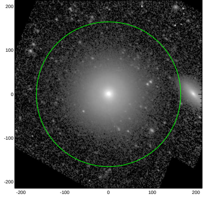
S4G: pa,inc= 135.0 36.0
