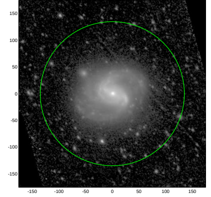
S4G: pa,inc= 131.3 38.6
