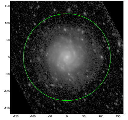
S4G: pa,inc= 120.1 47.3
