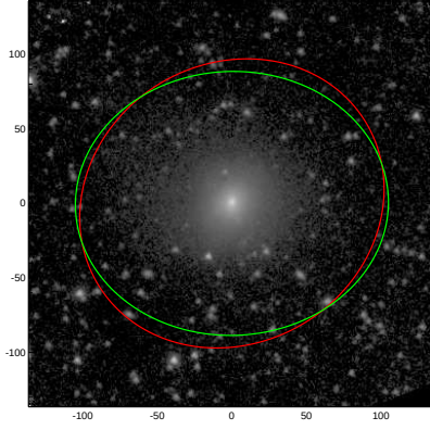
NGC3073
