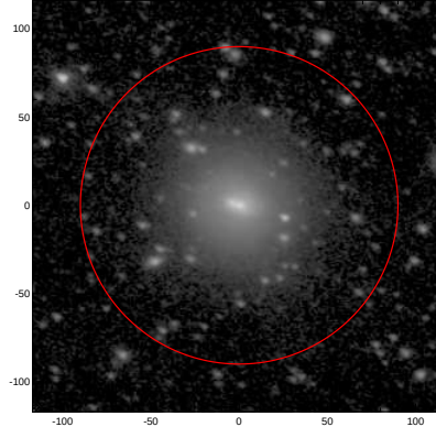
LEDA: pa,inc= 160.0 37.8
