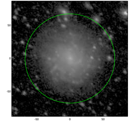
S4G: pa,inc= 140.8 40.7
