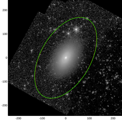
NGC4138
