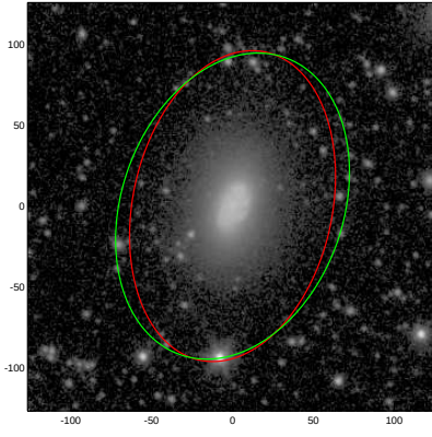
NGC4451
