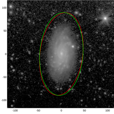
NGC4480
