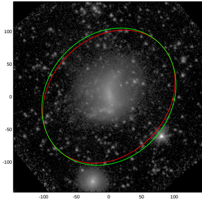
NGC4288
