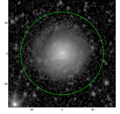
S4G: pa,inc= 94.7 34.2
