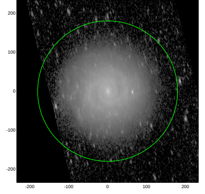
S4G: pa,inc= 99.2 66.6
