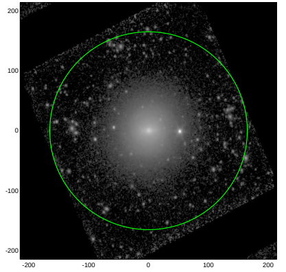
S4G: pa,inc= 85.7 23.8
