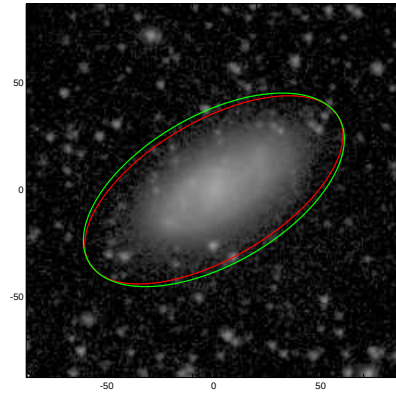
NGC4080
