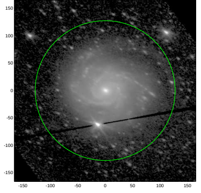
S4G: pa,inc= 152.4 52.0
