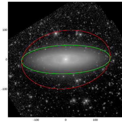
NGC4448
