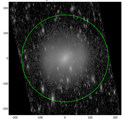
S4G: pa,inc= 93.1 67.4
