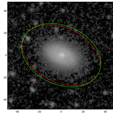
NGC4791
