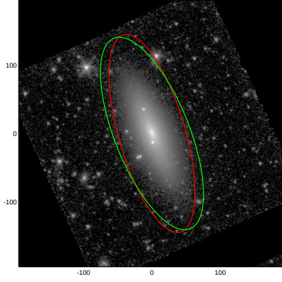
NGC4684
