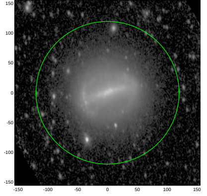
S4G: pa,inc= 96.3 49.9
