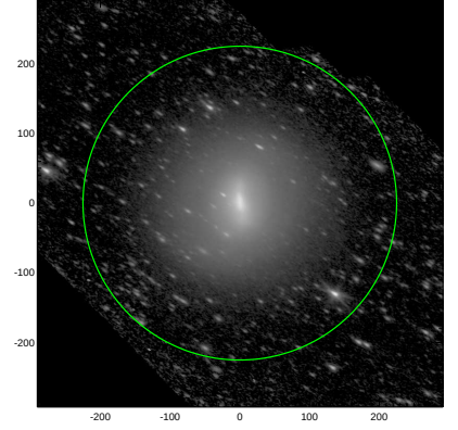
S4G: pa,inc= 148.9 62.0
