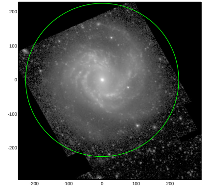
S4G: pa,inc= 143.6 27.1
