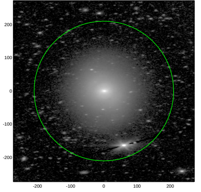
S4G: pa,inc= 4.2 63.0
