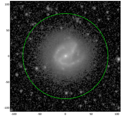
S4G: pa,inc= 57.4 17.1
