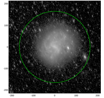
S4G: pa,inc= 110.8 59.2
