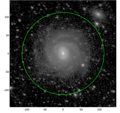
S4G: pa,inc= 152.9 34.8
