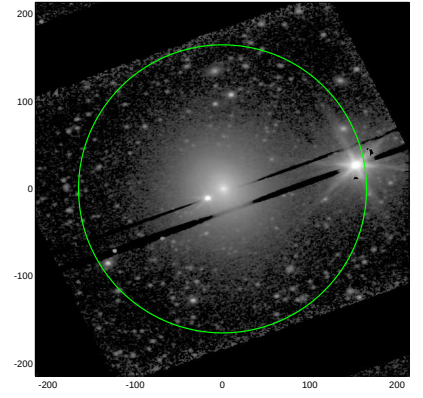
S4G: pa,inc= 9.5 40.9
