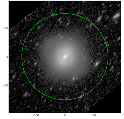
S4G: pa,inc= 55.5 64.2
