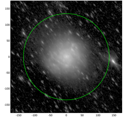
S4G: pa,inc= 128.1 66.3
