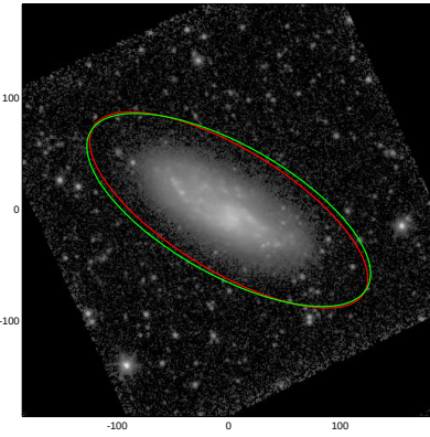
NGC4632
