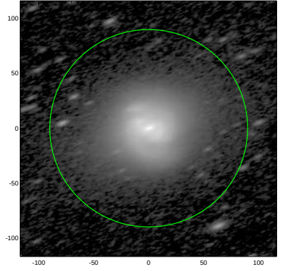
S4G: pa,inc= 22.8 67.0
