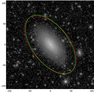
NGC4591
