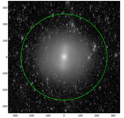
S4G: pa,inc= 88.1 59.0
