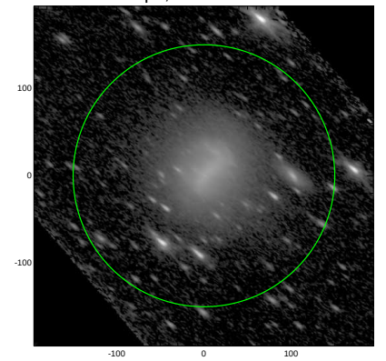
S4G: pa,inc= 143.0 67.0
