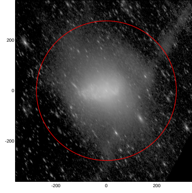
LEDA: pa,inc= 122.5 67.0
