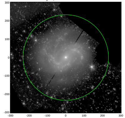
S4G: pa,inc= 122.3 30.5
