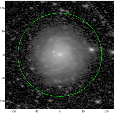
S4G: pa,inc= -10.7 50.5
