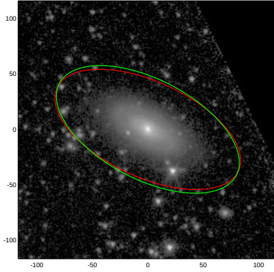
NGC4355
