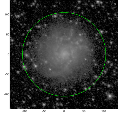
S4G: pa,inc= 144.1 30.1
