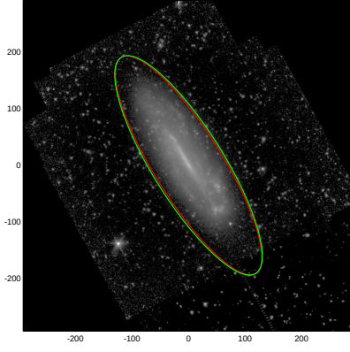
NGC4178
