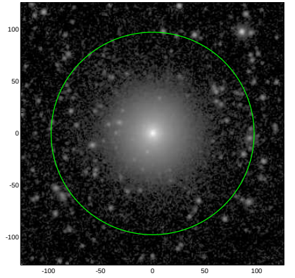
S4G: pa,inc= 54.0 19.6
