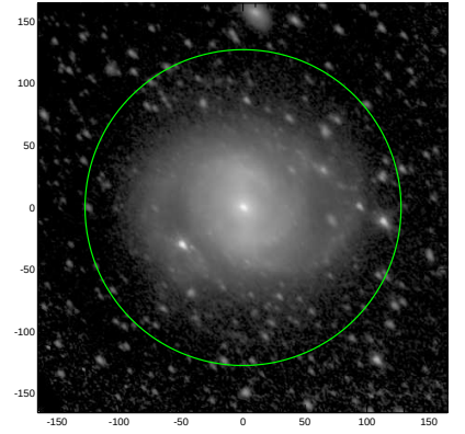
S4G: pa,inc= 134.5 49.2
