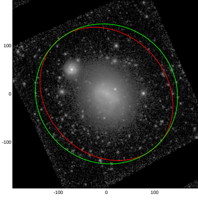
NGC4540
