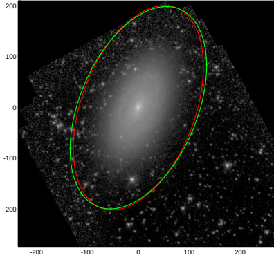
NGC4380
