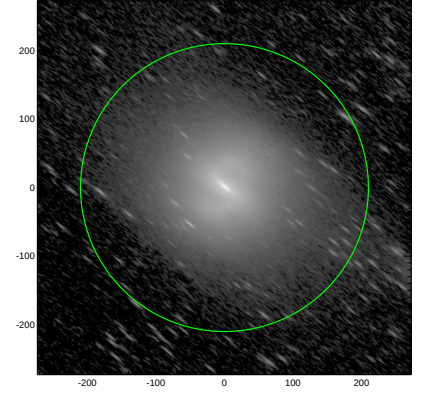
S4G: pa,inc= 141.3 76.6
