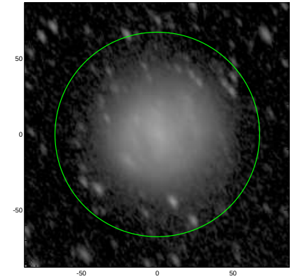
S4G: pa,inc= 120.0 58.9
