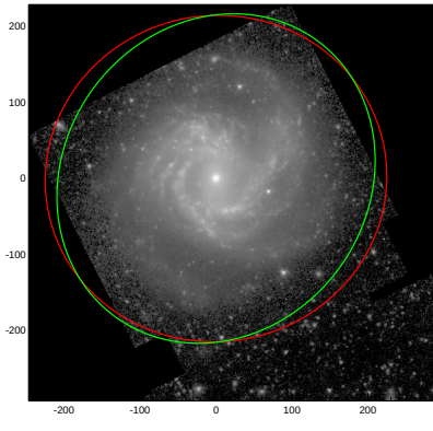
NGC4303
