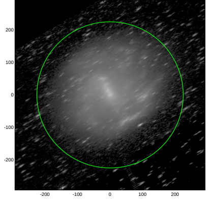
S4G: pa,inc= 31.9 73.7
