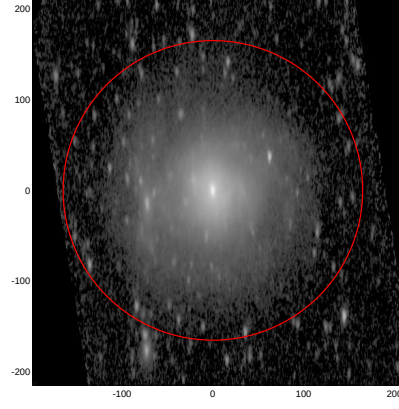
LEDA: pa,inc= 89.7 68.3
