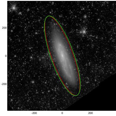
NGC4096
