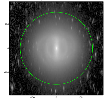
S4G: pa,inc= 92.0 71.2
