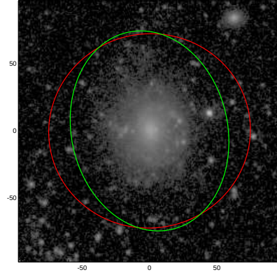
NGC4303A
