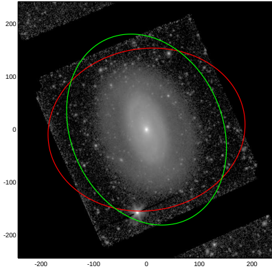
NGC4941
