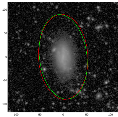
NGC4668
