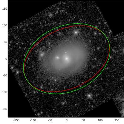
NGC4795
