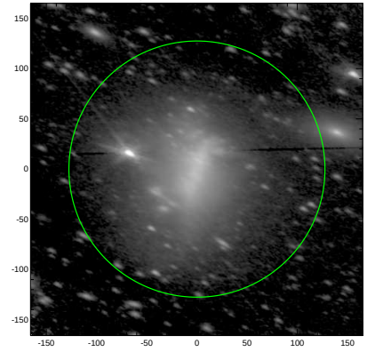
S4G: pa,inc= 156.6 60.3
