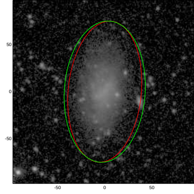
NGC4142
