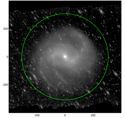
S4G: pa,inc= 125.5 64.2
