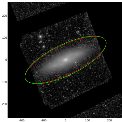
NGC4586
