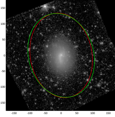
NGC4630
