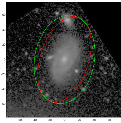
NGC4165
