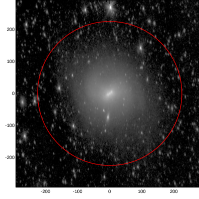
LEDA: pa,inc= 95.3 58.8
