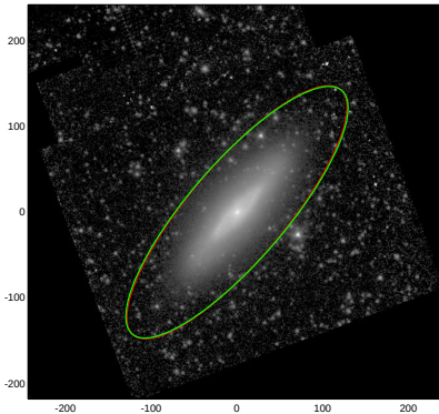
NGC4220
