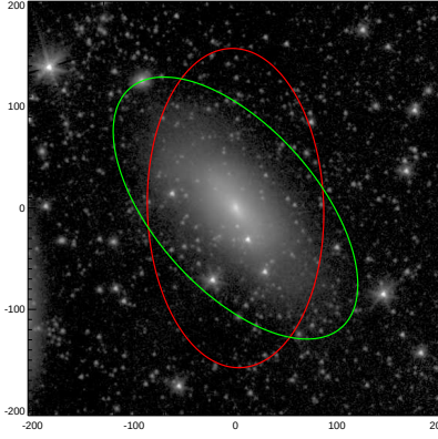
NGC4606
