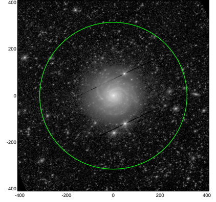
S4G: pa,inc= 29.6 39.0
