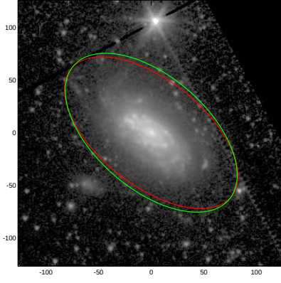
NGC4793
