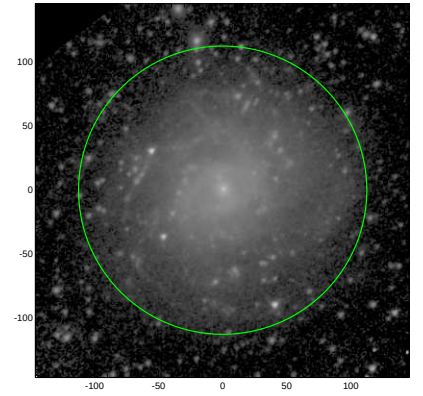
S4G: pa,inc= 44.6 27.3
