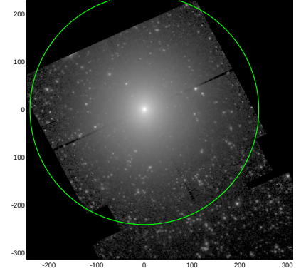
S4G: pa,inc= -1.5 22.5
