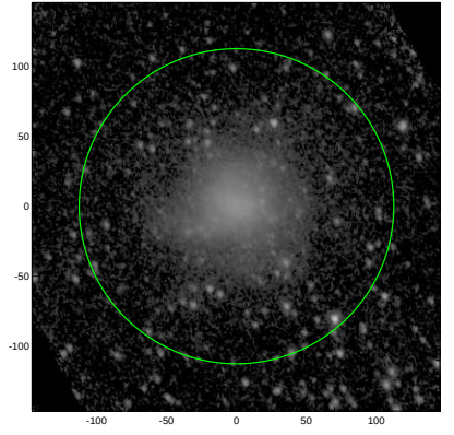
S4G: pa,inc= 113.8 35.8
