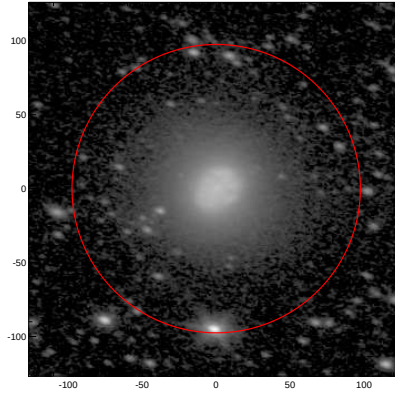
LEDA: pa,inc= 167.9 50.8
