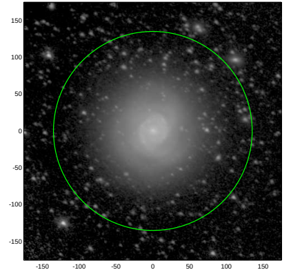
S4G: pa,inc= 155.1 40.7
