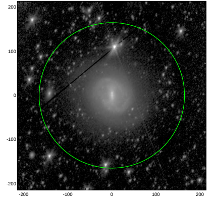
S4G: pa,inc= 69.3 44.6
