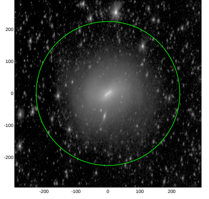
S4G: pa,inc= 85.2 56.4
