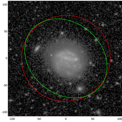
NGC4234
