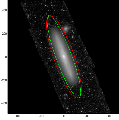
NGC4216
