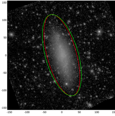
NGC4455
