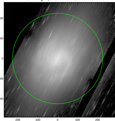
S4G: pa,inc= 62.6 82.8
