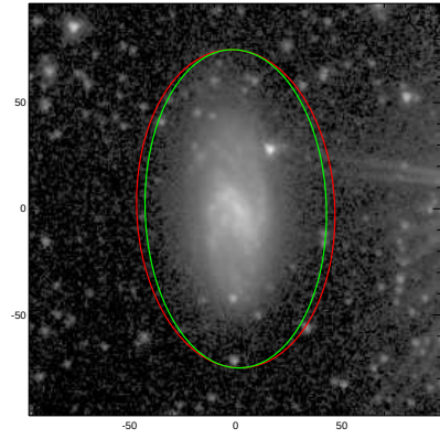
NGC4658
