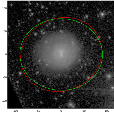
NGC4416
