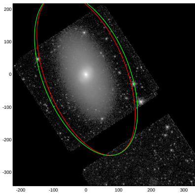
NGC4754
