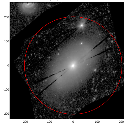
LEDA: pa,inc= 50.0 39.7
