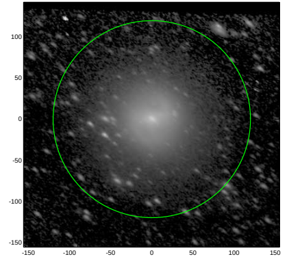
S4G: pa,inc= 146.1 59.0
