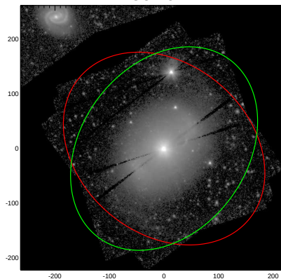
NGC4151
