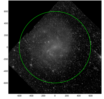
S4G: pa,inc= 135.2 38.3
