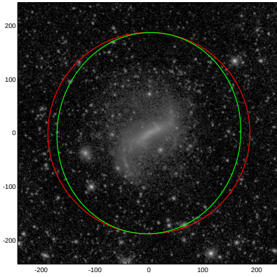
NGC4204
