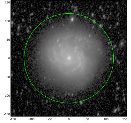
S4G: pa,inc= 74.8 49.1
