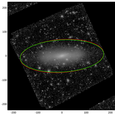
NGC4539
