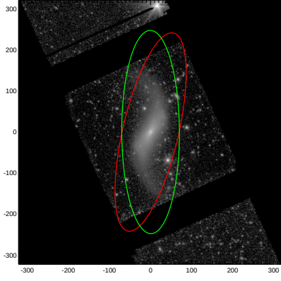
NGC4488
