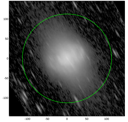
S4G: pa,inc= 119.6 77.4
