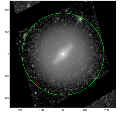
S4G: pa,inc= 57.2 36.8
