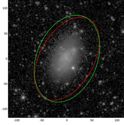
NGC4376
