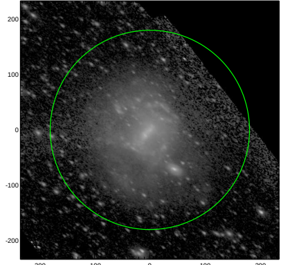
S4G: pa,inc= 144.9 56.1
