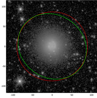
NGC4344
