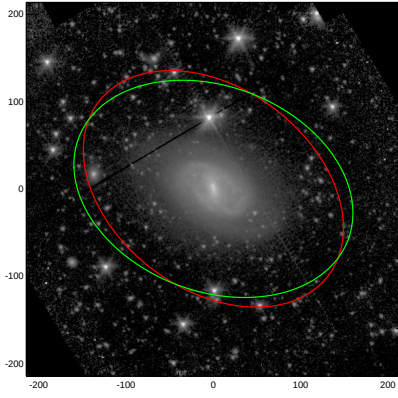
NGC4413
