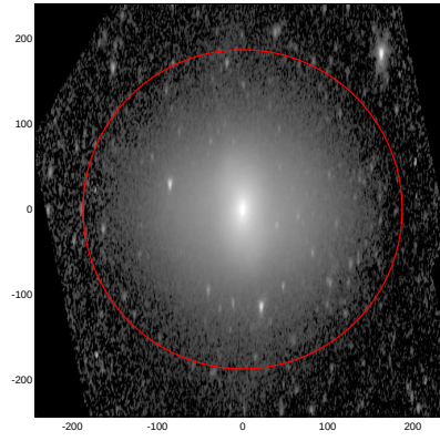
LEDA: pa,inc= 87.0 68.0
