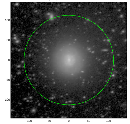
S4G: pa,inc= 18.9 40.5
