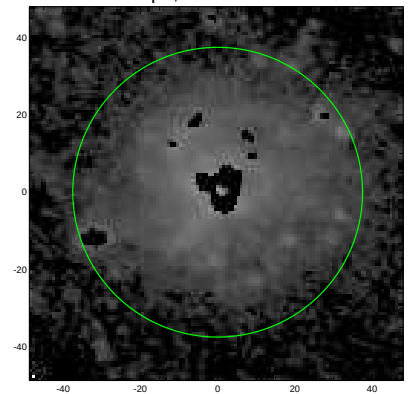
S4G: pa,inc= 152.0 31.4
