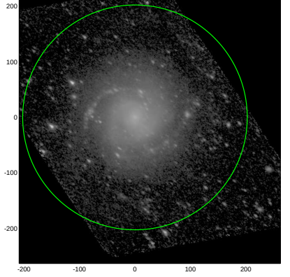
S4G: pa,inc= 141.7 52.8
