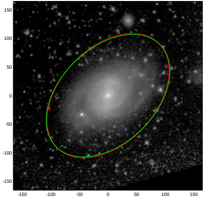
NGC4639
