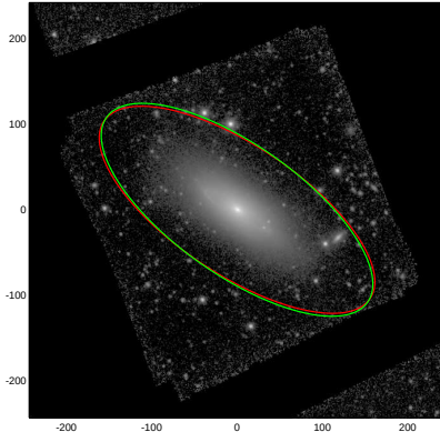
NGC4224
