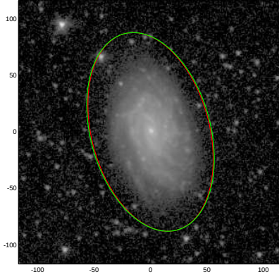
NGC4899
