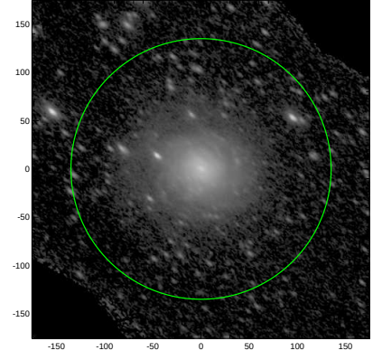
S4G: pa,inc= 139.6 58.8
