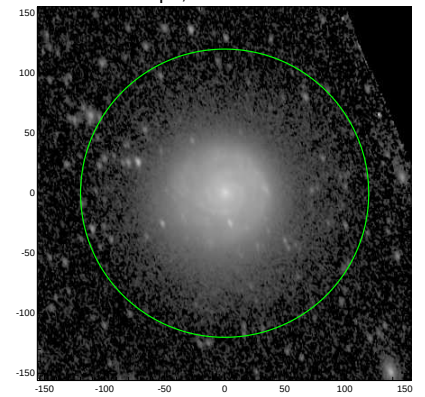
S4G: pa,inc= 105.6 51.6
