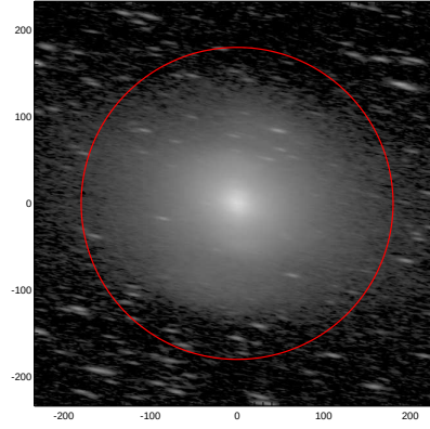
LEDA: pa,inc= 169.9 76.8
