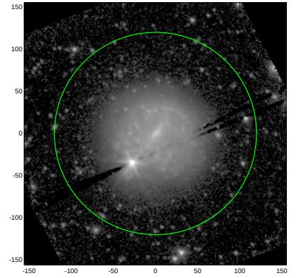
S4G: pa,inc= 140.8 18.5
