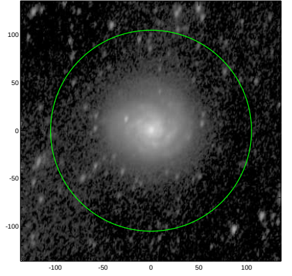
S4G: pa,inc= 74.9 55.8
