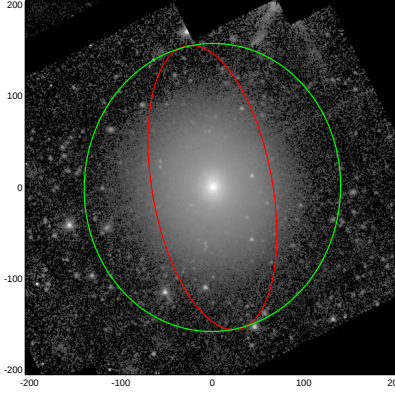
NGC4203
