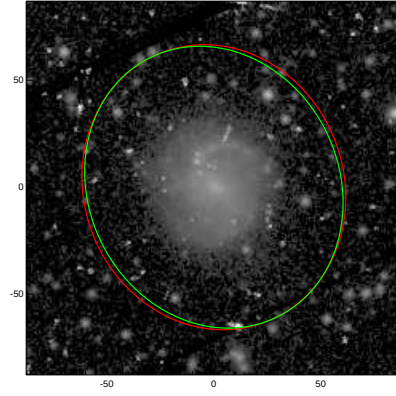
NGC4035
