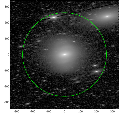
S4G: pa,inc= 9.1 68.1
