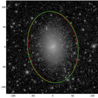
NGC4584
