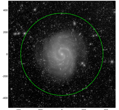
S4G: pa,inc= 22.8 25.6
