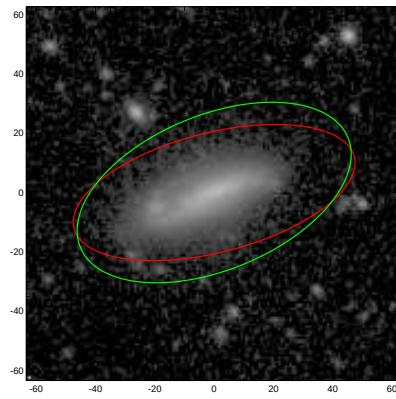
NGC4604
