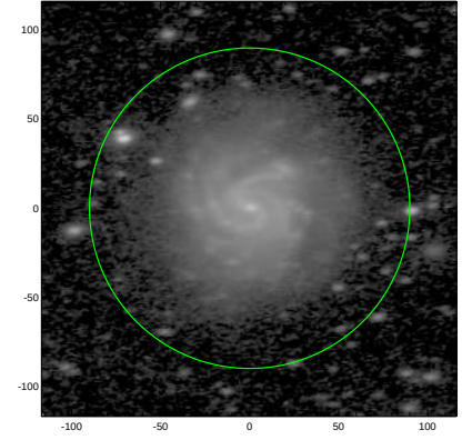
S4G: pa,inc= 7.6 54.4
