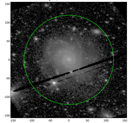
S4G: pa,inc= -10.5 40.4
