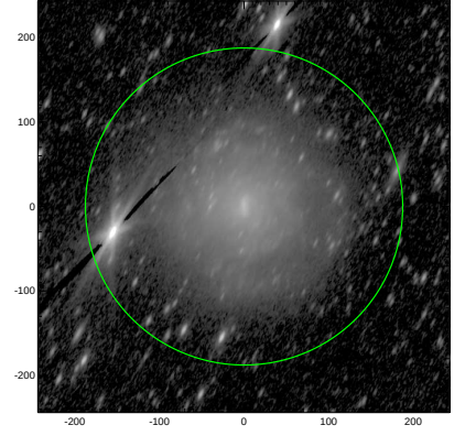
S4G: pa,inc= 63.9 67.9
