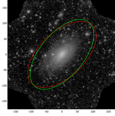
NGC4127
