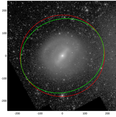
NGC4394
