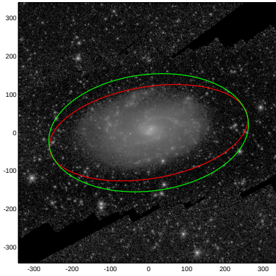
NGC4145
