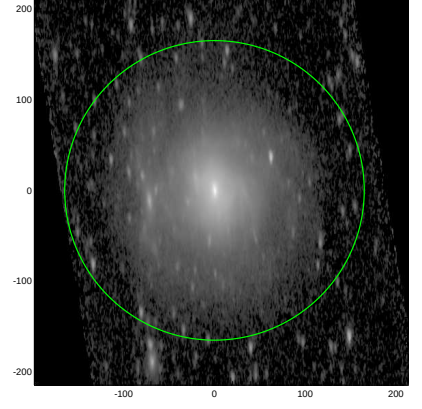
S4G: pa,inc= 91.5 70.3
