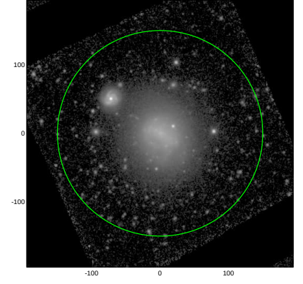
S4G: pa,inc= 56.0 18.0
