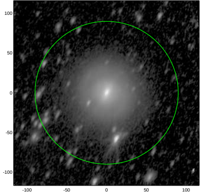
S4G: pa,inc= 62.5 59.9
