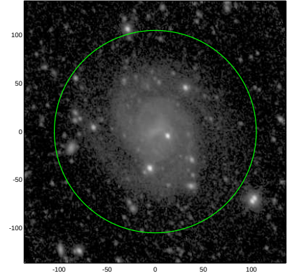
S4G: pa,inc= 115.2 32.4
