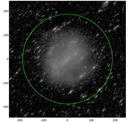
S4G: pa,inc= 42.5 64.6
