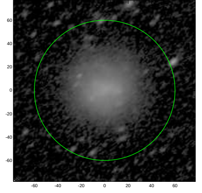
S4G: pa,inc= 40.0 57.3
