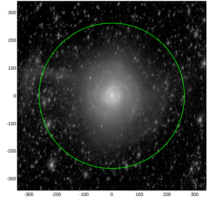
S4G: pa,inc= 77.7 54.6
