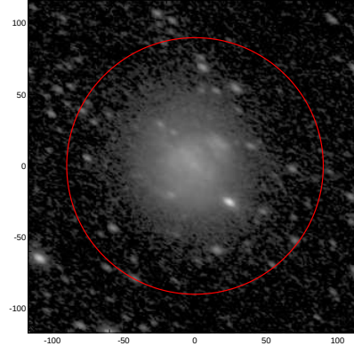
LEDA: pa,inc= 150.2 53.4
