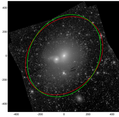
NGC4105
