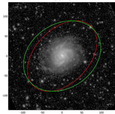
NGC4152
