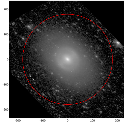
LEDA: pa,inc= 145.8 50.6
