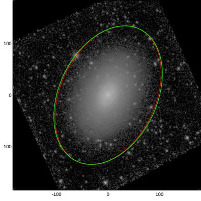
NGC4531
