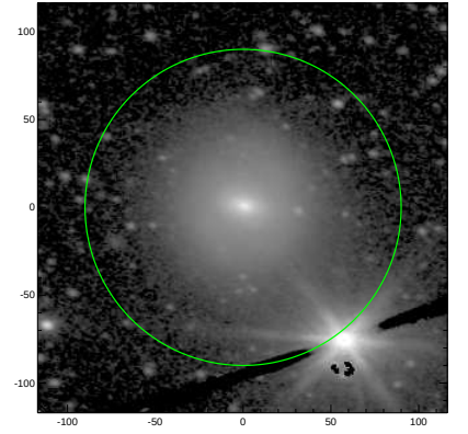
S4G: pa,inc= -6.5 43.5
