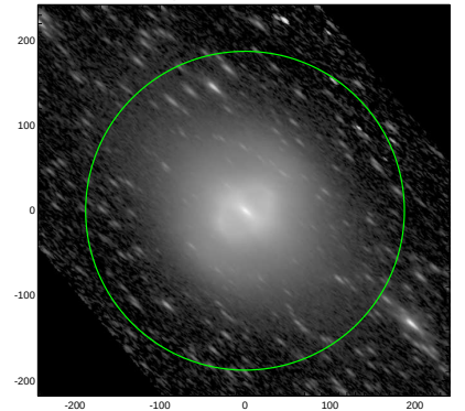
S4G: pa,inc= 139.3 72.4
