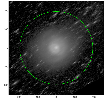
S4G: pa,inc= 34.2 74.8
