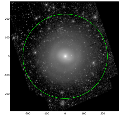
S4G: pa,inc= 66.4 21.7
