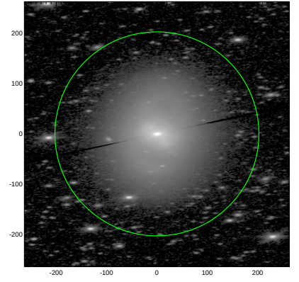
S4G: pa,inc= 4.5 67.2
