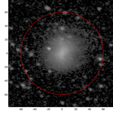
LEDA: pa,inc= 170.0 39.6
