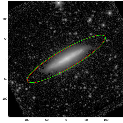
NGC4746
