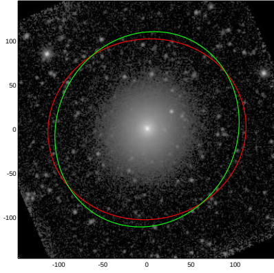
NGC4489
