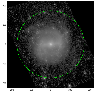
S4G: pa,inc= 122.7 46.9
