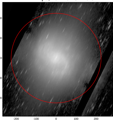
LEDA: pa,inc= 64.8 79.5
