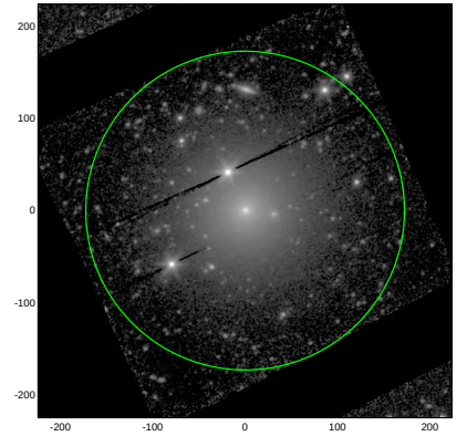
S4G: pa,inc= 27.9 25.9
