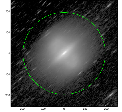
S4G: pa,inc= 41.6 79.7
