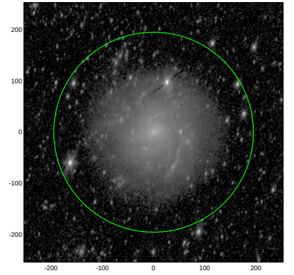
S4G: pa,inc= 75.3 51.3
