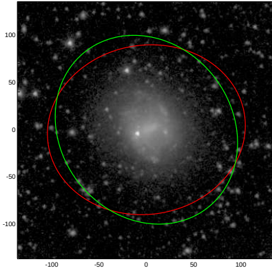
NGC4561
