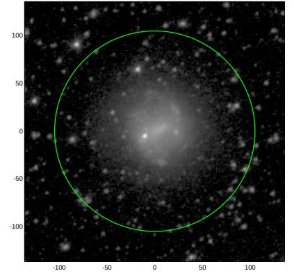
S4G: pa,inc= 37.6 29.9
