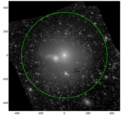
S4G: pa,inc= 150.4 37.4
