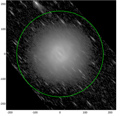
S4G: pa,inc= 133.7 76.3
