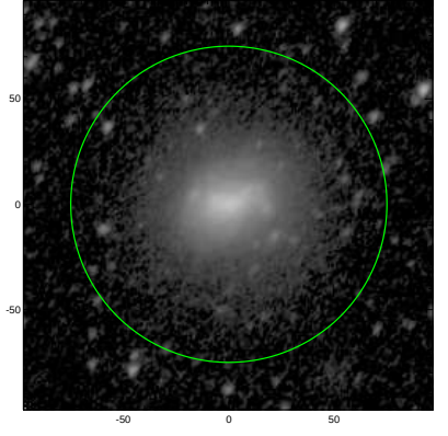
S4G: pa,inc= 55.4 46.9
