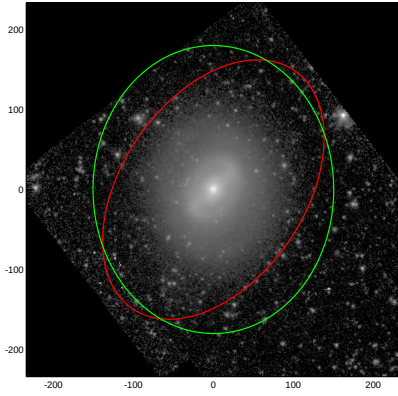
NGC4245
