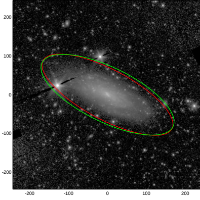
NGC4094
