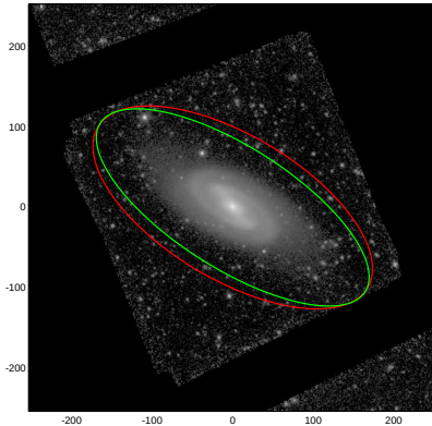
NGC4260
