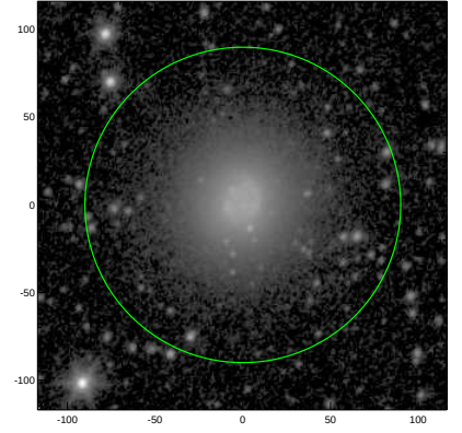
S4G: pa,inc= 56.6 28.4
