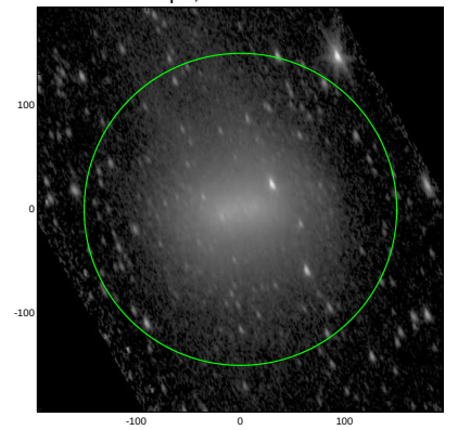
S4G: pa,inc= 110.3 62.1
