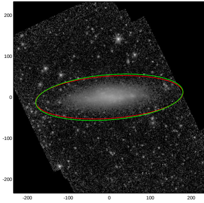
NGC4592
