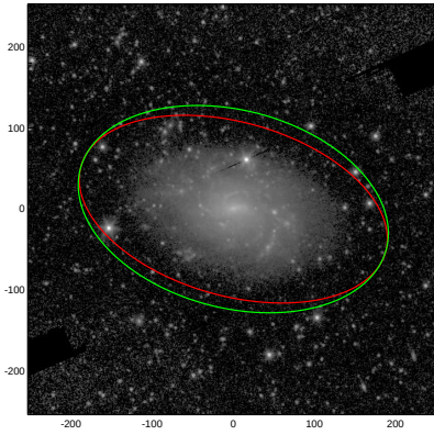
NGC4487
