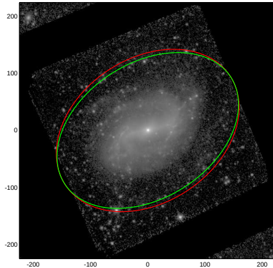
NGC4123
