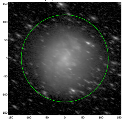
S4G: pa,inc= 154.6 64.0
