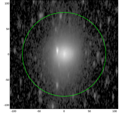
S4G: pa,inc= 88.2 70.9
