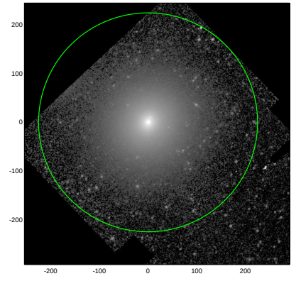
S4G: pa,inc= 41.9 32.7
