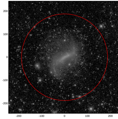
LEDA: pa,inc= 999.0 0.0
