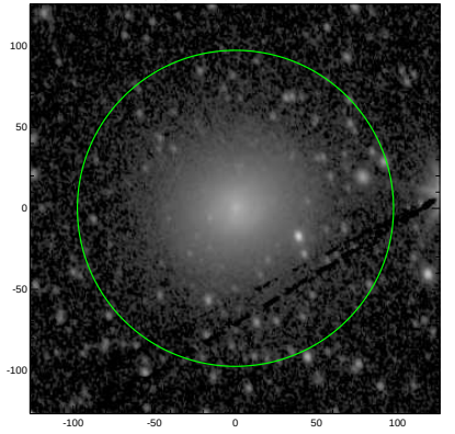
S4G: pa,inc= 104.4 39.1
