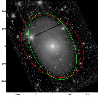
NGC4984
