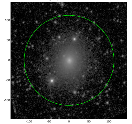
S4G: pa,inc= 70.1 24.1
