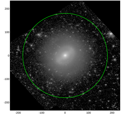
S4G: pa,inc= 0.2 33.3
