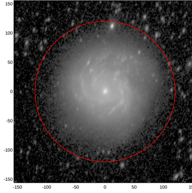
LEDA: pa,inc= 73.2 52.8
