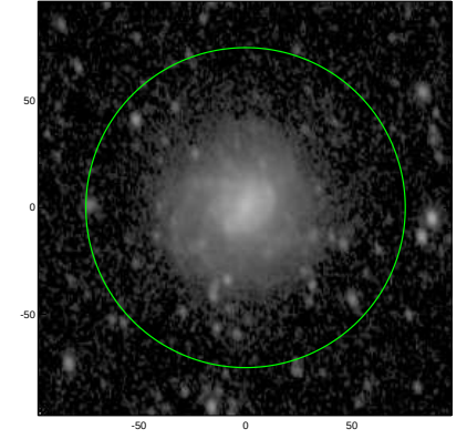
S4G: pa,inc= 99.2 45.4
