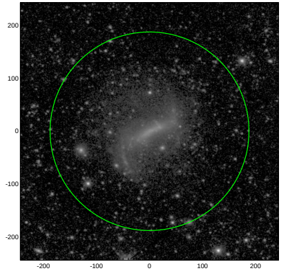
S4G: pa,inc= -6.4 24.6
