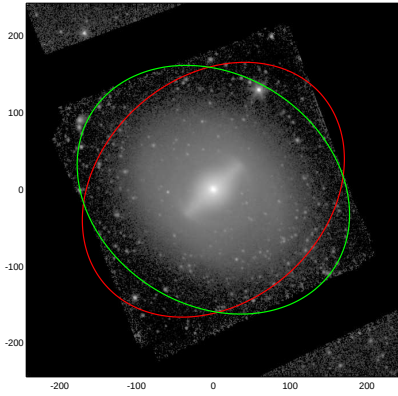
NGC4643
