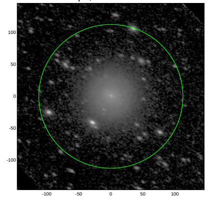
S4G: pa,inc= 152.7 51.8
