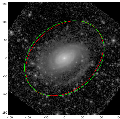
NGC4814
