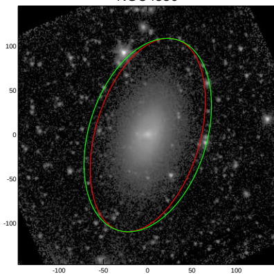
NGC4336
