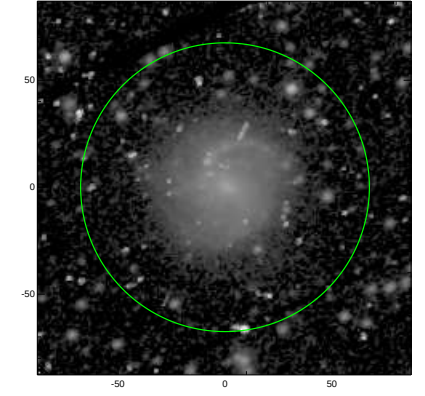
S4G: pa,inc= 26.0 29.8
