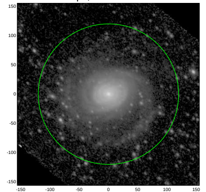
S4G: pa,inc= 128.6 39.7
