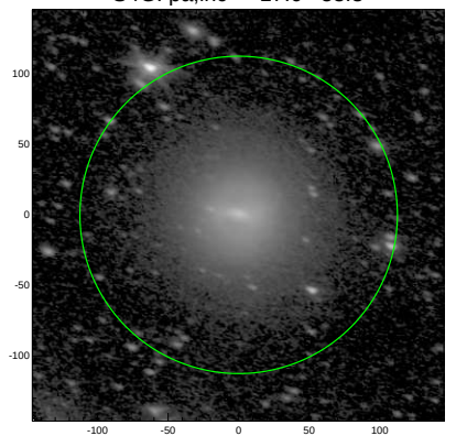
S4G: pa,inc= -17.6 53.8
