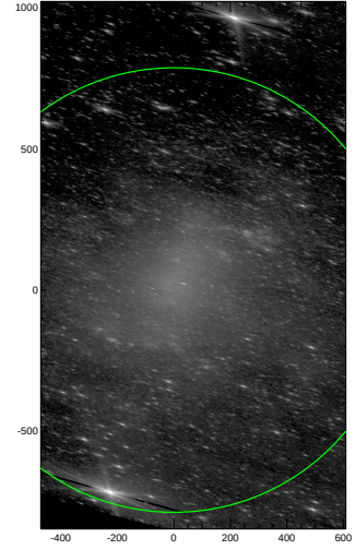
S4G: pa,inc= -18.5 73.7
