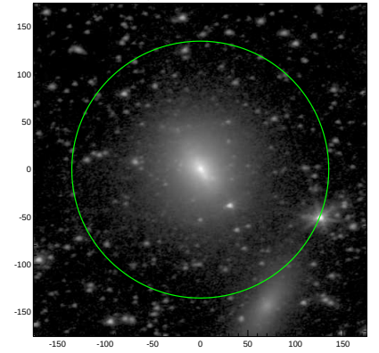
S4G: pa,inc= 8.3 44.5
