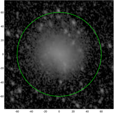
S4G: pa,inc= 112.3 41.5
