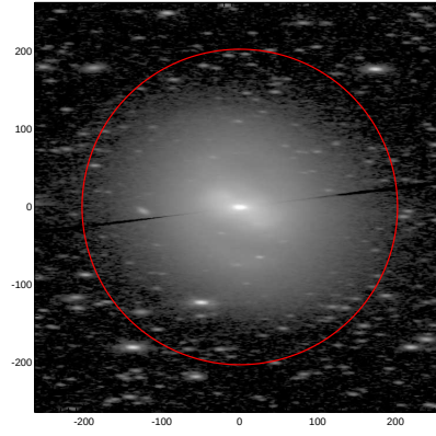
LEDA: pa,inc= 179.3 72.5
