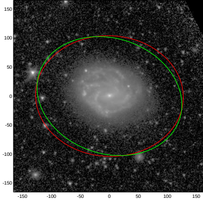
NGC4189
