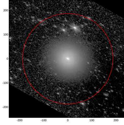
LEDA: pa,inc= 150.0 55.9
