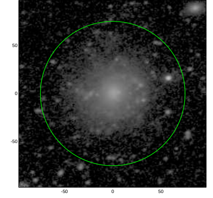
S4G: pa,inc= 12.5 39.3
