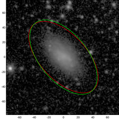
NGC4502
