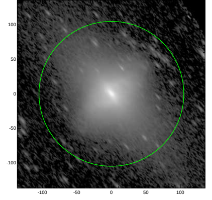
S4G: pa,inc= 130.0 69.5
