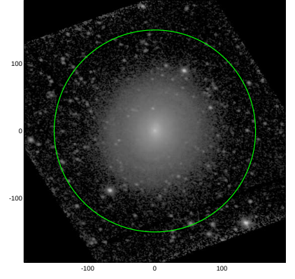
S4G: pa,inc= -17.3 37.5
