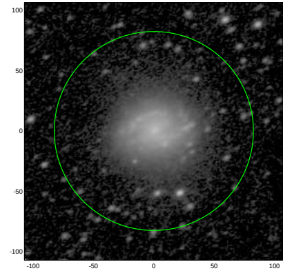
S4G: pa,inc= 28.3 44.8
