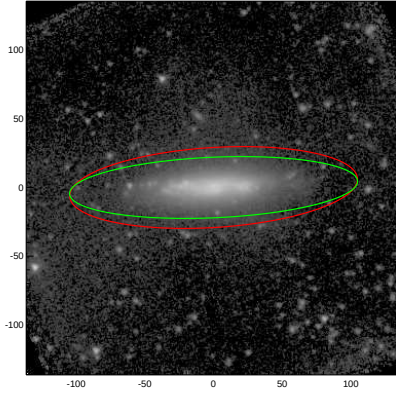
NGC4129
