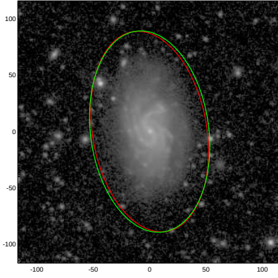
NGC4545
