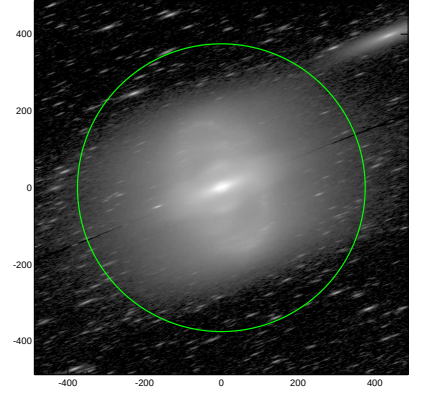
S4G: pa,inc= 20.4 79.6
