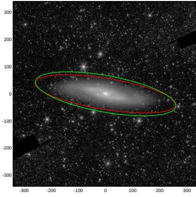
NGC4845
