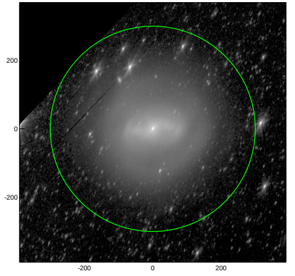
S4G: pa,inc= 64.0 62.1
