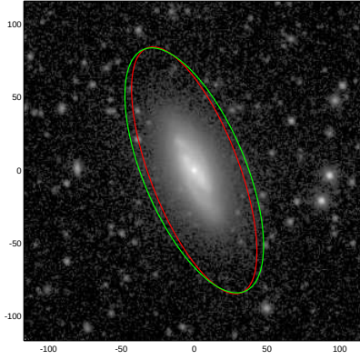
NGC4180
