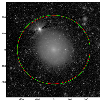
NGC4571
