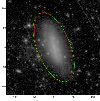
NGC4020
