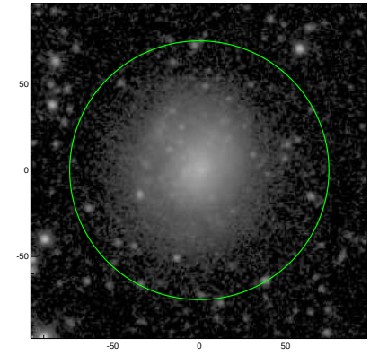
S4G: pa,inc= 31.5 16.7
