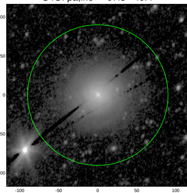
S4G: pa,inc= 67.5 40.4
