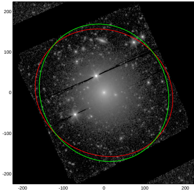
NGC4492
