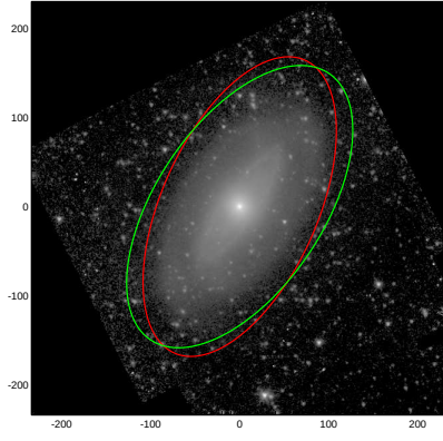
NGC4772
