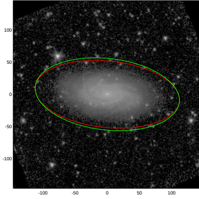
NGC4682
