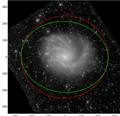
NGC4254
