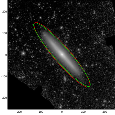
NGC4256
