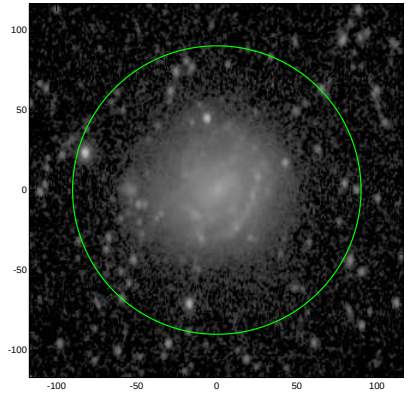
S4G: pa,inc= 87.4 40.2
