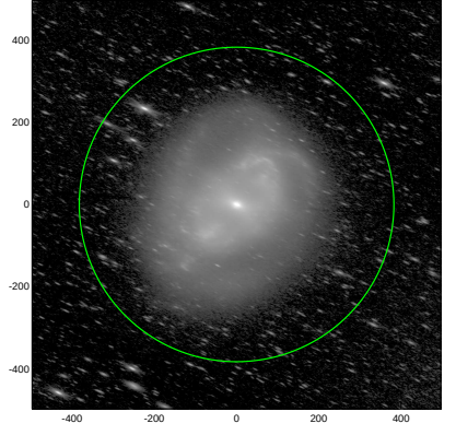
S4G: pa,inc= 156.3 72.0
