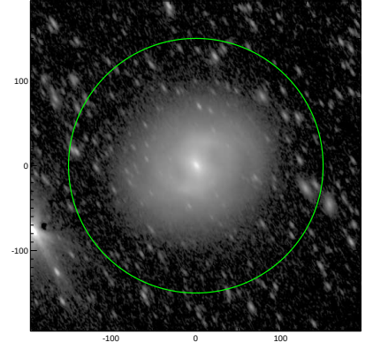
S4G: pa,inc= 120.0 63.3
