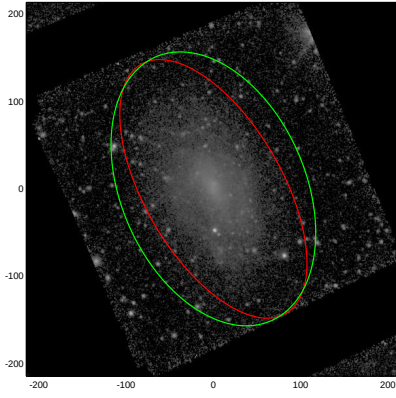
NGC4517A
