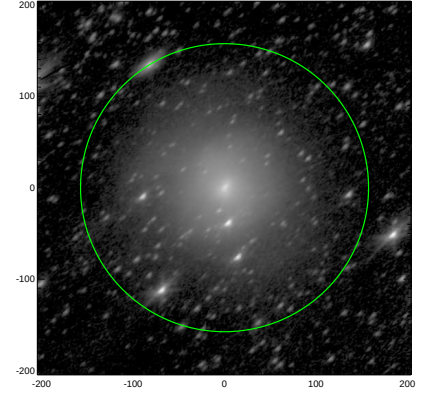
S4G: pa,inc= 41.6 59.4
