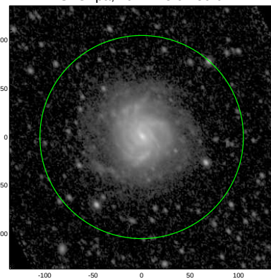
S4G: pa,inc= 123.9 39.6
