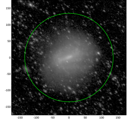
S4G: pa,inc= 138.2 52.2
