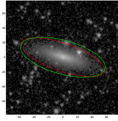
NGC4287
