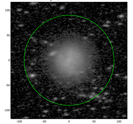
S4G: pa,inc= 7.1 56.3
