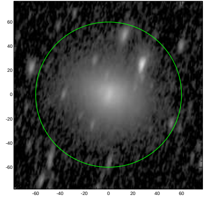
S4G: pa,inc= 74.7 67.5
