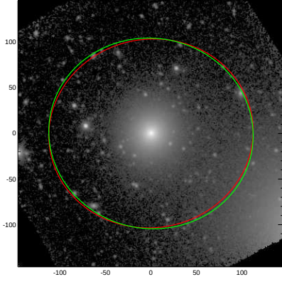
NGC4283
