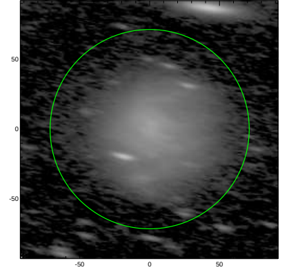
S4G: pa,inc= -12.0 73.0
