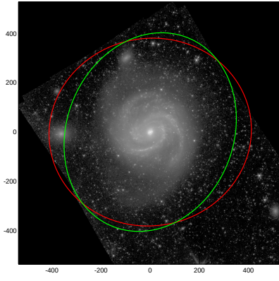
NGC4321
