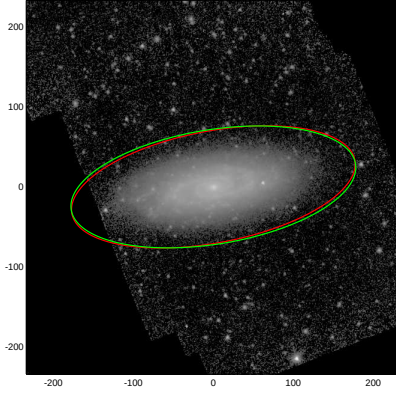
NGC4062
