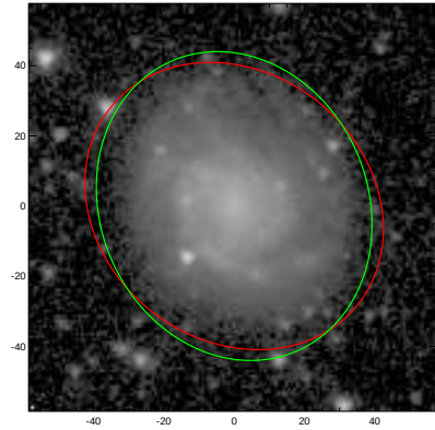
NGC4806
