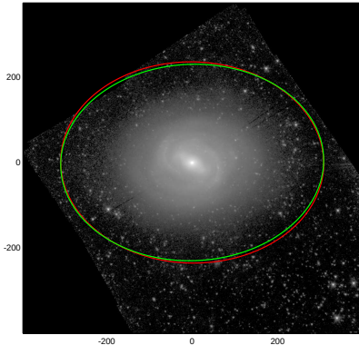
NGC4579
