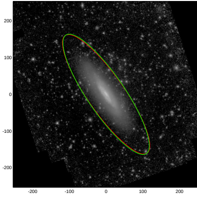
NGC4522
