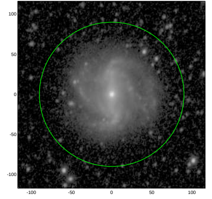
S4G: pa,inc= 68.9 36.7
