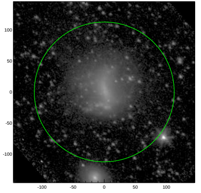
S4G: pa,inc= 138.7 33.0
