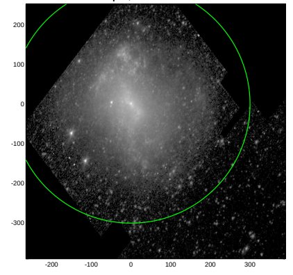
S4G: pa,inc= 71.0 45.1
