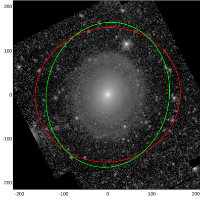
NGC4378
