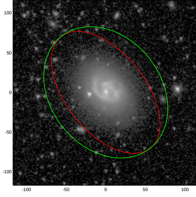
NGC4680
