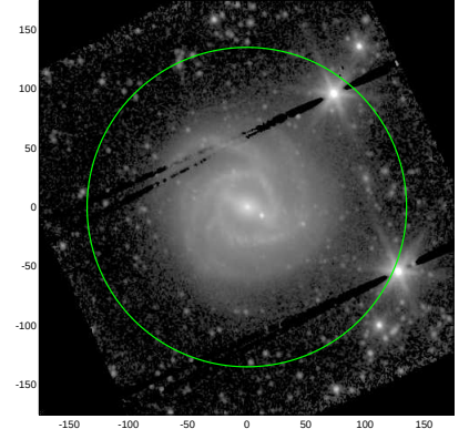
S4G: pa,inc= 101.4 21.5
