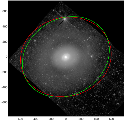
NGC4736
