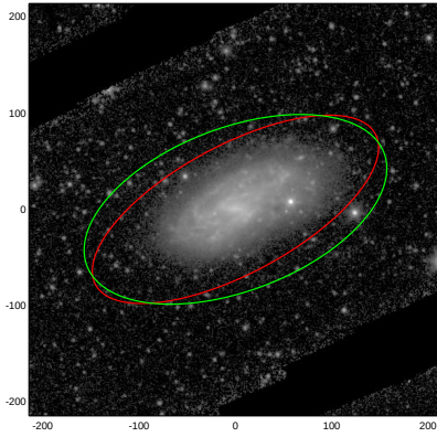
NGC4781
