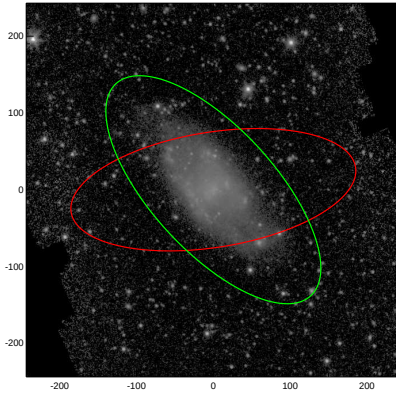
NGC4597
