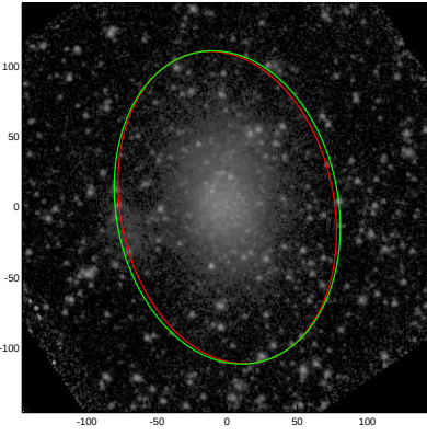
NGC4163
