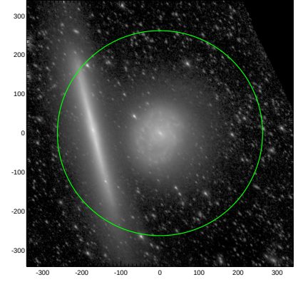
S4G: pa,inc= 131.1 54.8
