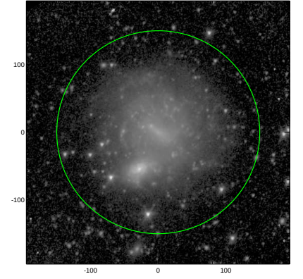
S4G: pa,inc= 62.4 29.1
