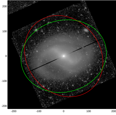
NGC4593
