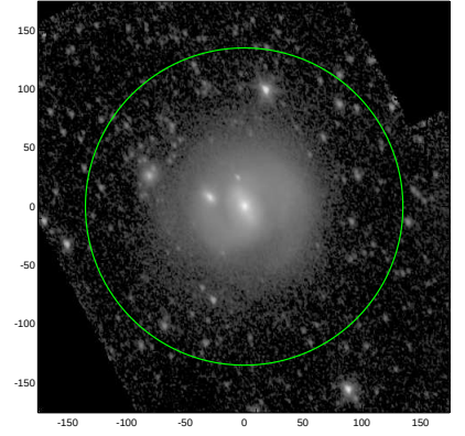
S4G: pa,inc= 114.8 43.7
