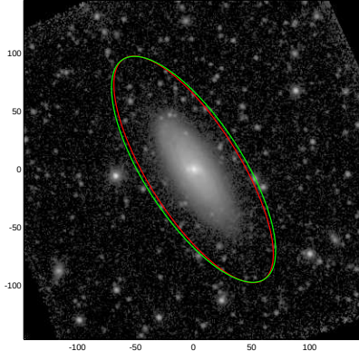
NGC4722
