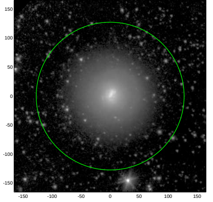
S4G: pa,inc= 101.2 13.0
