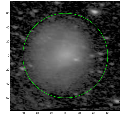
S4G: pa,inc= -10.4 59.0
