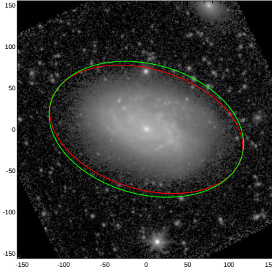
NGC4212
