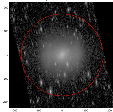
LEDA: pa,inc= 93.9 66.7
