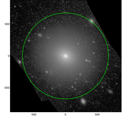
S4G: pa,inc= 153.2 44.4
