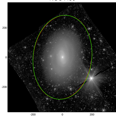
NGC4450
