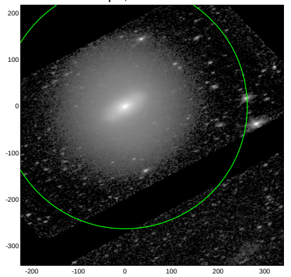
S4G: pa,inc= 22.4 59.7
