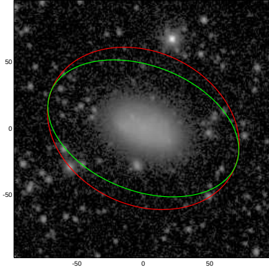
NGC4353
