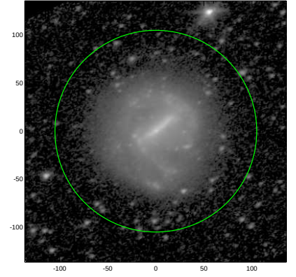
S4G: pa,inc= 26.3 44.9
