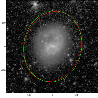
NGC4027
