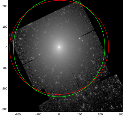
NGC4494
