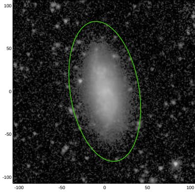
NGC4409
