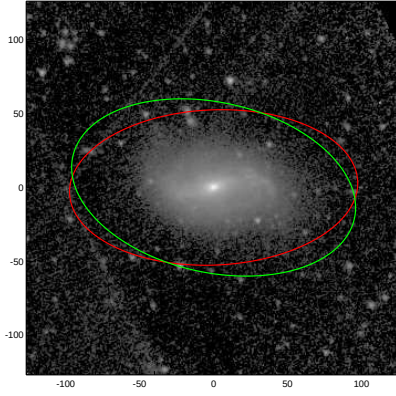
NGC4385
