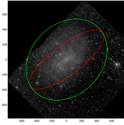
NGC4395
