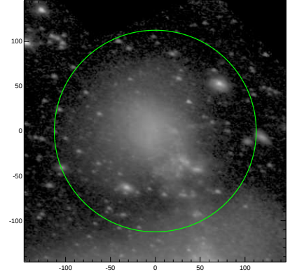
S4G: pa,inc= -14.3 44.6
