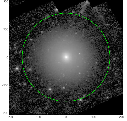
S4G: pa,inc= -2.1 27.1
