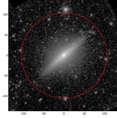
LEDA: pa,inc= 999.0 0.0
