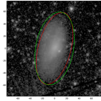
NGC4980
