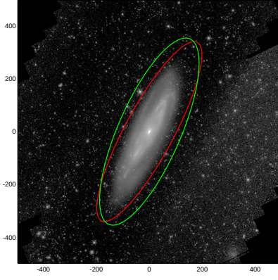
NGC4192
