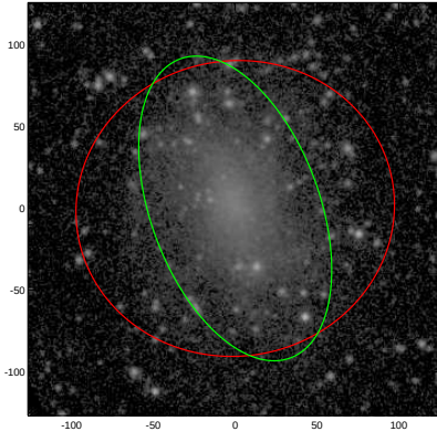
NGC4393
