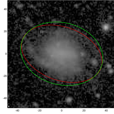
NGC4141
