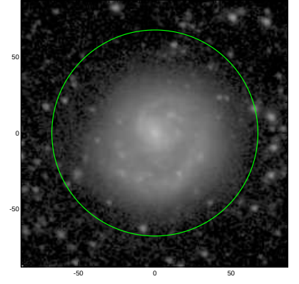
S4G: pa,inc= -18.9 20.0
