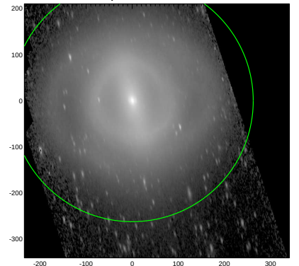
S4G: pa,inc= 101.2 70.2
