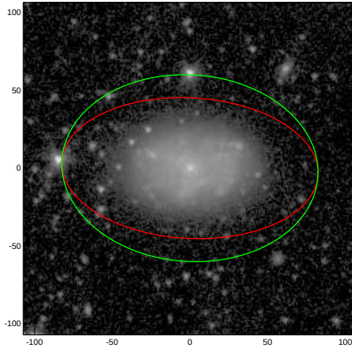
NGC4790
