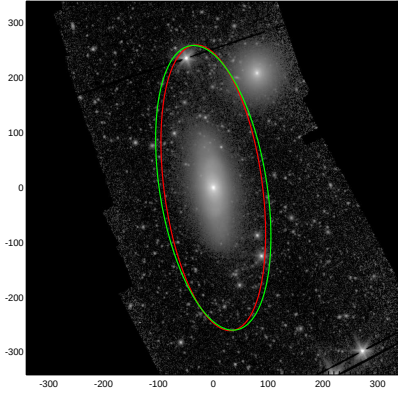
NGC4461
