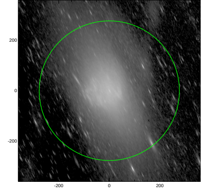
S4G: pa,inc= 115.2 77.3
