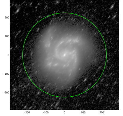
S4G: pa,inc= 53.2 68.9
