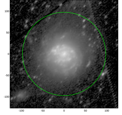
S4G: pa,inc= 49.2 56.7
