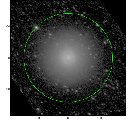
S4G: pa,inc= 154.5 48.2
