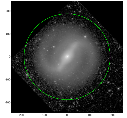
S4G: pa,inc= 51.6 20.4
