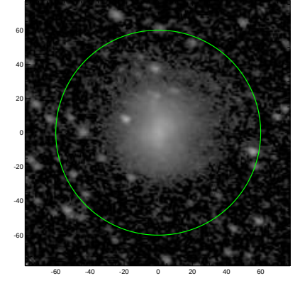
S4G: pa,inc= 158.1 40.6
