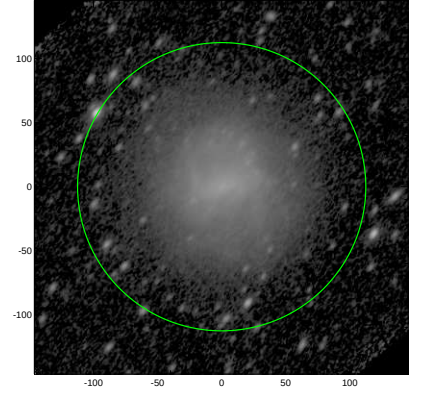
S4G: pa,inc= 53.2 56.8
