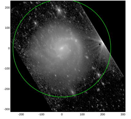
S4G: pa,inc= 120.7 56.7
