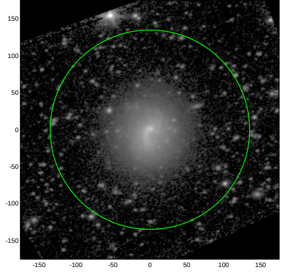
S4G: pa,inc= 15.5 39.9
