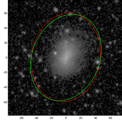
NGC4920
