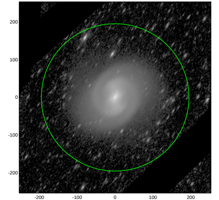
S4G: pa,inc= 57.5 67.2
