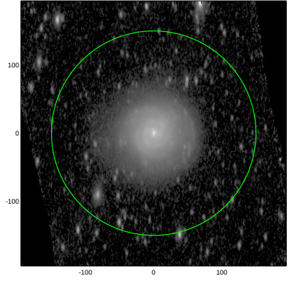
S4G: pa,inc= 88.8 62.7
