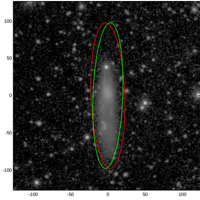
NGC4331
