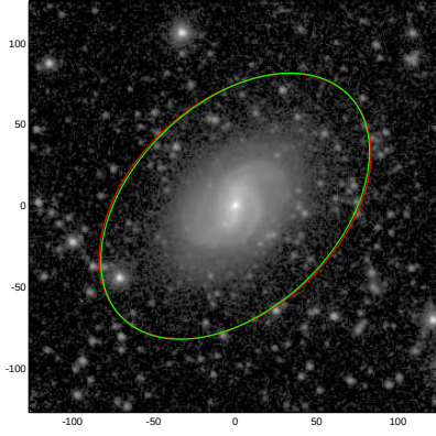
NGC4133
