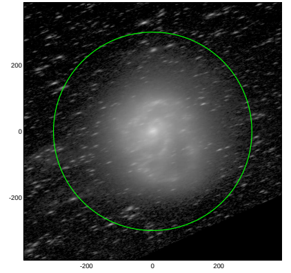
S4G: pa,inc= 19.7 74.0
