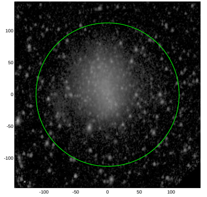
S4G: pa,inc= 81.3 41.2
