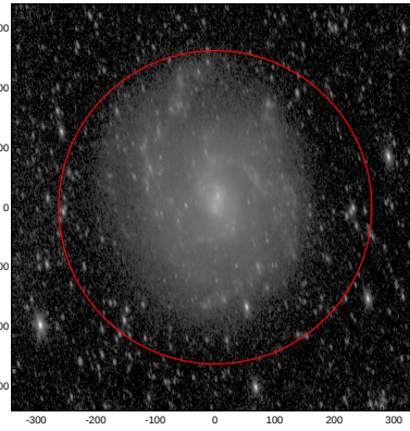
LEDA: pa,inc= 99.5 62.8
