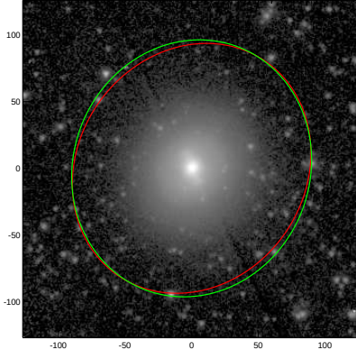
NGC4262
