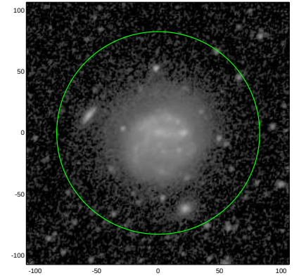
S4G: pa,inc= 50.6 36.4
