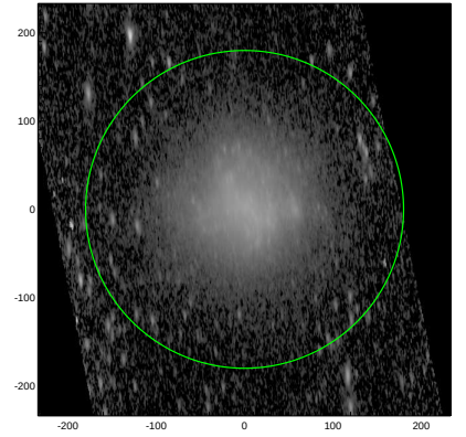
S4G: pa,inc= 94.6 72.2
