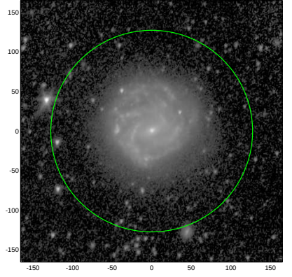
S4G: pa,inc= 71.7 38.7
