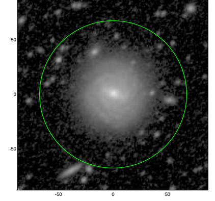
S4G: pa,inc= 44.2 41.9
