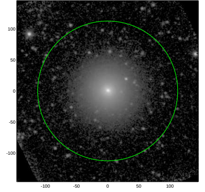
S4G: pa,inc= 153.4 24.6
