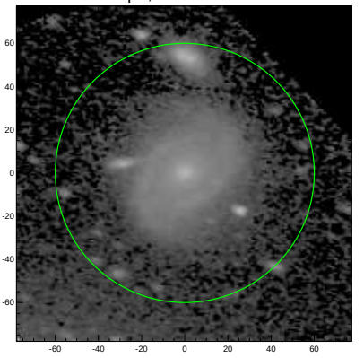
S4G: pa,inc= -10.2 48.3
