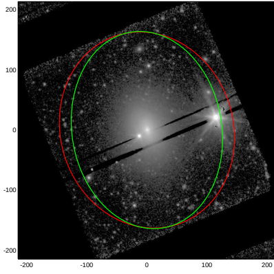
NGC4802
