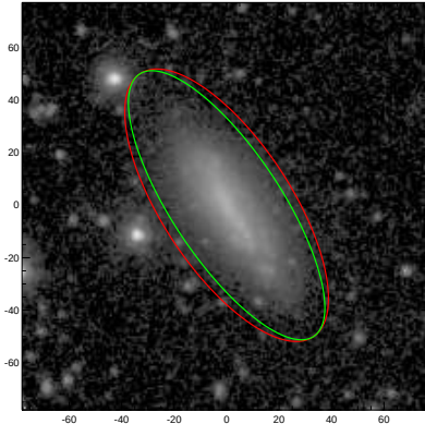
NGC4159
