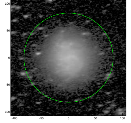
S4G: pa,inc= 9.4 60.9
