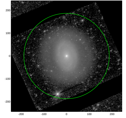
S4G: pa,inc= 23.5 40.0
