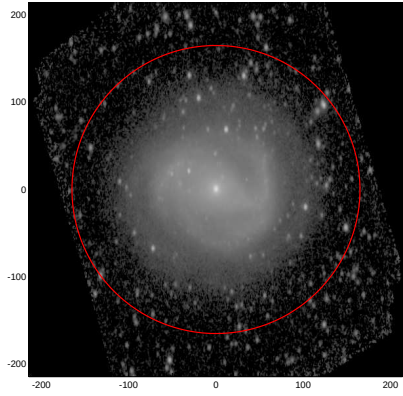
LEDA: pa,inc= 89.0 51.3
