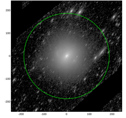
S4G: pa,inc= 54.7 66.1
