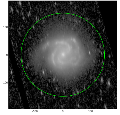
S4G: pa,inc= 100.7 67.8
