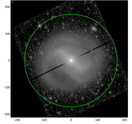
S4G: pa,inc= 104.4 33.4
