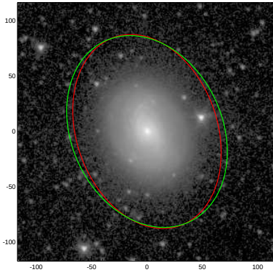
NGC4800
