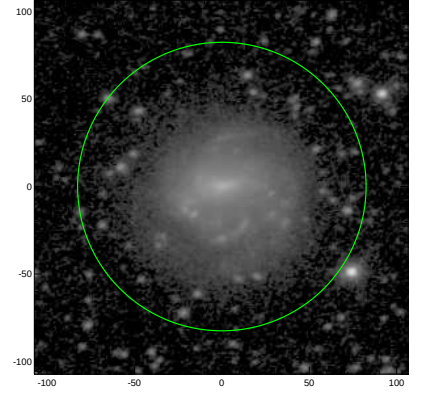
S4G: pa,inc= 12.2 35.5
