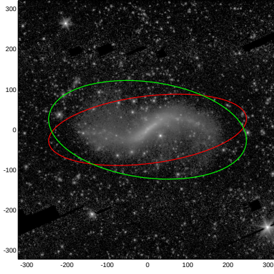
NGC4731
