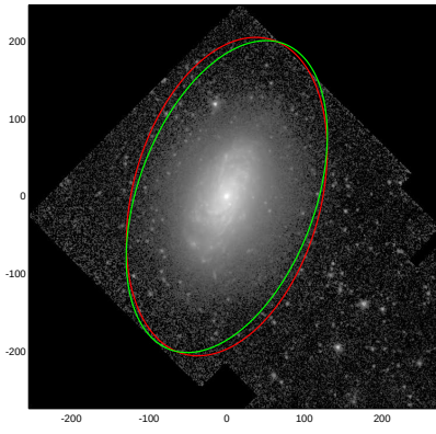
NGC4414
