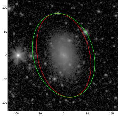
NGC4034
