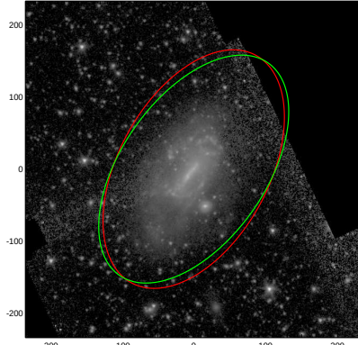
NGC4116
