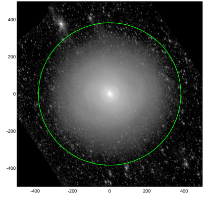
S4G: pa,inc= 115.9 56.4
