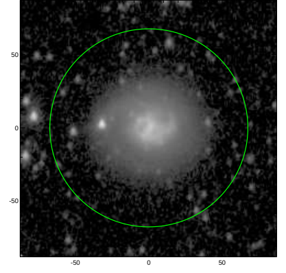
S4G: pa,inc= 82.6 38.4
