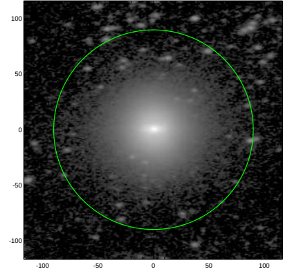
S4G: pa,inc= 6.0 54.6
