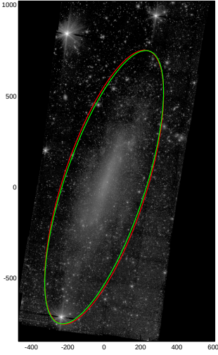
NGC4236
