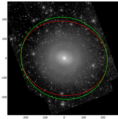
NGC4457
