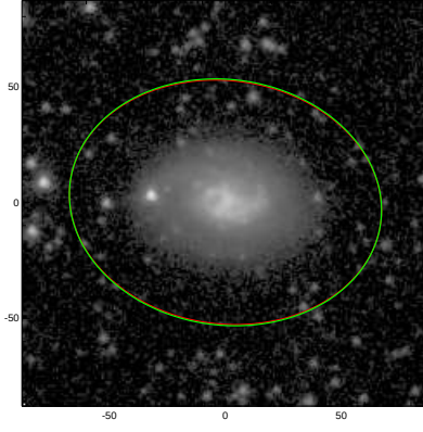
NGC4384
