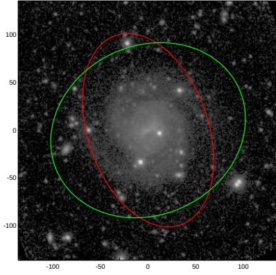
NGC4411A
