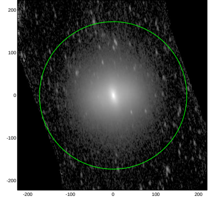
S4G: pa,inc= 99.0 67.8
