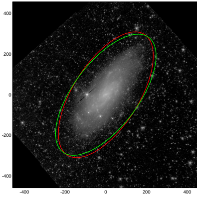
NGC4559
