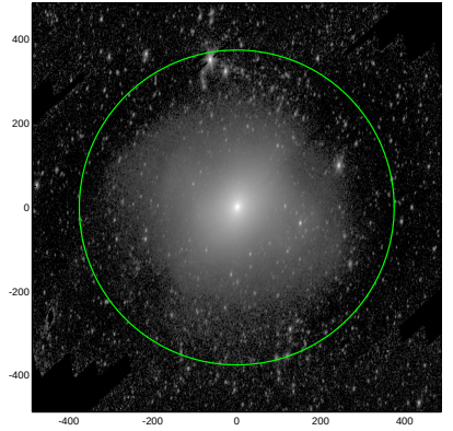
S4G: pa,inc= 82.2 57.2
