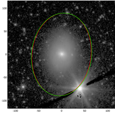
NGC4659
