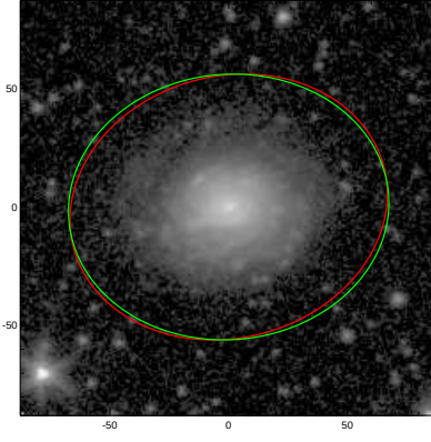
NGC4108
