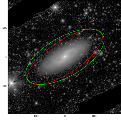
NGC4462
