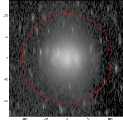
LEDA: pa,inc= 93.6 73.9
