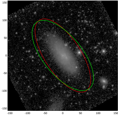
NGC4633
