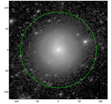
S4G: pa,inc= 25.0 40.9
