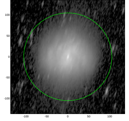
S4G: pa,inc= 75.3 75.1
