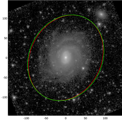
NGC4897
