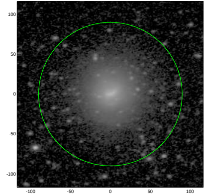
S4G: pa,inc= 7.9 44.9
