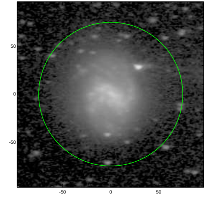
S4G: pa,inc= 1.6 55.3
