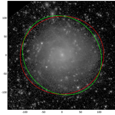
NGC4136
