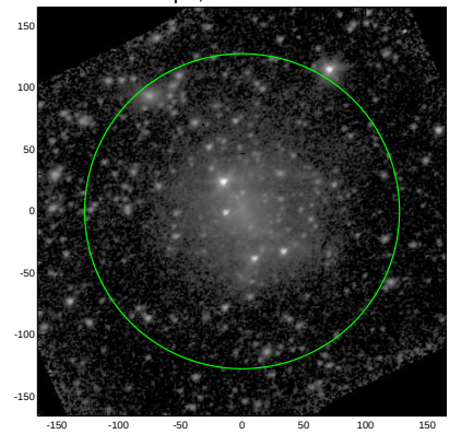
S4G: pa,inc= 28.6 31.7
