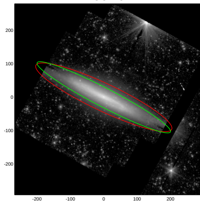
NGC4157
