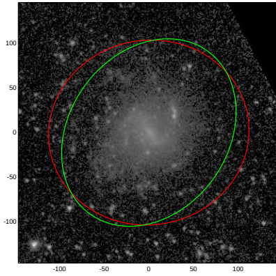
NGC4688
