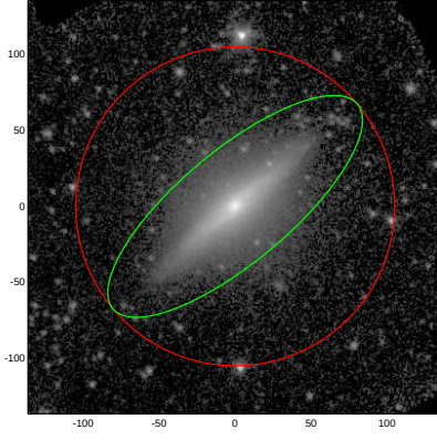
NGC4343
