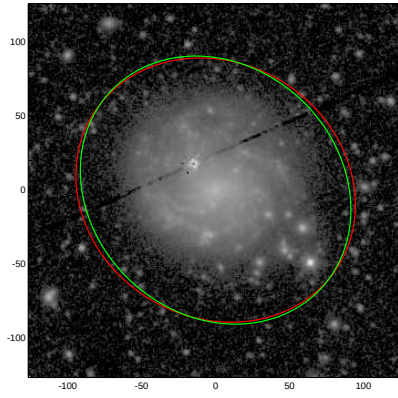
NGC4775
