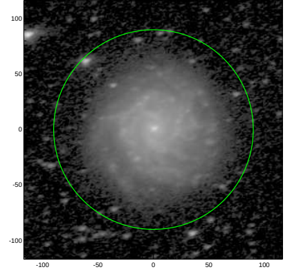
S4G: pa,inc= 15.2 53.8
