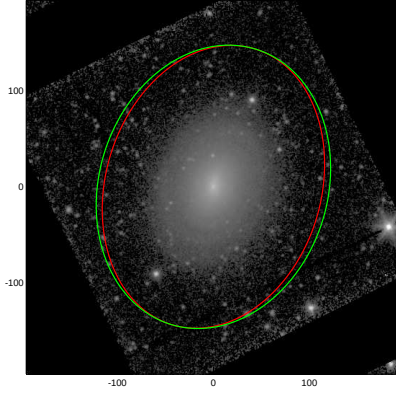
NGC4880
