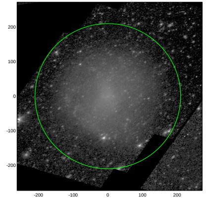
S4G: pa,inc= 29.4 45.7
