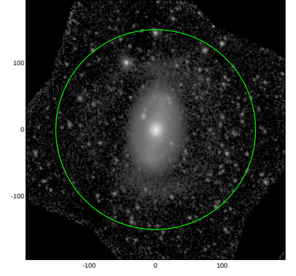
S4G: pa,inc= 99.0 28.7
