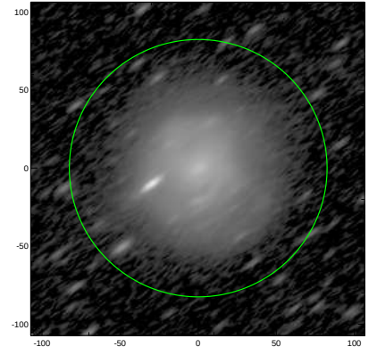
S4G: pa,inc= 36.8 72.3
