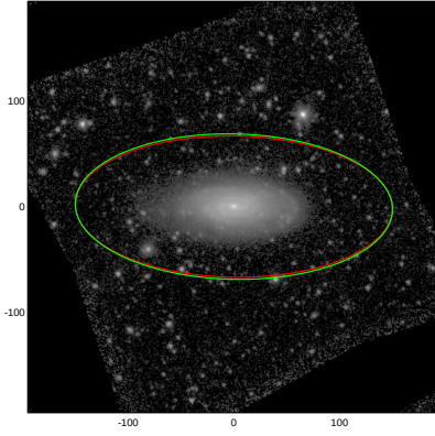
NGC4193
