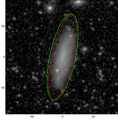
NGC4120
