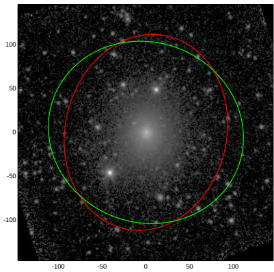
NGC4641
