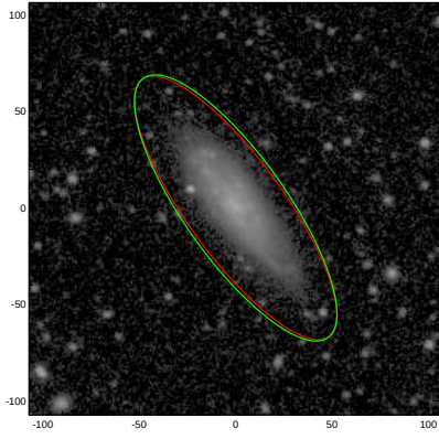
NGC4238
