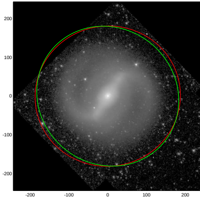
NGC4314
