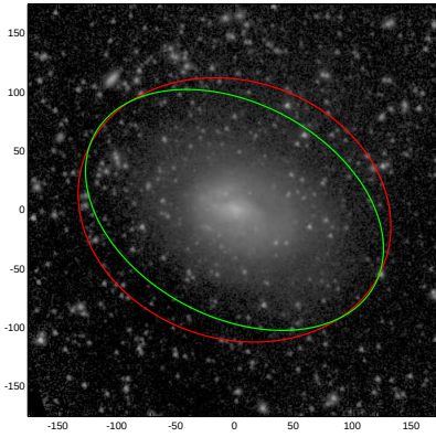
NGC4351
