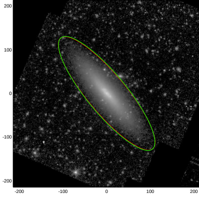
NGC4460
