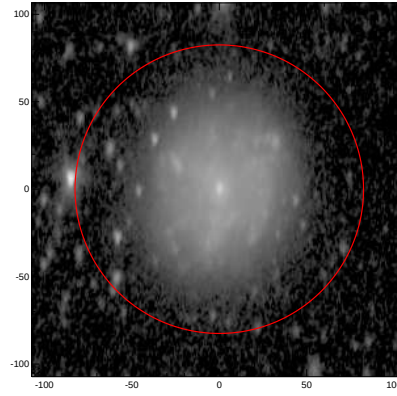
LEDA: pa,inc= 87.0 56.8
