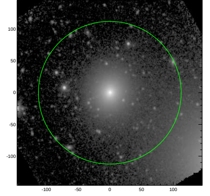
S4G: pa,inc= 80.7 22.0
