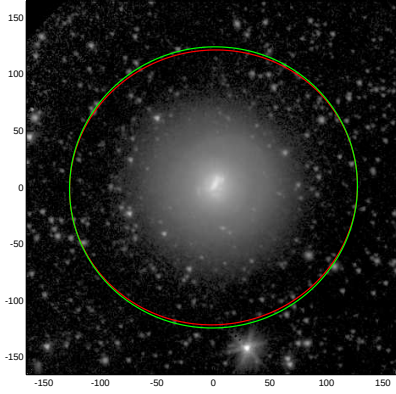
NGC4369
