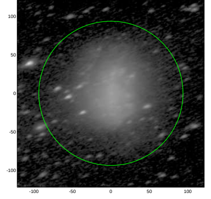
S4G: pa,inc= 22.1 62.9
