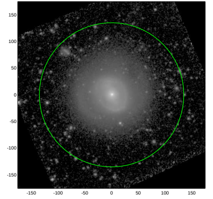
S4G: pa,inc= 25.9 17.6
