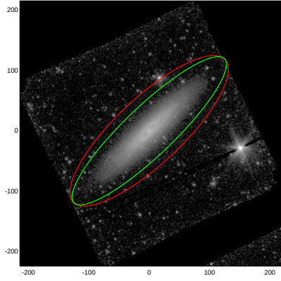
NGC4771
