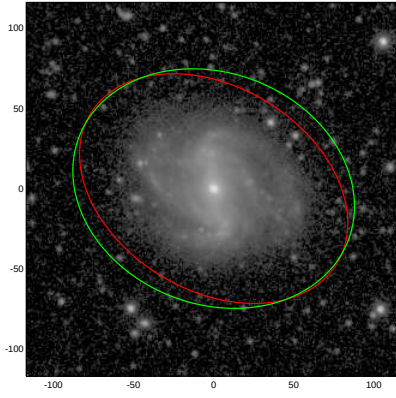
NGC4779
