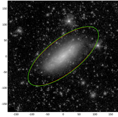
NGC4808
