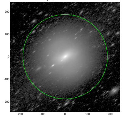
S4G: pa,inc= 38.2 68.7
