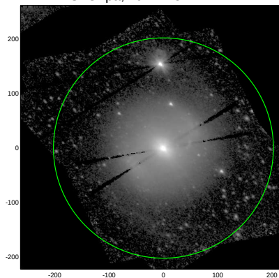
S4G: pa,inc= 143.7 41.4
