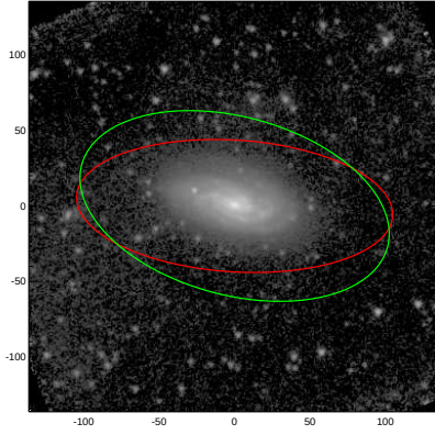
NGC4428
