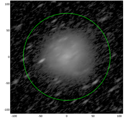
S4G: pa,inc= 35.4 71.2
