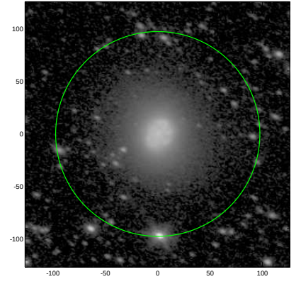
S4G: pa,inc= -19.5 45.4
