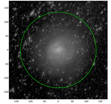
S4G: pa,inc= 61.8 47.8
