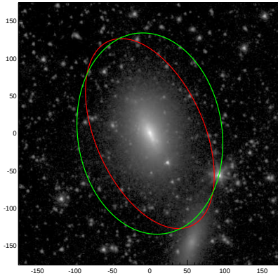
NGC4383
