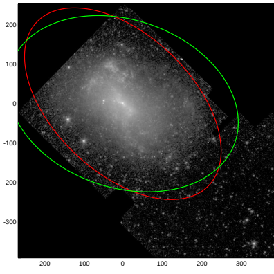
NGC4449
