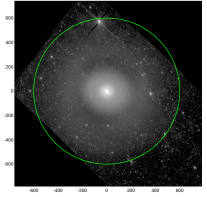
S4G: pa,inc= 123.5 34.0
