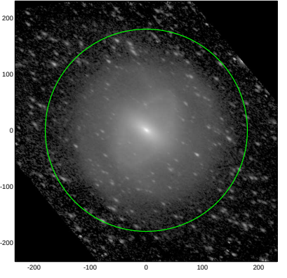
S4G: pa,inc= 146.2 58.5
