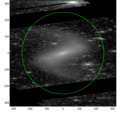
S4G: pa,inc= 0.2 73.5
