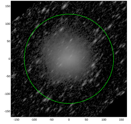
S4G: pa,inc= 48.6 69.1
