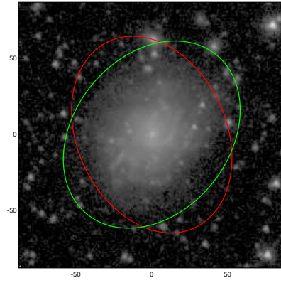
NGC4942
