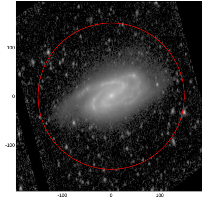
LEDA: pa,inc= 88.5 51.9
