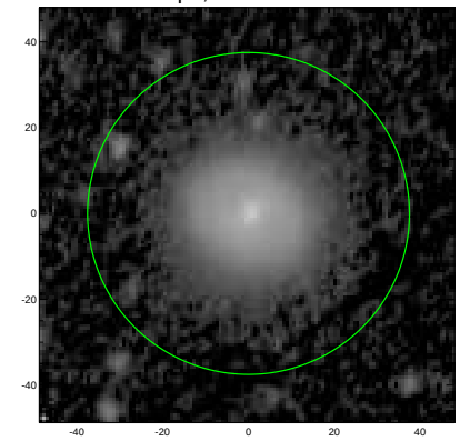
S4G: pa,inc= 66.3 45.1
