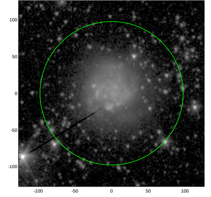
S4G: pa,inc= 87.8 19.6
