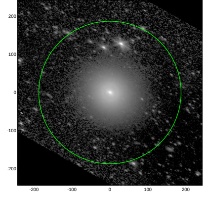
S4G: pa,inc= 149.7 55.7
