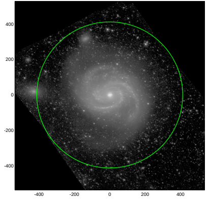
S4G: pa,inc= 158.2 34.6
