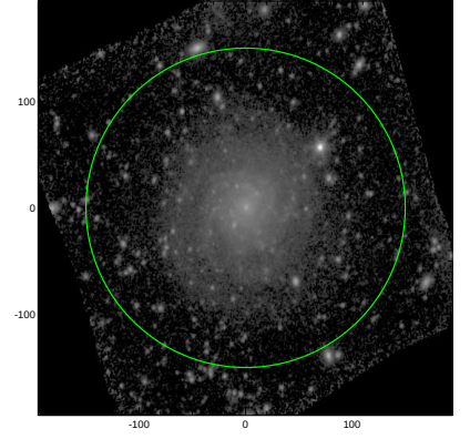
S4G: pa,inc= 77.0 33.9
