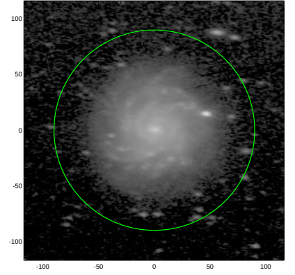
S4G: pa,inc= -3.9 58.7
