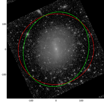
NGC4037
