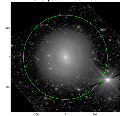
S4G: pa,inc= -6.5 45.9
