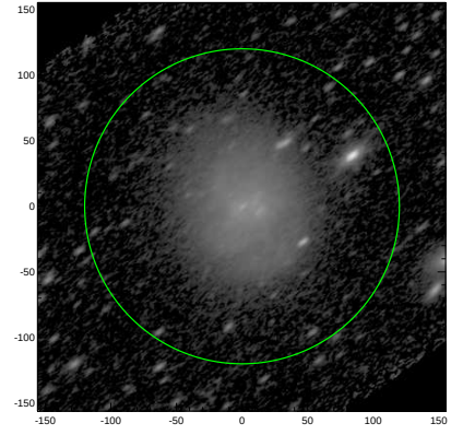
S4G: pa,inc= 39.1 62.5
