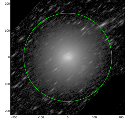
S4G: pa,inc= 39.5 74.1
