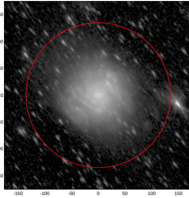
LEDA: pa,inc= 128.0 66.8
