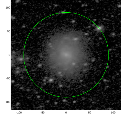
S4G: pa,inc= 16.2 45.7
