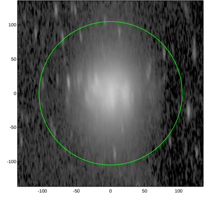
S4G: pa,inc= 92.5 77.9
