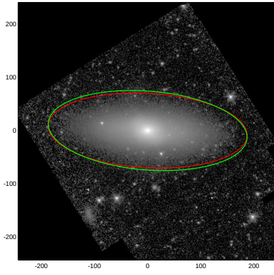
NGC4442
