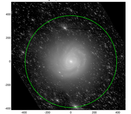
S4G: pa,inc= 142.6 59.6
