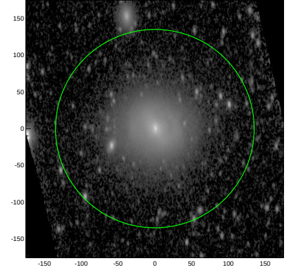
S4G: pa,inc= 93.0 57.0
