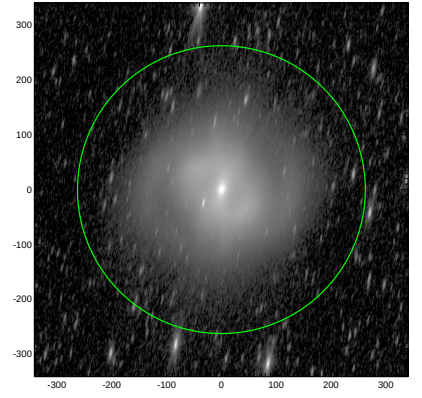
S4G: pa,inc= 79.7 75.1
