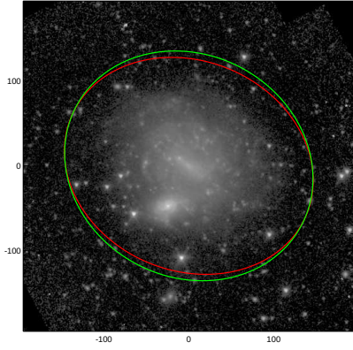
NGC4496A
