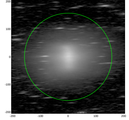
S4G: pa,inc= 2.6 81.3
