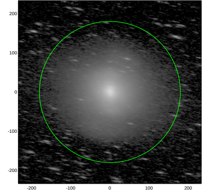
S4G: pa,inc= -9.8 74.5
