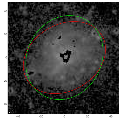
NGC4108B
