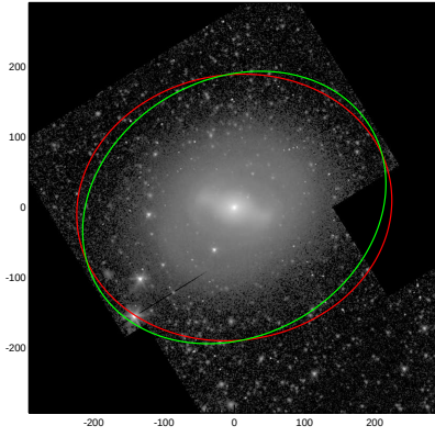
NGC4596
