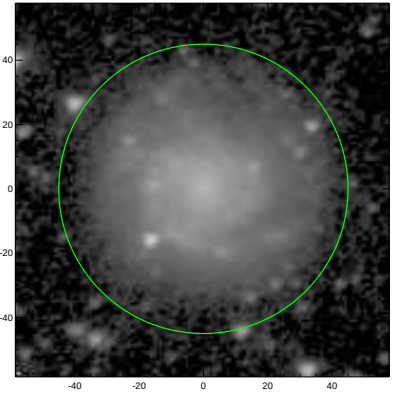
S4G: pa,inc= 23.1 32.2
