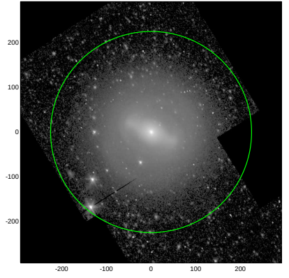
S4G: pa,inc= 119.2 35.5
