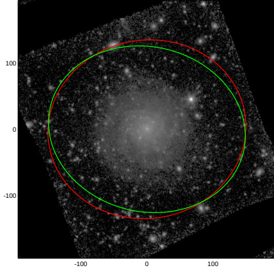
NGC4411B
