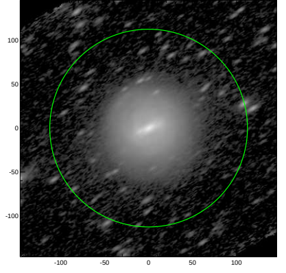
S4G: pa,inc= 32.9 67.9
