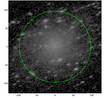
S4G: pa,inc= 20.2 58.0
