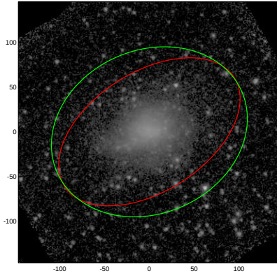
NGC4534
