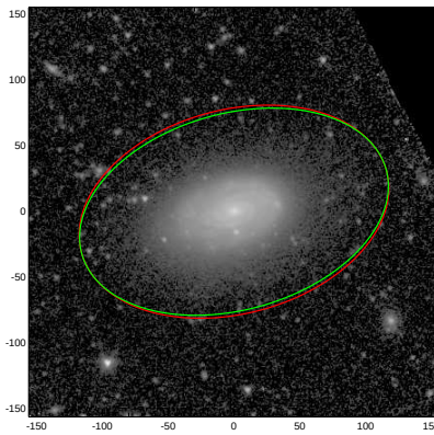
NGC4237
