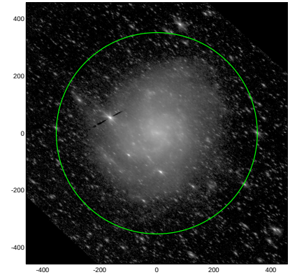
S4G: pa,inc= 143.2 63.0
