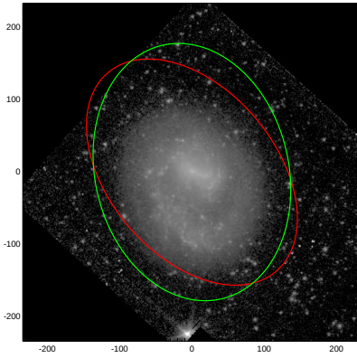
NGC4618
