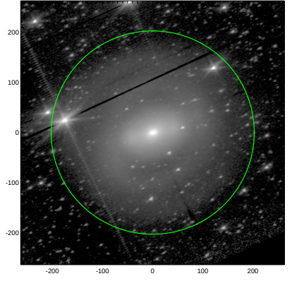
S4G: pa,inc= 24.6 53.9
