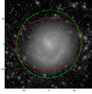
NGC4625
