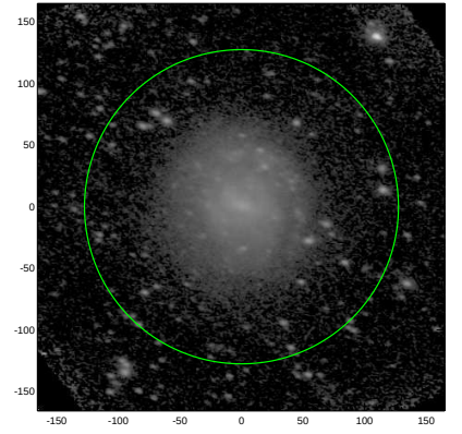
S4G: pa,inc= -13.2 48.1
