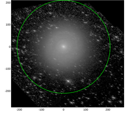
S4G: pa,inc= 157.2 56.6
