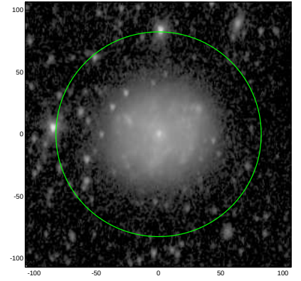
S4G: pa,inc= 86.2 43.3
