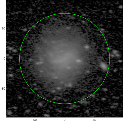
S4G: pa,inc= -3.8 55.1
