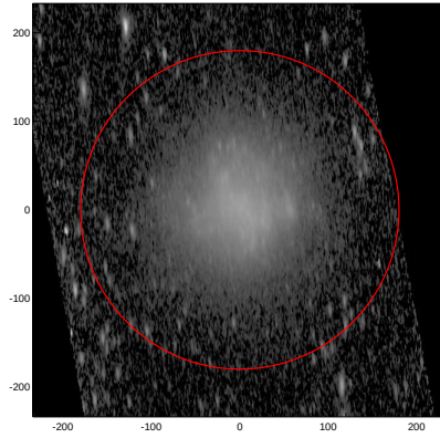
LEDA: pa,inc= 93.9 73.4
