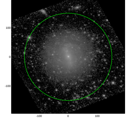
S4G: pa,inc= -18.2 31.3
