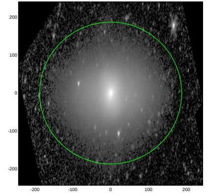
S4G: pa,inc= 85.5 66.7
