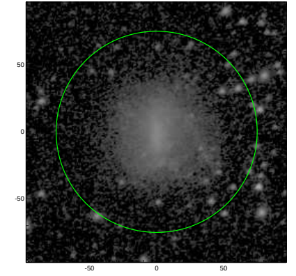
S4G: pa,inc= 26.3 35.2
