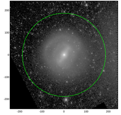
S4G: pa,inc= 109.8 30.4
