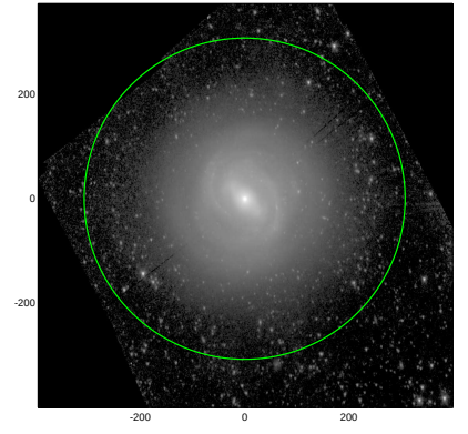
S4G: pa,inc= 92.1 41.6
