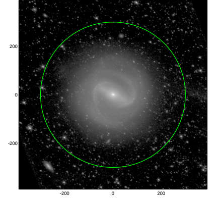
S4G: pa,inc= 149.2 39.0
