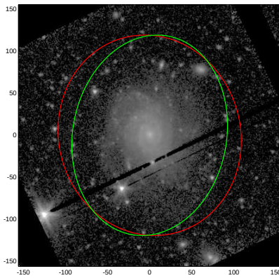
NGC4653
