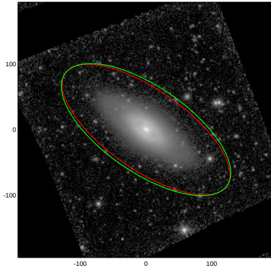
NGC4324
