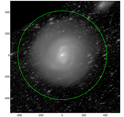
S4G: pa,inc= 24.8 66.0
