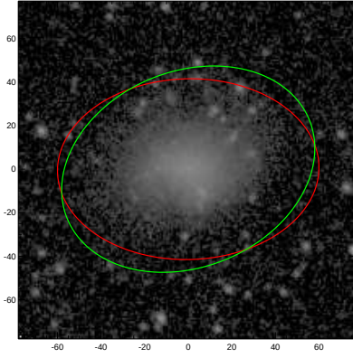
NGC4629
