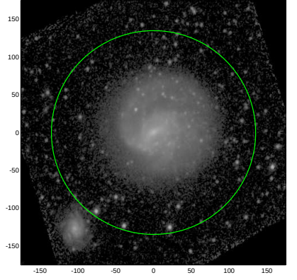
S4G: pa,inc= 74.1 31.7
