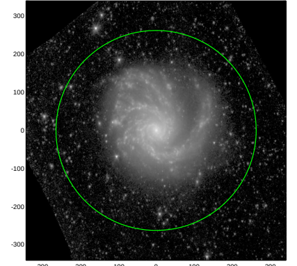
S4G: pa,inc= 85.1 35.6
