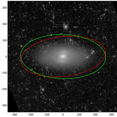
NGC4371
