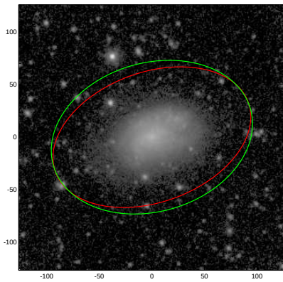
NGC4595
