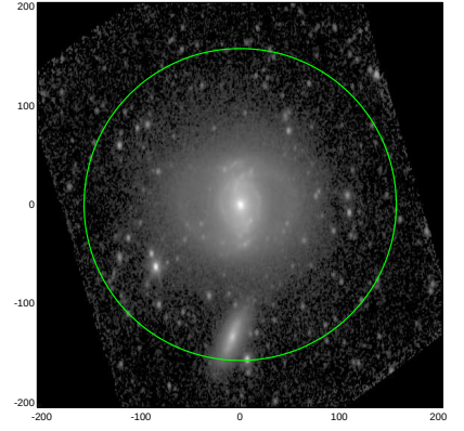
S4G: pa,inc= 87.9 48.4
