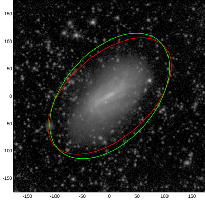
NGC4498
