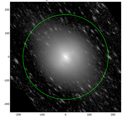
S4G: pa,inc= 131.8 71.3
