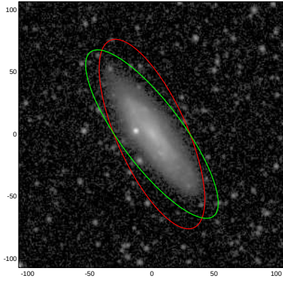
NGC4642
