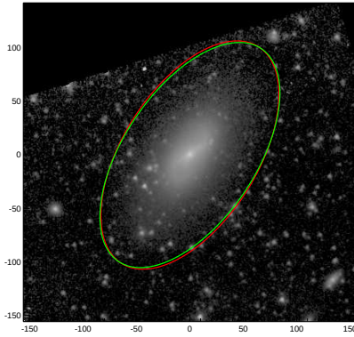
NGC4491
