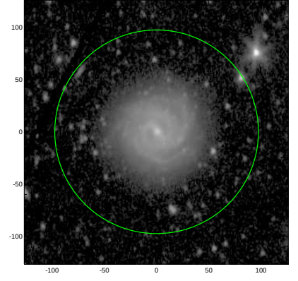
S4G: pa,inc= 93.1 41.9
