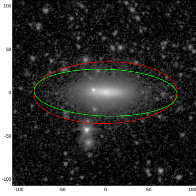
NGC4799
