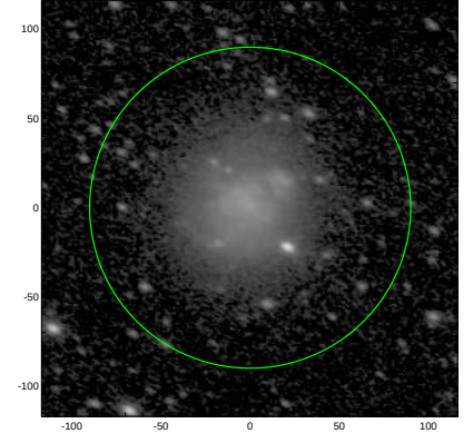
S4G: pa,inc= 157.7 48.0
