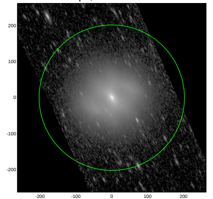
S4G: pa,inc= 115.7 69.8
