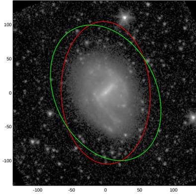
NGC4904
