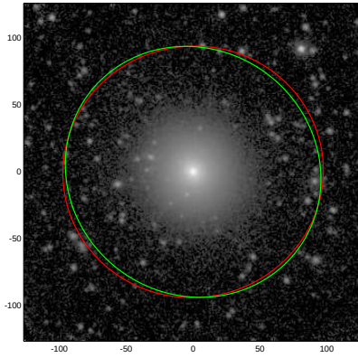
NGC4434
