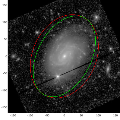
NGC4981
