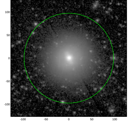
S4G: pa,inc= 158.1 24.5
