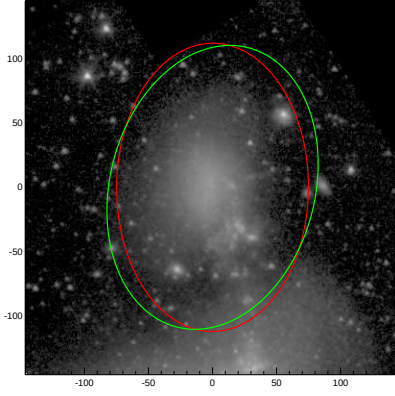
NGC4485
