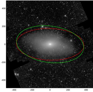
NGC4753
