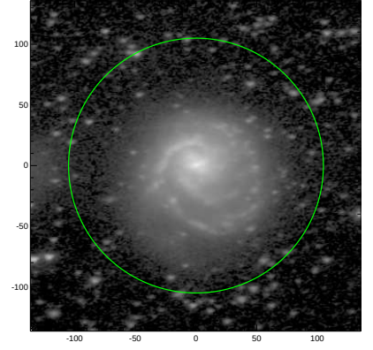
S4G: pa,inc= 7.1 52.3
