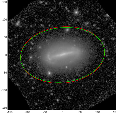
NGC4389
