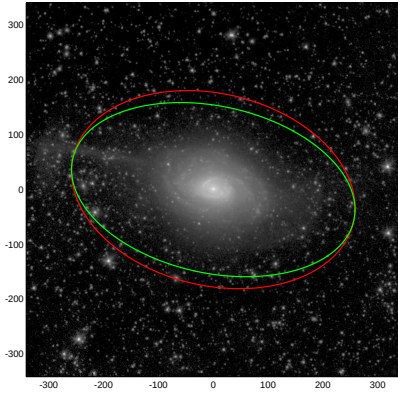
NGC4651
