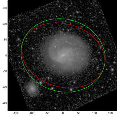
NGC4430
