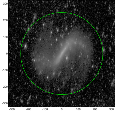
S4G: pa,inc= 82.2 61.3
