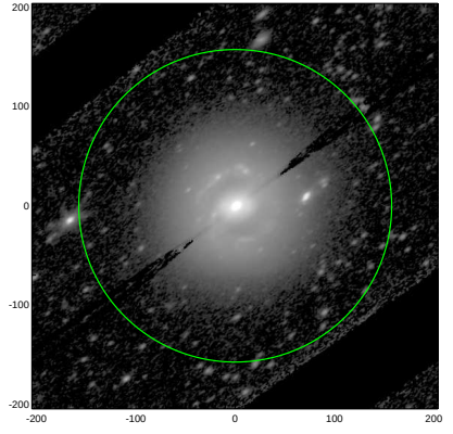
S4G: pa,inc= 39.7 56.6
