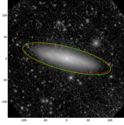
NGC4085
