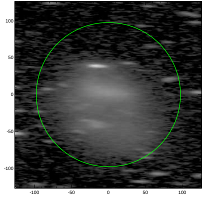
S4G: pa,inc= -2.0 78.2
