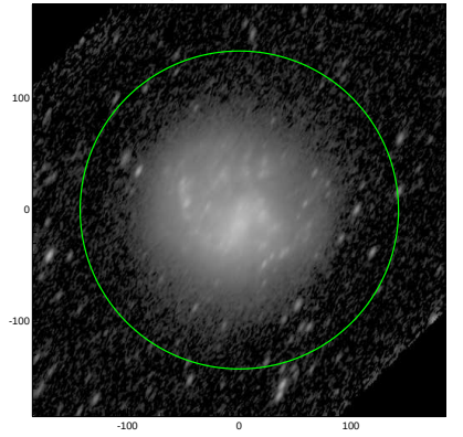
S4G: pa,inc= 60.5 65.9
