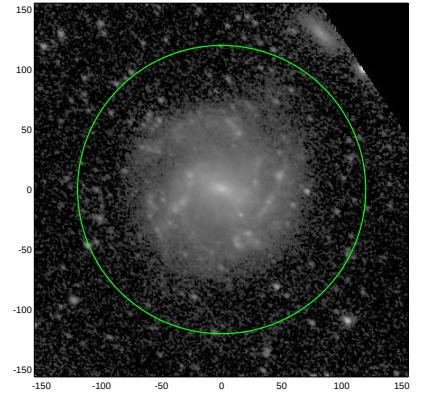
S4G: pa,inc= 146.8 38.9
