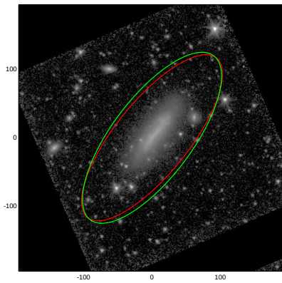
NGC4948
