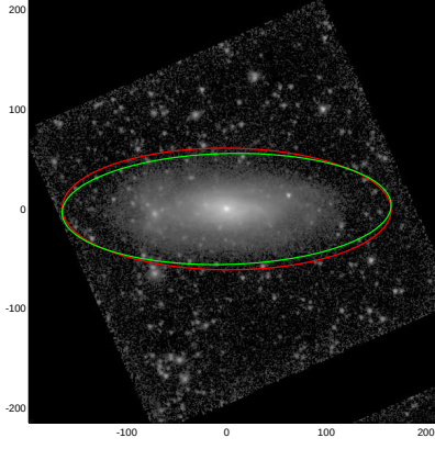
NGC4951
