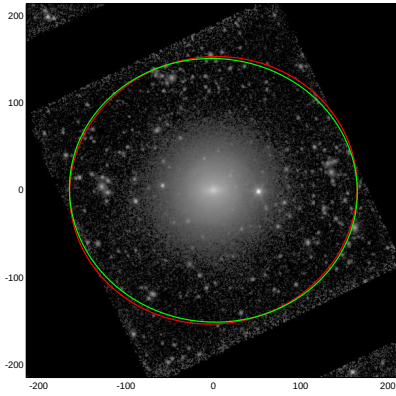
NGC4733
