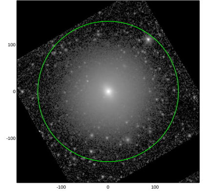
S4G: pa,inc= 118.5 11.9
