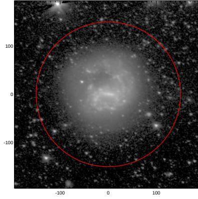
LEDA: pa,inc= 162.7 37.8
