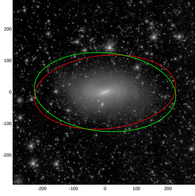
NGC4424
