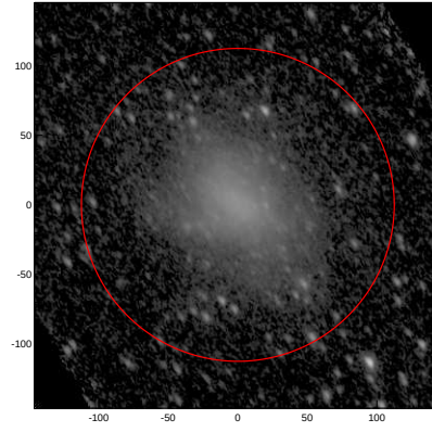
LEDA: pa,inc= 122.8 53.7
