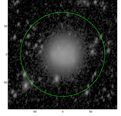
S4G: pa,inc= 68.6 51.1
