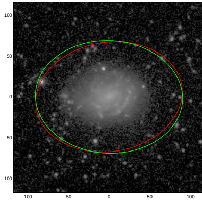
NGC4390
