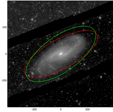
NGC4536
