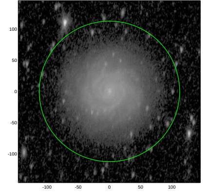
S4G: pa,inc= 83.6 60.4
