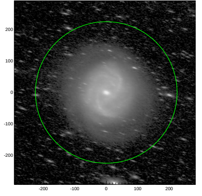
S4G: pa,inc= -15.7 70.8
