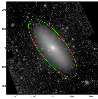
NGC4856
