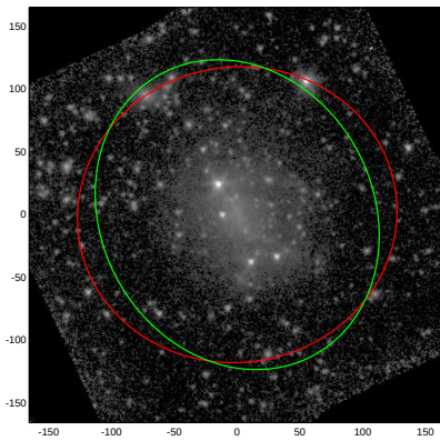
NGC4523
