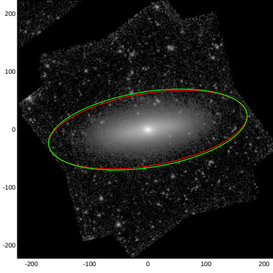
NGC4346
