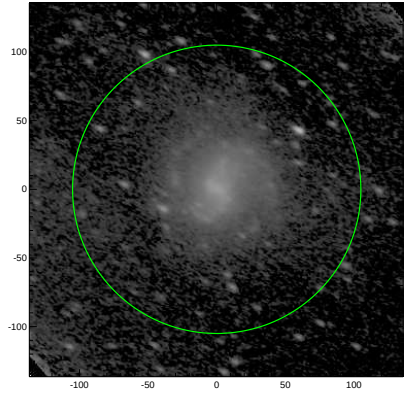
S4G: pa,inc= 152.6 57.4
