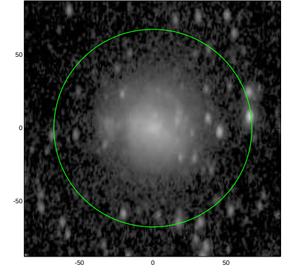
S4G: pa,inc= 87.1 53.9
