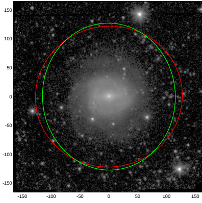
NGC5957
