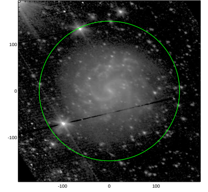
S4G: pa,inc= 156.9 43.6
