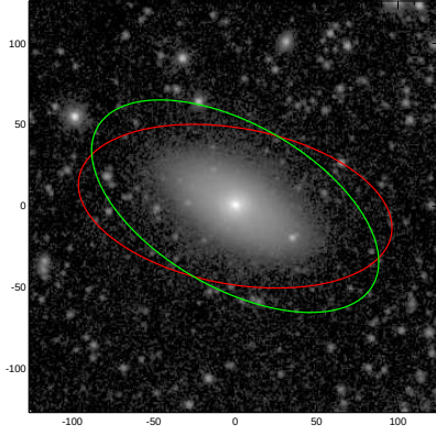
NGC5507
