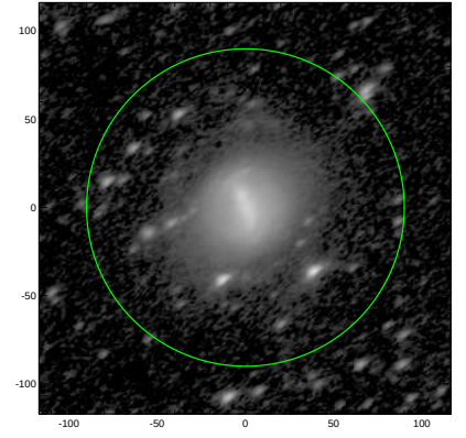
S4G: pa,inc= 35.0 59.2
