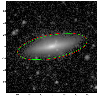
NGC5014
