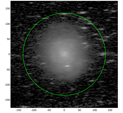
S4G: pa,inc= 1.9 74.7
