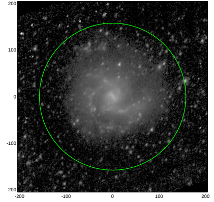
S4G: pa,inc= 60.7 42.2
