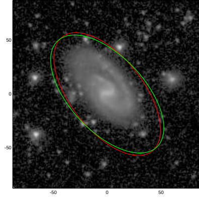
NGC5950
