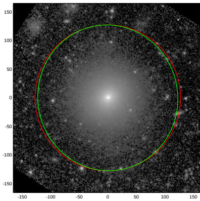
NGC5631
