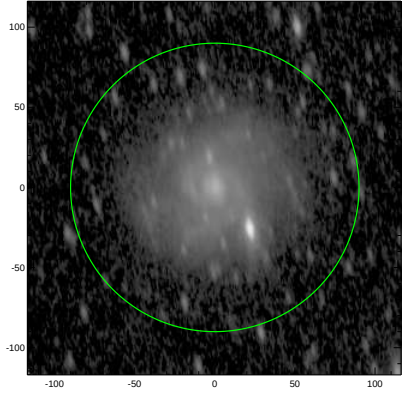
S4G: pa,inc= 98.9 66.7
