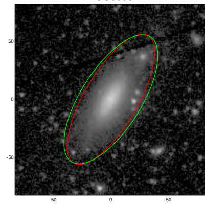
NGC5809
