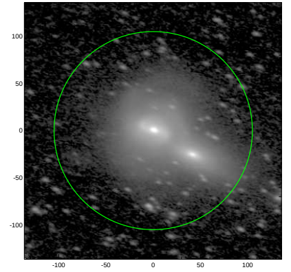
S4G: pa,inc= -17.9 57.9
