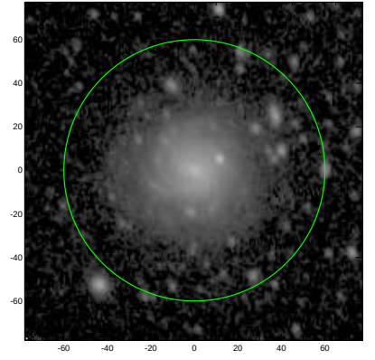
S4G: pa,inc= 101.4 36.3
