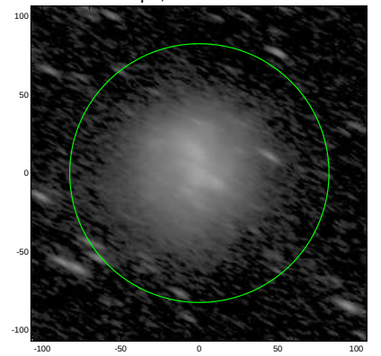
S4G: pa,inc= 151.9 71.3
