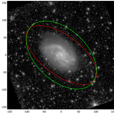
NGC5595
