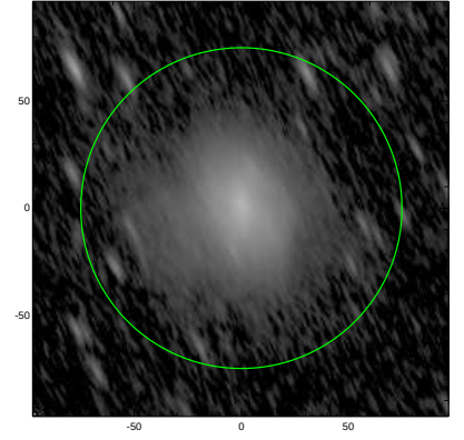
S4G: pa,inc= 114.2 74.4
