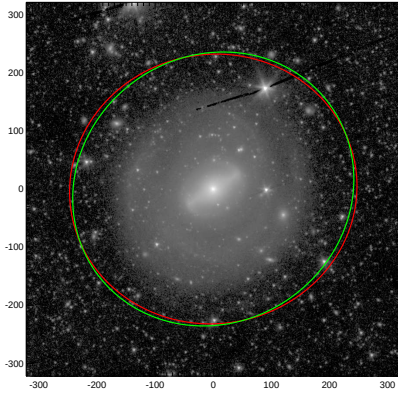
NGC5101
