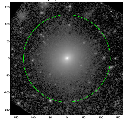
S4G: pa,inc= 10.2 16.0
