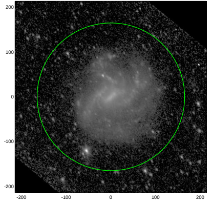
S4G: pa,inc= 119.7 48.3
