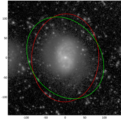
NGC5480
