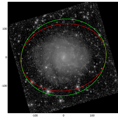
NGC5892
