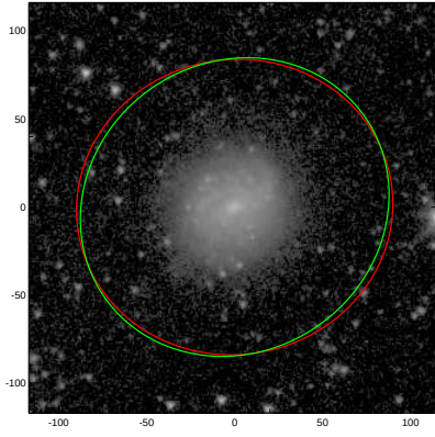
NGC5476
