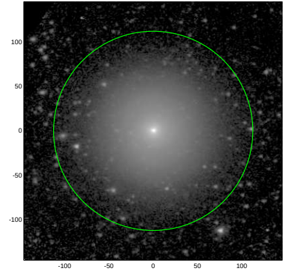
S4G: pa,inc= 5.5 30.8
