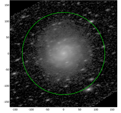
S4G: pa,inc= 17.5 61.2
