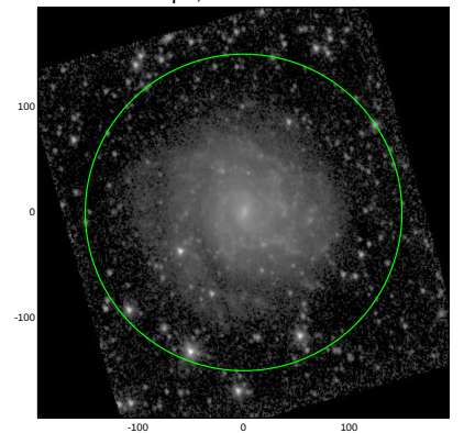
S4G: pa,inc= 107.0 27.3
