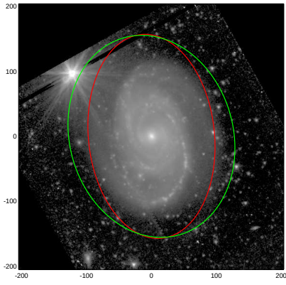
NGC5371
