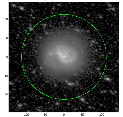
S4G: pa,inc= 154.7 51.7
