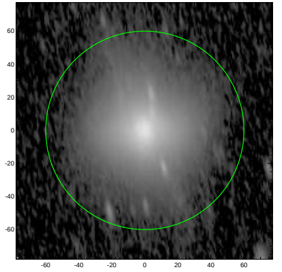
S4G: pa,inc= 101.0 71.4
