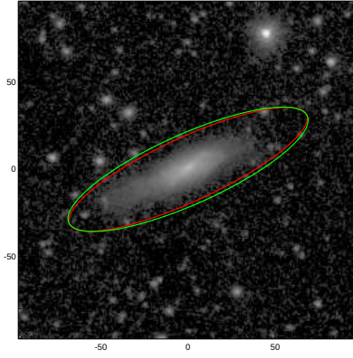
NGC5731
