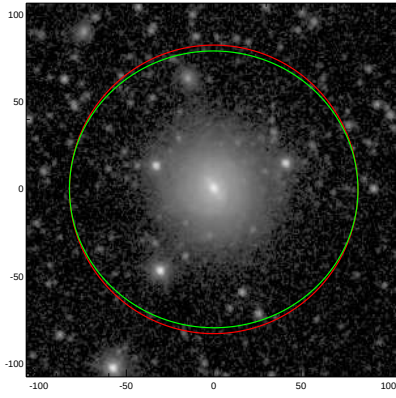
NGC5956
