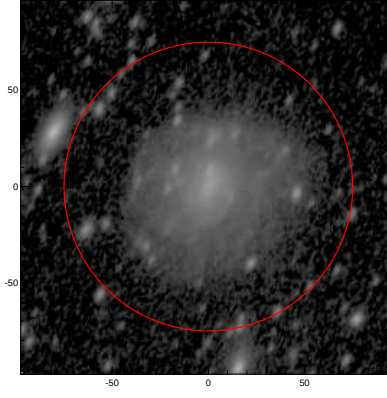
LEDA: pa,inc= 65.9 52.7
