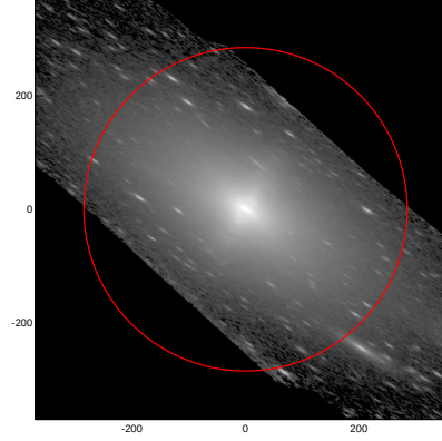
LEDA: pa,inc= 146.8 76.1
