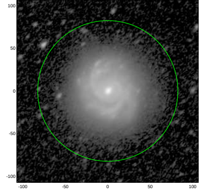
S4G: pa,inc= 46.2 54.7
