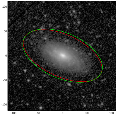
NGC5520
