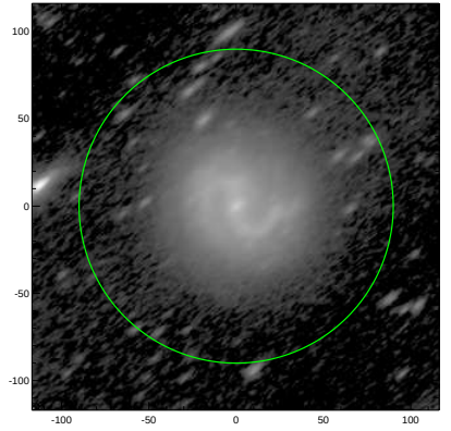
S4G: pa,inc= 38.9 66.4
