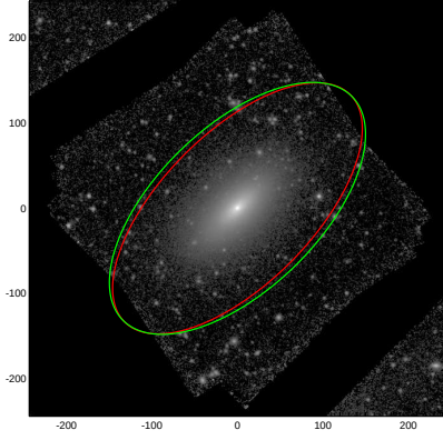
NGC5326
