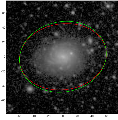
NGC5336
