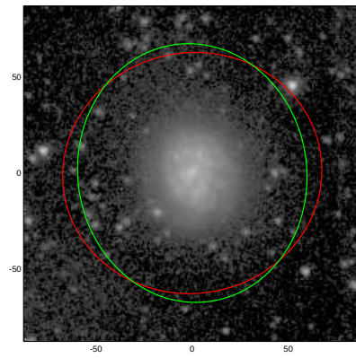
NGC5958
