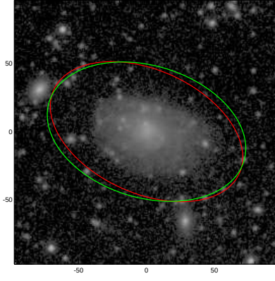
NGC5486
