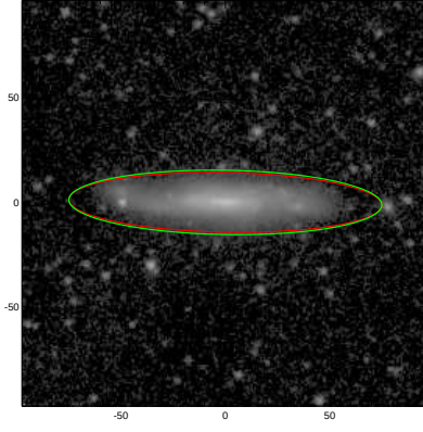
NGC5730
