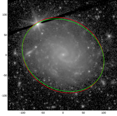
NGC5885
