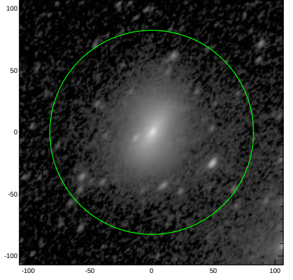
S4G: pa,inc= 50.4 56.7
