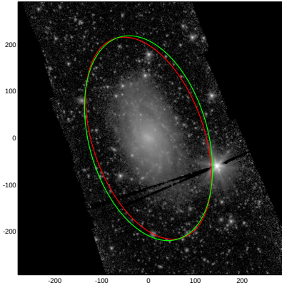
NGC5042
