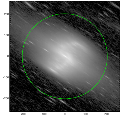
S4G: pa,inc= 146.3 81.8
