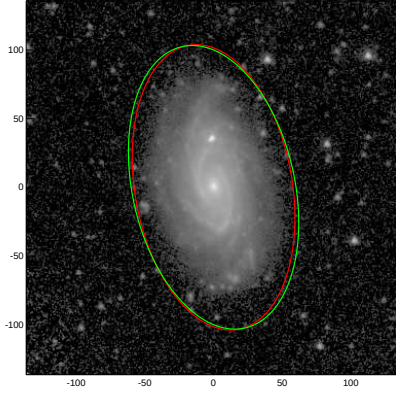
NGC5012
