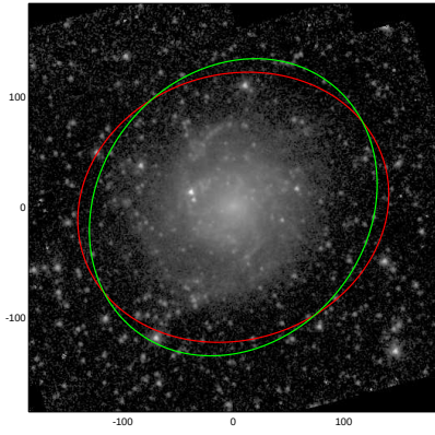
NGC5668
