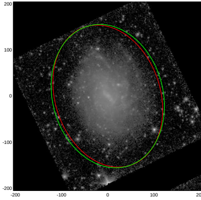
NGC5334
