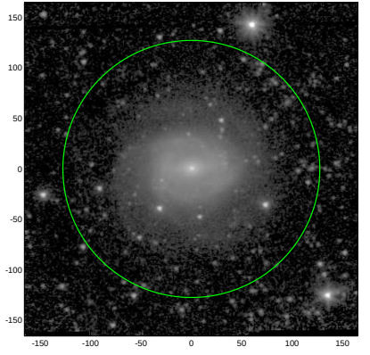
S4G: pa,inc= 2.8 25.4
