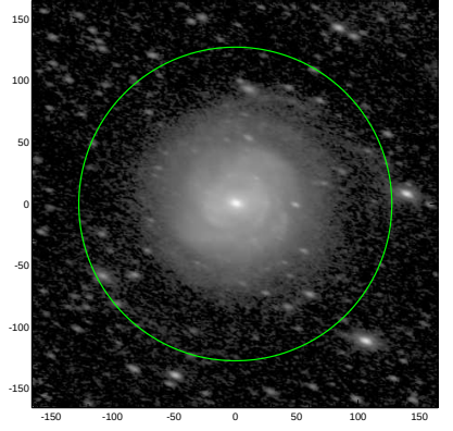
S4G: pa,inc= -17.8 58.1
