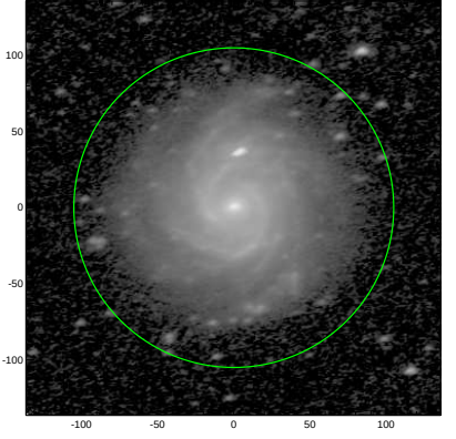
S4G: pa,inc= 12.5 55.8
