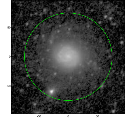
S4G: pa,inc= 46.6 36.7
