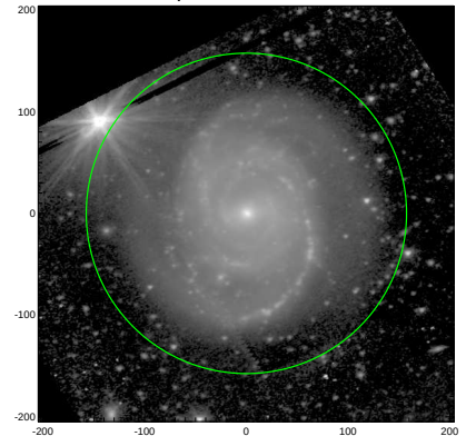
S4G: pa,inc= 15.7 36.8
