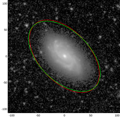
NGC5313
