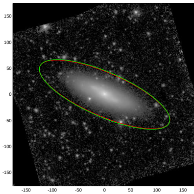
NGC5864
