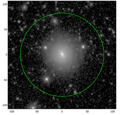
S4G: pa,inc= 88.2 16.4
