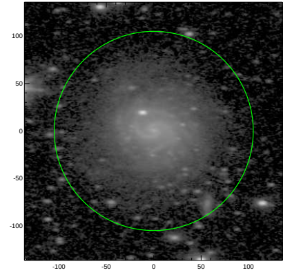
S4G: pa,inc= -2.2 56.1
