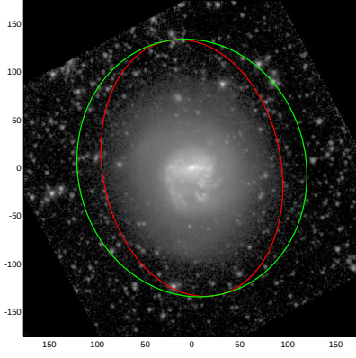
NGC5713
