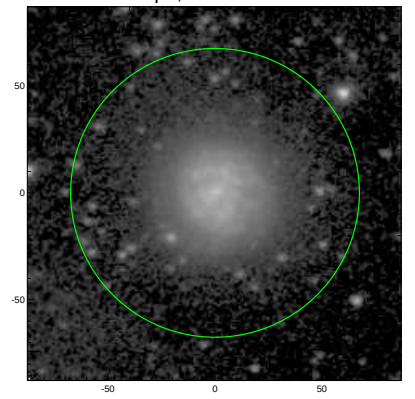
S4G: pa,inc= 7.2 28.1
