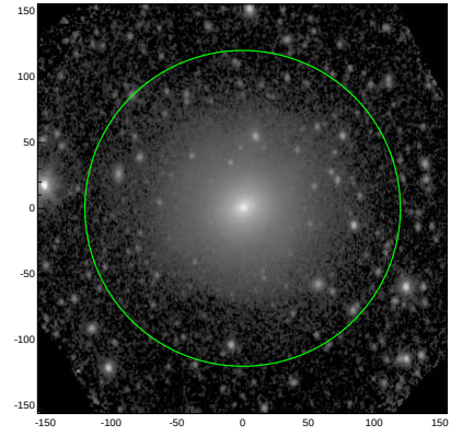
S4G: pa,inc= 90.6 35.5
