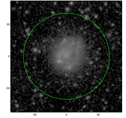
S4G: pa,inc= 63.0 14.7
