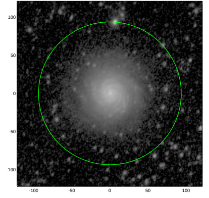
S4G: pa,inc= 63.1 41.5
