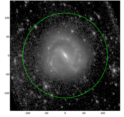
S4G: pa,inc= 112.4 41.1
