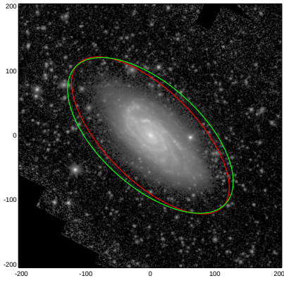
NGC5676
