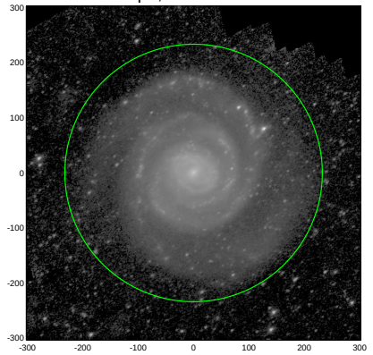
S4G: pa,inc= 35.6 47.8
