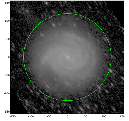
S4G: pa,inc= 130.9 64.6
