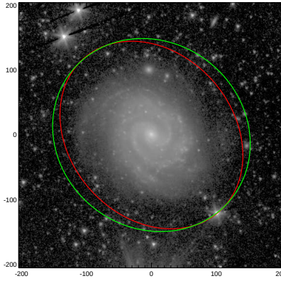
NGC5085
