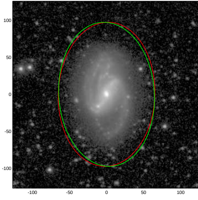
NGC5430
