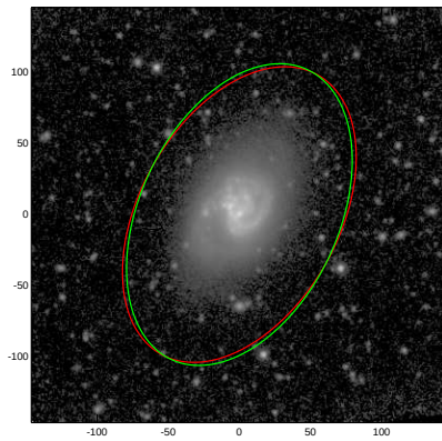
NGC5665
