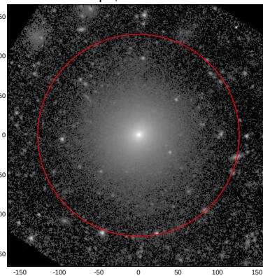
LEDA: pa,inc= 999.0 0.0
