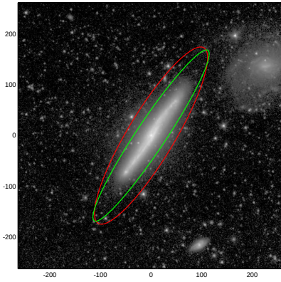
NGC5775
