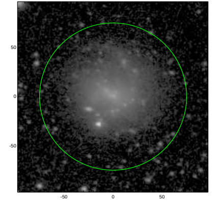
S4G: pa,inc= -4.3 22.6
