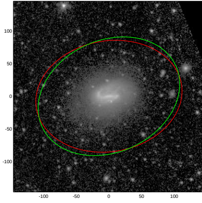
NGC5691
