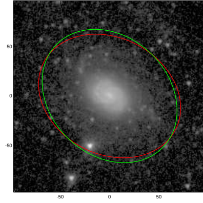
NGC5963
