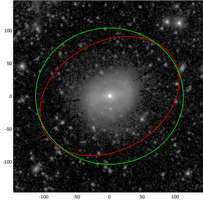
NGC5347
