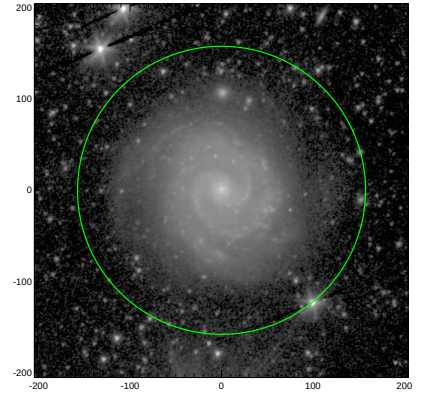
S4G: pa,inc= 52.1 24.6
