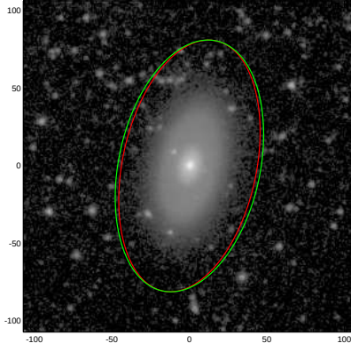
NGC5602
