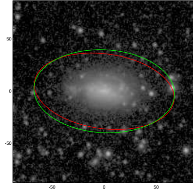
NGC5464
