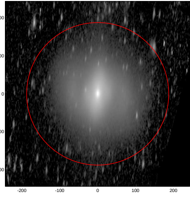
LEDA: pa,inc= 86.0 75.7
