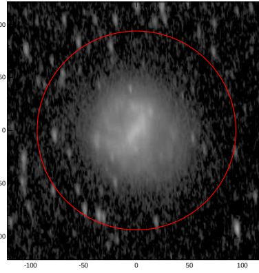
LEDA: pa,inc= 95.3 69.3
