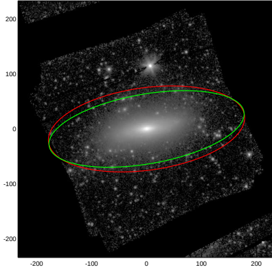
NGC5719
