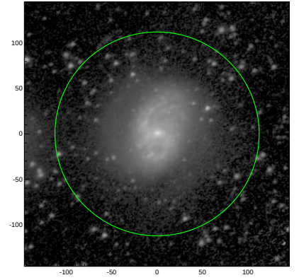
S4G: pa,inc= 37.2 37.5
