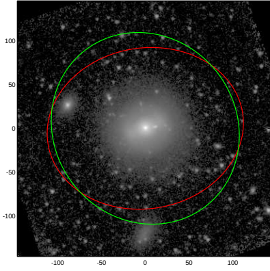
NGC5770
