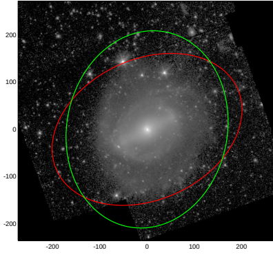
NGC5850
