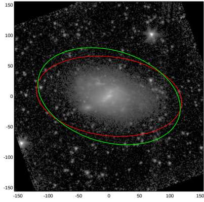
NGC5645
