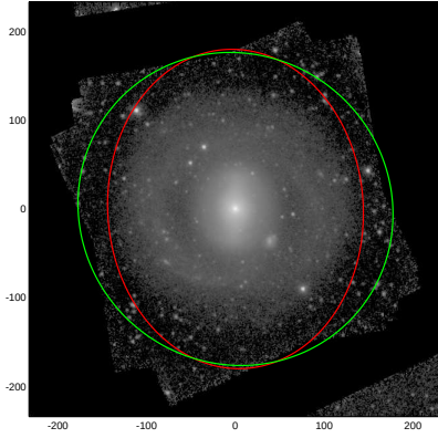
NGC5701
