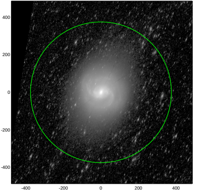
S4G: pa,inc= 67.0 66.7
