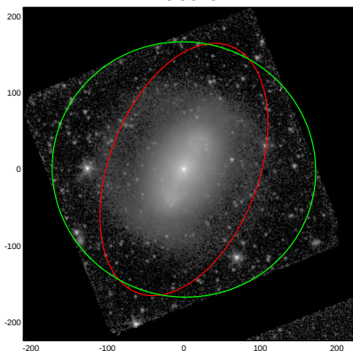
NGC5134
