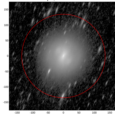
LEDA: pa,inc= 66.5 72.1
