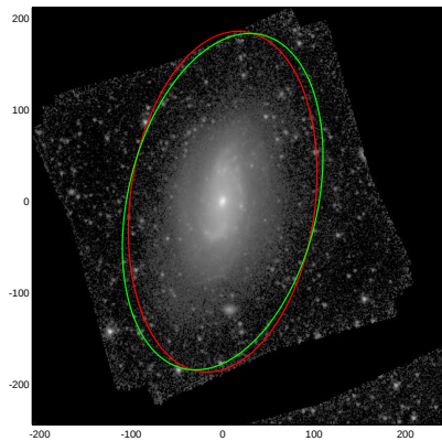
NGC5806
