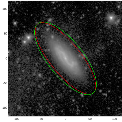
NGC5116
