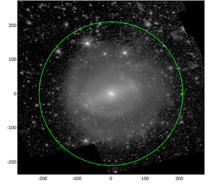
S4G: pa,inc= -10.6 36.0
