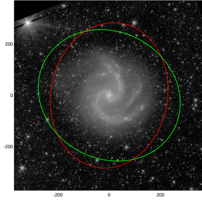
NGC5247
