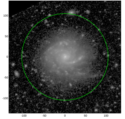
S4G: pa,inc= 7.9 23.3
