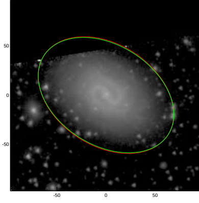
NGC5240
