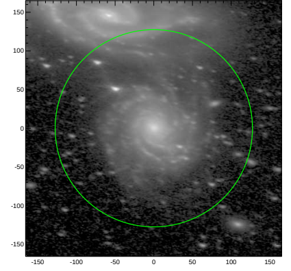
S4G: pa,inc= -10.2 59.9
