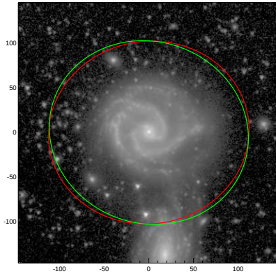
NGC5427
