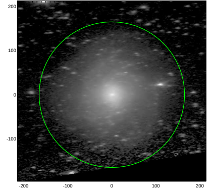
S4G: pa,inc= 3.9 67.4
