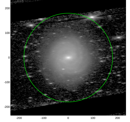
S4G: pa,inc= 3.3 68.1
