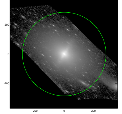
S4G: pa,inc= 146.7 70.3
