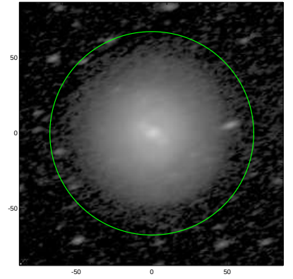
S4G: pa,inc= 21.9 62.2
