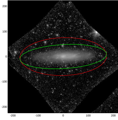
NGC5523
