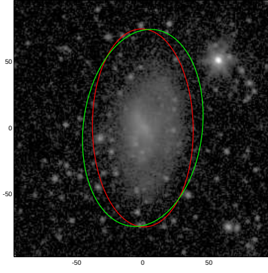
NGC5002
