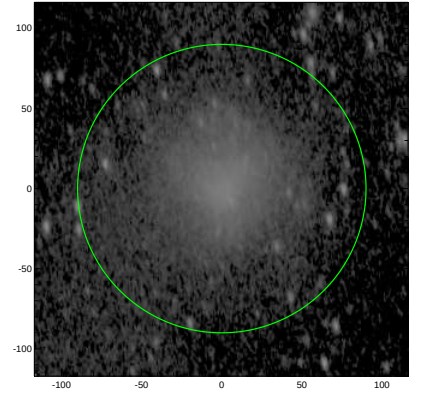
S4G: pa,inc= 96.9 58.8
