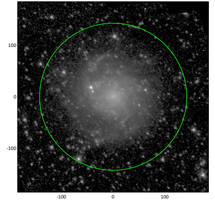
S4G: pa,inc= 140.8 31.6
