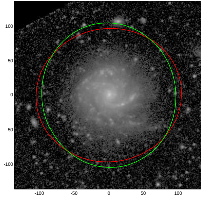
NGC5660
