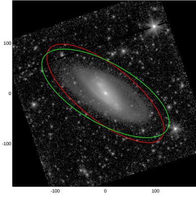
NGC5756
