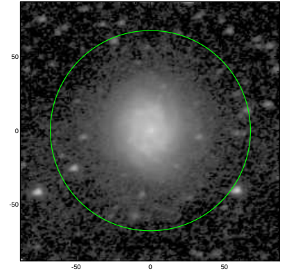
S4G: pa,inc= 18.4 40.7
