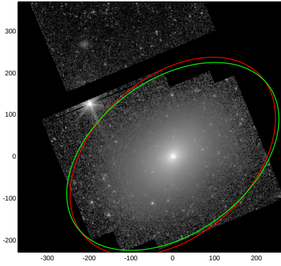
NGC5363
