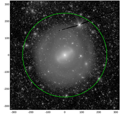
S4G: pa,inc= 124.9 22.0
