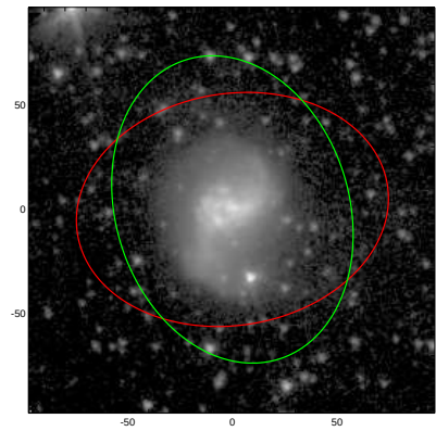
NGC5915
