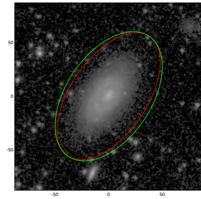
NGC5821
