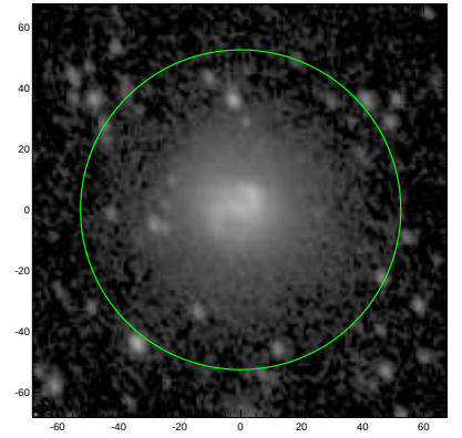
S4G: pa,inc= 113.7 41.3
