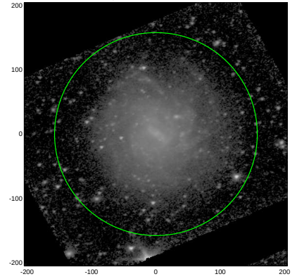
S4G: pa,inc= 15.1 40.5
