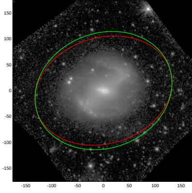
NGC5383
