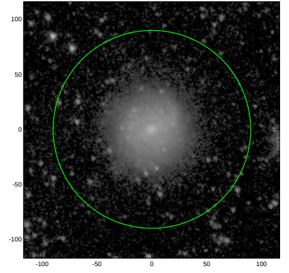
S4G: pa,inc= 124.1 23.7
