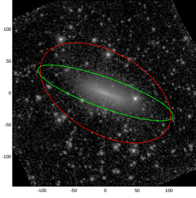
NGC5360
