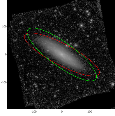
NGC5577
