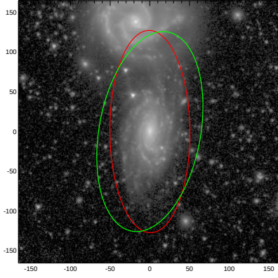
NGC5426
