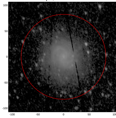
LEDA: pa,inc= 107.7 50.4
