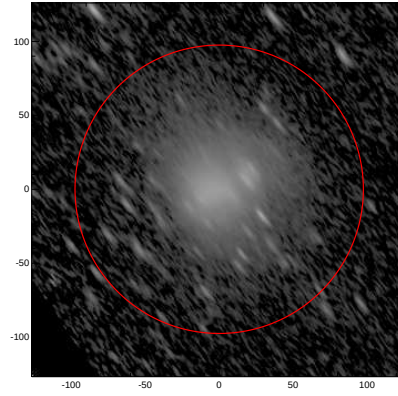
LEDA: pa,inc= 128.0 72.8
