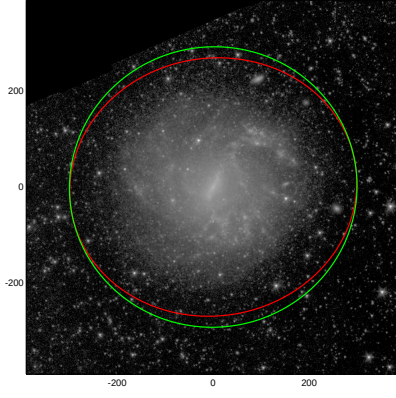
NGC5068
