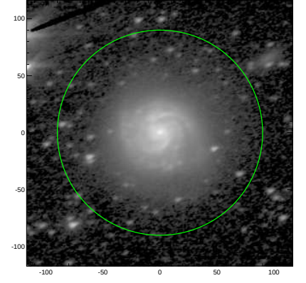
S4G: pa,inc= 19.4 52.7
