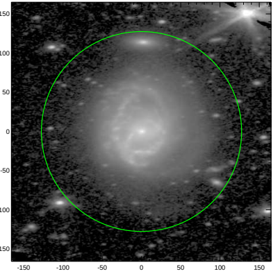
S4G: pa,inc= 2.5 56.9
