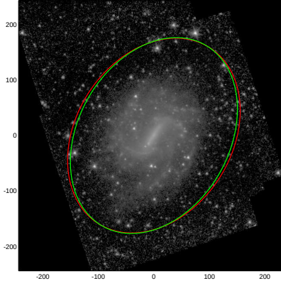
NGC5964
