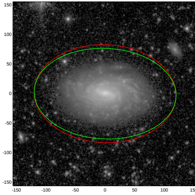
NGC5970
