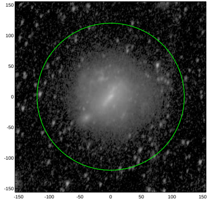
S4G: pa,inc= 73.8 51.2
