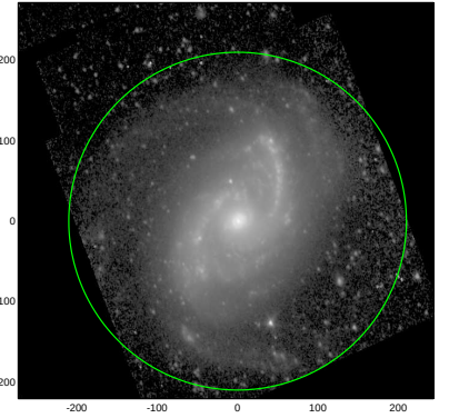
S4G: pa,inc= 103.9 38.6
