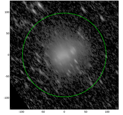
S4G: pa,inc= 128.7 69.4
