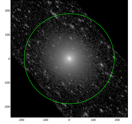
S4G: pa,inc= 134.3 59.4
