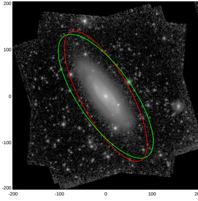
NGC5443
