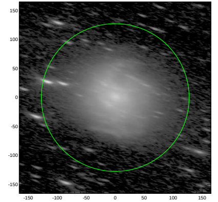
S4G: pa,inc= -15.7 75.2
