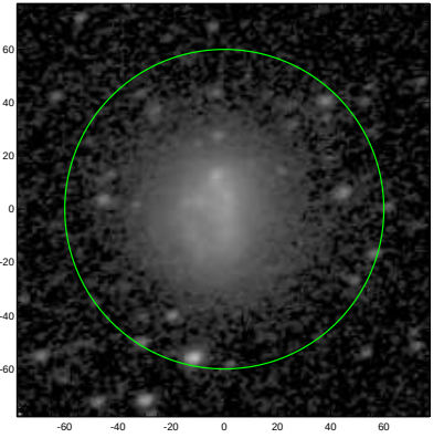
S4G: pa,inc= 17.6 39.8
