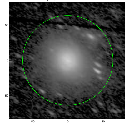
S4G: pa,inc= 147.7 65.9
