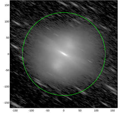
S4G: pa,inc= 149.8 79.3
