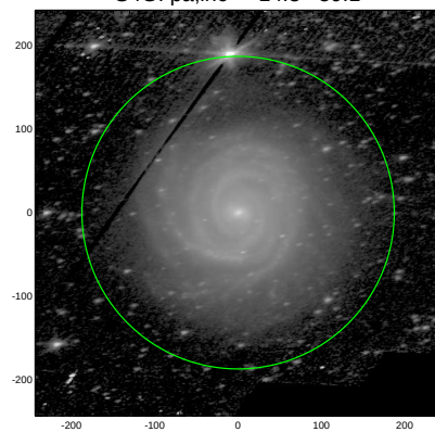
S4G: pa,inc= 14.8 59.1
