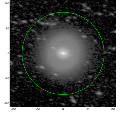
S4G: pa,inc= -12.2 56.4
