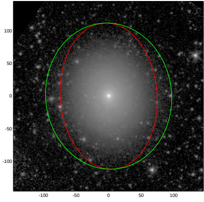
NGC5273
