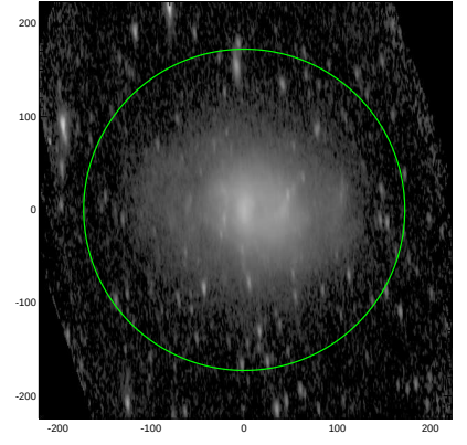
S4G: pa,inc= 93.3 73.9
