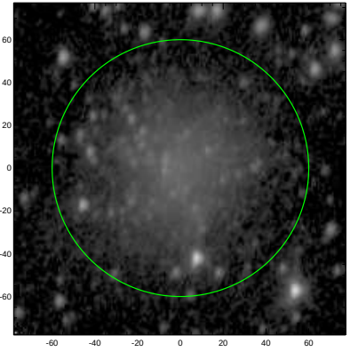
S4G: pa,inc= 81.2 44.1
