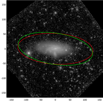
NGC5362
