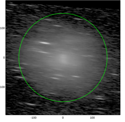
S4G: pa,inc= -7.7 82.0
