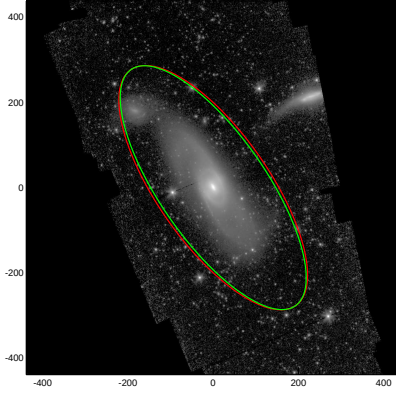
NGC5566
