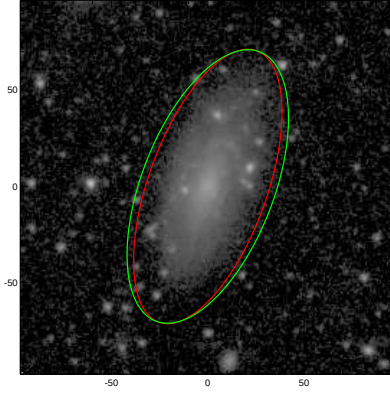
NGC5346
