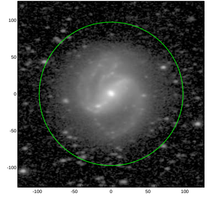
S4G: pa,inc= 3.8 48.6
