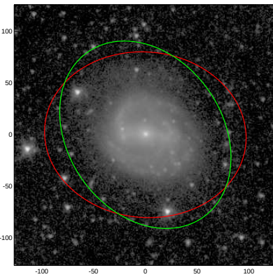
NGC5339
