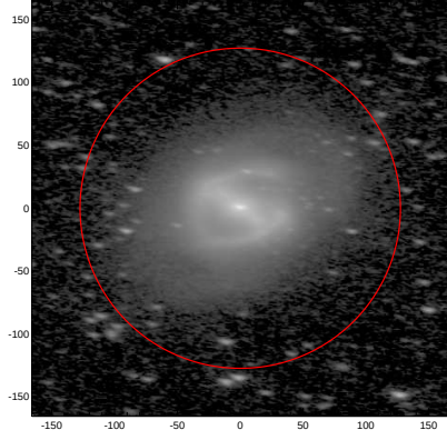
LEDA: pa,inc= 173.5 66.1
