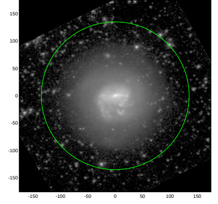
S4G: pa,inc= 13.8 28.3
