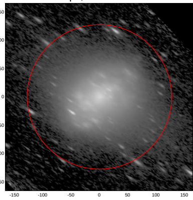
LEDA: pa,inc= 145.8 72.0
