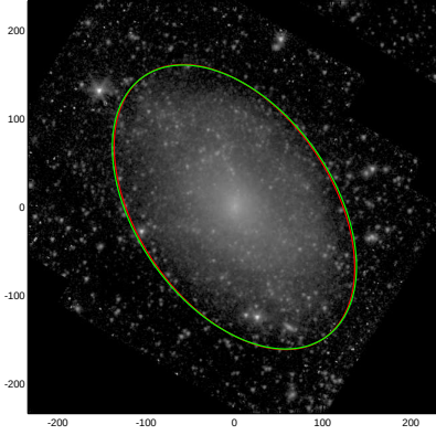
NGC5585
