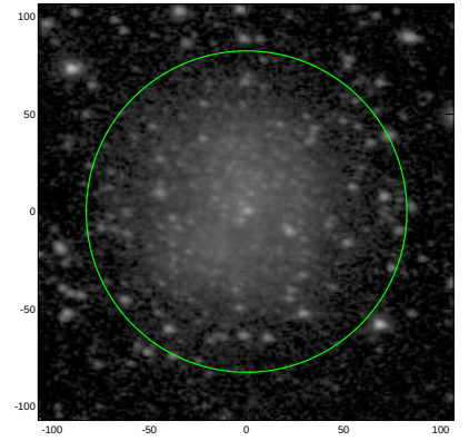
S4G: pa,inc= -6.7 41.0
