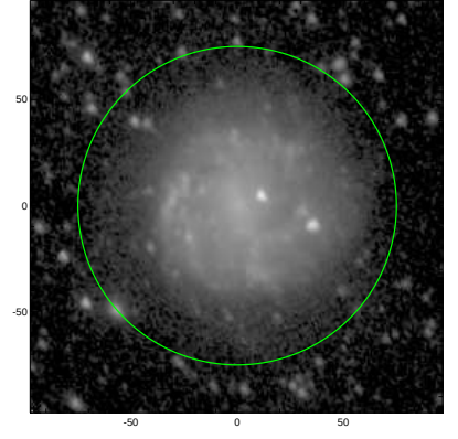
S4G: pa,inc= 119.8 35.2
