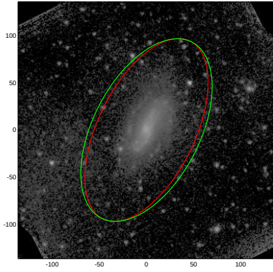
NGC5117
