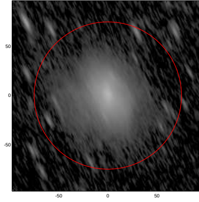
LEDA: pa,inc= 114.8 75.9
