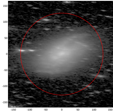
LEDA: pa,inc= 175.1 75.4
