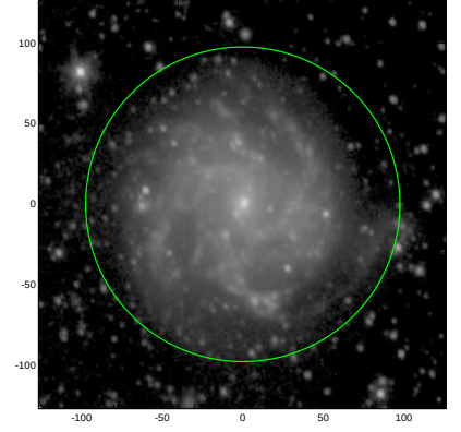
S4G: pa,inc= 100.3 27.6
