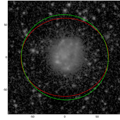
NGC5789
