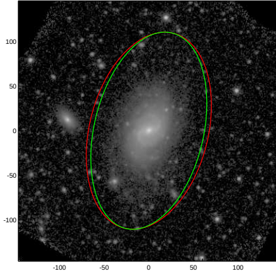
NGC5205
