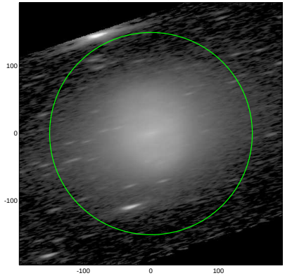
S4G: pa,inc= 15.4 79.3
