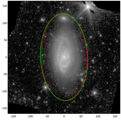
NGC5678
