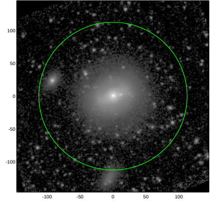
S4G: pa,inc= 38.4 22.4
