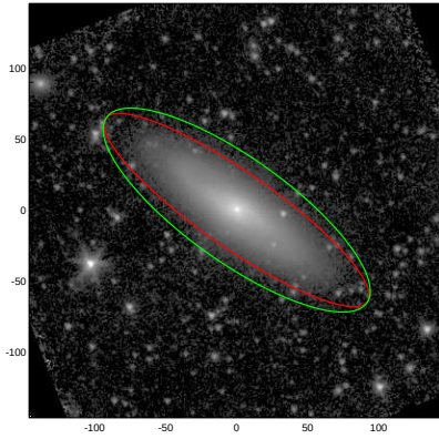
NGC5854
