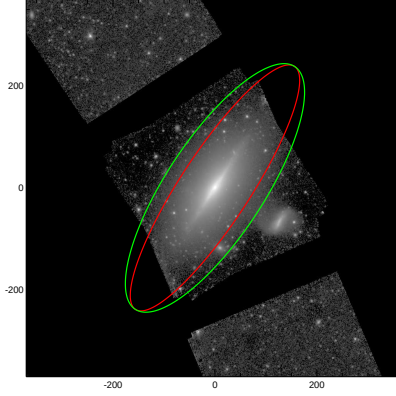
NGC5078
