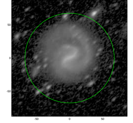
S4G: pa,inc= 42.8 58.9
