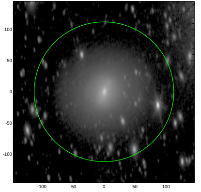
S4G: pa,inc= 93.5 61.1
