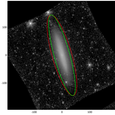
NGC5356
