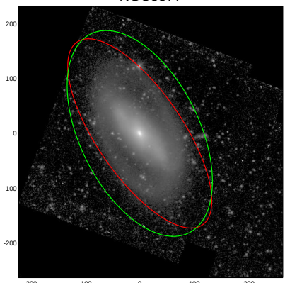
NGC5377
