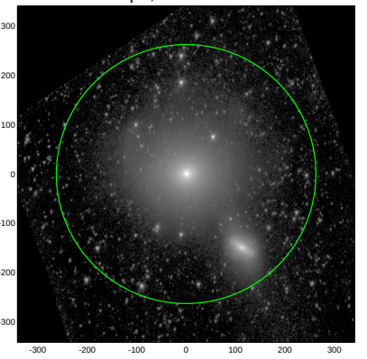
S4G: pa,inc= 83.0 39.6
