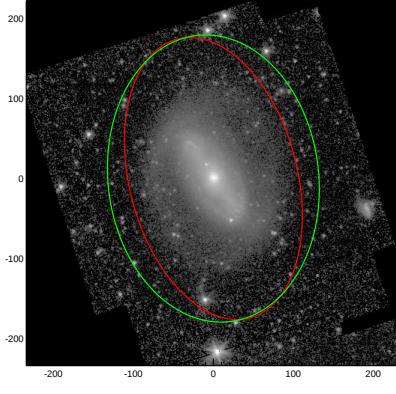
NGC5728
