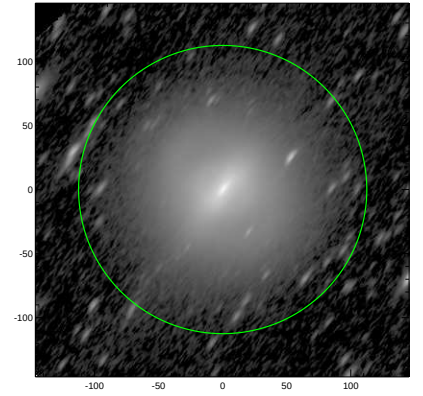
S4G: pa,inc= 54.5 71.1
