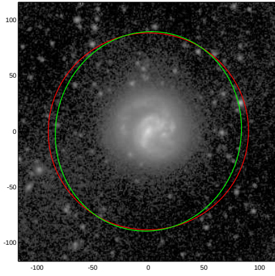
NGC5600
