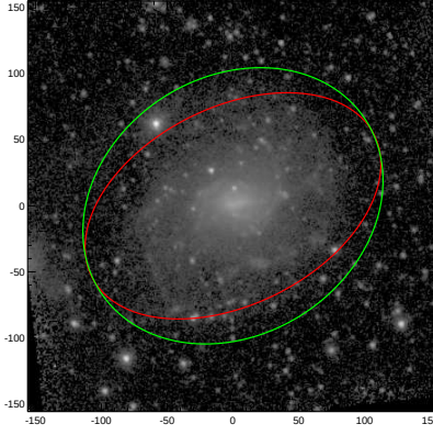
NGC5774
