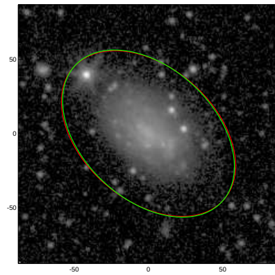
NGC5798
