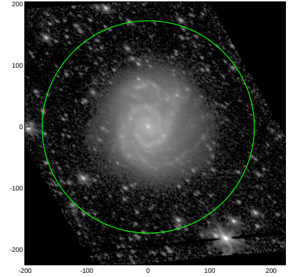
S4G: pa,inc= 145.3 51.2
