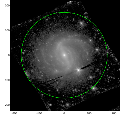
S4G: pa,inc= 144.6 33.5
