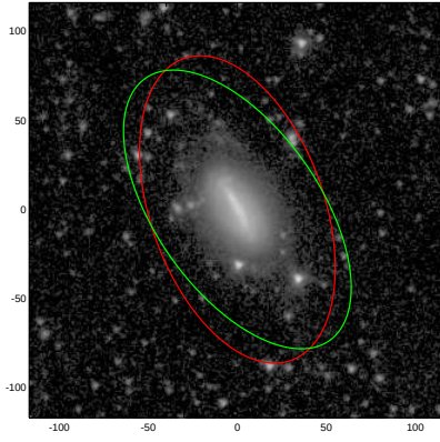
NGC5781
