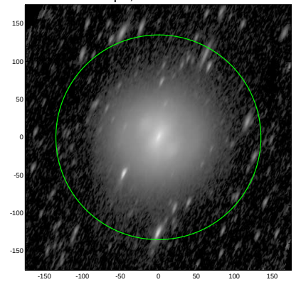
S4G: pa,inc= 66.3 71.6
