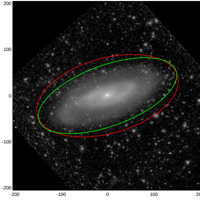
NGC5448
