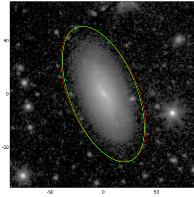
NGC5337
