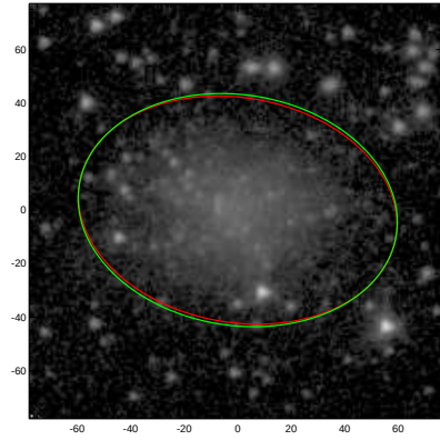
NGC5477
