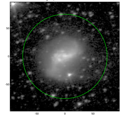
S4G: pa,inc= 17.0 41.9
