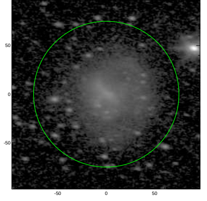
S4G: pa,inc= -7.0 53.1
