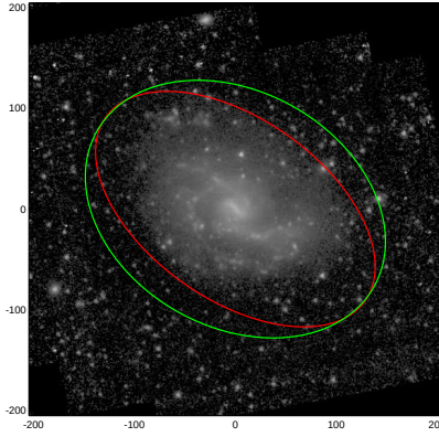
NGC5669
