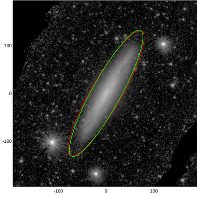
NGC5301
