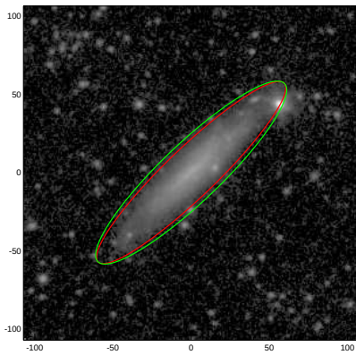
NGC5673
