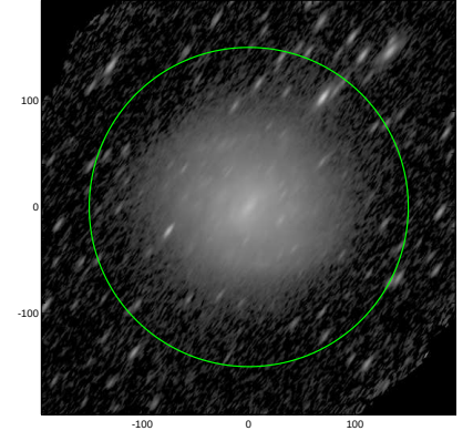
S4G: pa,inc= 54.2 73.3
