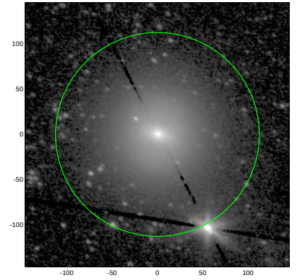
S4G: pa,inc= 151.8 39.0
