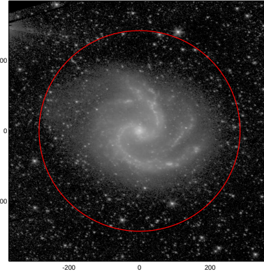
LEDA: pa,inc= 170.2 36.9
