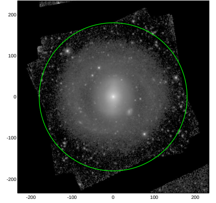
S4G: pa,inc= 50.2 15.2
