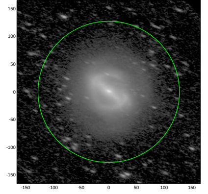
S4G: pa,inc= -19.1 64.1
