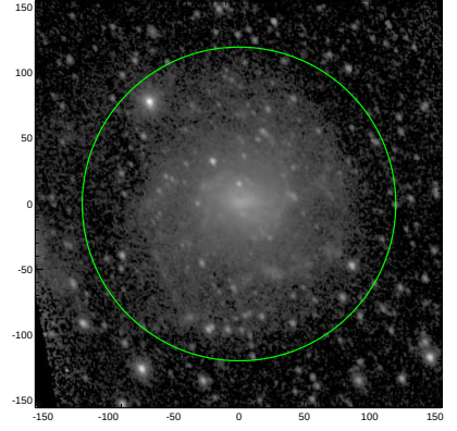
S4G: pa,inc= 122.6 35.4
