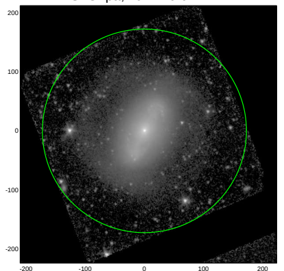
S4G: pa,inc= 79.0 14.7
