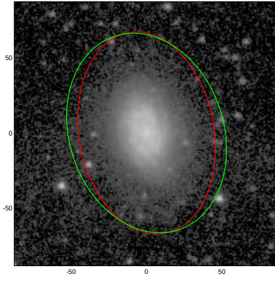
NGC5633
