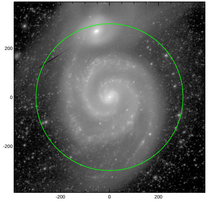
S4G: pa,inc= 39.1 32.8
