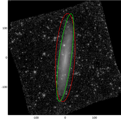
NGC5496
