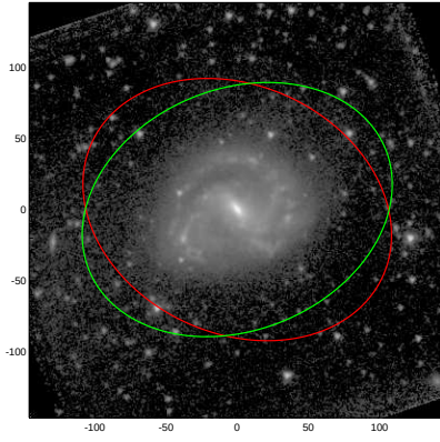
NGC5597
