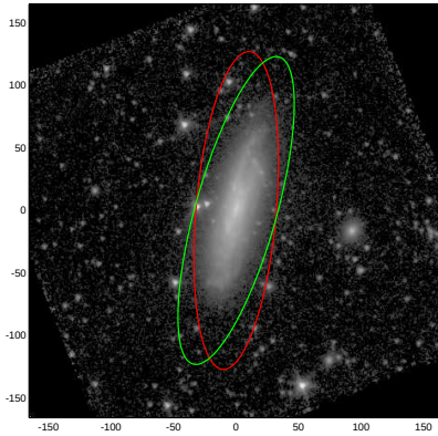
NGC5729
