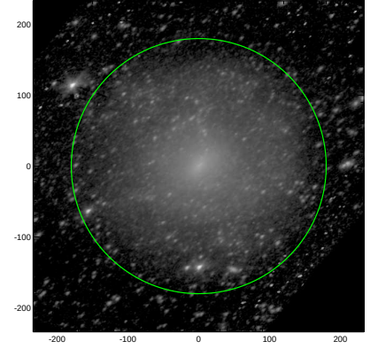
S4G: pa,inc= 35.1 51.5
