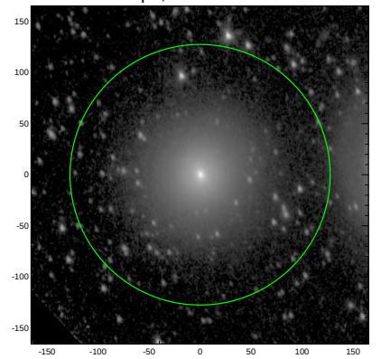
S4G: pa,inc= 103.1 44.1
