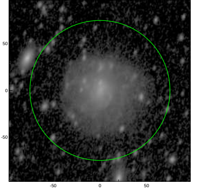
S4G: pa,inc= 73.2 49.6
