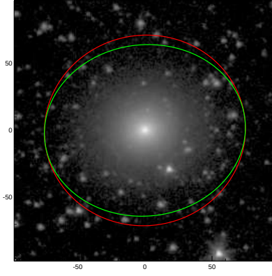
NGC5173
