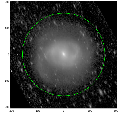
S4G: pa,inc= 110.2 65.4
