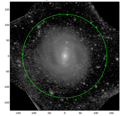
S4G: pa,inc= -20.7 29.8
