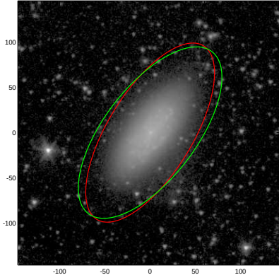
NGC5949
