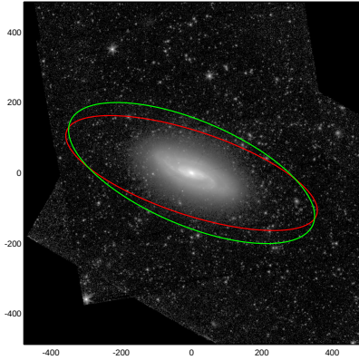
NGC5005
