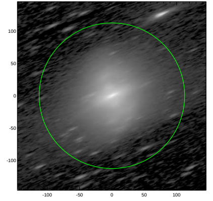
S4G: pa,inc= 23.5 77.3
