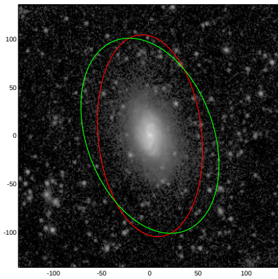
NGC5604
