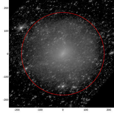
LEDA: pa,inc= 34.2 52.1
