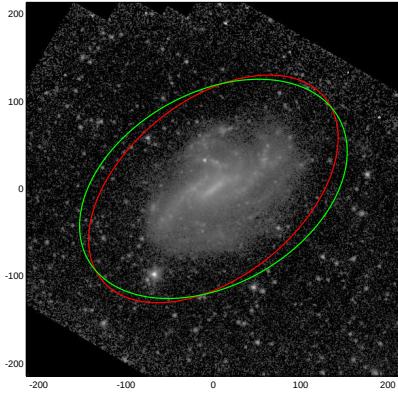
NGC5112
