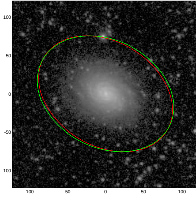
NGC5016
