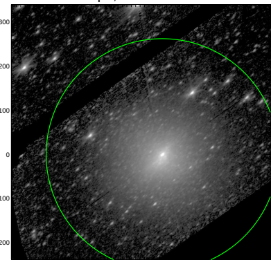
S4G: pa,inc= 42.2 62.0
