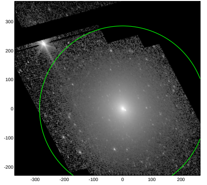
S4G: pa,inc= 126.5 49.9
