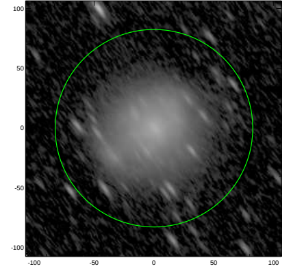
S4G: pa,inc= 126.7 70.9
