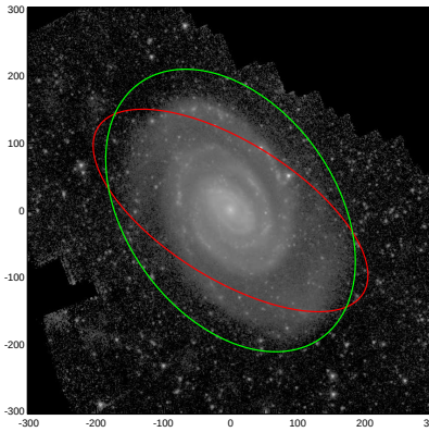
NGC5364
