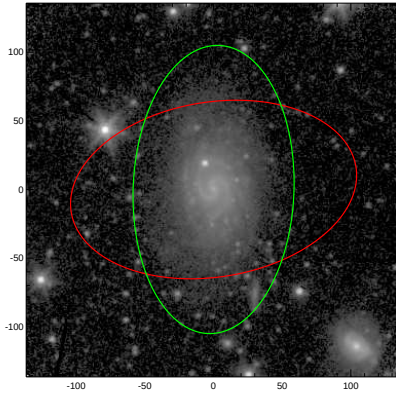
NGC5783
