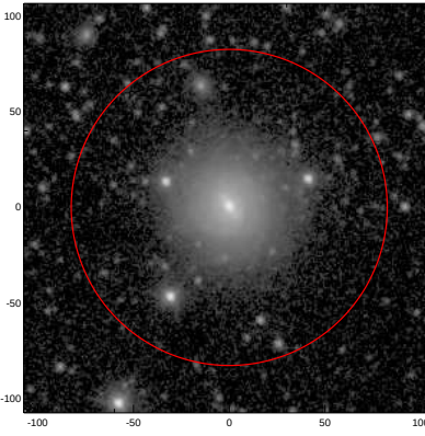
LEDA: pa,inc= 999.0 0.0
