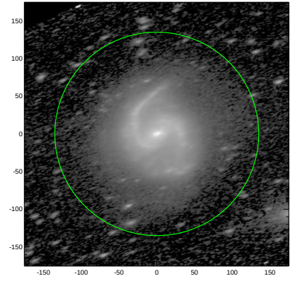
S4G: pa,inc= 19.6 67.2
