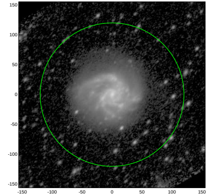
S4G: pa,inc= 47.2 52.1
