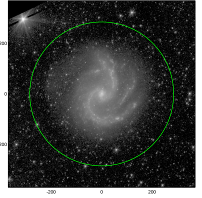
S4G: pa,inc= 61.6 29.7
