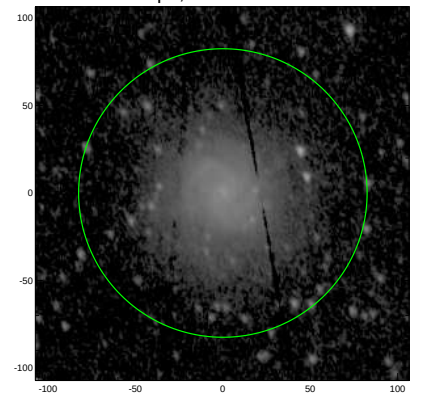
S4G: pa,inc= 107.6 47.0
