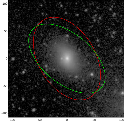
NGC5355
