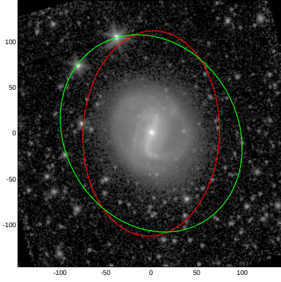
NGC5757
