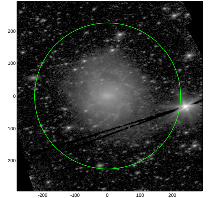
S4G: pa,inc= 15.9 55.7
