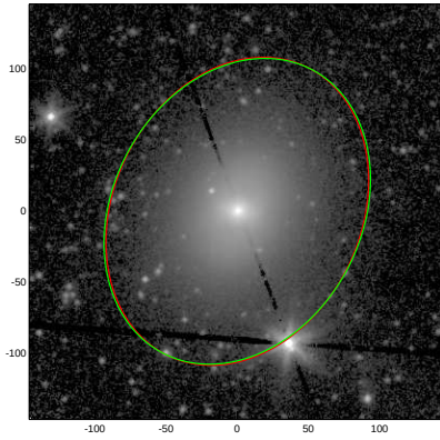
NGC5473
