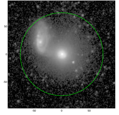
S4G: pa,inc= 35.9 20.4
