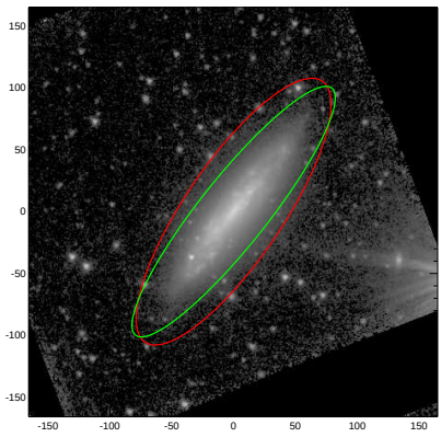
NGC5690
