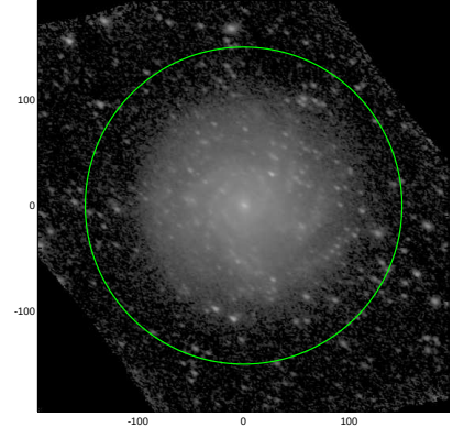
S4G: pa,inc= 149.7 49.8
