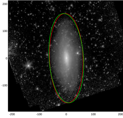
NGC5879
