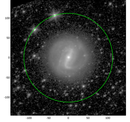
S4G: pa,inc= 30.9 32.7
