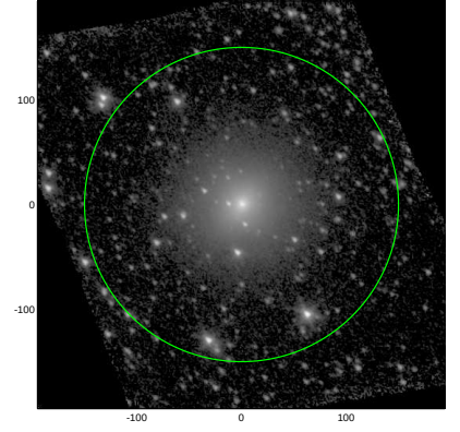
S4G: pa,inc= 138.4 38.3
