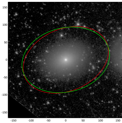
NGC5481
