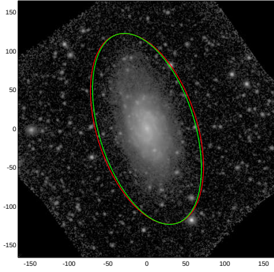
NGC5320
