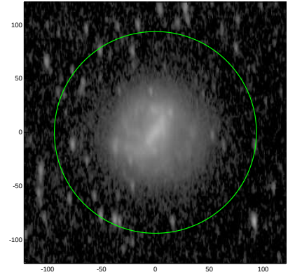
S4G: pa,inc= 92.6 68.6
