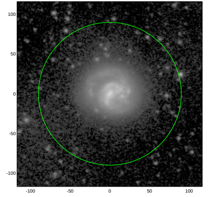
S4G: pa,inc= -12.0 22.2
