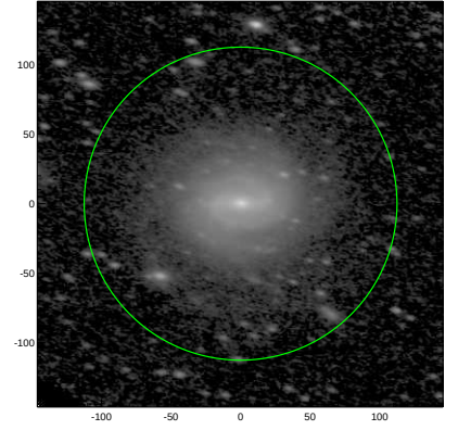
S4G: pa,inc= -13.3 57.0
