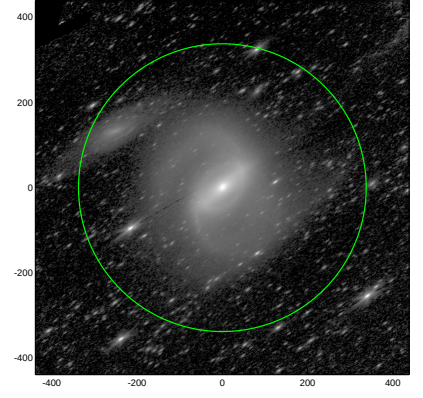
S4G: pa,inc= 34.8 68.4
