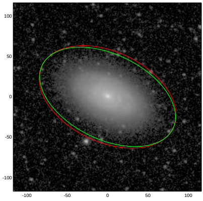
NGC5376
