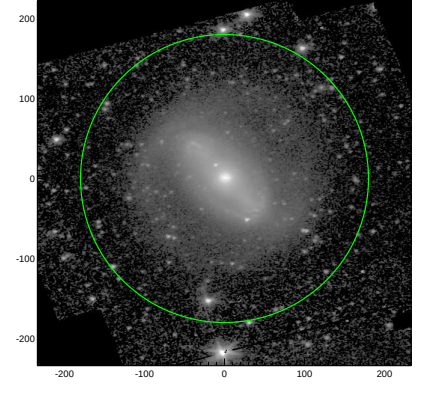
S4G: pa,inc= 6.7 43.0
