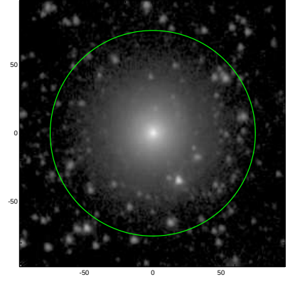
S4G: pa,inc= 96.0 31.6
