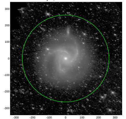
S4G: pa,inc= 156.6 52.3
