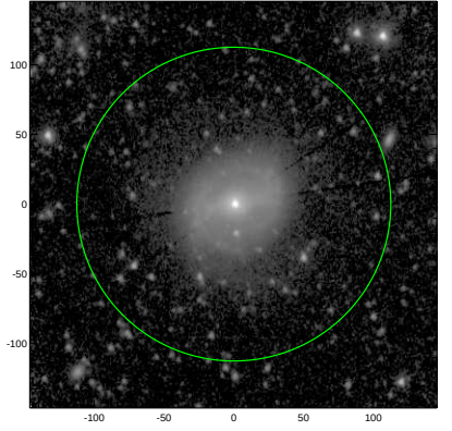
S4G: pa,inc= 89.4 22.8
