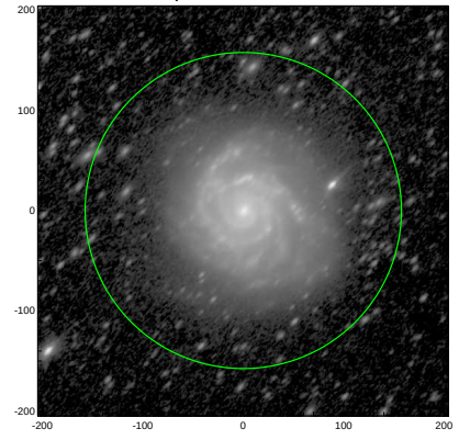
S4G: pa,inc= 48.1 59.8
