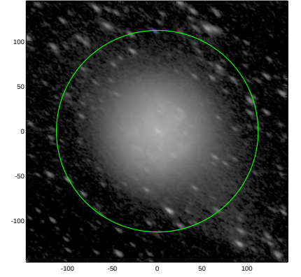
S4G: pa,inc= 142.7 63.1
