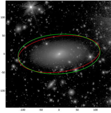
NGC5338
