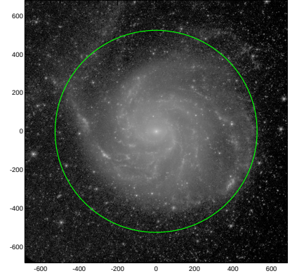
S4G: pa,inc= 37.7 21.7
