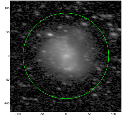
S4G: pa,inc= -11.3 61.7
