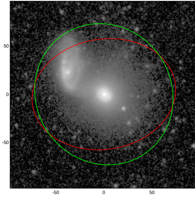
NGC5953
