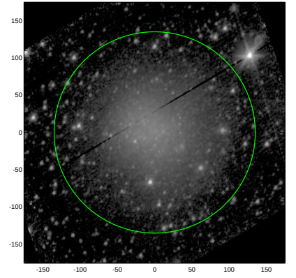
S4G: pa,inc= 59.8 37.3
