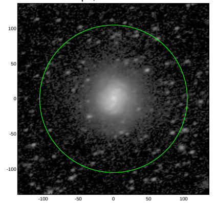
S4G: pa,inc= 20.2 51.2
