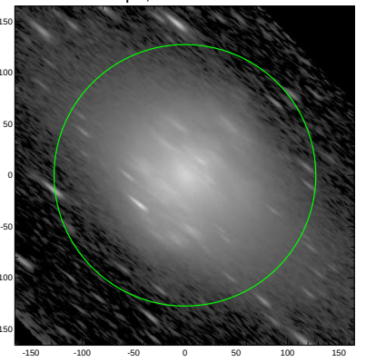
S4G: pa,inc= 141.5 77.6
