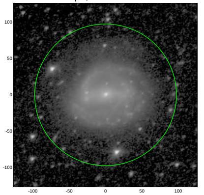
S4G: pa,inc= 34.5 40.0
