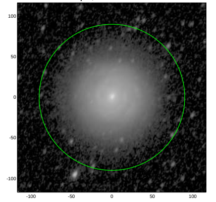
S4G: pa,inc= 64.0 54.3
