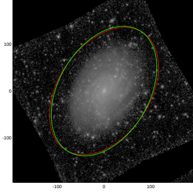
NGC5300
