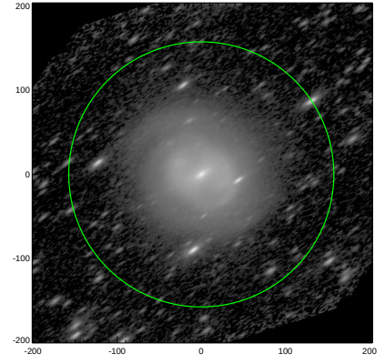
S4G: pa,inc= 35.1 68.0
