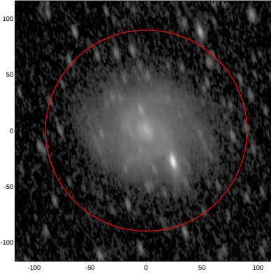
LEDA: pa,inc= 104.9 66.6
