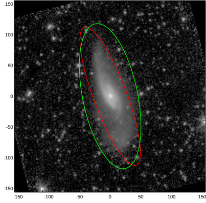
NGC5916
