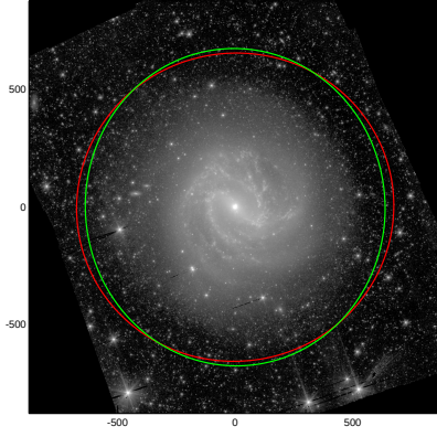
NGC5236
