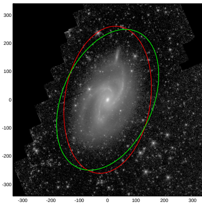
NGC5054
