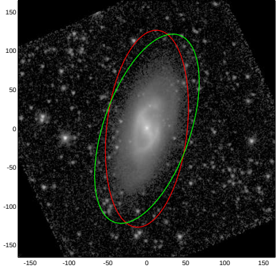
NGC5913
