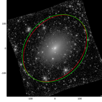
NGC5304
