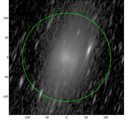
S4G: pa,inc= 70.4 77.9
