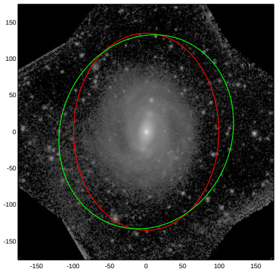
NGC5375
