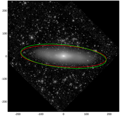
NGC5689
