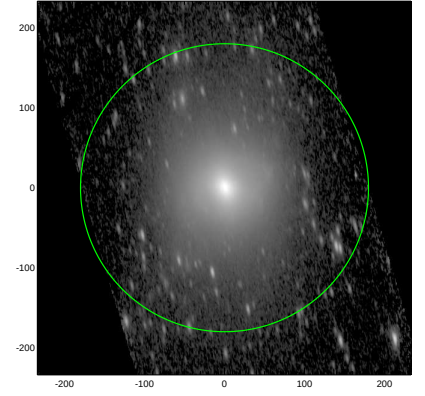
S4G: pa,inc= 99.9 69.4
