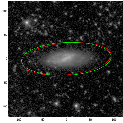
NGC5630
