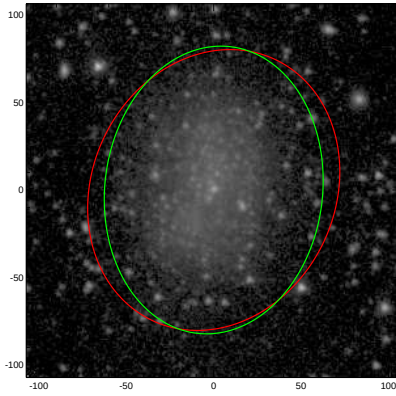
NGC5238
