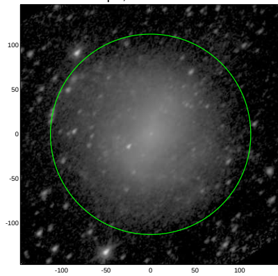
S4G: pa,inc= 48.4 50.6
