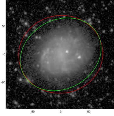
NGC5147
