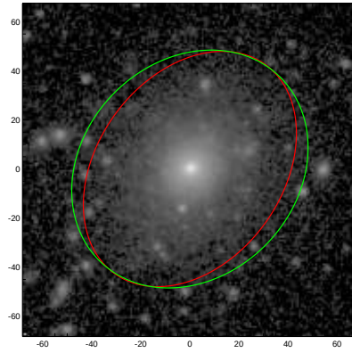
NGC5762
