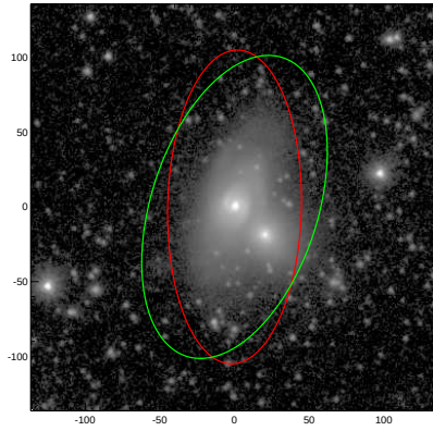
NGC5930
