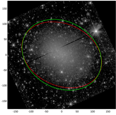
NGC5264
