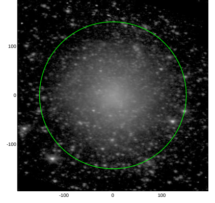
S4G: pa,inc= -6.3 50.5
