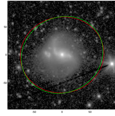
NGC5534
