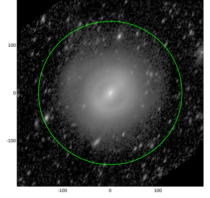
S4G: pa,inc= 62.9 60.2
