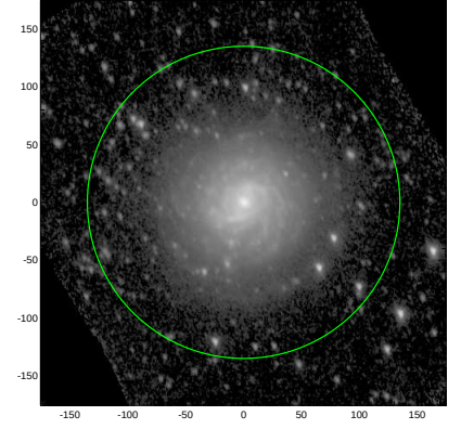
S4G: pa,inc= 106.2 44.7
