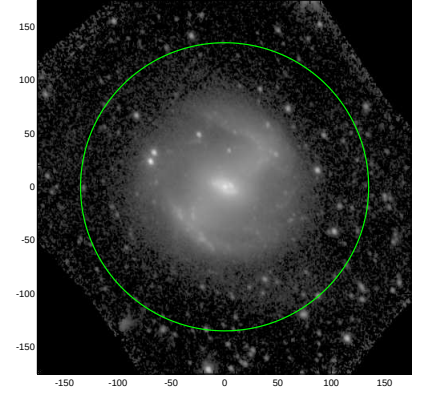
S4G: pa,inc= 110.6 34.7
