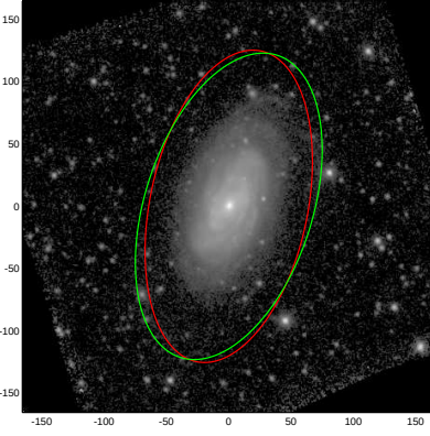
NGC5740
