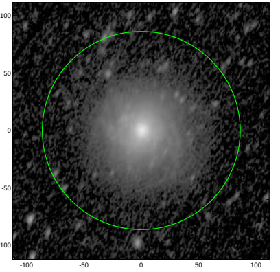
S4G: pa,inc= 66.8 57.5
