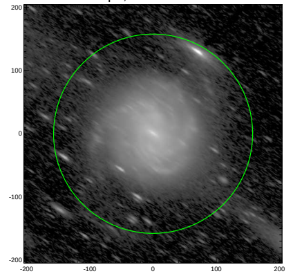
S4G: pa,inc= 146.3 73.6
