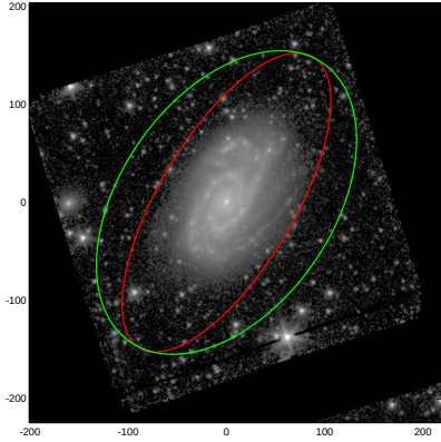
NGC5861
