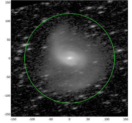
S4G: pa,inc= 11.7 68.1
