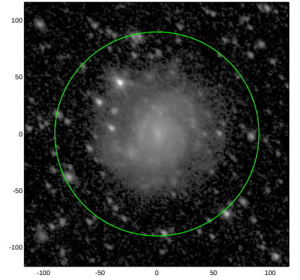
S4G: pa,inc= 135.6 42.1
