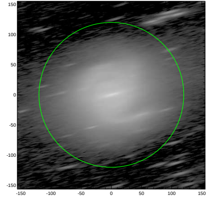
S4G: pa,inc= 13.6 81.5
