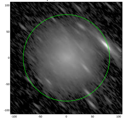
S4G: pa,inc= 133.6 77.0
