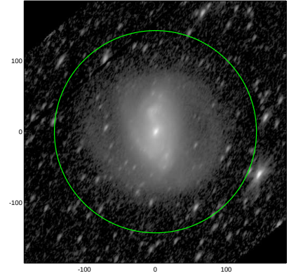
S4G: pa,inc= 59.9 65.3
