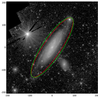
NGC5297
