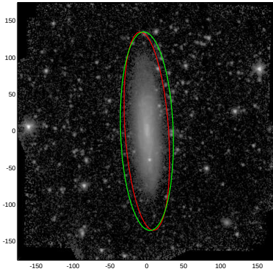
NGC5951
