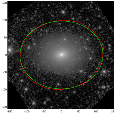
NGC5311
