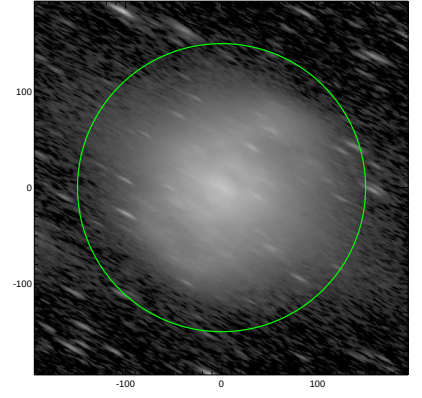
S4G: pa,inc= 151.1 78.4
