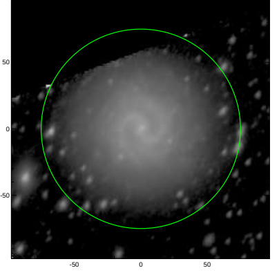
S4G: pa,inc= 57.9 47.2
