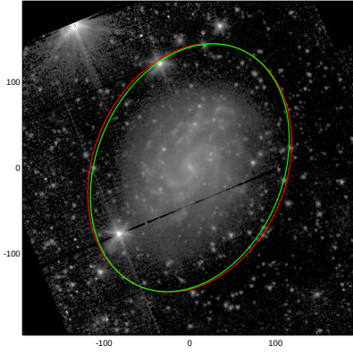
NGC5584
