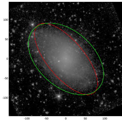
NGC5832
