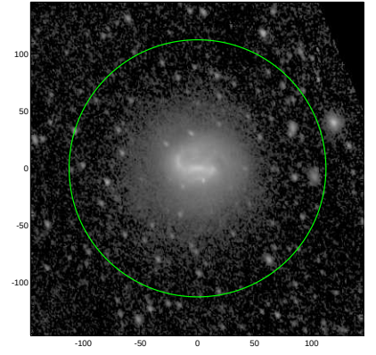
S4G: pa,inc= 114.6 40.5
