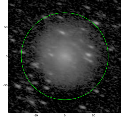
S4G: pa,inc= 158.9 62.7
