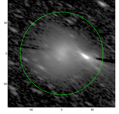
S4G: pa,inc= 149.8 70.2
