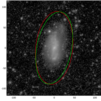
NGC5667
