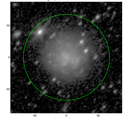
S4G: pa,inc= 46.8 48.8
