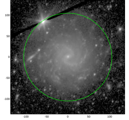
S4G: pa,inc= 61.7 36.0
