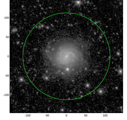
S4G: pa,inc= 120.6 21.8
