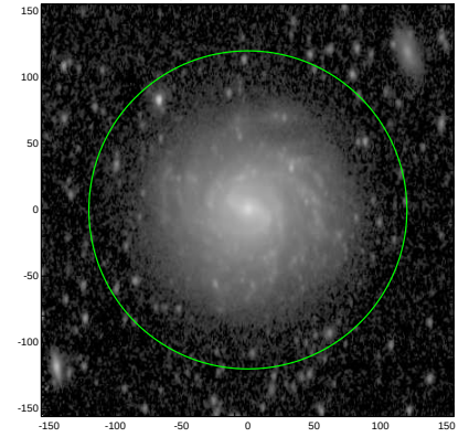
S4G: pa,inc= 87.5 50.3
