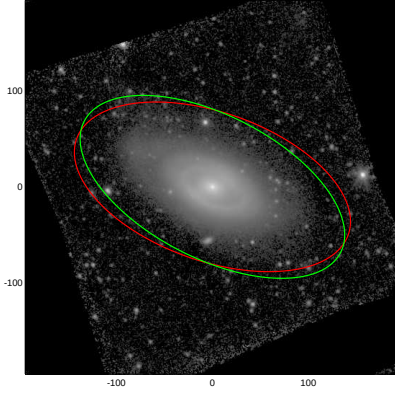
NGC5750
