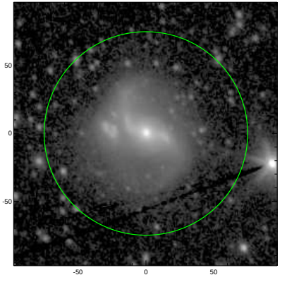
S4G: pa,inc= 119.7 26.8
