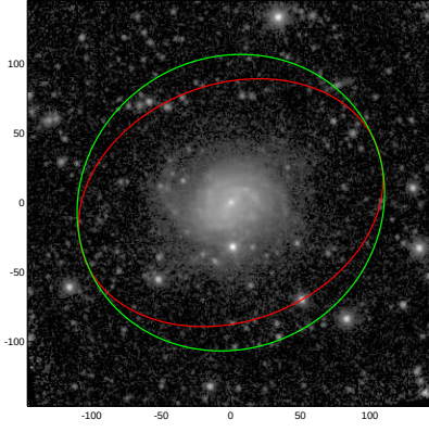
NGC5768
