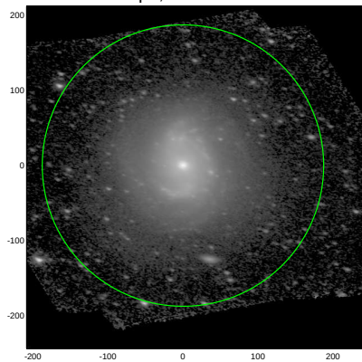
S4G: pa,inc= -13.4 56.5
