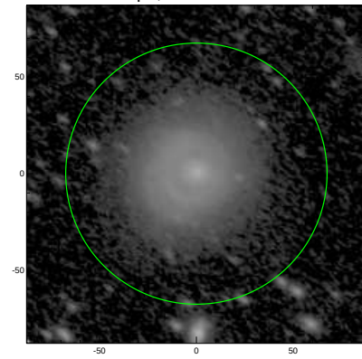
S4G: pa,inc= 146.1 54.0
