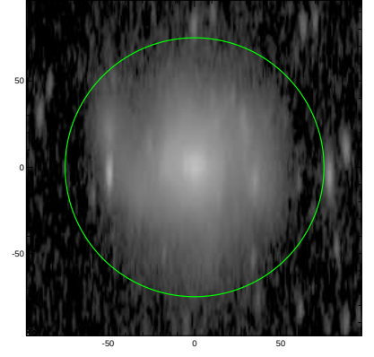
S4G: pa,inc= 89.0 78.2
