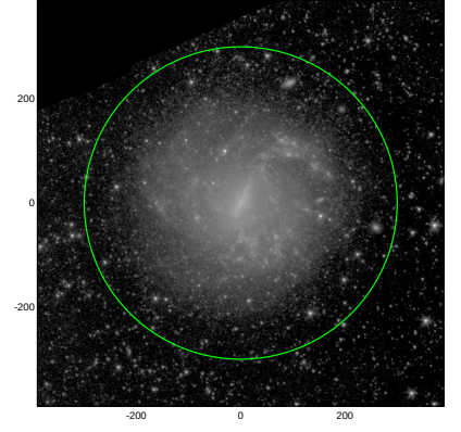
S4G: pa,inc= 99.1 13.1
