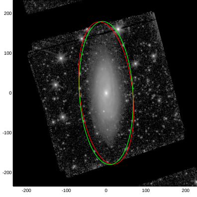
NGC5878
