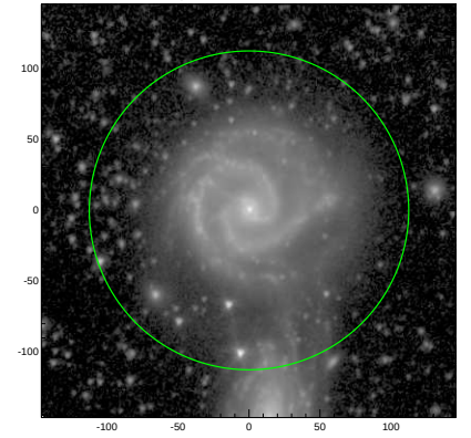
S4G: pa,inc= 71.6 25.2
