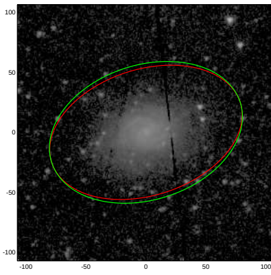
NGC5452
