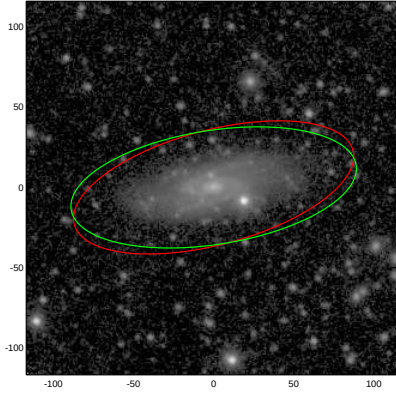
NGC5169
