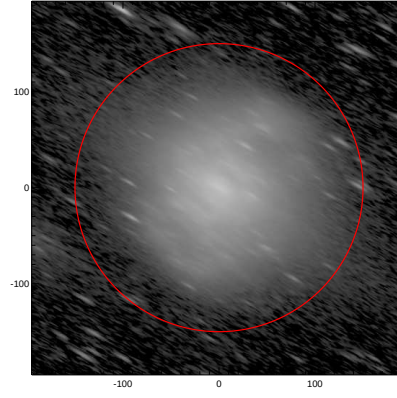
LEDA: pa,inc= 150.1 77.8
