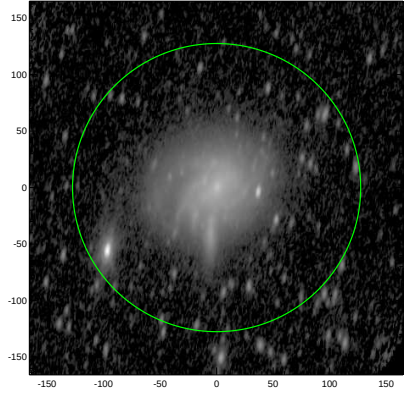
S4G: pa,inc= 80.8 65.4
