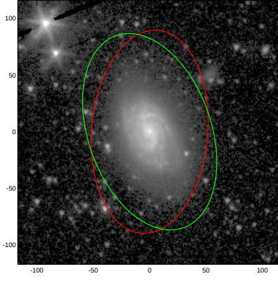
NGC5937
