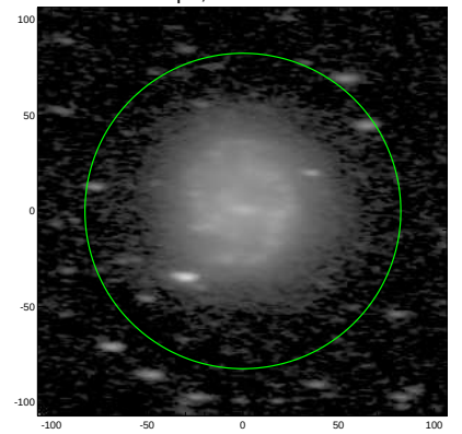
S4G: pa,inc= -3.2 67.5
