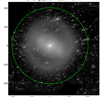
S4G: pa,inc= 26.4 57.4
