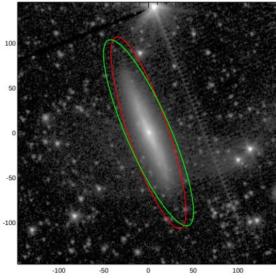
NGC5022
