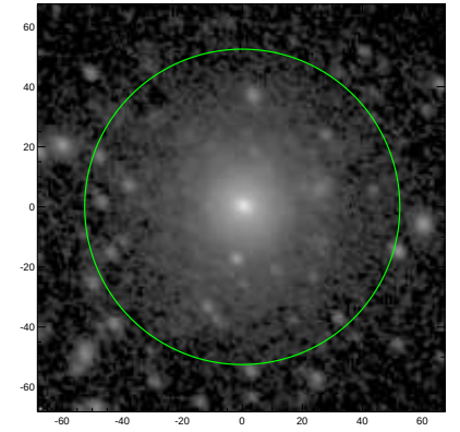
S4G: pa,inc= 136.0 33.6
