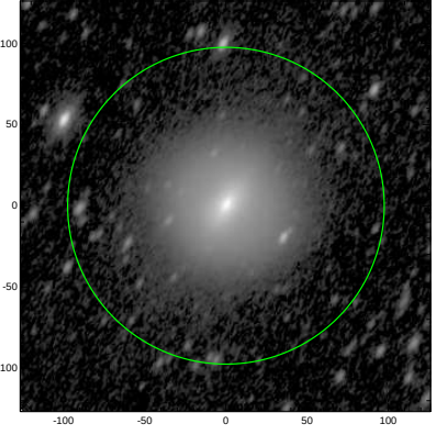
S4G: pa,inc= 60.1 59.0
