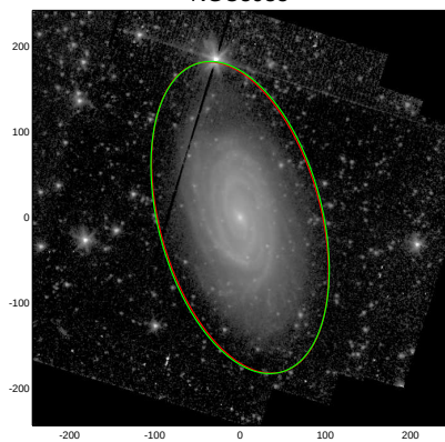
NGC5985
