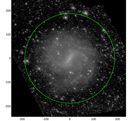
S4G: pa,inc= 150.4 43.4
