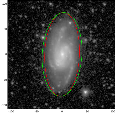
NGC6181
