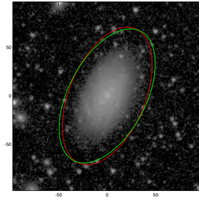
NGC6063
