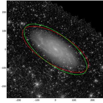
NGC6118
