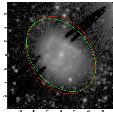
NGC6267
