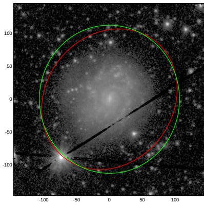
NGC6412
