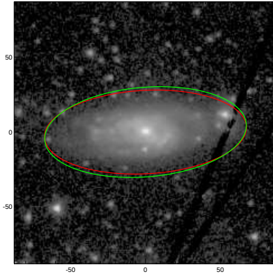
NGC6434
