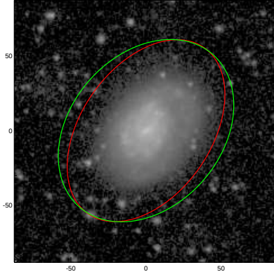
NGC6155
