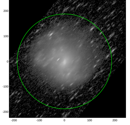
S4G: pa,inc= 44.2 72.7
