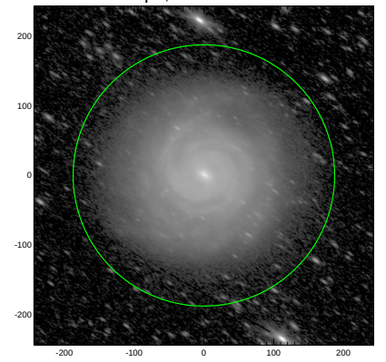
S4G: pa,inc= 145.8 67.0
