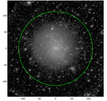
S4G: pa,inc= 17.9 28.6
