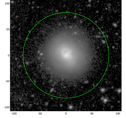
S4G: pa,inc= -12.7 12.5
