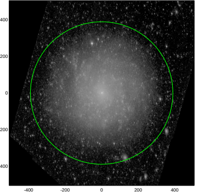
S4G: pa,inc= 96.7 52.2
