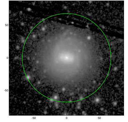
S4G: pa,inc= 66.3 21.3
