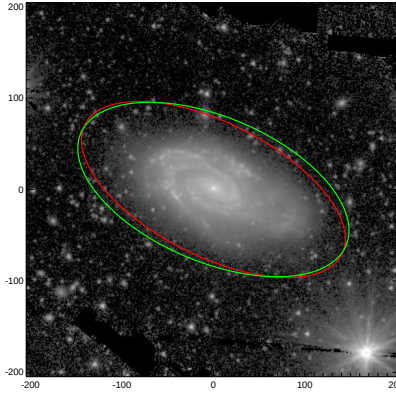
NGC7205
