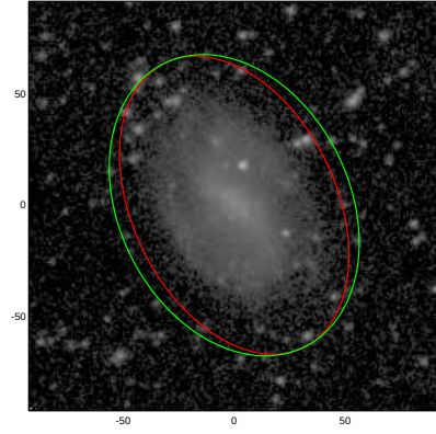
NGC7661
