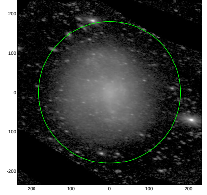
S4G: pa,inc= -13.5 61.4
