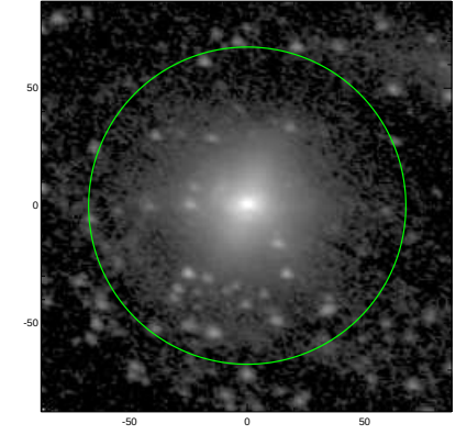
S4G: pa,inc= 157.7 42.9
