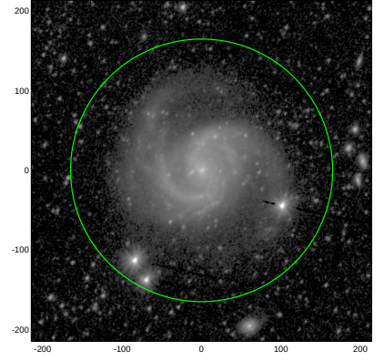
S4G: pa,inc= 62.7 33.4
