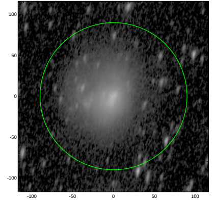
S4G: pa,inc= 77.7 64.3
