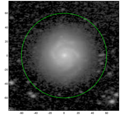
S4G: pa,inc= 2.2 50.4
