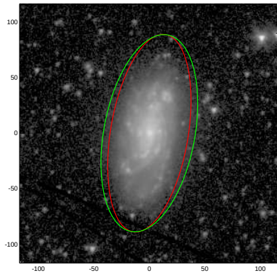
NGC7448
