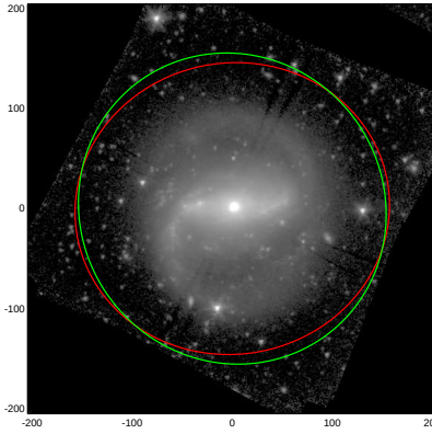
NGC7552
