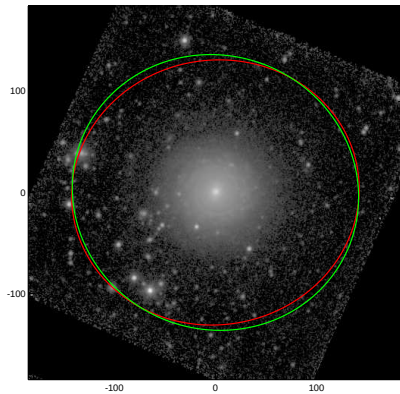
NGC7371
