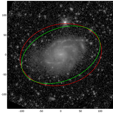
NGC7757
