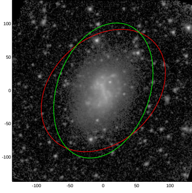
NGC7764
