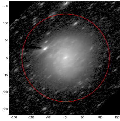
LEDA: pa,inc= 33.7 66.1
