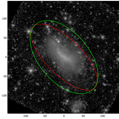
NGC7800
