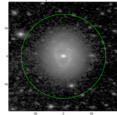
S4G: pa,inc= -4.0 51.5
