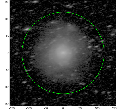
S4G: pa,inc= 12.7 65.2
