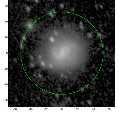
S4G: pa,inc= 124.6 48.7
