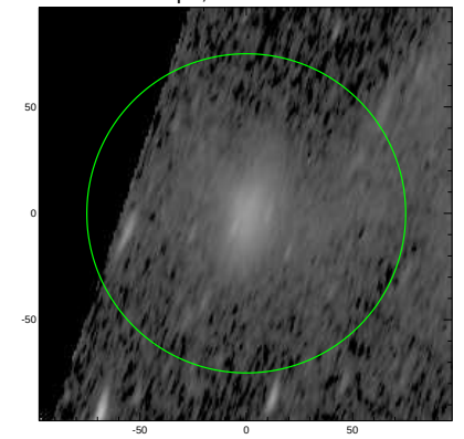
S4G: pa,inc= 72.8 75.0
