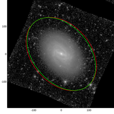
NGC7723
