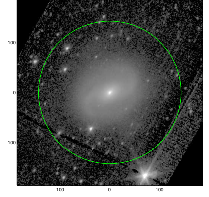
S4G: pa,inc= 56.5 41.7
