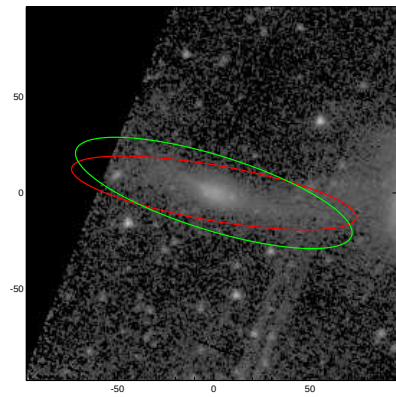
NGC7715
