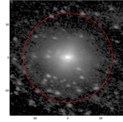
LEDA: pa,inc= 161.5 52.8
