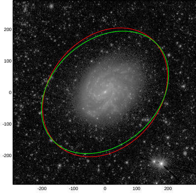
NGC7418
