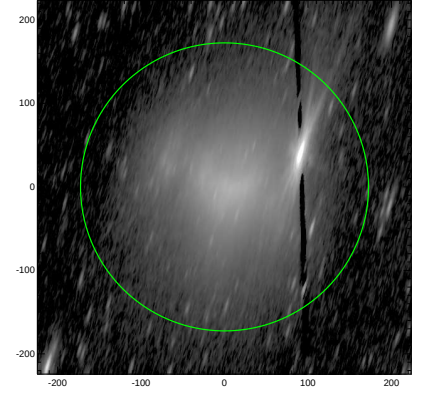
S4G: pa,inc= 75.2 78.7
