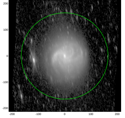
S4G: pa,inc= 99.0 72.8
