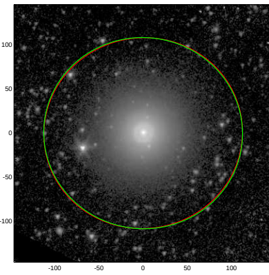
NGC7742
