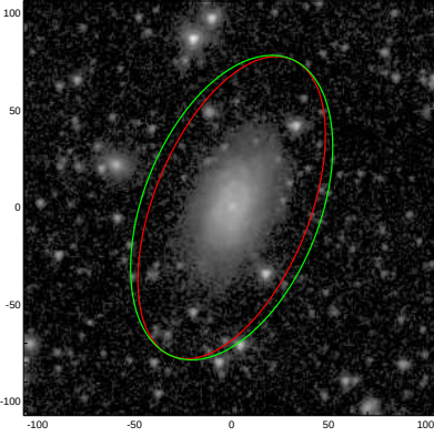
NGC7290
