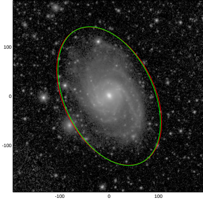
NGC7755
