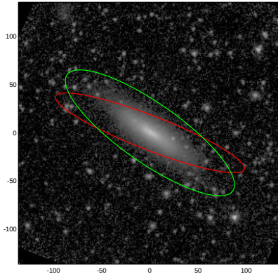
NGC7709
