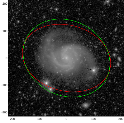
NGC7412
