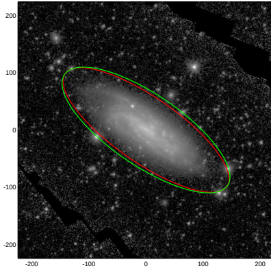
NGC7599
