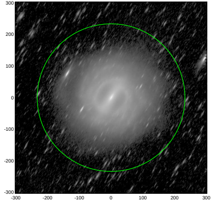
S4G: pa,inc= 59.5 75.1
