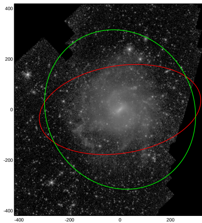
NGC7424
