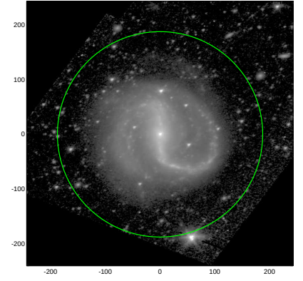
S4G: pa,inc= 19.5 41.2
