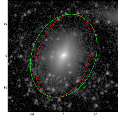
NGC7465
