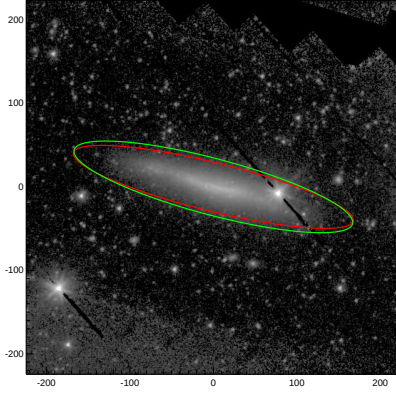
NGC7462
