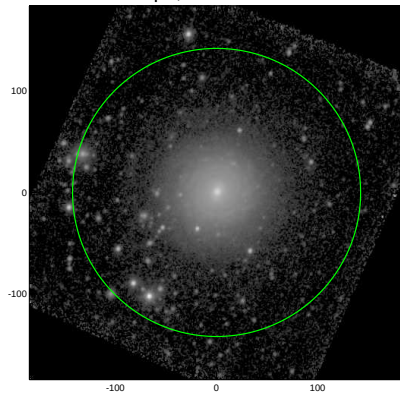
S4G: pa,inc= 69.0 18.1
