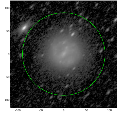
S4G: pa,inc= 46.3 61.0
