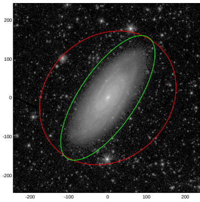
NGC7606
