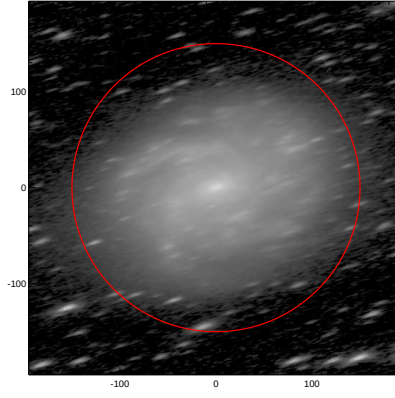
LEDA: pa,inc= 16.2 75.5
