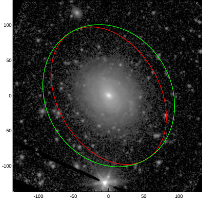
NGC7716
