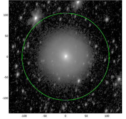
S4G: pa,inc= 74.8 49.0
