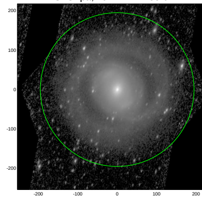
S4G: pa,inc= 72.2 55.0
