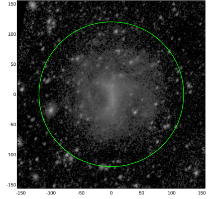
S4G: pa,inc= 55.8 35.8
