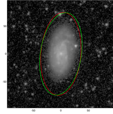
NGC7750
