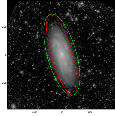
NGC7721
