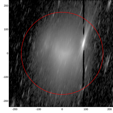
LEDA: pa,inc= 76.3 80.3
