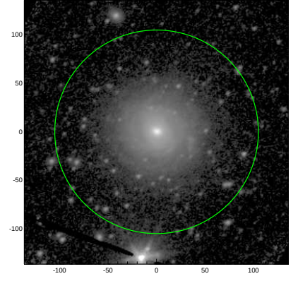
S4G: pa,inc= 31.3 31.7
