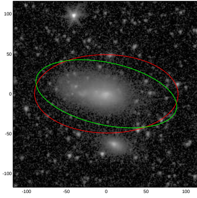
NGC7694
