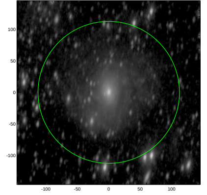
S4G: pa,inc= 82.9 59.9
