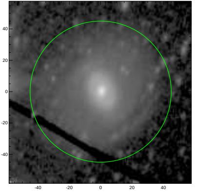
S4G: pa,inc= 73.7 44.5
