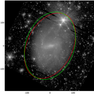
NGC7741
