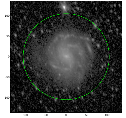
S4G: pa,inc= 112.4 51.0
