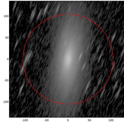
LEDA: pa,inc= 68.8 80.3
