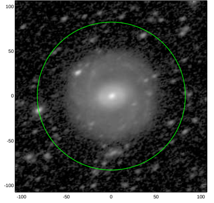
S4G: pa,inc= 28.7 50.4
