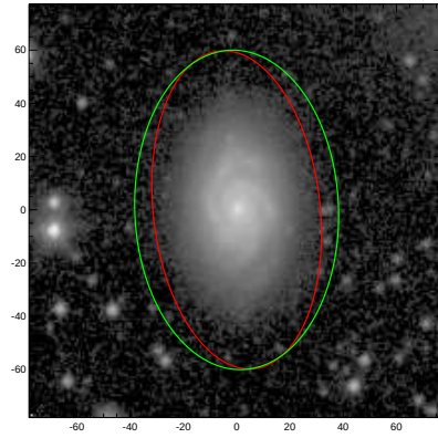
NGC7247
