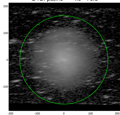
S4G: pa,inc= 4.9 76.5
