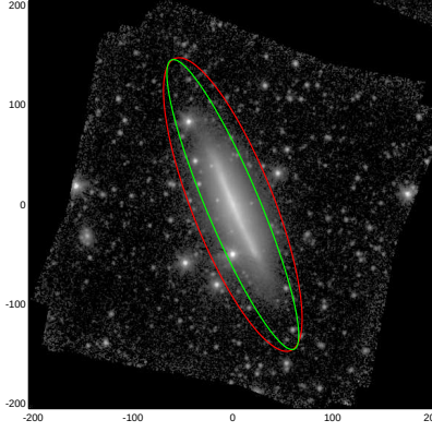
NGC7241
