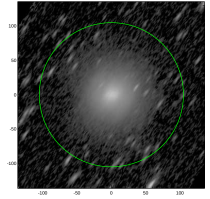
S4G: pa,inc= 54.9 73.0
