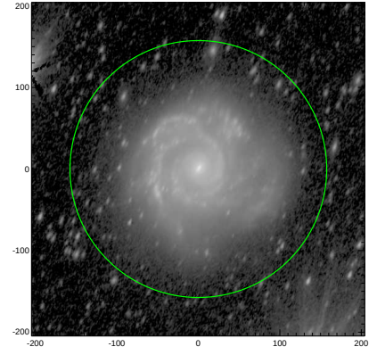
S4G: pa,inc= 67.0 59.8
