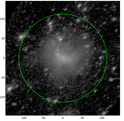
S4G: pa,inc= 40.8 55.1
