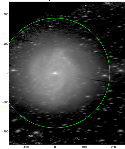
S4G: pa,inc= 2.7 66.9
