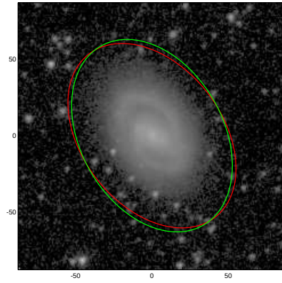
NGC7724
