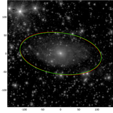
NGC7418A
