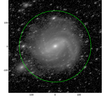
S4G: pa,inc= 25.5 53.1
