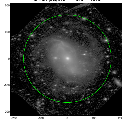
S4G: pa,inc= 3.5 49.8
