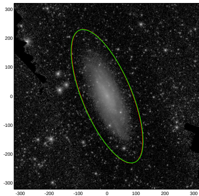
NGC7456
