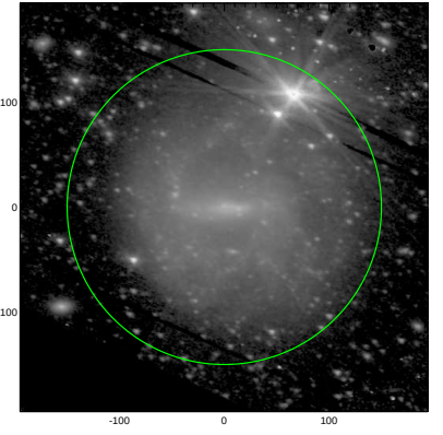
S4G: pa,inc= -19.1 45.5
