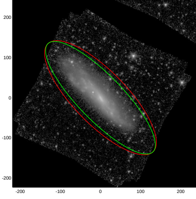
NGC7497
