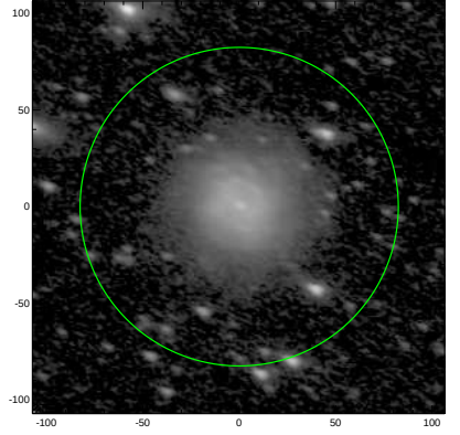
S4G: pa,inc= 158.4 56.6
