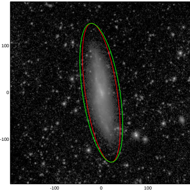
NGC7307
