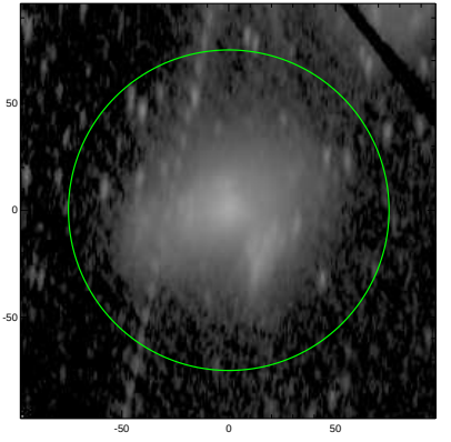
S4G: pa,inc= 87.5 67.7
