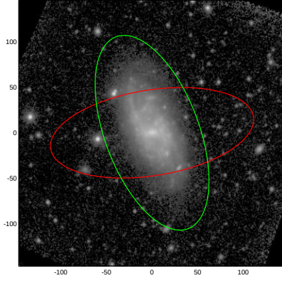
NGC7218
