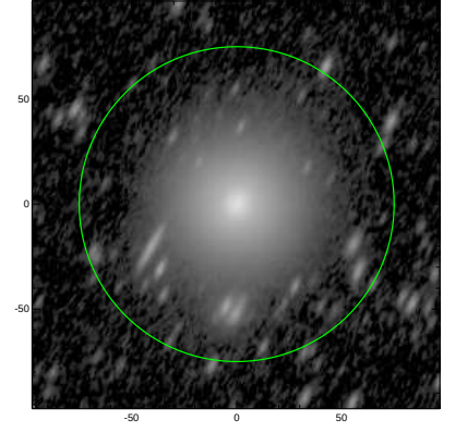
S4G: pa,inc= 64.4 62.7
