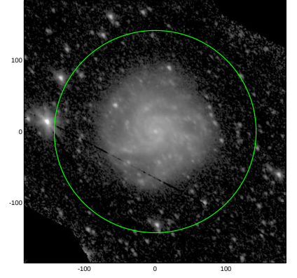
S4G: pa,inc= 128.5 49.1
