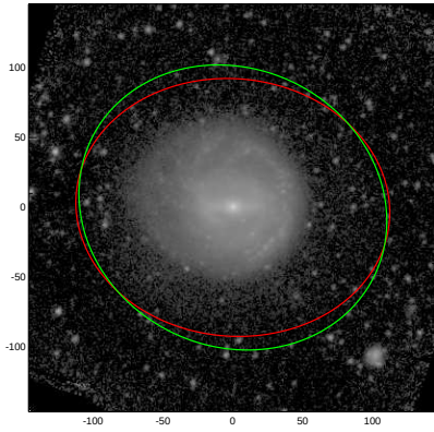
NGC7421
