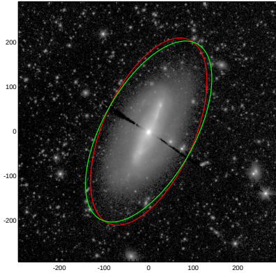
NGC7582
