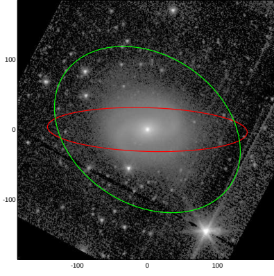
NGC7743
