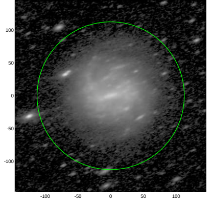
S4G: pa,inc= 20.5 62.7
