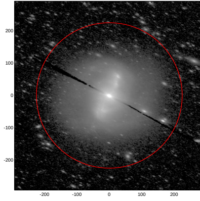
LEDA: pa,inc= 156.3 62.8
