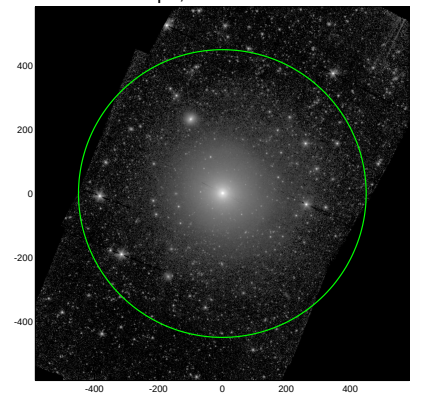
S4G: pa,inc= 159.2 20.1
