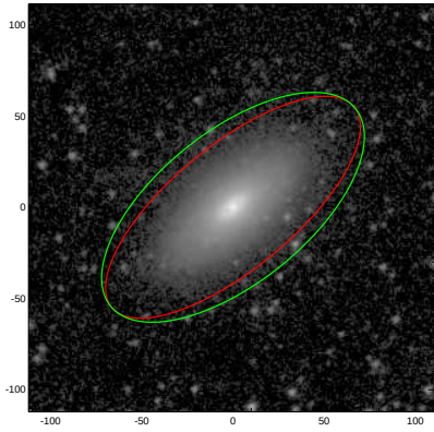
NGC7690
