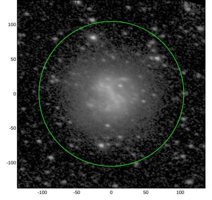
S4G: pa,inc= 159.9 48.7
