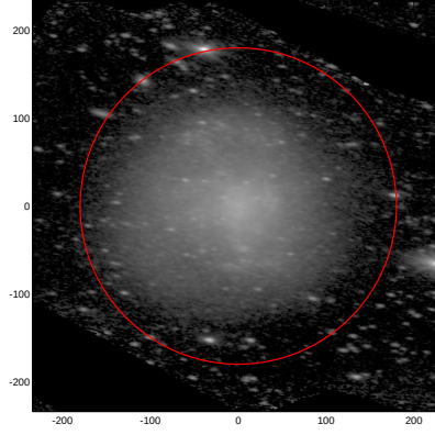
LEDA: pa,inc= 170.2 64.2
