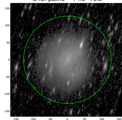
S4G: pa,inc= 74.6 70.5
