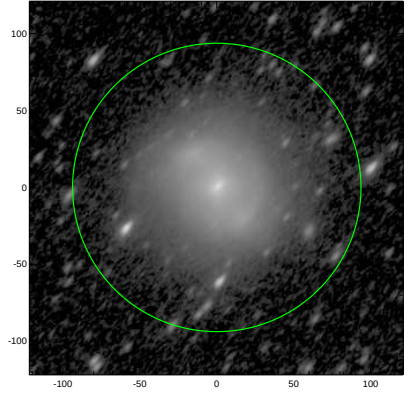
S4G: pa,inc= 50.5 58.9
