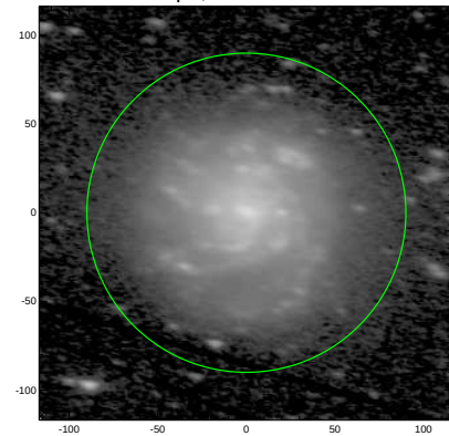
S4G: pa,inc= -10.6 62.9
