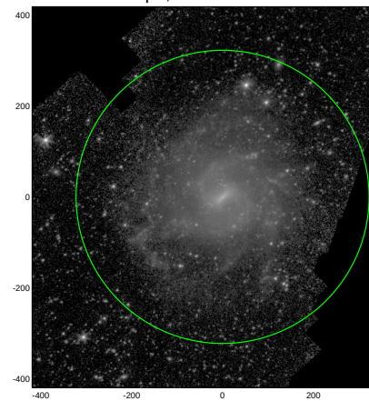
S4G: pa,inc= 29.3 25.3
