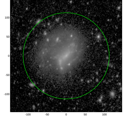
S4G: pa,inc= 74.8 35.4
