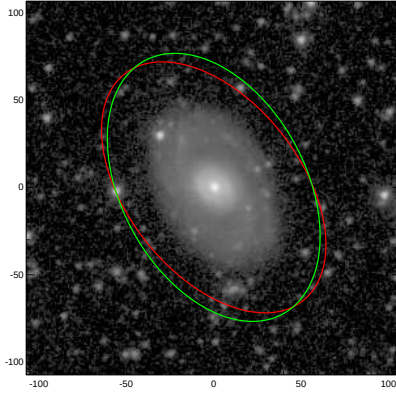
NGC7219
