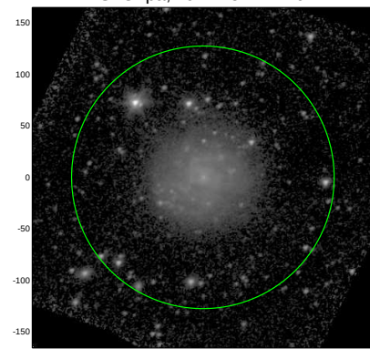
S4G: pa,inc= 25.1 27.9
