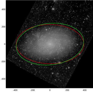
NGC7793
