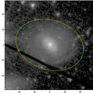
NGC7731
