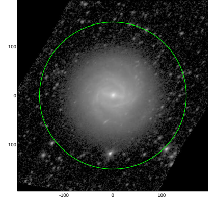
S4G: pa,inc= 40.2 47.8
