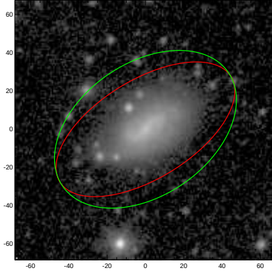
NGC7254
