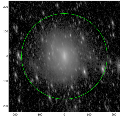
S4G: pa,inc= 101.4 66.1
