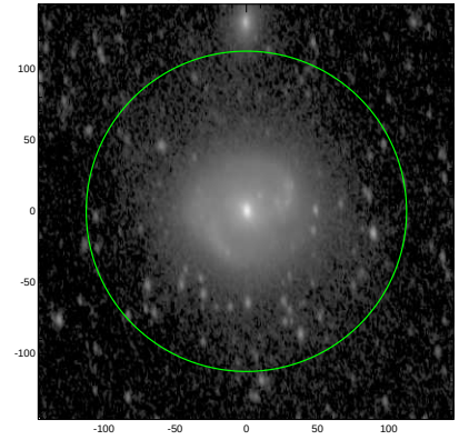
S4G: pa,inc= 98.1 57.5
