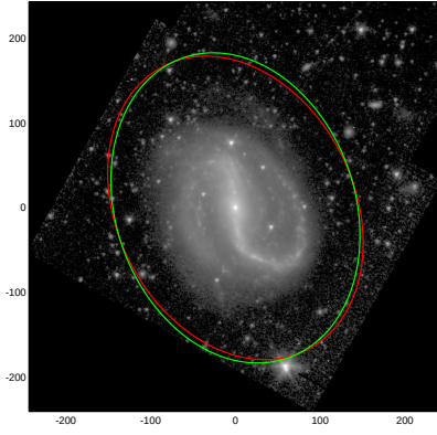
NGC7479
