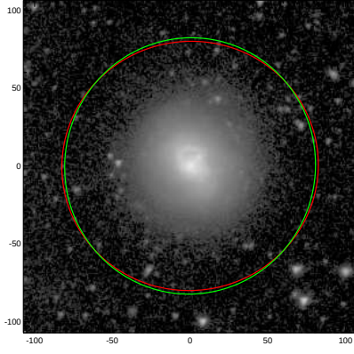
NGC7625
