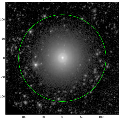
S4G: pa,inc= 84.2 15.9
