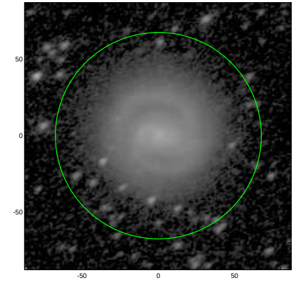
S4G: pa,inc= 30.0 46.3
