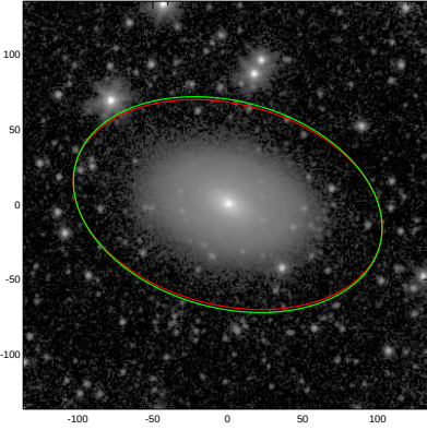
NGC7280
