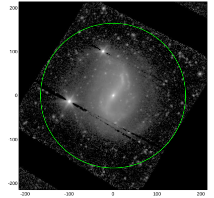
S4G: pa,inc= 33.2 16.4
