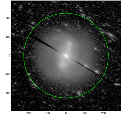
S4G: pa,inc= 151.1 62.6
