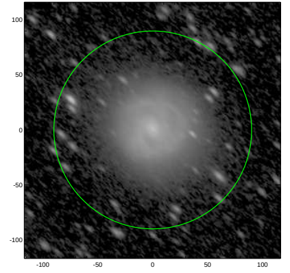
S4G: pa,inc= 136.7 65.0
