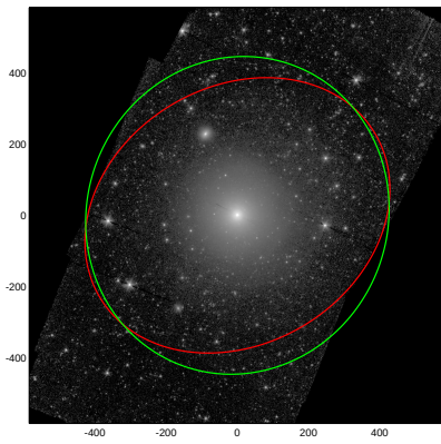
NGC7213
