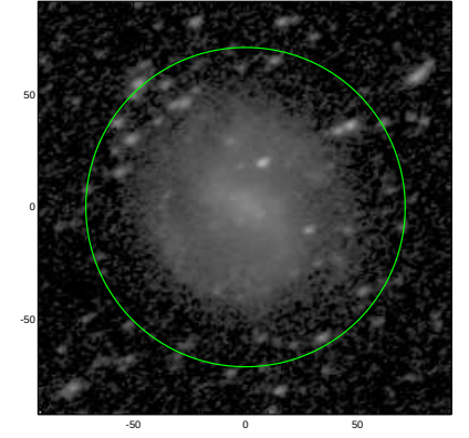
S4G: pa,inc= 26.5 43.2
