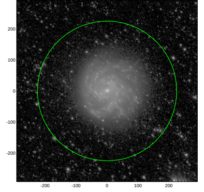
S4G: pa,inc= 131.4 42.2
