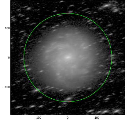
S4G: pa,inc= 15.8 69.7
