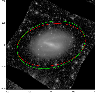
NGC7513
