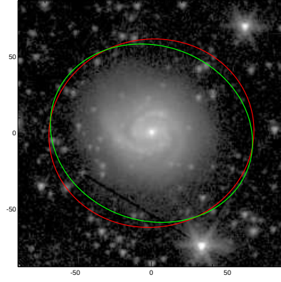
NGC7798
