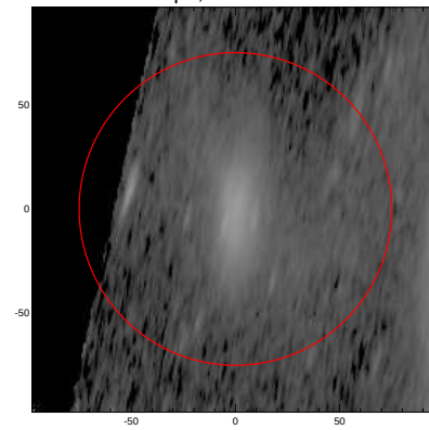
LEDA: pa,inc= 80.1 78.9
