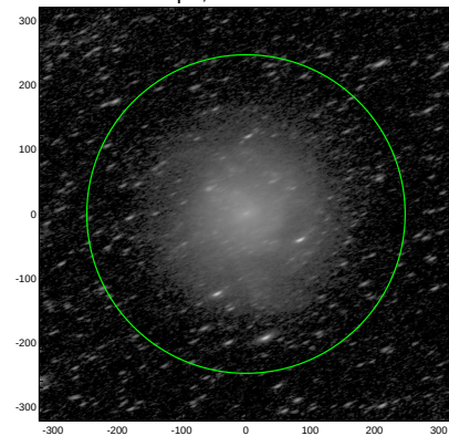
S4G: pa,inc= 22.9 69.7
