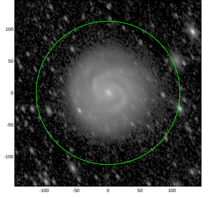
S4G: pa,inc= 119.9 57.5
