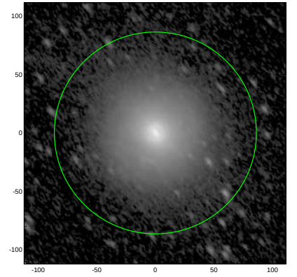
S4G: pa,inc= 128.8 61.3
