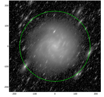
S4G: pa,inc= 55.8 68.8
