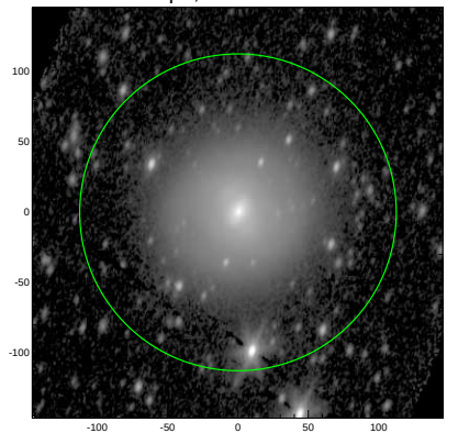
S4G: pa,inc= 75.5 51.3
