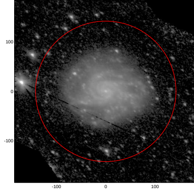
LEDA: pa,inc= 141.1 50.4
