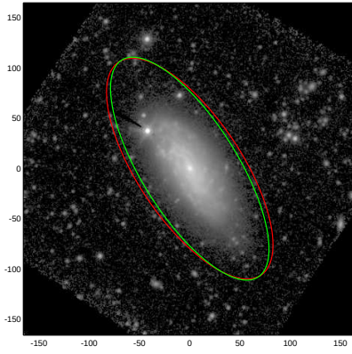
NGC7590
