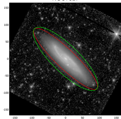
NGC7817
