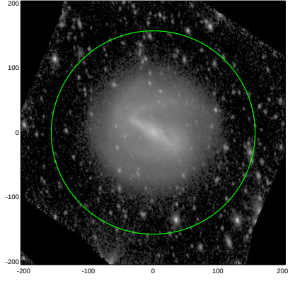
S4G: pa,inc= 105.6 48.4
