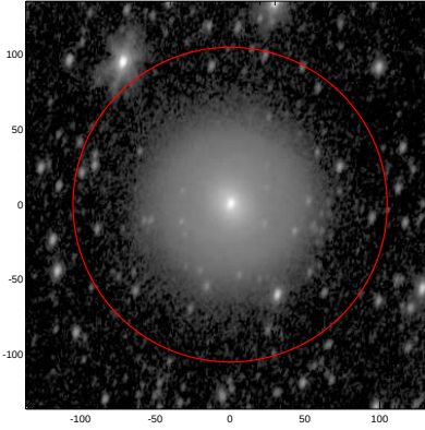
LEDA: pa,inc= 75.7 50.2
