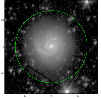
S4G: pa,inc= 70.5 31.9
