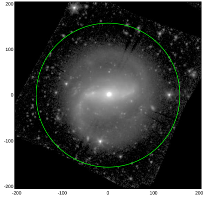
S4G: pa,inc= 38.5 15.8
