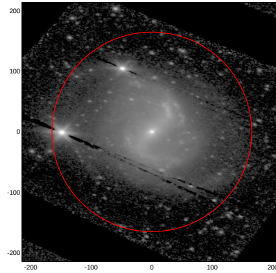
LEDA: pa,inc= 168.9 50.4
