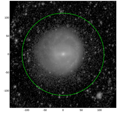
S4G: pa,inc= 64.6 27.9
