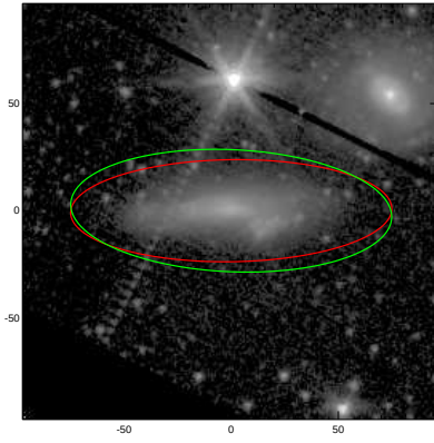
NGC7732
