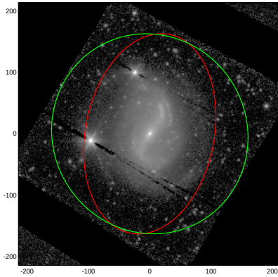
NGC7496
