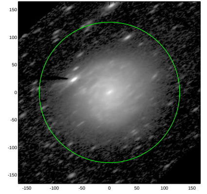
S4G: pa,inc= 32.1 68.1
