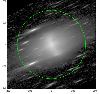
S4G: pa,inc= 23.0 80.3
