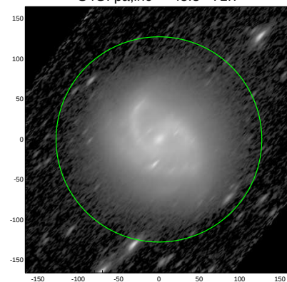
S4G: pa,inc= 45.8 71.7
