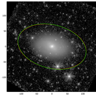
NGC7079
