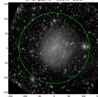
S4G: pa,inc= 100.6 28.8
