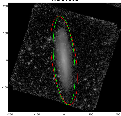
NGC7361
