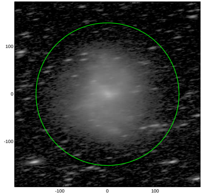
S4G: pa,inc= 8.9 74.5
