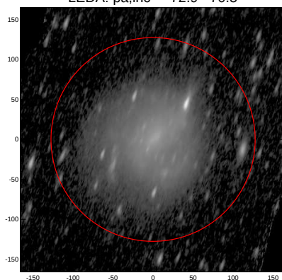
LEDA: pa,inc= 72.9 70.5
