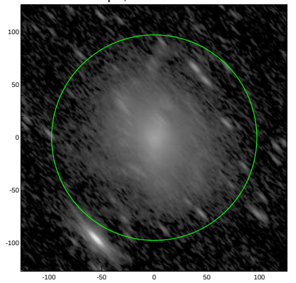
S4G: pa,inc= 133.7 72.8
