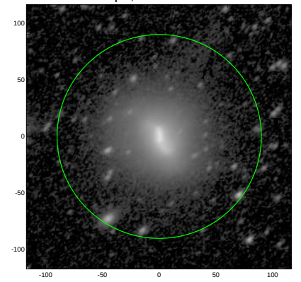
S4G: pa,inc= 42.3 49.3
