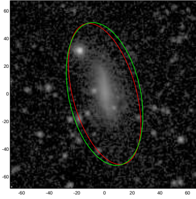
PGC1059326
