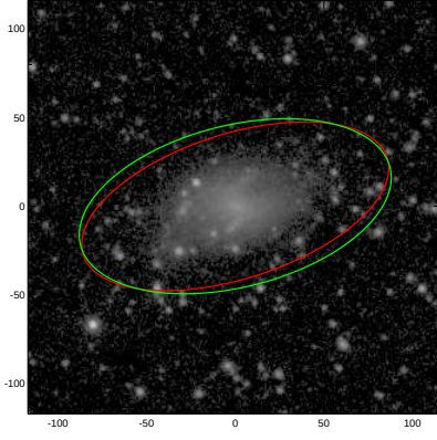
PGC044735
