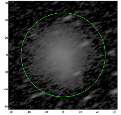
S4G: pa,inc= 23.4 67.8
