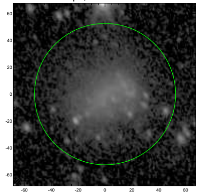
S4G: pa,inc= 115.0 41.5
