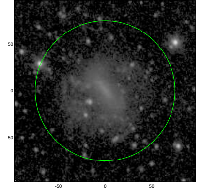
S4G: pa,inc= 121.1 24.9
