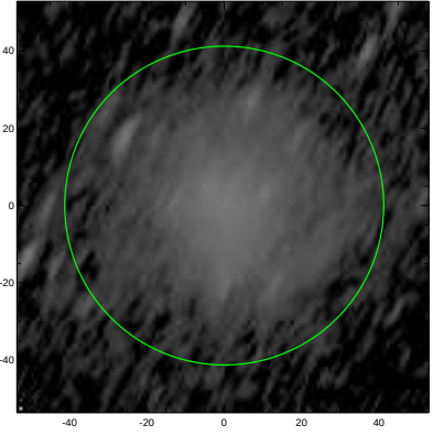
S4G: pa,inc= 63.2 71.9
