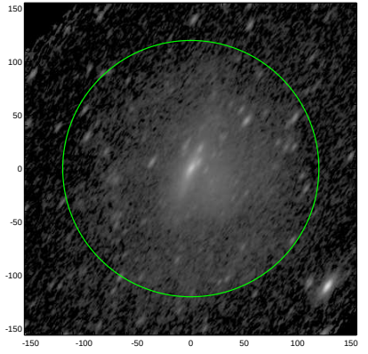
S4G: pa,inc= 55.7 67.1
