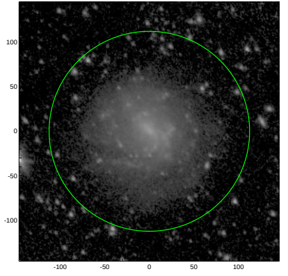
S4G: pa,inc= 126.2 39.4
