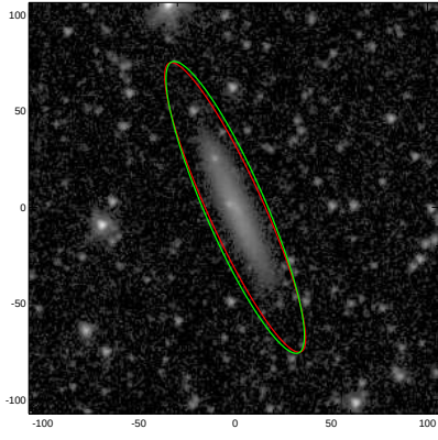
PGC053764
