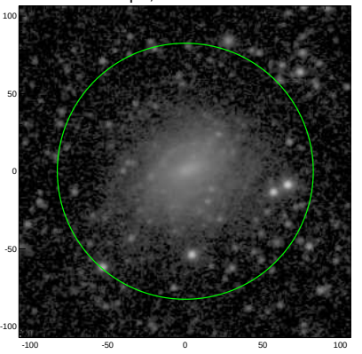
S4G: pa,inc= 14.3 27.6
