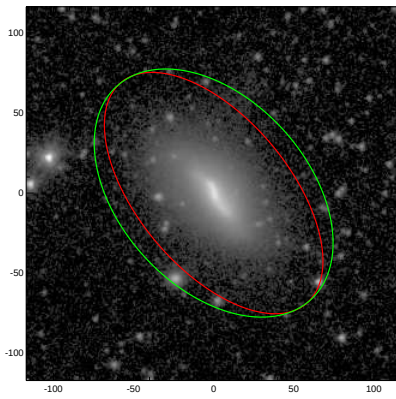
PGC013821
