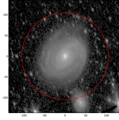
LEDA: pa,inc= 107.9 54.4
