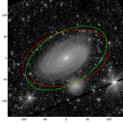
PGC047721
