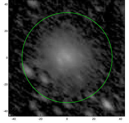
S4G: pa,inc= 138.0 60.4
