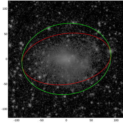
PGC012981
