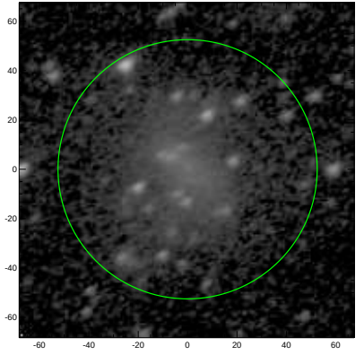
S4G: pa,inc= 28.6 45.8
