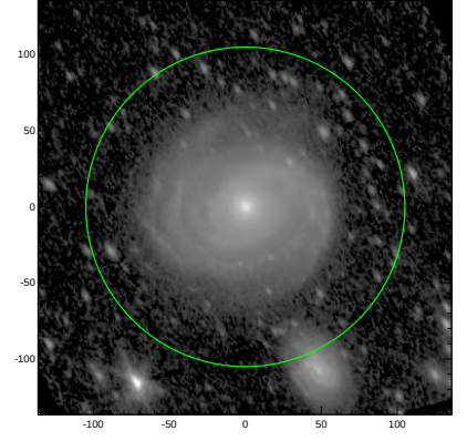
S4G: pa,inc= 121.0 54.9
