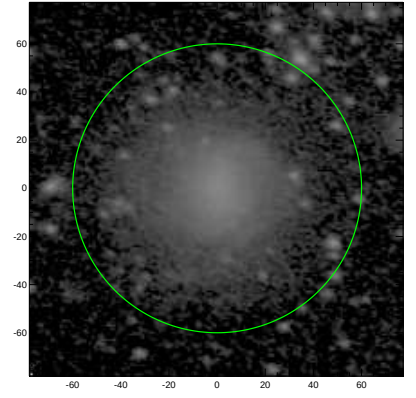
S4G: pa,inc= -15.5 45.9
