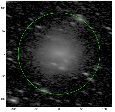
S4G: pa,inc= -14.3 69.3
