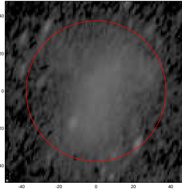
LEDA: pa,inc= 68.5 65.1
