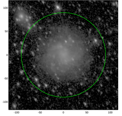
S4G: pa,inc= 121.7 43.0
