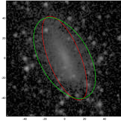
PGC016090
