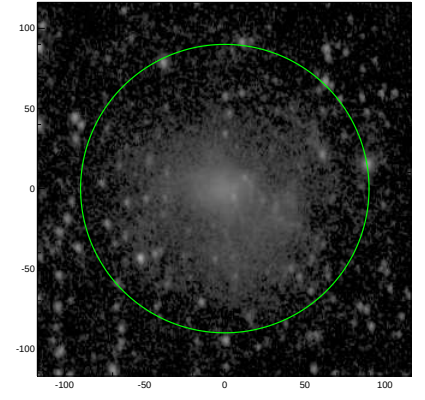
S4G: pa,inc= 99.8 38.3
