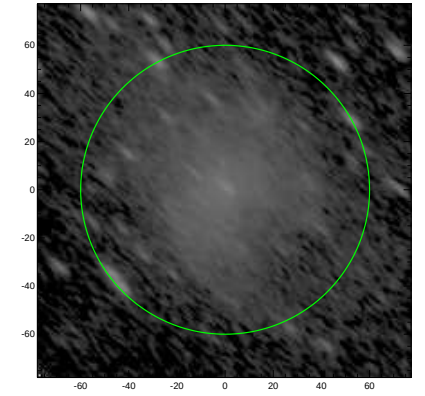
S4G: pa,inc= 137.5 68.6
