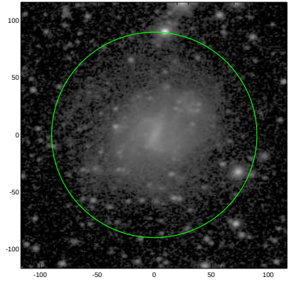
S4G: pa,inc= 8.9 37.6
