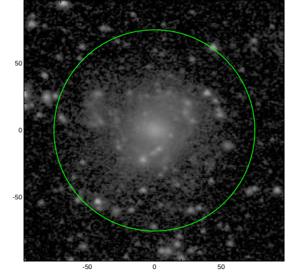
S4G: pa,inc= -0.6 29.8
