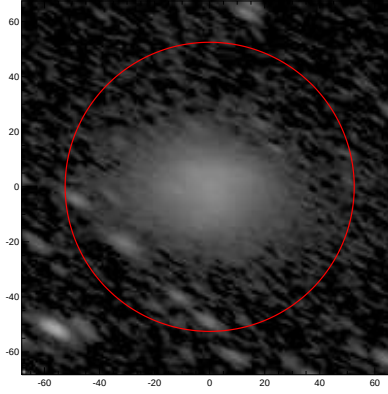
LEDA: pa,inc= 150.5 66.6
