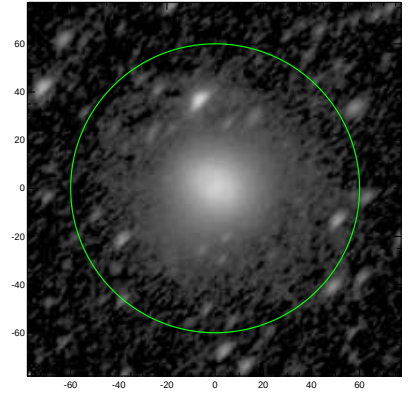
S4G: pa,inc= 47.3 58.2
