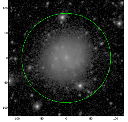
S4G: pa,inc= 22.1 18.1
