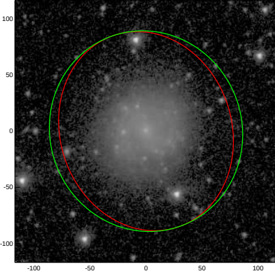
PGC011367
