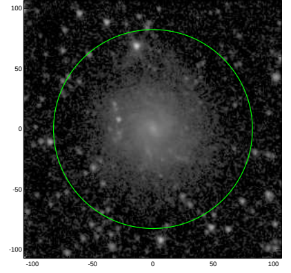
S4G: pa,inc= 125.2 18.3
