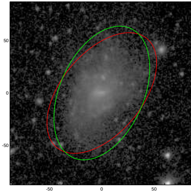
PGC012664
