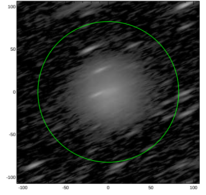
S4G: pa,inc= 23.5 79.0
