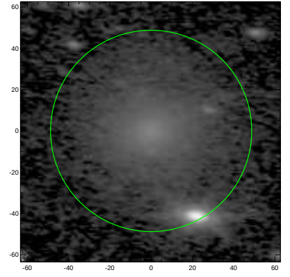
S4G: pa,inc= -7.9 61.0
