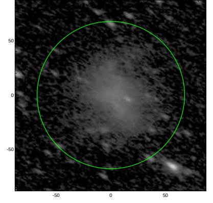
S4G: pa,inc= 152.1 61.6
