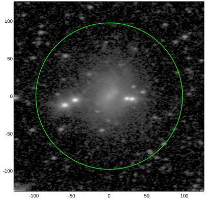
S4G: pa,inc= 5.1 52.1
