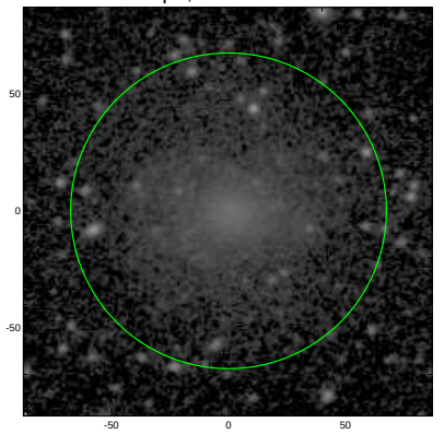
S4G: pa,inc= 5.7 25.3
