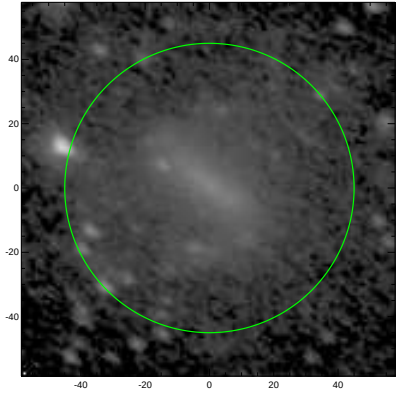
S4G: pa,inc= 147.2 49.0
