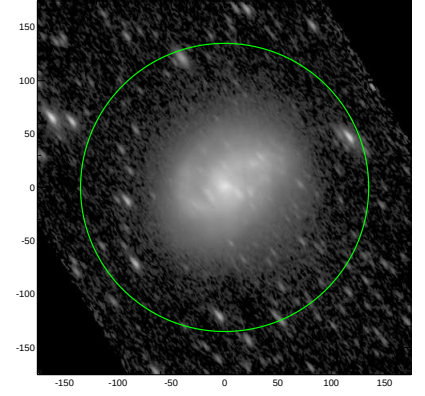
S4G: pa,inc= 126.7 66.1
