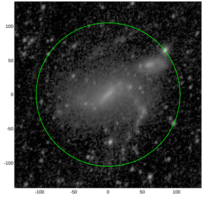
S4G: pa,inc= 56.5 40.6
