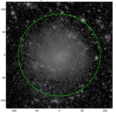
S4G: pa,inc= 140.9 26.0
