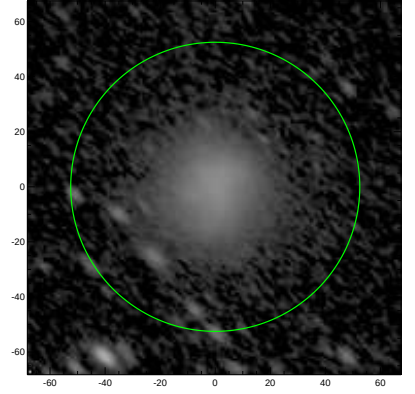
S4G: pa,inc= 139.6 60.0
