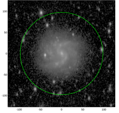
S4G: pa,inc= 90.9 49.2
