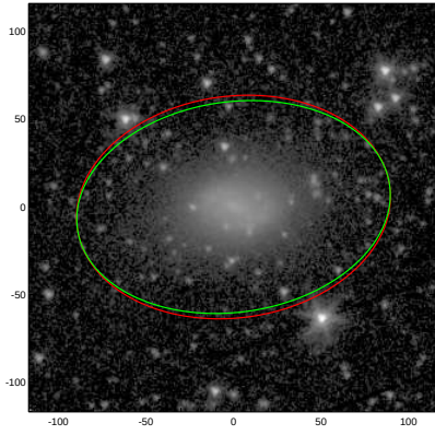
PGC053779
