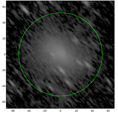
S4G: pa,inc= 131.8 72.4
