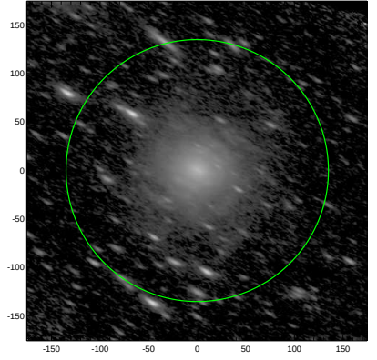
S4G: pa,inc= 151.7 69.4
