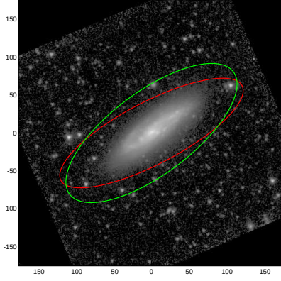
PGC045877
