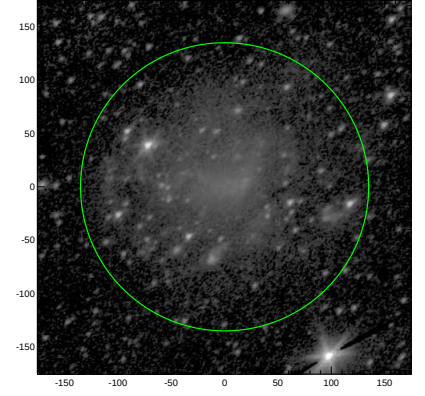
S4G: pa,inc= 39.6 48.2
