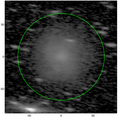
S4G: pa,inc= -10.4 72.5
