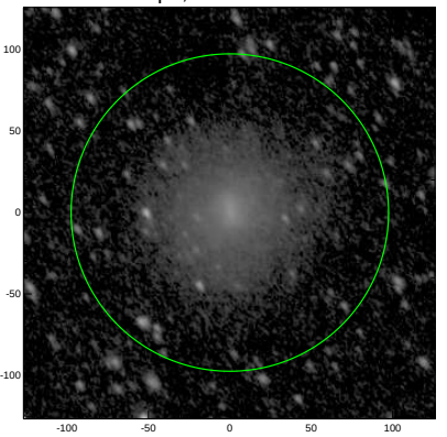
S4G: pa,inc= 126.1 50.5
