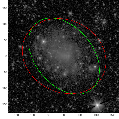
PGC045195
