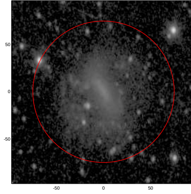
LEDA: pa,inc= 95.0 40.2
