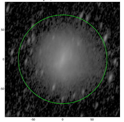
S4G: pa,inc= 72.9 67.6
