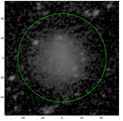
S4G: pa,inc= 30.3 40.2
