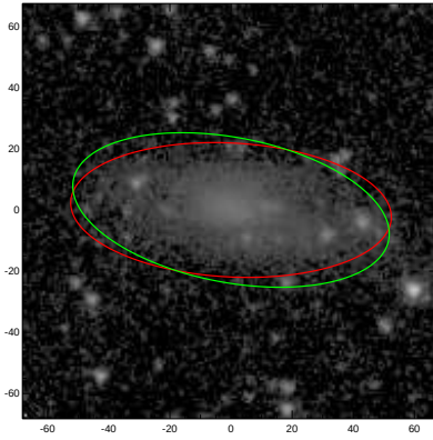
PGC053568
