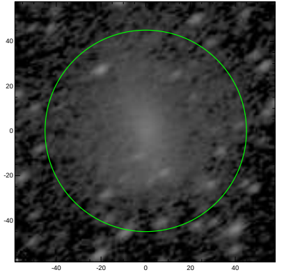
S4G: pa,inc= 30.3 57.0
