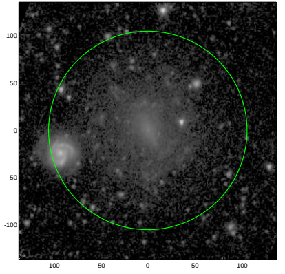
S4G: pa,inc= 91.9 25.8
