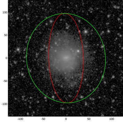
PGC027833
