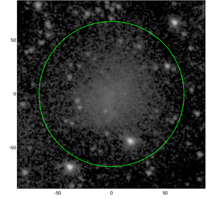
S4G: pa,inc= 160.1 27.1
