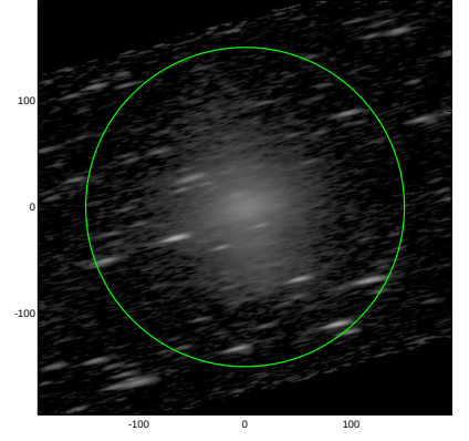
S4G: pa,inc= 13.9 79.7
