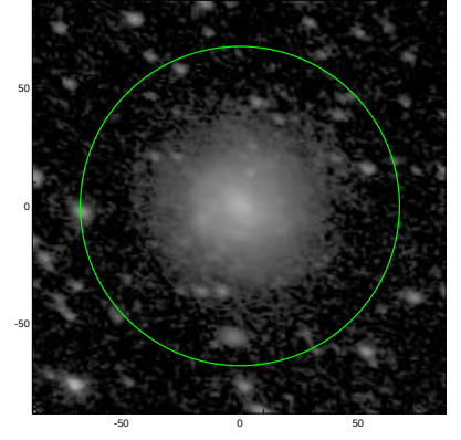
S4G: pa,inc= 155.3 46.2
