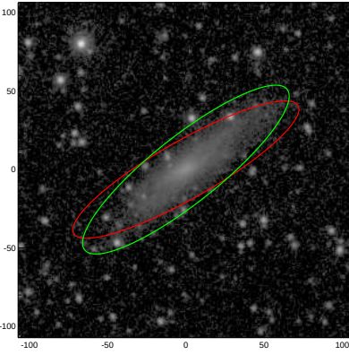
PGC053634
