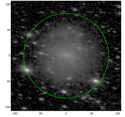
S4G: pa,inc= -13.5 58.0
