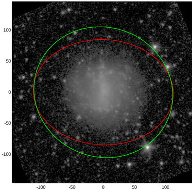
PGC048179
