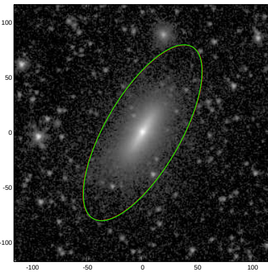
PGC053724
