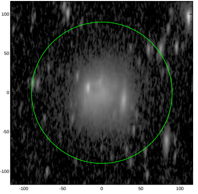
S4G: pa,inc= 89.0 72.0
