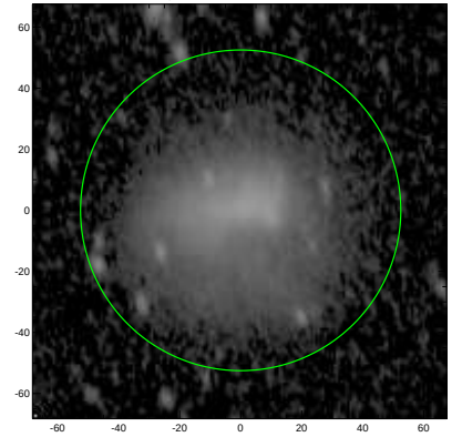
S4G: pa,inc= 101.7 54.4
