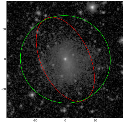
PGC011677
