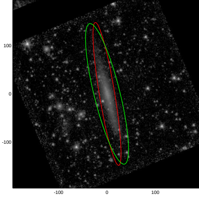
PGC029086
