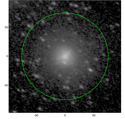
S4G: pa,inc= 152.5 50.1
