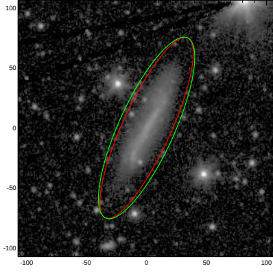
PGC027747
