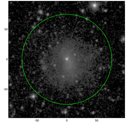
S4G: pa,inc= 68.8 14.8
