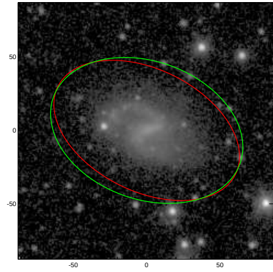
PGC028380
