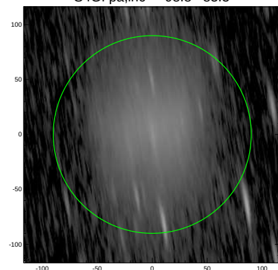
S4G: pa,inc= 98.8 83.3
