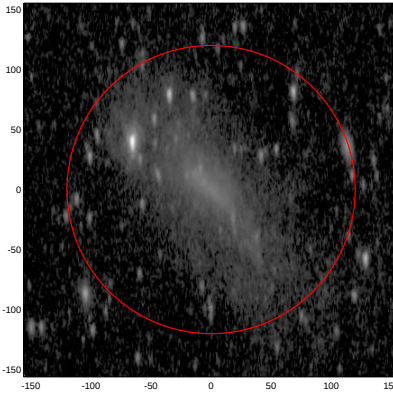
LEDA: pa,inc= 91.5 66.2
