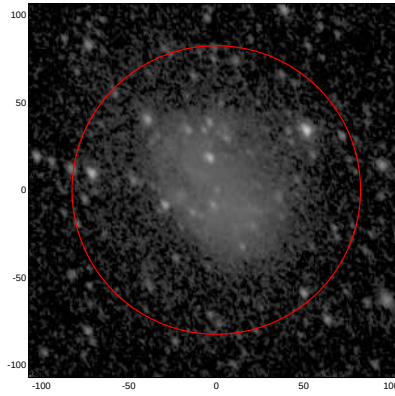
LEDA: pa,inc= 120.0 43.4
