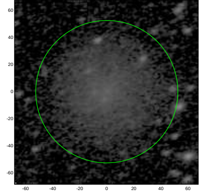
S4G: pa,inc= 15.3 50.6
