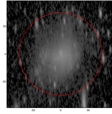
LEDA: pa,inc= 92.0 72.4
