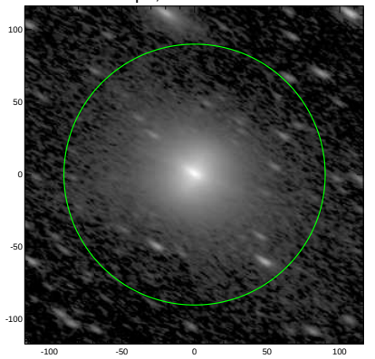
S4G: pa,inc= 150.0 67.6
