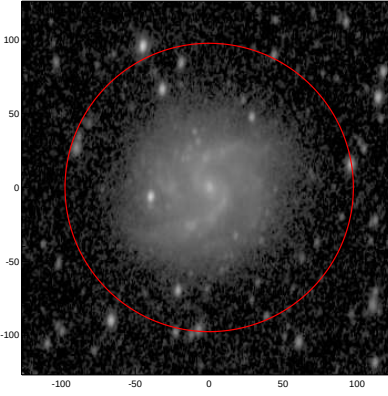
LEDA: pa,inc= 84.7 50.3
