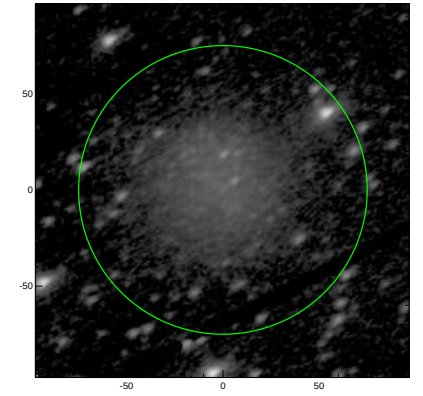
S4G: pa,inc= 32.2 52.4
