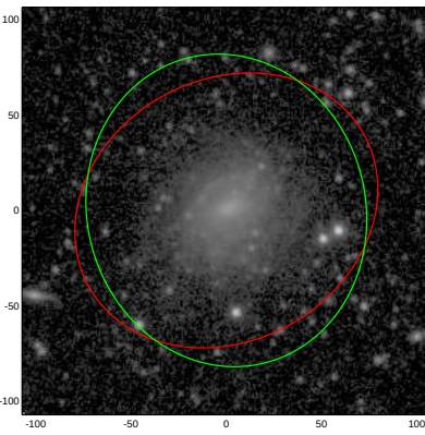
PGC027616
