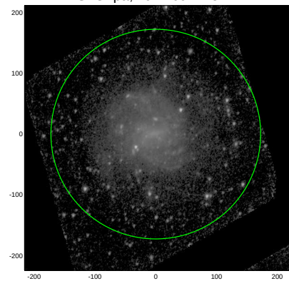
S4G: pa,inc= 69.2 37.4
