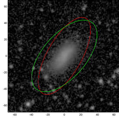
PGC071479
