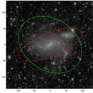
PGC053134
