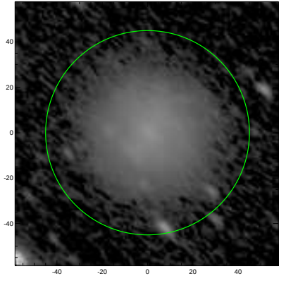
S4G: pa,inc= 138.6 62.0
