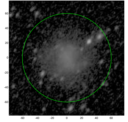
S4G: pa,inc= 54.4 51.3
