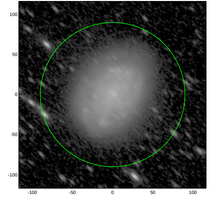
S4G: pa,inc= 137.3 65.0
