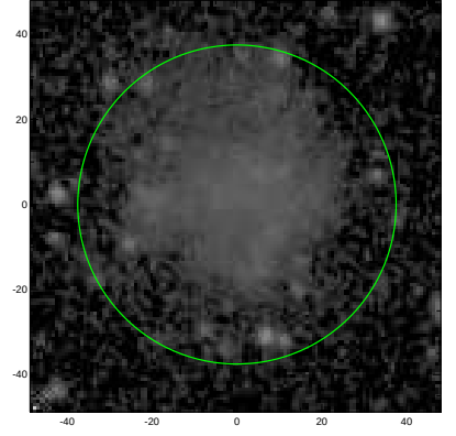
S4G: pa,inc= 126.6 24.5
