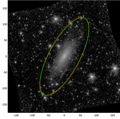
PGC027810
