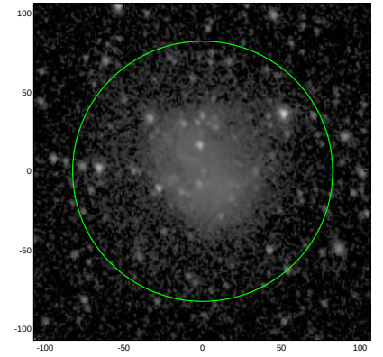
S4G: pa,inc= 105.6 32.5
