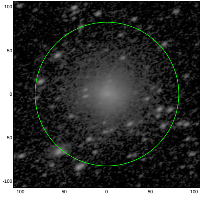
S4G: pa,inc= 27.2 53.3
