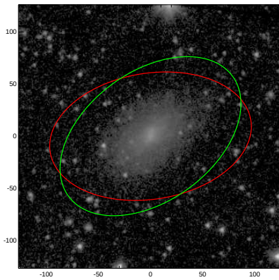
PGC015869
