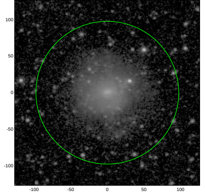
S4G: pa,inc= 8.8 27.8
