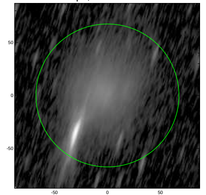
S4G: pa,inc= 72.7 78.6
