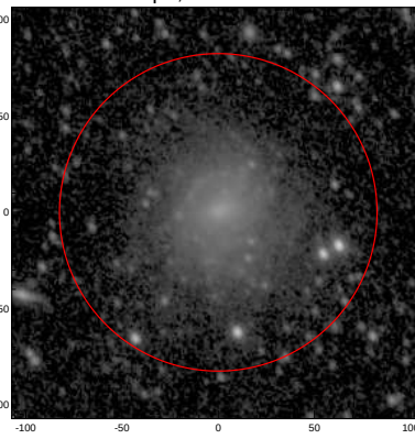
LEDA: pa,inc= 118.8 33.7
