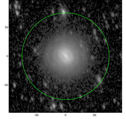
S4G: pa,inc= 103.4 54.7
