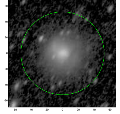
S4G: pa,inc= 58.6 57.3
