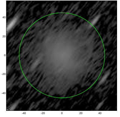
S4G: pa,inc= 50.6 75.4
