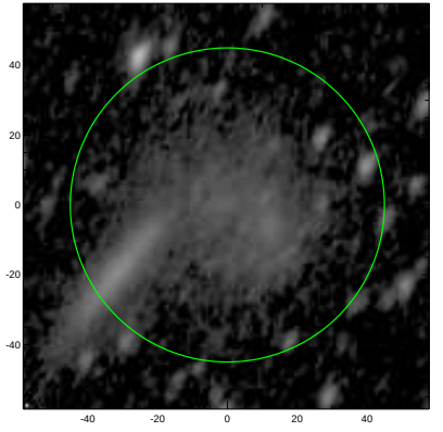
S4G: pa,inc= 67.1 55.7
