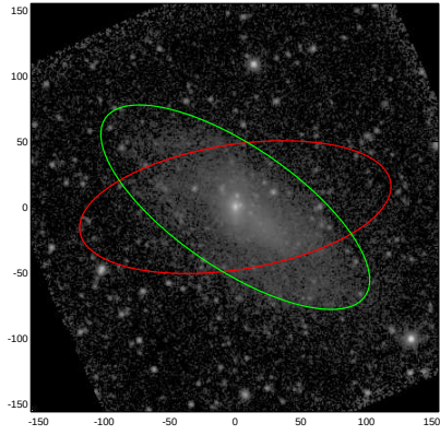
PGC041965
