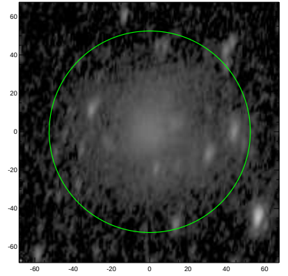
S4G: pa,inc= 79.2 63.2
