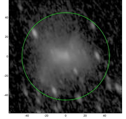
S4G: pa,inc= 112.9 62.2
