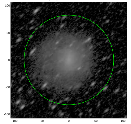
S4G: pa,inc= 41.1 62.4
