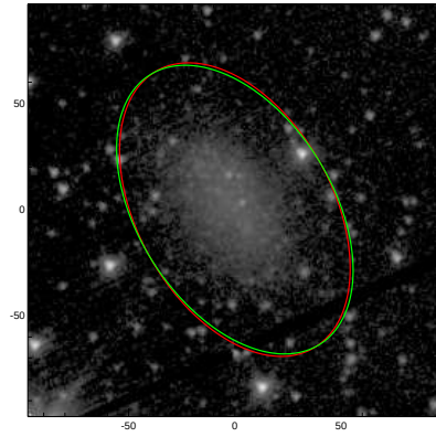
PGC044982
