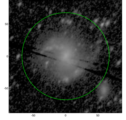
S4G: pa,inc= 55.2 52.3
