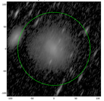
S4G: pa,inc= 64.1 73.1
