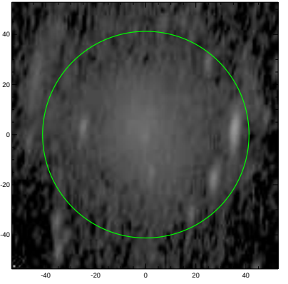
S4G: pa,inc= 83.2 68.4
