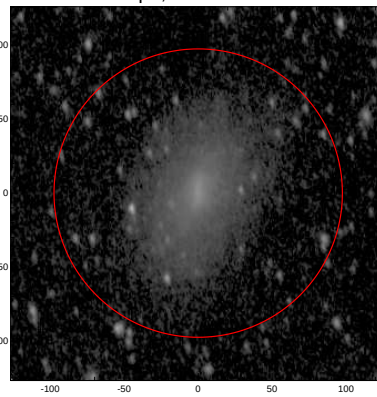
LEDA: pa,inc= 999.0 51.7
