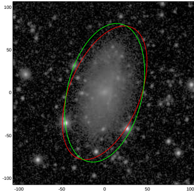
PGC013684
