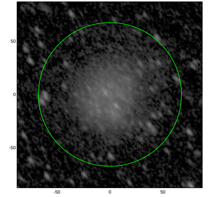
S4G: pa,inc= 127.7 56.5
