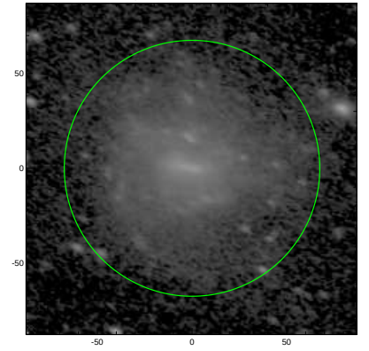
S4G: pa,inc= 156.1 53.6
