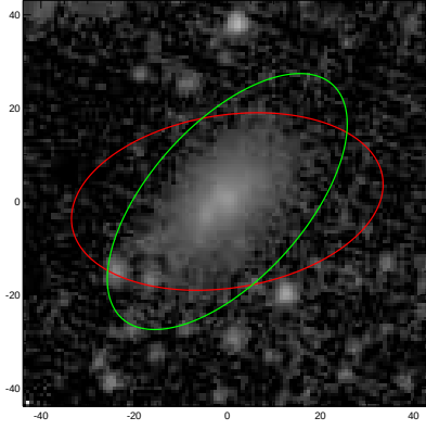
PGC010813
