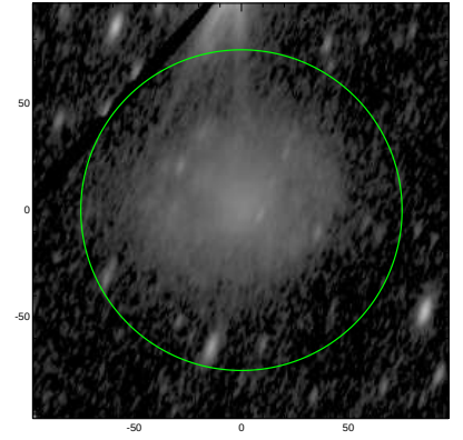
S4G: pa,inc= 70.4 66.8
