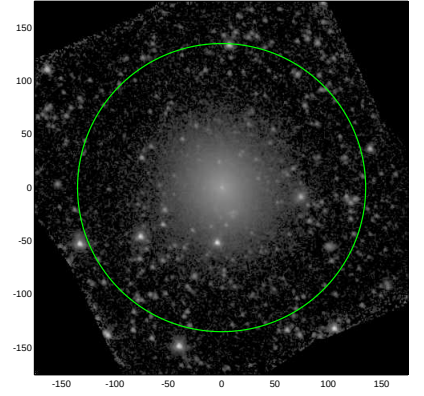
S4G: pa,inc= 144.3 19.3
