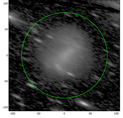
S4G: pa,inc= 155.5 73.7
