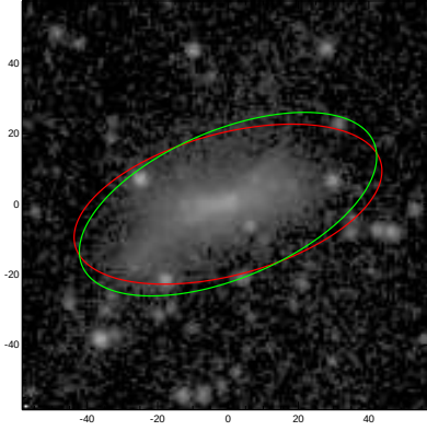
PGC051291
