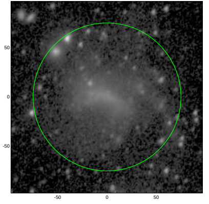
S4G: pa,inc= 67.1 36.4
