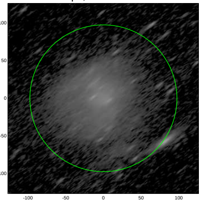
S4G: pa,inc= 36.5 74.5
