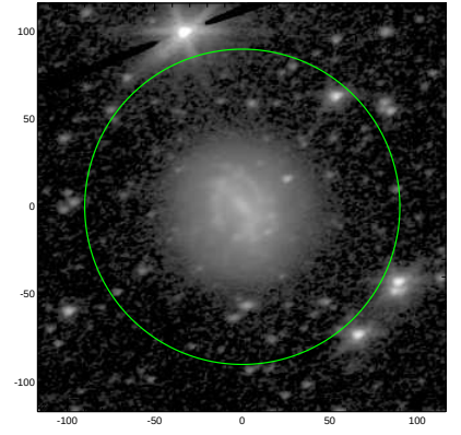
S4G: pa,inc= 20.7 46.5
