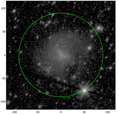
S4G: pa,inc= 47.8 31.2
