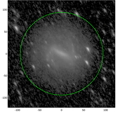
S4G: pa,inc= 124.3 63.6
