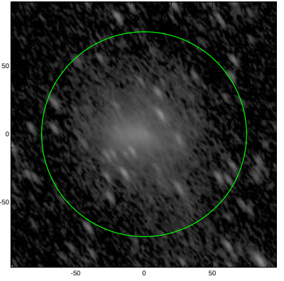
S4G: pa,inc= 125.2 67.6
