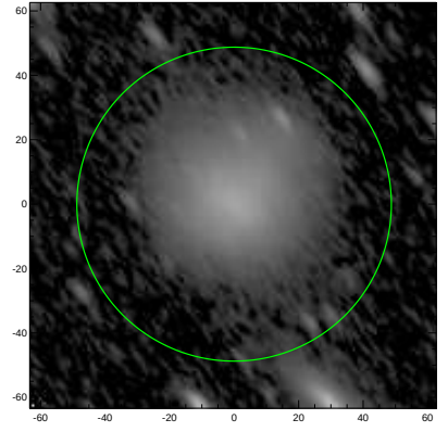
S4G: pa,inc= 127.0 67.9
