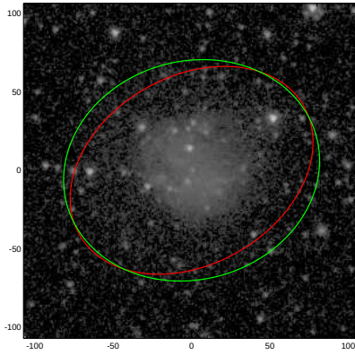
PGC046382
