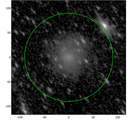
S4G: pa,inc= 128.3 62.2
