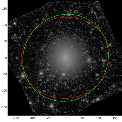
PGC029300
