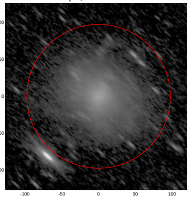
LEDA: pa,inc= 138.3 72.5
