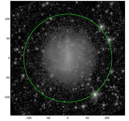
S4G: pa,inc= 68.9 22.2
