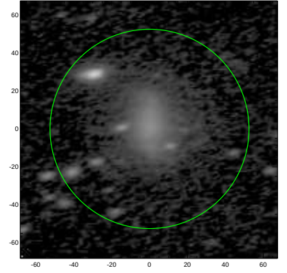
S4G: pa,inc= 12.4 60.5
