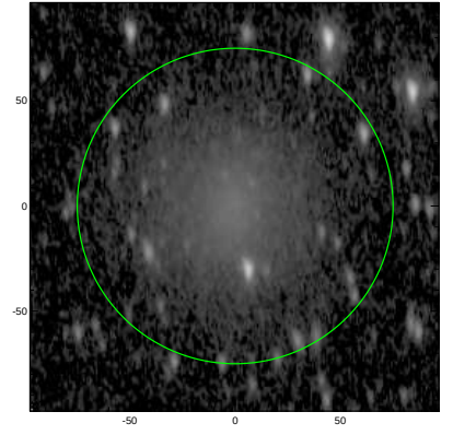
S4G: pa,inc= 94.3 61.1
