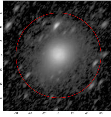
LEDA: pa,inc= 50.0 64.4
