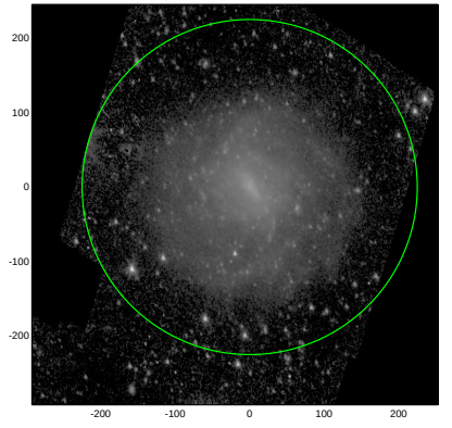
S4G: pa,inc= 106.4 41.7
