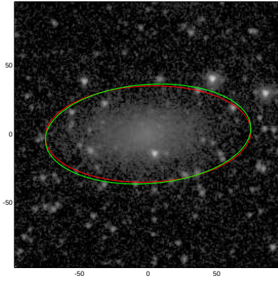
PGC041743
