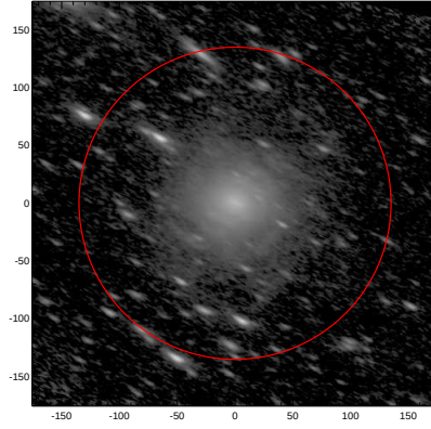
LEDA: pa,inc= 152.7 68.7
