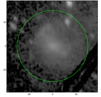
S4G: pa,inc= 108.7 38.0
