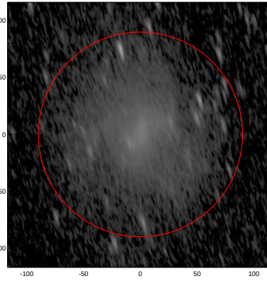
LEDA: pa,inc= 106.5 74.6
