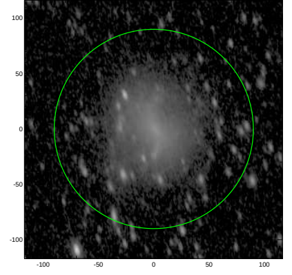
S4G: pa,inc= 104.1 59.5
