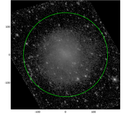
S4G: pa,inc= 139.9 42.5
