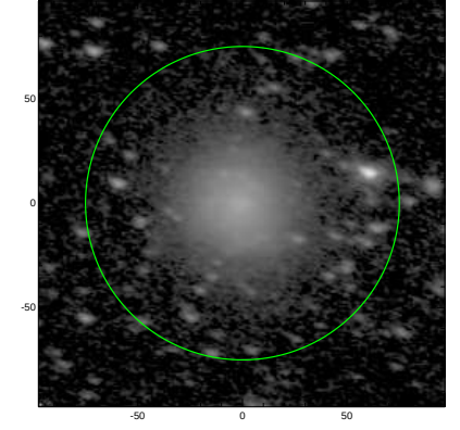
S4G: pa,inc= -14.1 54.5
