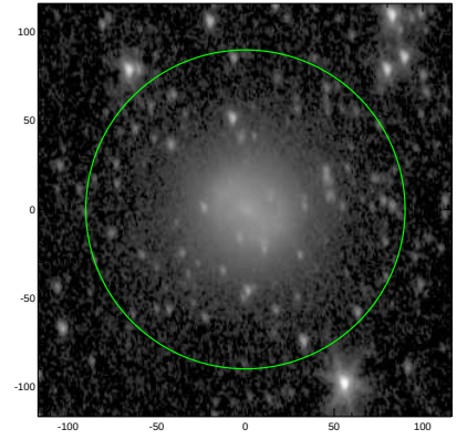
S4G: pa,inc= 98.1 48.1
