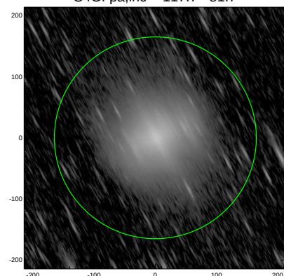
S4G: pa,inc= 117.7 81.7
