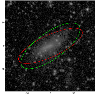
PGC007998
