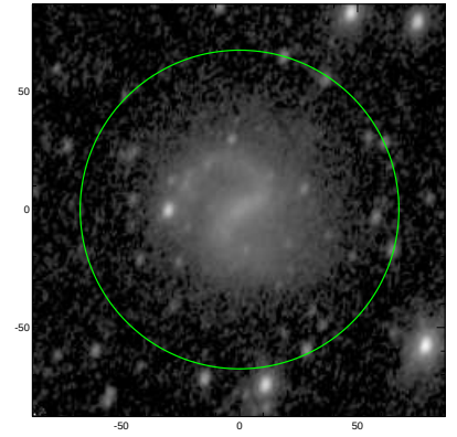
S4G: pa,inc= 70.5 45.9
