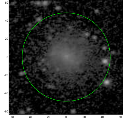
S4G: pa,inc= 9.7 35.6
