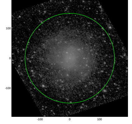
S4G: pa,inc= 152.9 35.6
