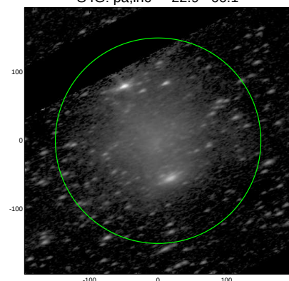
S4G: pa,inc= 22.9 66.1
