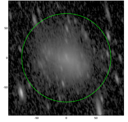
S4G: pa,inc= 103.4 70.5
