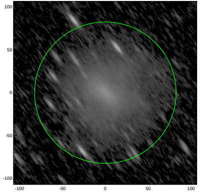
S4G: pa,inc= 128.4 75.1
