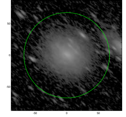
S4G: pa,inc= 138.7 69.0
