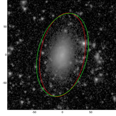
PGC044952
