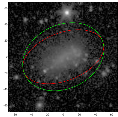
PGC042160
