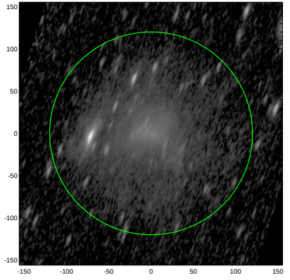
S4G: pa,inc= 68.9 71.2
