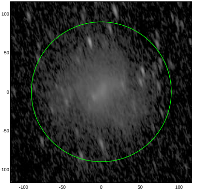
S4G: pa,inc= 107.3 72.0
