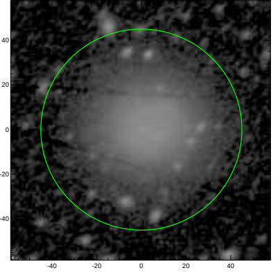
S4G: pa,inc= 35.0 39.9
