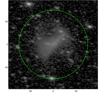
S4G: pa,inc= -9.8 54.2
