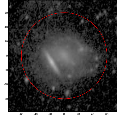
LEDA: pa,inc= 75.6 45.3
