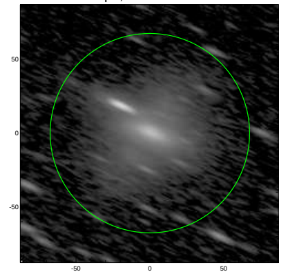
S4G: pa,inc= 156.0 75.1
