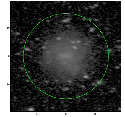
S4G: pa,inc= -3.4 54.6
