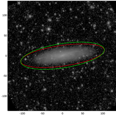
UGC04824
