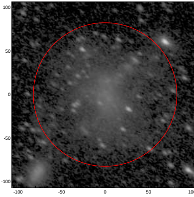
LEDA: pa,inc= 145.0 53.8
