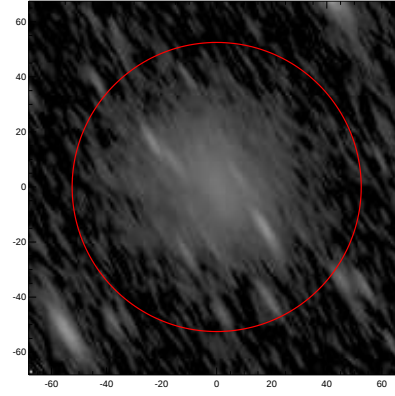
LEDA: pa,inc= 120.4 75.5
