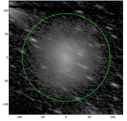
S4G: pa,inc= 155.3 71.7
