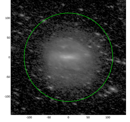
S4G: pa,inc= -19.2 63.5
