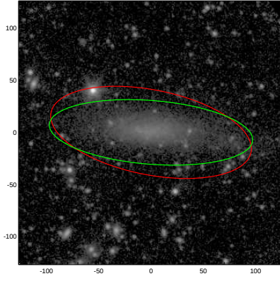
UGC07125
