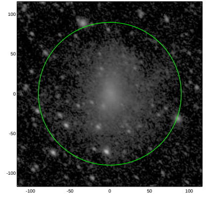
S4G: pa,inc= 139.9 41.6
