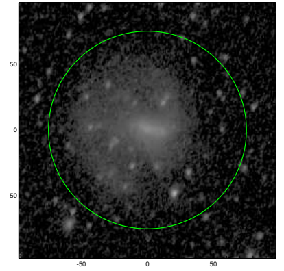
S4G: pa,inc= 68.7 43.8
