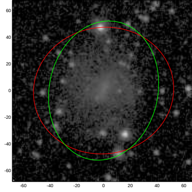
UGC08877
