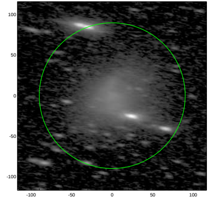
S4G: pa,inc= -8.9 70.3
