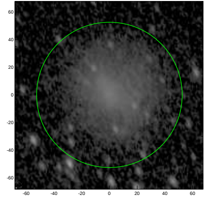
S4G: pa,inc= 110.0 54.1
