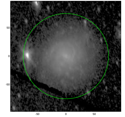
S4G: pa,inc= 103.2 56.3
