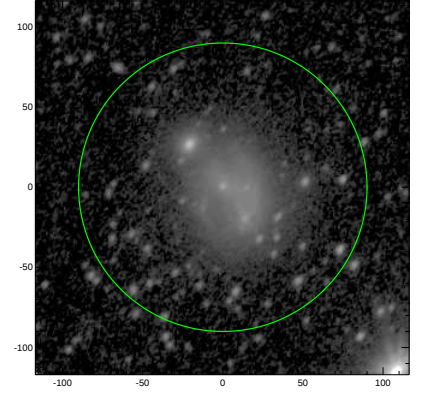
S4G: pa,inc= 55.7 43.7
