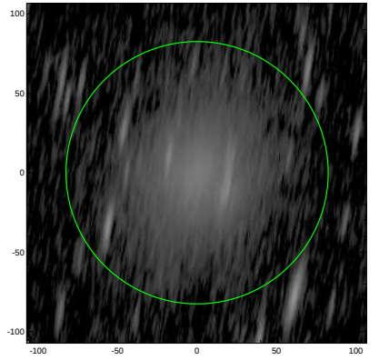
S4G: pa,inc= 80.9 81.7
