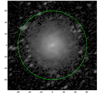
S4G: pa,inc= 34.1 53.0
