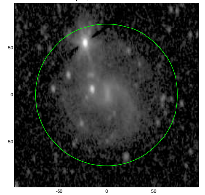
S4G: pa,inc= 92.3 52.5
