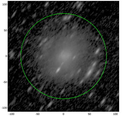
S4G: pa,inc= 53.3 69.9
