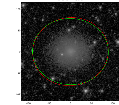
UGC12893
