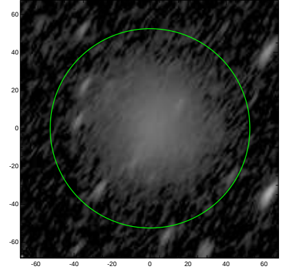
S4G: pa,inc= 57.2 70.6
