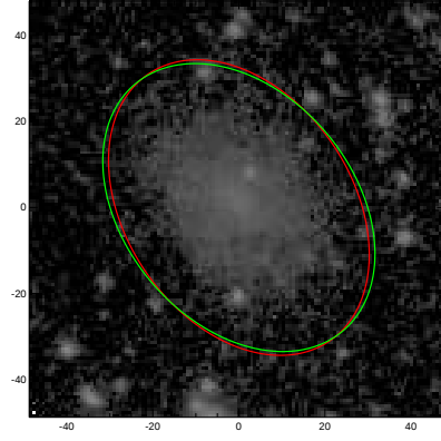
UGC07730
