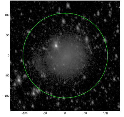
S4G: pa,inc= 104.1 47.1
