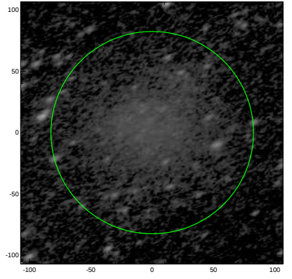
S4G: pa,inc= 26.2 59.6
