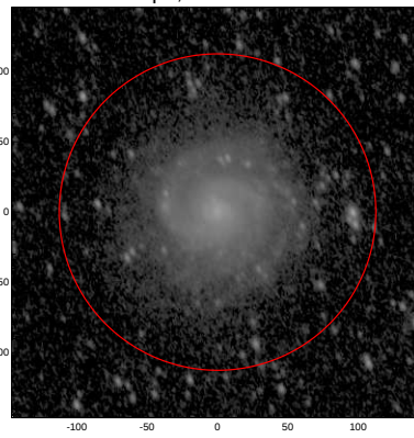
LEDA: pa,inc= 110.4 52.3
