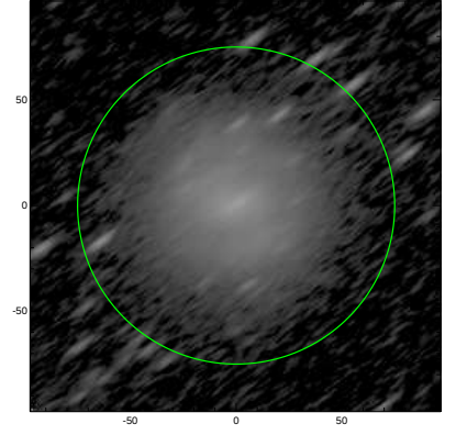
S4G: pa,inc= 36.6 74.6
