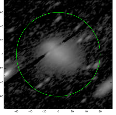
S4G: pa,inc= 38.7 66.9
