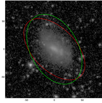
UGC12707
