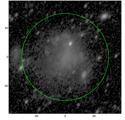
S4G: pa,inc= 57.0 54.0
