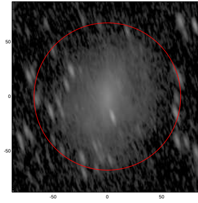
LEDA: pa,inc= 105.8 72.3
