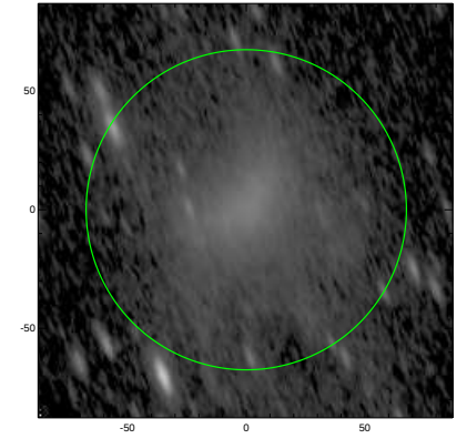
S4G: pa,inc= 109.1 70.2
