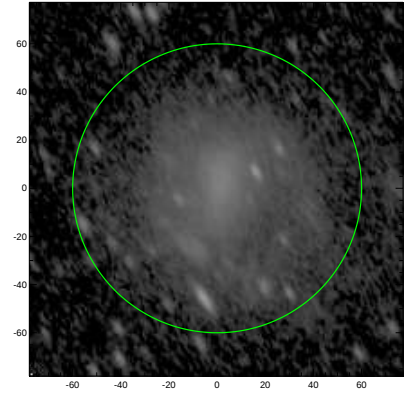
S4G: pa,inc= 117.9 59.4
