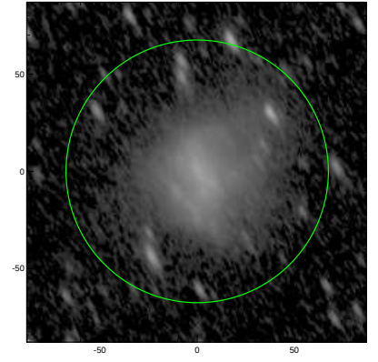
S4G: pa,inc= 119.3 64.9
