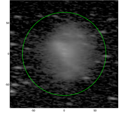
S4G: pa,inc= -4.7 71.2
