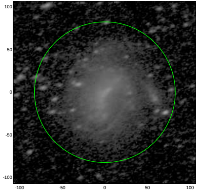
S4G: pa,inc= 21.3 53.6
