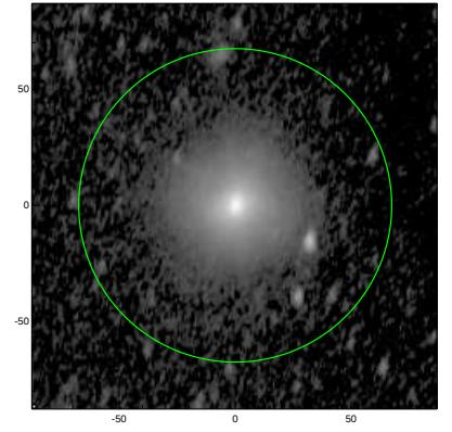
S4G: pa,inc= 77.9 58.5
