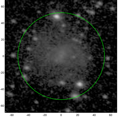
S4G: pa,inc= -11.2 39.3
