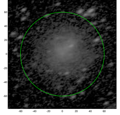
S4G: pa,inc= 25.5 60.0
