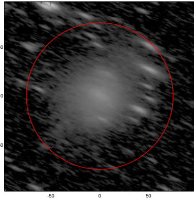
LEDA: pa,inc= 156.0 75.6
