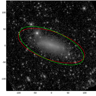
UGC04514
