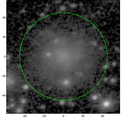
S4G: pa,inc= 20.3 36.3
