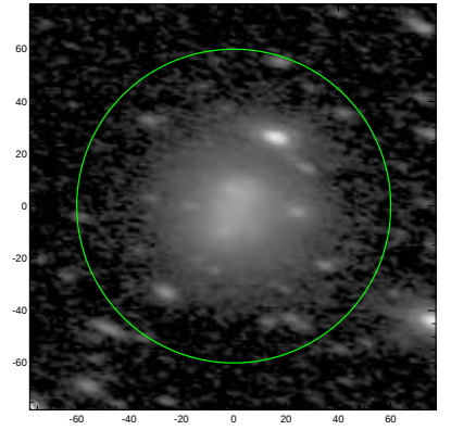
S4G: pa,inc= -12.6 59.0
