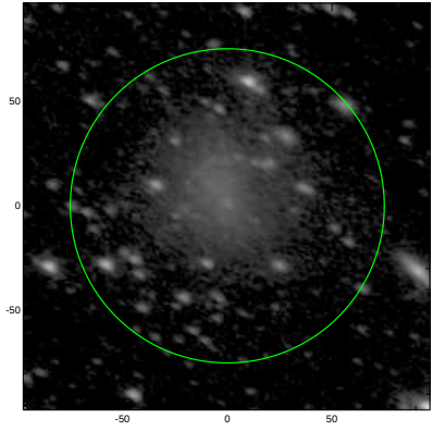
S4G: pa,inc= 151.8 51.7
