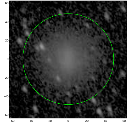
S4G: pa,inc= 120.7 52.5
