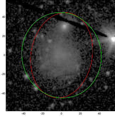
UGC01014
