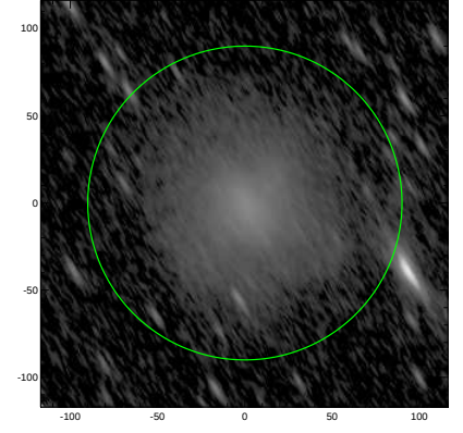
S4G: pa,inc= 120.6 74.7
