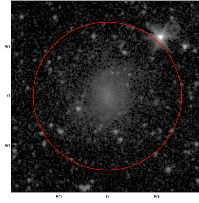
LEDA: pa,inc= 999.0 0.0
