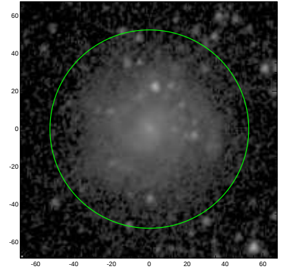
S4G: pa,inc= 68.7 30.6
