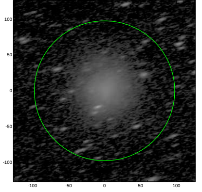
S4G: pa,inc= 15.3 69.4
