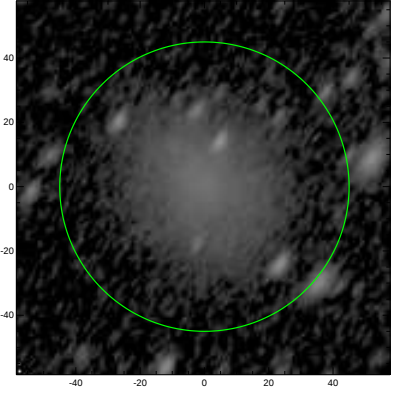
S4G: pa,inc= 57.4 59.2
