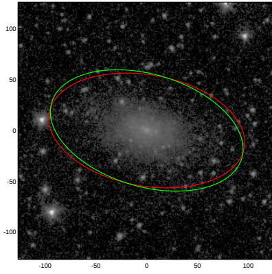
UGC02081
