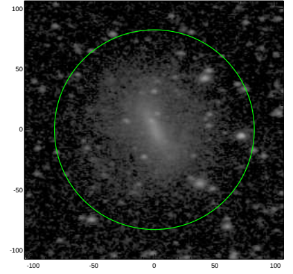
S4G: pa,inc= -2.8 43.3
