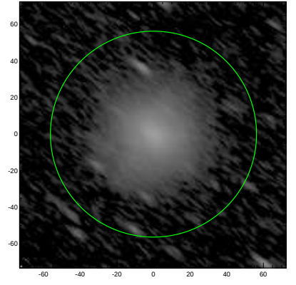
S4G: pa,inc= 141.7 71.5
