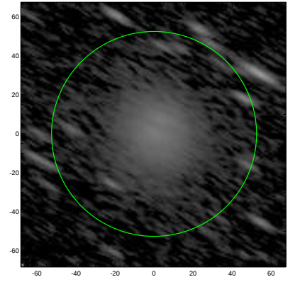
S4G: pa,inc= 150.4 73.7
