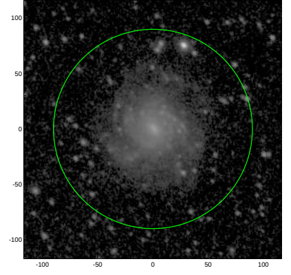
S4G: pa,inc= 123.3 30.6
