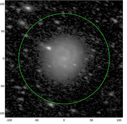
S4G: pa,inc= -18.1 56.6
