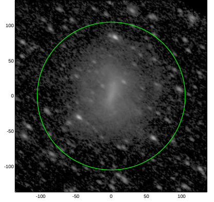
S4G: pa,inc= 141.8 58.0
