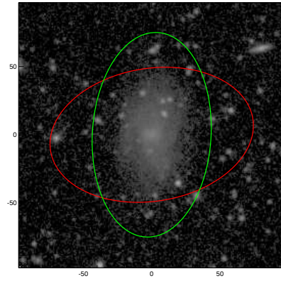
UGC07133
