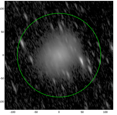
S4G: pa,inc= 111.0 73.7
