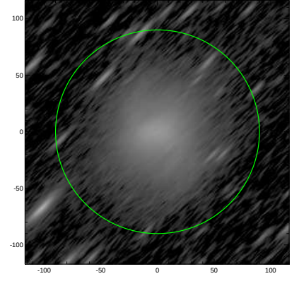
S4G: pa,inc= 44.2 79.7
