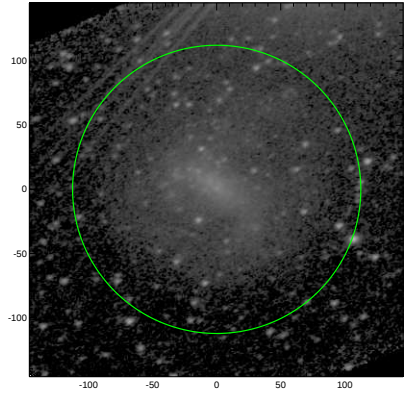
S4G: pa,inc= 23.9 44.0
