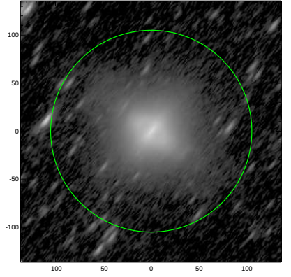
S4G: pa,inc= 50.7 73.5
