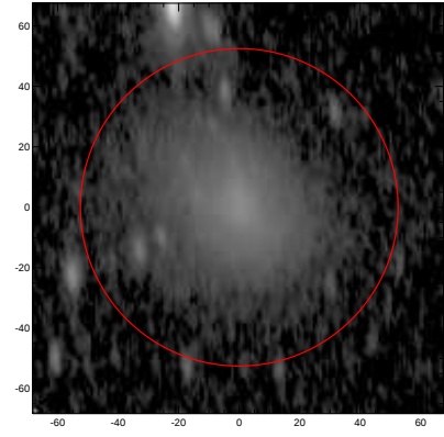
LEDA: pa,inc= 94.8 68.6
