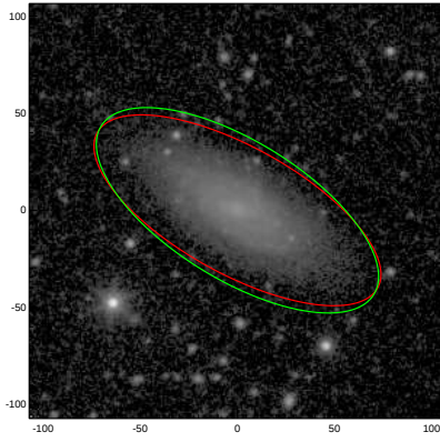
UGC07848
