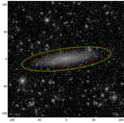
UGC07697
