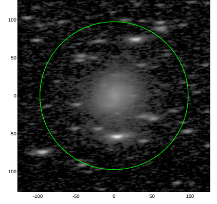
S4G: pa,inc= 4.0 70.3
