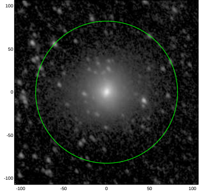
S4G: pa,inc= 124.0 42.6
