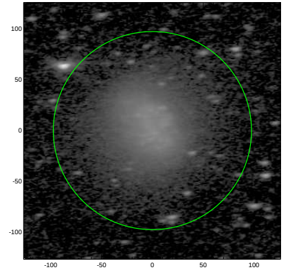
S4G: pa,inc= 3.8 63.6
