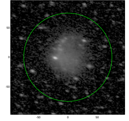
S4G: pa,inc= -15.4 52.3
