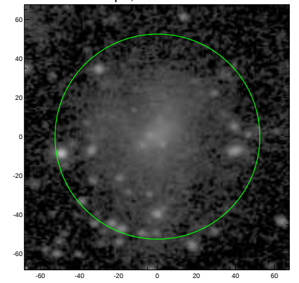
S4G: pa,inc= 4.0 34.2
