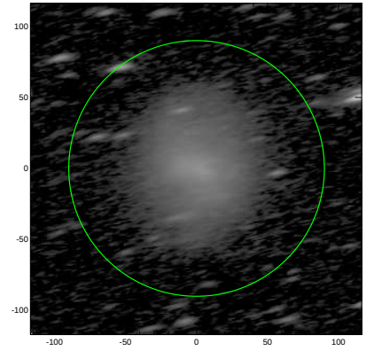
S4G: pa,inc= 13.2 74.3
