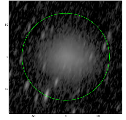
S4G: pa,inc= 73.3 73.6
