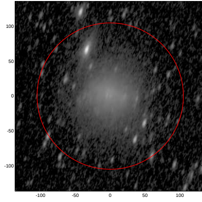
LEDA: pa,inc= 71.2 66.3
