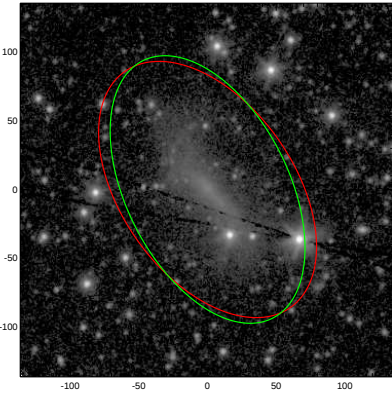
UGC11782
