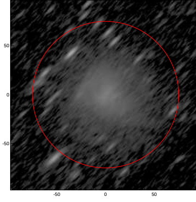
LEDA: pa,inc= 44.2 75.0
