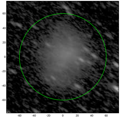
S4G: pa,inc= 146.0 67.2
