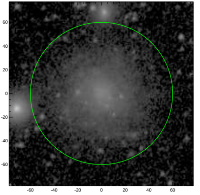
S4G: pa,inc= 65.4 28.6
