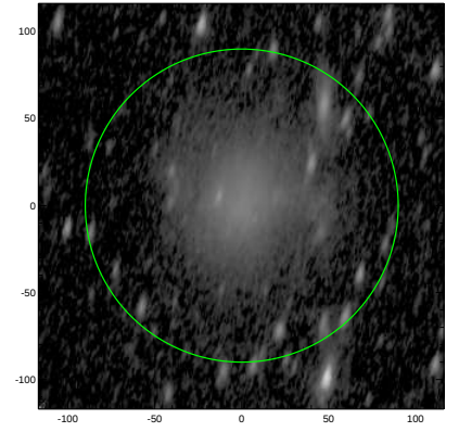
S4G: pa,inc= 76.5 68.1
