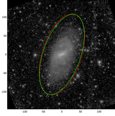
UGC09215
