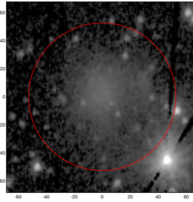
LEDA: pa,inc= 80.0 37.8
