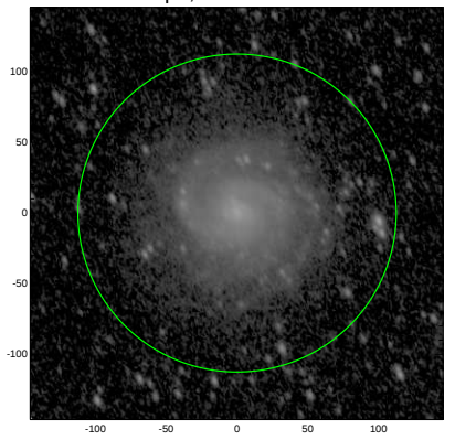
S4G: pa,inc= 114.7 54.1
