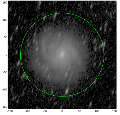
S4G: pa,inc= 72.7 71.1
