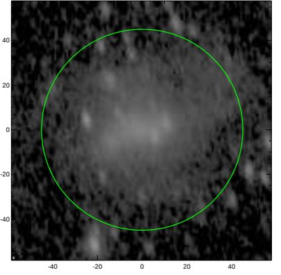
S4G: pa,inc= 100.9 59.5
