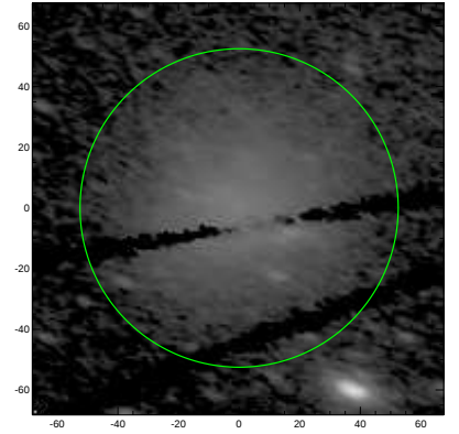
S4G: pa,inc= 160.4 61.2
