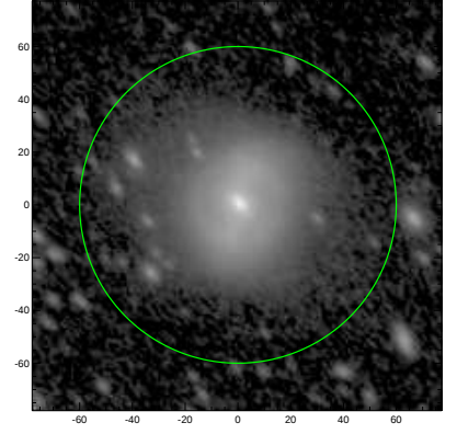
S4G: pa,inc= 133.2 53.2
