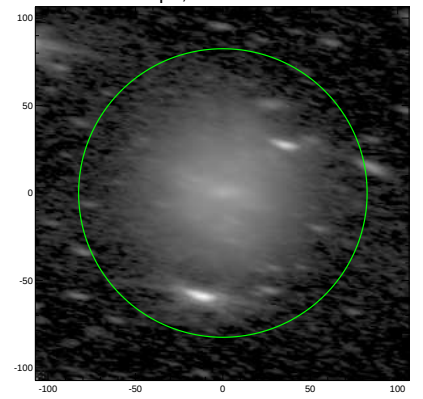
S4G: pa,inc= -12.1 71.8
