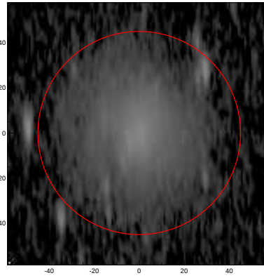
LEDA: pa,inc= 92.9 74.3
