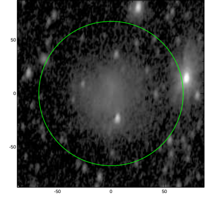
S4G: pa,inc= 81.5 59.2
