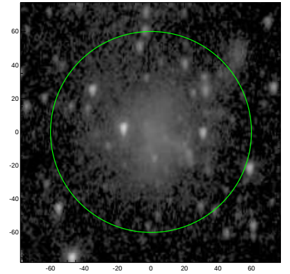
S4G: pa,inc= 87.2 46.5
