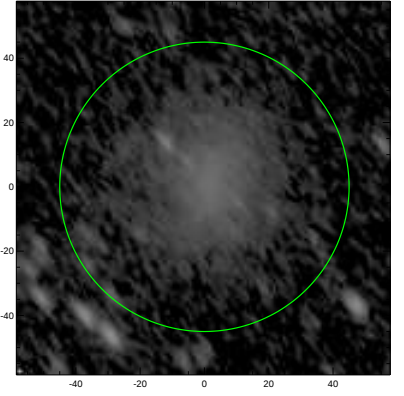
S4G: pa,inc= 126.1 63.3
