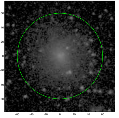
S4G: pa,inc= 39.3 21.3
