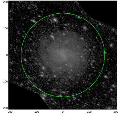
S4G: pa,inc= 142.7 46.8
