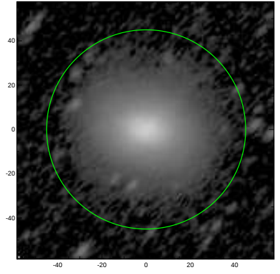
S4G: pa,inc= 45.9 61.3
