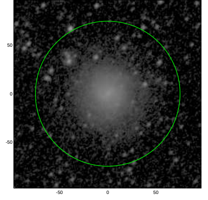
S4G: pa,inc= 57.5 34.8
