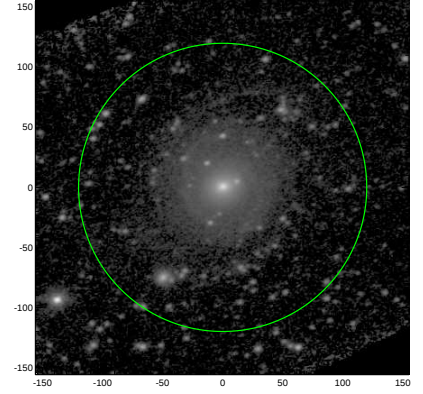
S4G: pa,inc= 15.1 37.1
