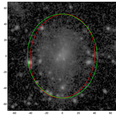
UGC04543
