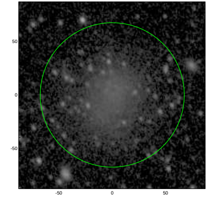
S4G: pa,inc= 113.8 33.9
