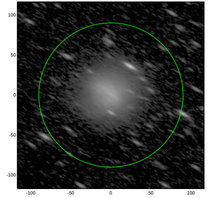
S4G: pa,inc= 150.4 71.5
