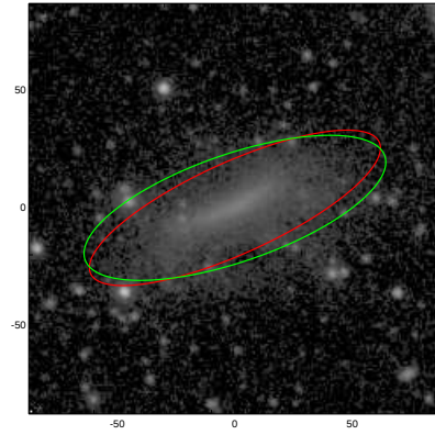
UGC08365
