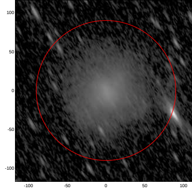
LEDA: pa,inc= 120.1 72.6
