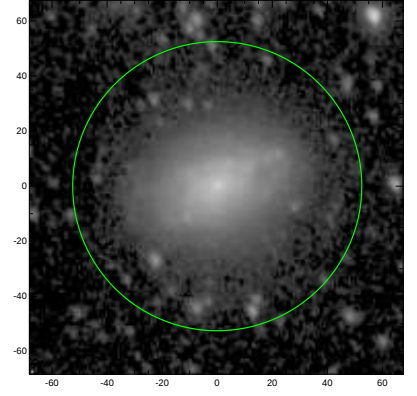
S4G: pa,inc= 107.9 37.5
