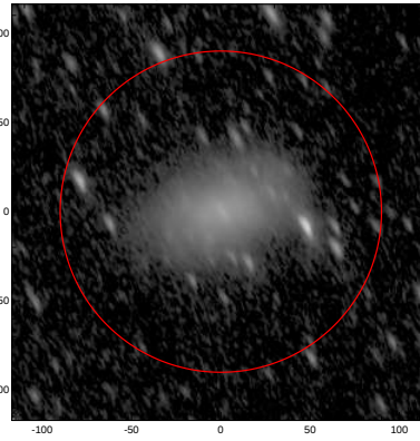
LEDA: pa,inc= 115.3 66.5
