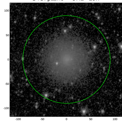
S4G: pa,inc= 87.2 29.7
