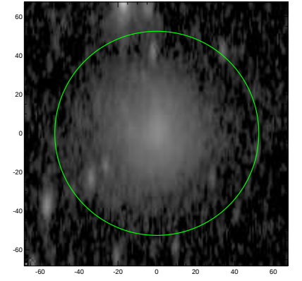
S4G: pa,inc= 88.7 71.0
