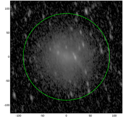
S4G: pa,inc= 101.1 64.6
