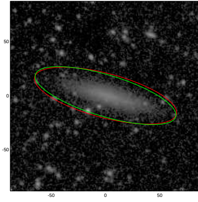
UGC04628
