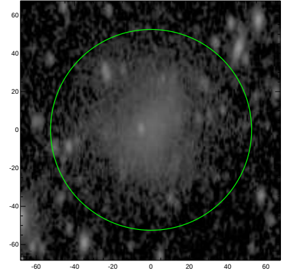
S4G: pa,inc= 89.1 56.8
