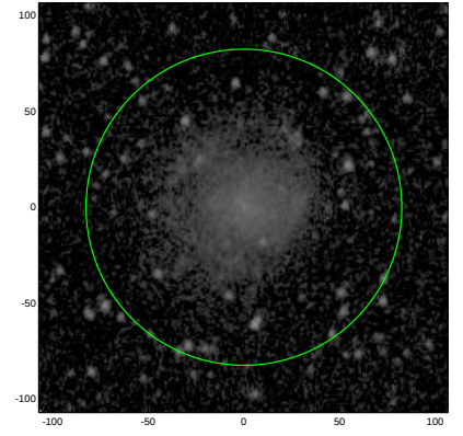
S4G: pa,inc= 86.9 32.4
