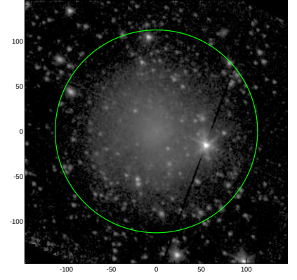
S4G: pa,inc= 130.0 26.2
