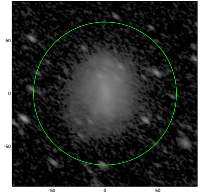
S4G: pa,inc= 142.7 59.8
