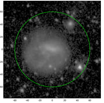
S4G: pa,inc= 103.2 28.6
