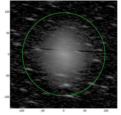
S4G: pa,inc= -9.4 75.9
