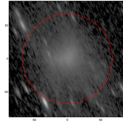
LEDA: pa,inc= 114.5 73.3
