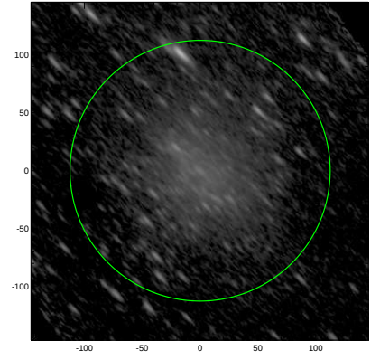
S4G: pa,inc= 134.0 71.1
