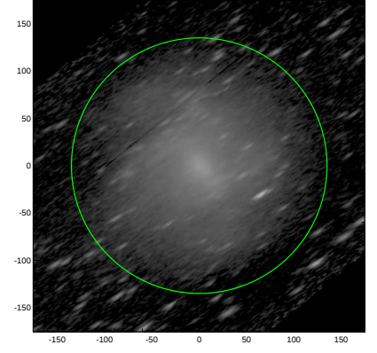
S4G: pa,inc= 34.2 74.0
