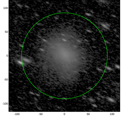
S4G: pa,inc= 154.3 67.2
