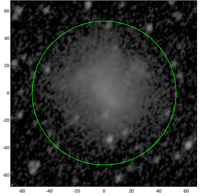
S4G: pa,inc= 64.5 46.3
