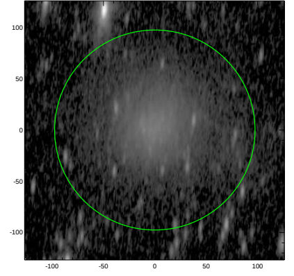
S4G: pa,inc= 85.4 71.8
