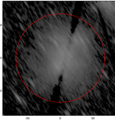
LEDA: pa,inc= 123.5 76.9
