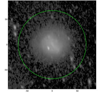
S4G: pa,inc= 103.9 58.6
