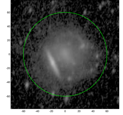
S4G: pa,inc= 76.3 55.3
