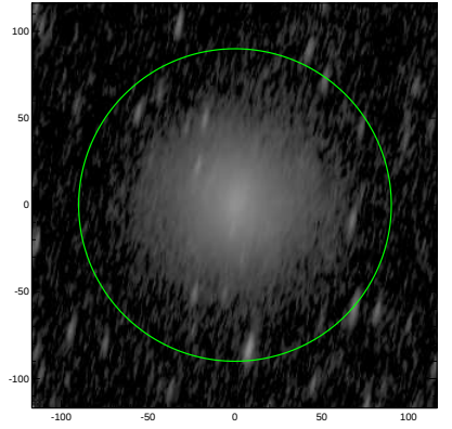
S4G: pa,inc= 77.1 75.6
