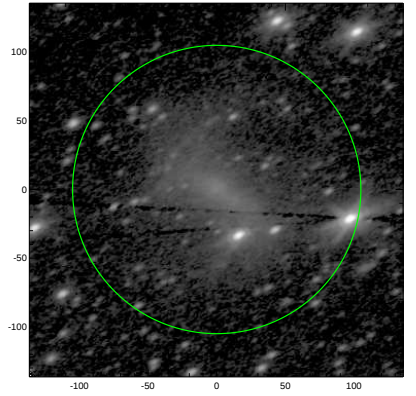
S4G: pa,inc= 26.8 55.7
