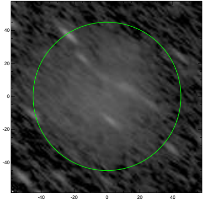
S4G: pa,inc= 141.4 72.5
