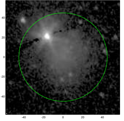
S4G: pa,inc= 114.4 35.5
