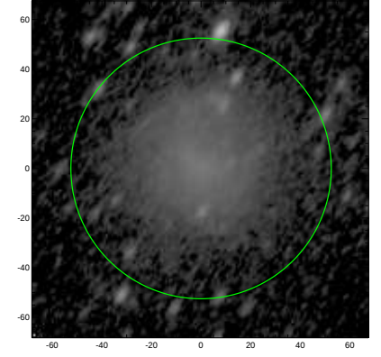
S4G: pa,inc= 55.3 58.6
