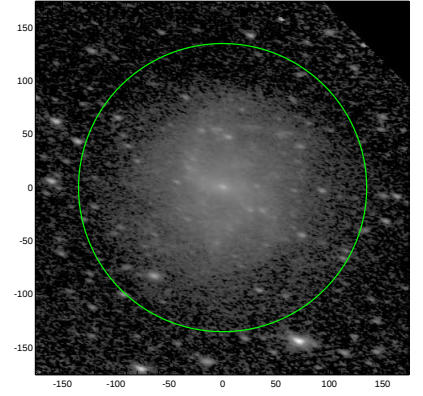
S4G: pa,inc= -16.3 59.5
