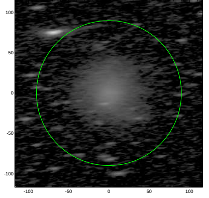
S4G: pa,inc= 5.7 75.3
