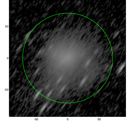
S4G: pa,inc= 54.0 75.5
