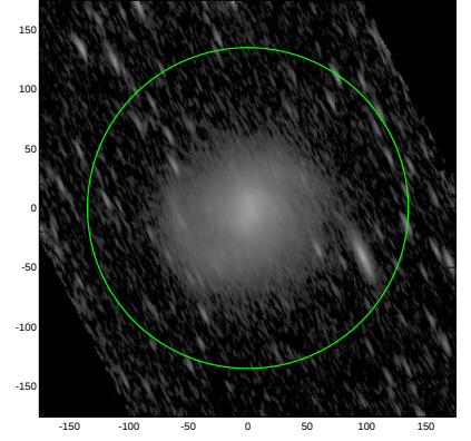
S4G: pa,inc= 114.8 75.7
