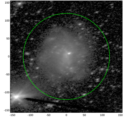
S4G: pa,inc= 10.8 54.9
