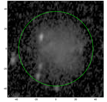
S4G: pa,inc= 79.7 51.7
