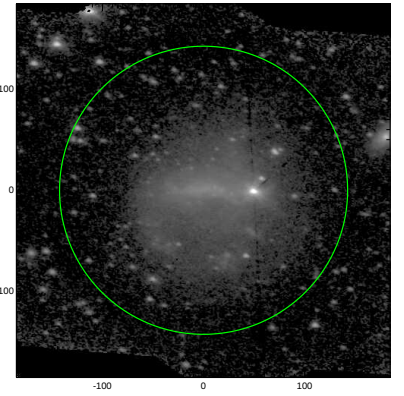
S4G: pa,inc= -13.2 43.1
