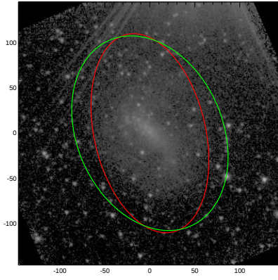
UGC07911
