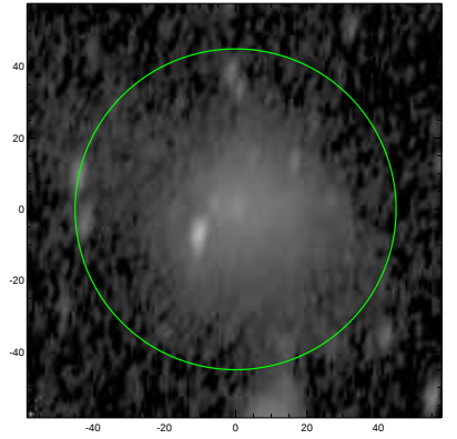
S4G: pa,inc= 80.2 64.6
