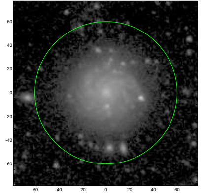
S4G: pa,inc= 147.8 20.8
