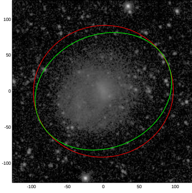
UGC07239
