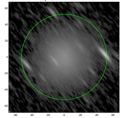
S4G: pa,inc= 129.0 76.0
