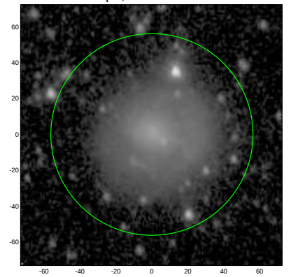
S4G: pa,inc= 100.3 35.3
