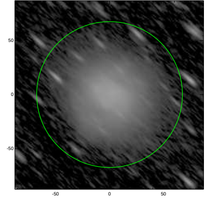
S4G: pa,inc= 137.9 74.8
