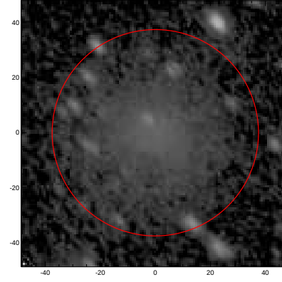
LEDA: pa,inc= 129.4 50.1
