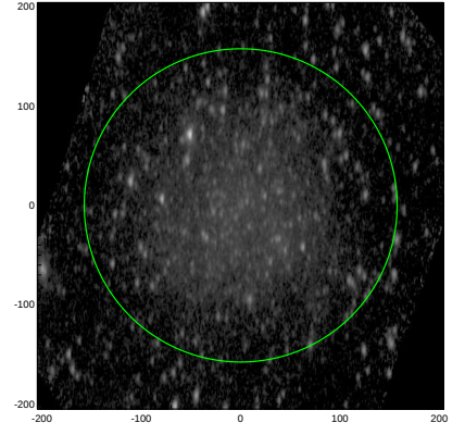
S4G: pa,inc= 88.0 63.3
