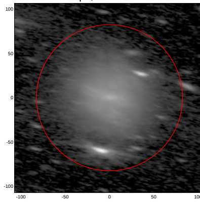
LEDA: pa,inc= 166.8 72.9
