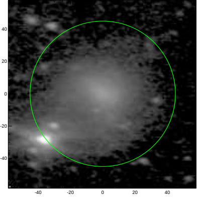
S4G: pa,inc= -7.4 54.8
