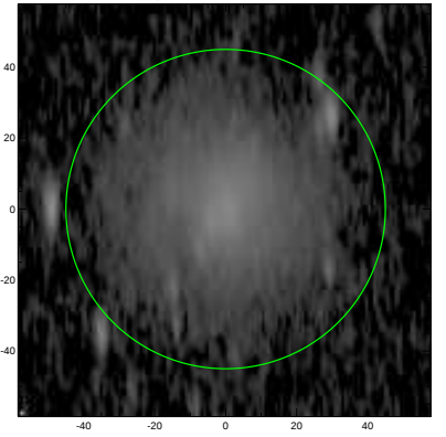
S4G: pa,inc= 92.1 72.4
