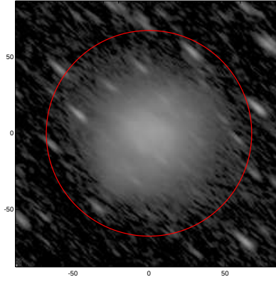
LEDA: pa,inc= 138.6 72.7
