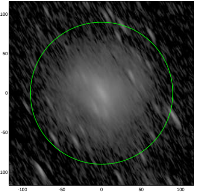
S4G: pa,inc= 118.9 77.9
