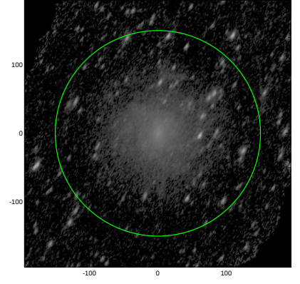
S4G: pa,inc= 59.2 63.0
