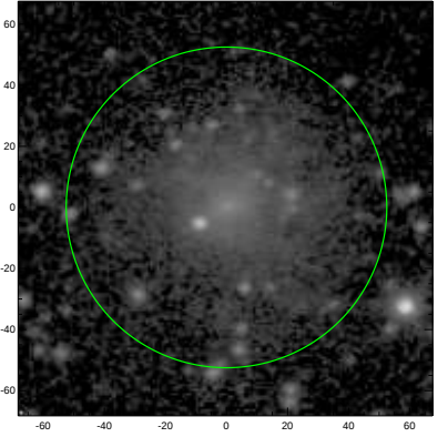
S4G: pa,inc= 2.6 27.5
