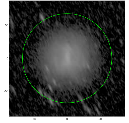
S4G: pa,inc= 115.6 70.1
