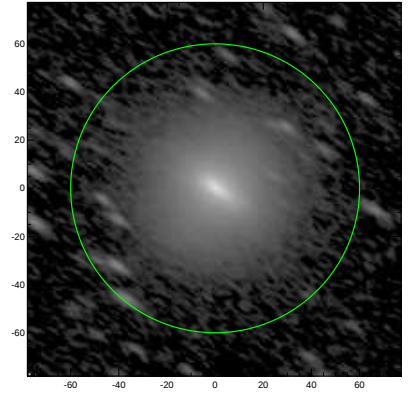
S4G: pa,inc= 146.9 66.9
