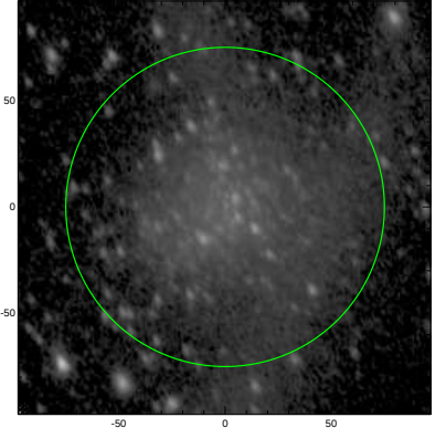
S4G: pa,inc= 113.3 49.5
