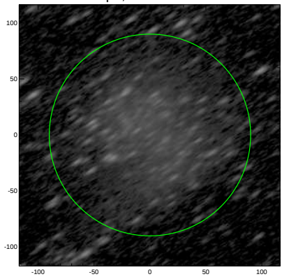
S4G: pa,inc= 32.6 71.7
