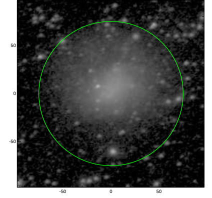
S4G: pa,inc= 18.9 40.0
