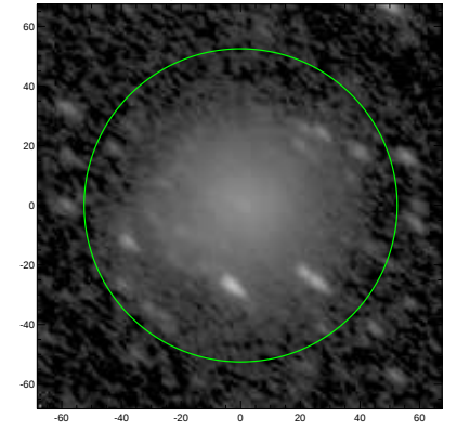
S4G: pa,inc= 139.4 59.3
