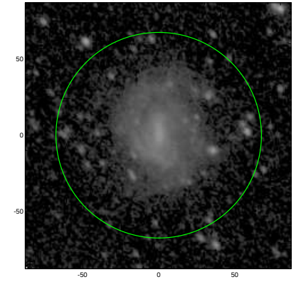
S4G: pa,inc= 125.0 38.6
