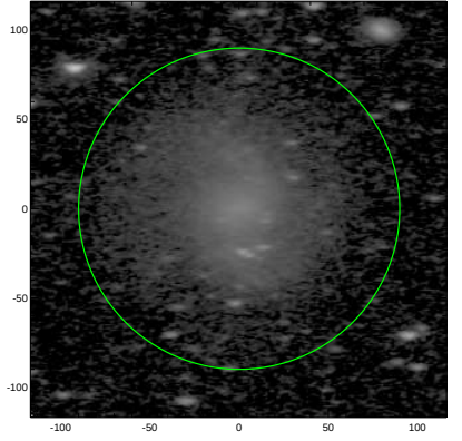
S4G: pa,inc= 2.0 63.1
