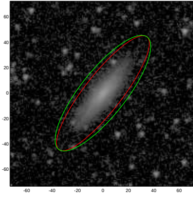
UGC12641
