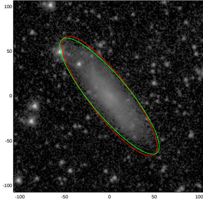
UGC05349
