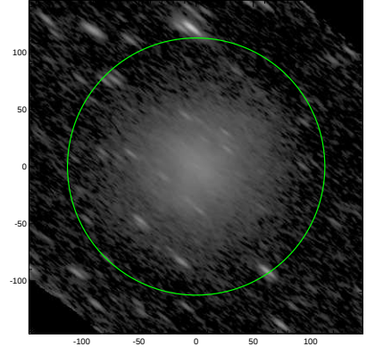
S4G: pa,inc= 141.5 74.1
