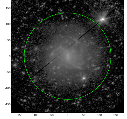
S4G: pa,inc= 21.4 32.8
