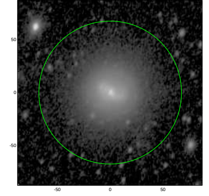
S4G: pa,inc= 71.2 45.5
