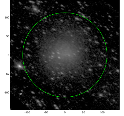
S4G: pa,inc= 150.7 53.4
