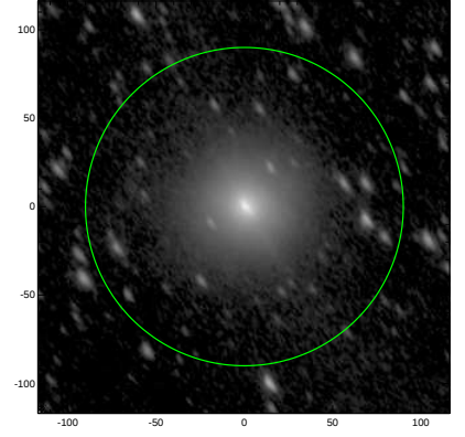
S4G: pa,inc= 123.4 60.7
