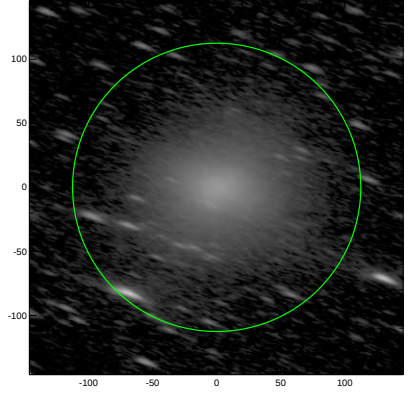
S4G: pa,inc= -19.5 74.5
