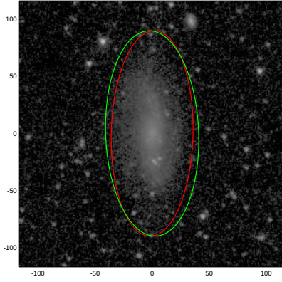
UGC08995
