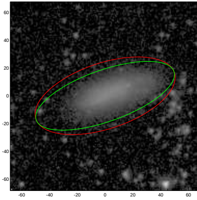
UGC01112
