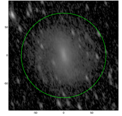
S4G: pa,inc= 108.9 66.4
