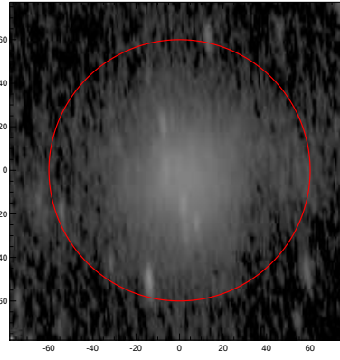
LEDA: pa,inc= 94.5 75.0
