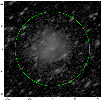
S4G: pa,inc= 35.9 61.2
