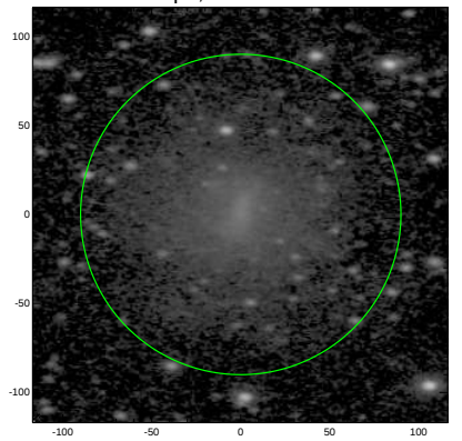
S4G: pa,inc= -2.7 52.5
