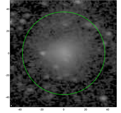
S4G: pa,inc= -5.7 44.5
