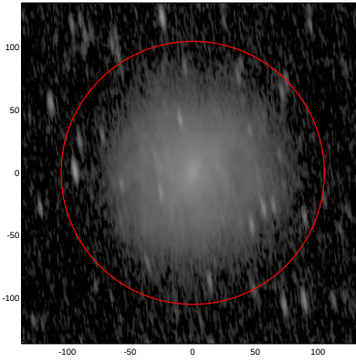
LEDA: pa,inc= 97.9 75.9
