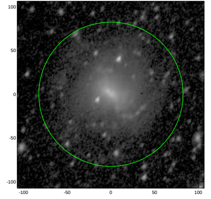
S4G: pa,inc= 55.9 47.5
