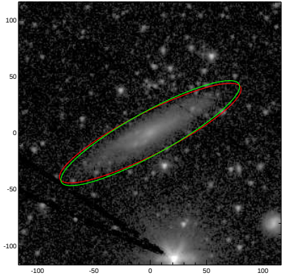
UGC12308
