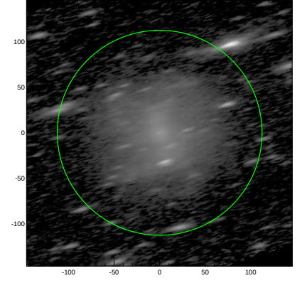
S4G: pa,inc= 16.4 76.0
