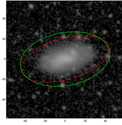
UGC07143
