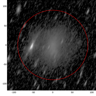
LEDA: pa,inc= 66.0 72.8
