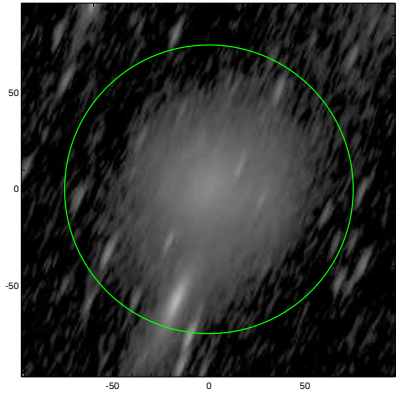
S4G: pa,inc= 66.9 76.8
