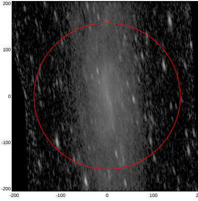
LEDA: pa,inc= 999.0 75.5
