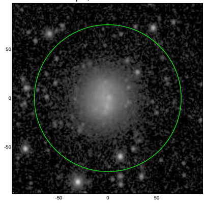
S4G: pa,inc= 81.2 22.5
