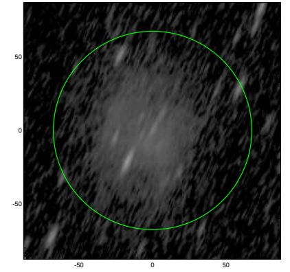
S4G: pa,inc= 65.3 74.8
