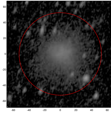
LEDA: pa,inc= 70.0 57.8
