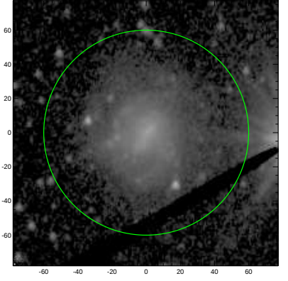
S4G: pa,inc= 78.4 32.9
