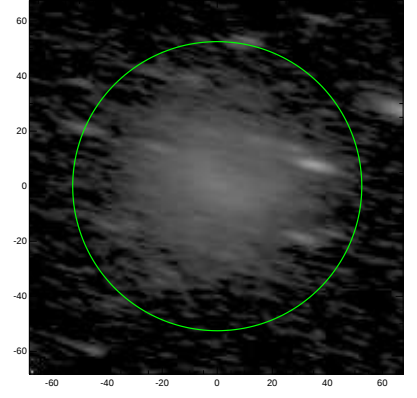
S4G: pa,inc= -13.1 73.5
