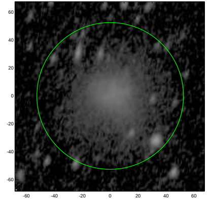
S4G: pa,inc= 70.9 58.3
