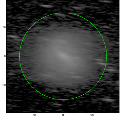
S4G: pa,inc= -6.5 78.7
