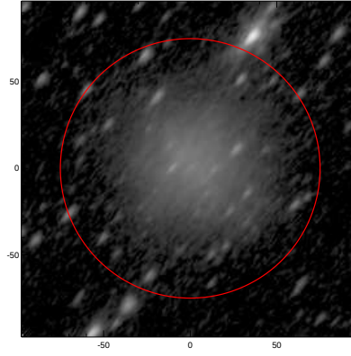
LEDA: pa,inc= 50.9 64.6
