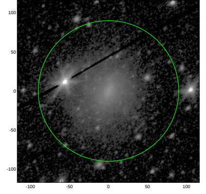
S4G: pa,inc= 46.1 42.6
