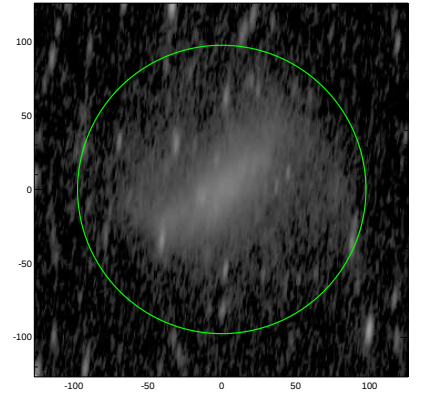
S4G: pa,inc= 83.0 75.9
