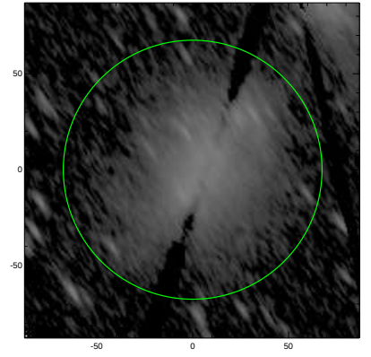
S4G: pa,inc= 121.9 73.2
