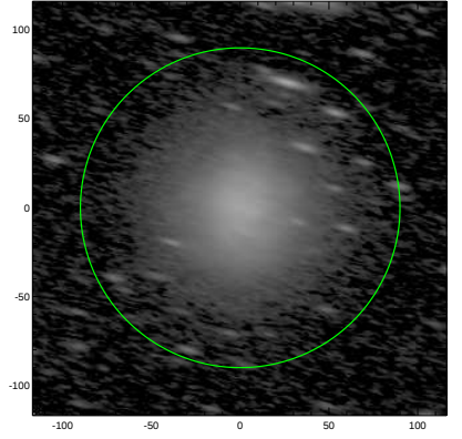
S4G: pa,inc= -14.3 73.0
