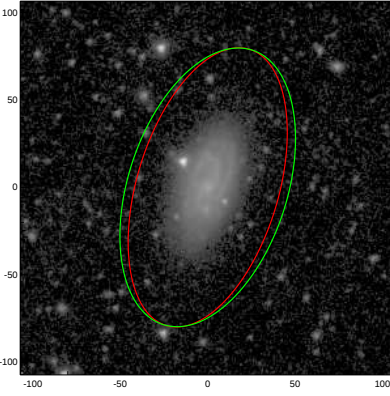
UGC02443
