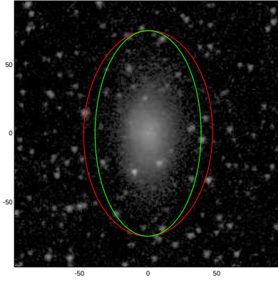
UGC01104
