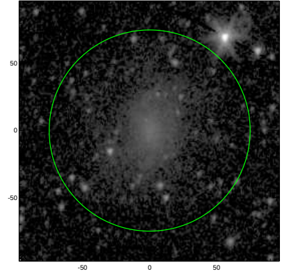
S4G: pa,inc= 77.7 29.1
