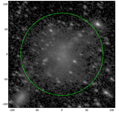
S4G: pa,inc= 150.3 49.9
