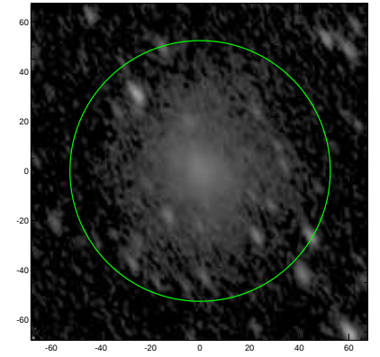
S4G: pa,inc= 120.5 60.4
