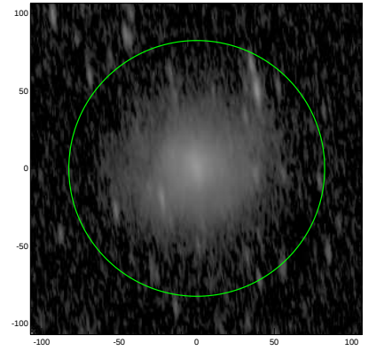
S4G: pa,inc= 97.2 76.0
