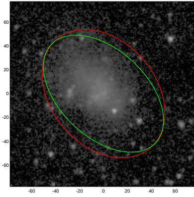
UGC12682
