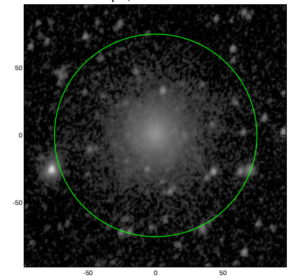
S4G: pa,inc= 65.3 40.4
