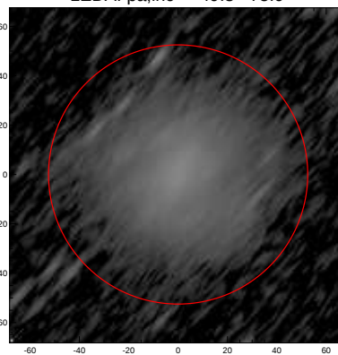
LEDA: pa,inc= 49.8 75.9
