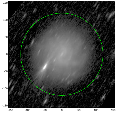
S4G: pa,inc= 58.4 73.9
