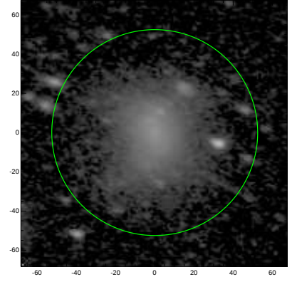
S4G: pa,inc= -13.7 49.3
