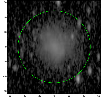
S4G: pa,inc= 90.0 64.6
