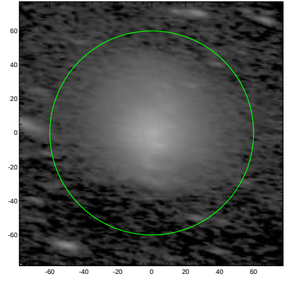
S4G: pa,inc= -10.6 70.8
