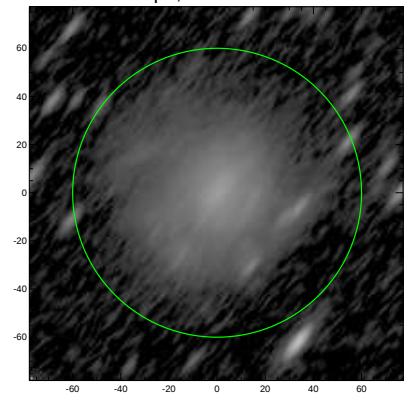
S4G: pa,inc= 51.5 72.7
