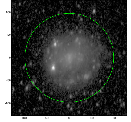
S4G: pa,inc= 85.0 54.2
