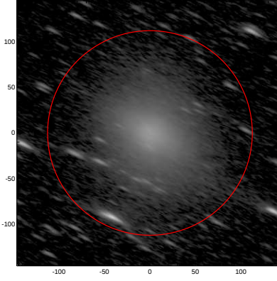
LEDA: pa,inc= 154.5 75.1
