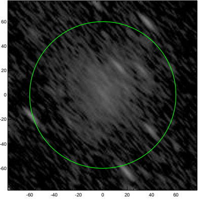
S4G: pa,inc= 132.2 77.1
