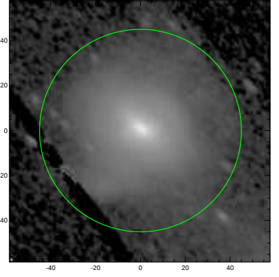
S4G: pa,inc= 132.3 53.6
