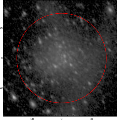
LEDA: pa,inc= 123.0 52.5
