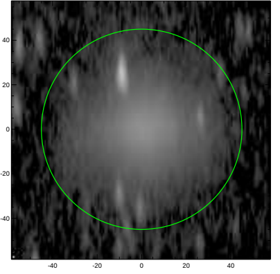
S4G: pa,inc= 91.5 73.4
