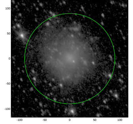
S4G: pa,inc= 125.3 46.1
