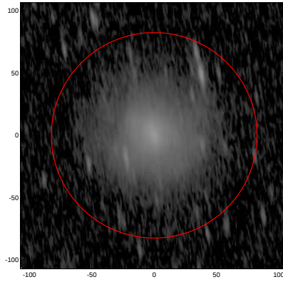
LEDA: pa,inc= 98.7 76.8
