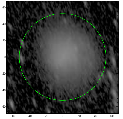
S4G: pa,inc= 109.5 69.4
