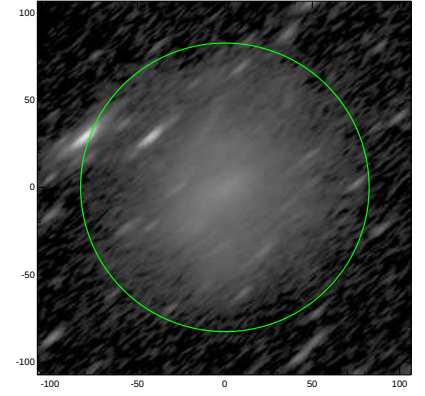
S4G: pa,inc= 39.8 74.8
