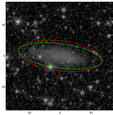
UGC12791
