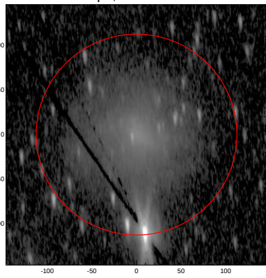
LEDA: pa,inc= 95.0 72.7
