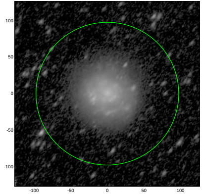
S4G: pa,inc= 50.0 59.7
