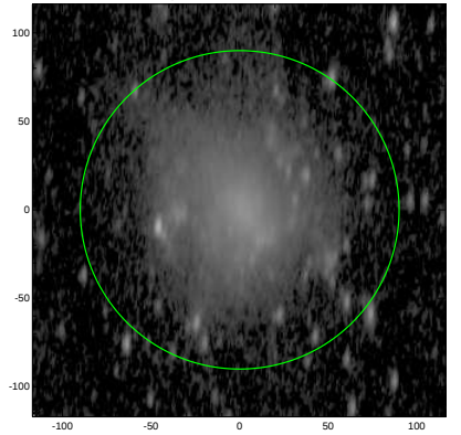
S4G: pa,inc= 86.3 68.1
