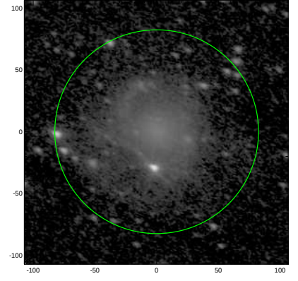
S4G: pa,inc= 154.5 50.9
