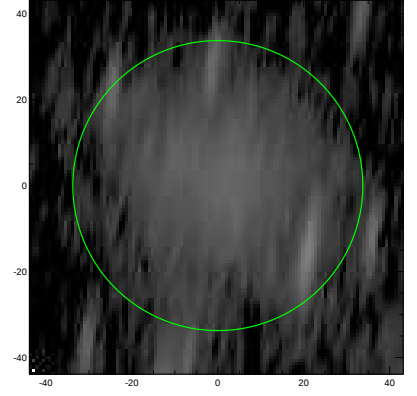
S4G: pa,inc= 83.0 79.9
