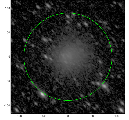
S4G: pa,inc= 133.8 60.5
