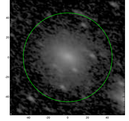
S4G: pa,inc= 147.0 56.4
