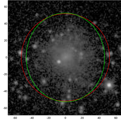
UGC08153
