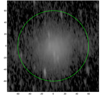
S4G: pa,inc= 94.8 73.0
