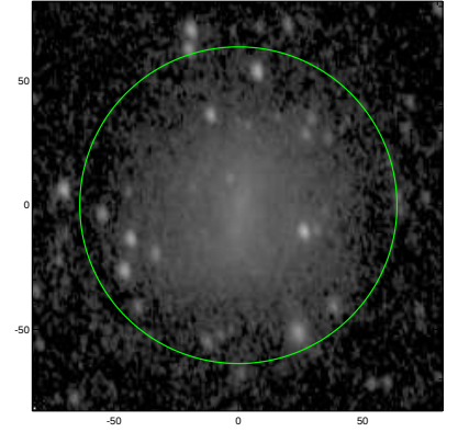
S4G: pa,inc= 99.4 50.5
