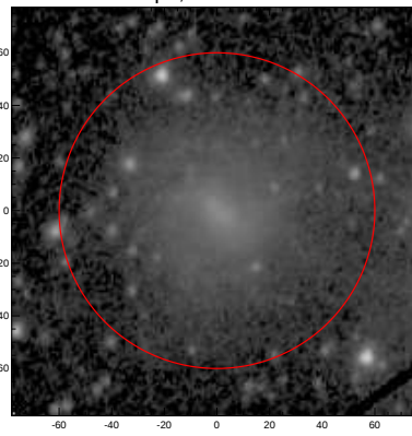
LEDA: pa,inc= 75.0 33.7
