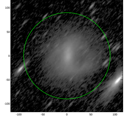
S4G: pa,inc= 47.9 73.9
