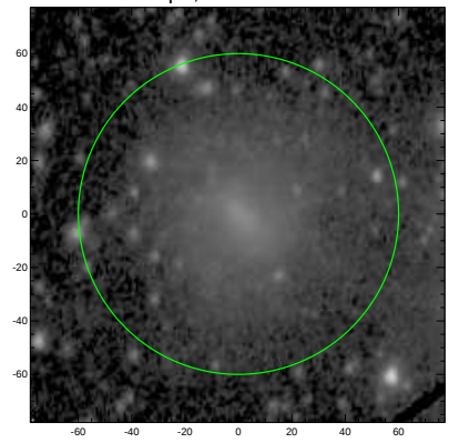
S4G: pa,inc= 82.5 38.5
