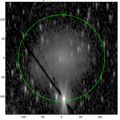
S4G: pa,inc= 92.4 72.1
