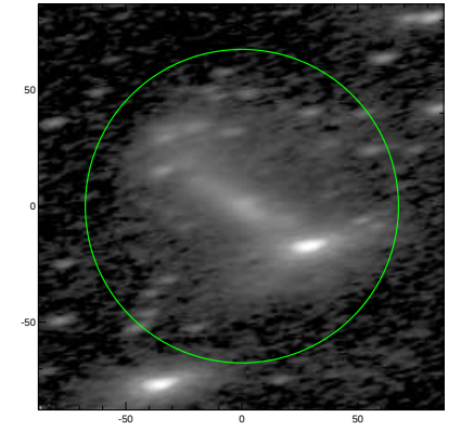
S4G: pa,inc= 11.6 69.4
