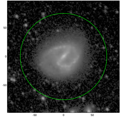
S4G: pa,inc= 125.6 31.5
