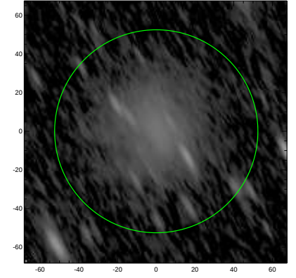
S4G: pa,inc= 118.0 74.3
