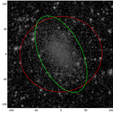
UGC02275
