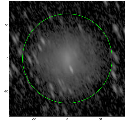
S4G: pa,inc= 112.6 70.7
