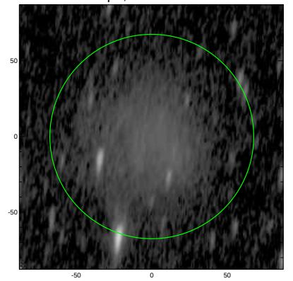
S4G: pa,inc= 82.6 73.1
