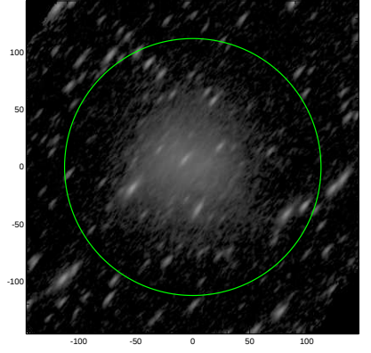
S4G: pa,inc= 49.8 68.5
