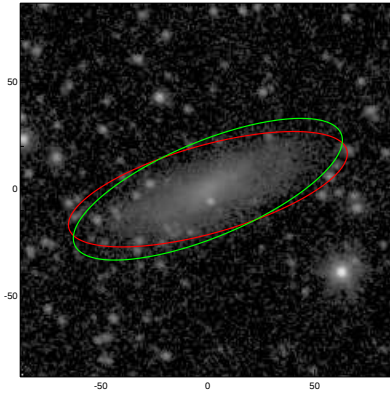
UGC04659
