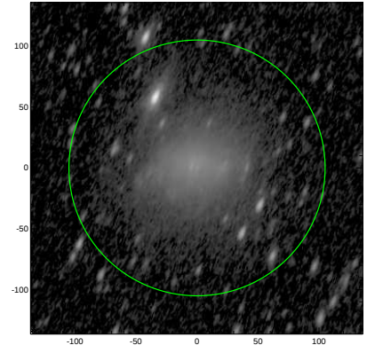
S4G: pa,inc= 65.8 65.8
