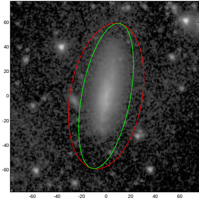
UGC08693
