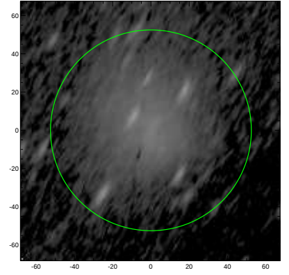
S4G: pa,inc= 61.0 70.6
