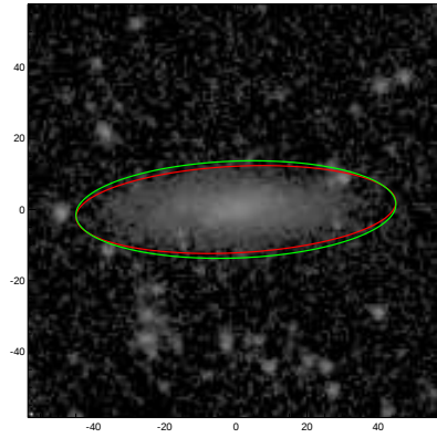
UGC08899
