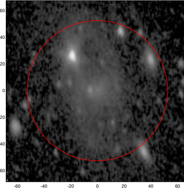
LEDA: pa,inc= 999.0 51.7
