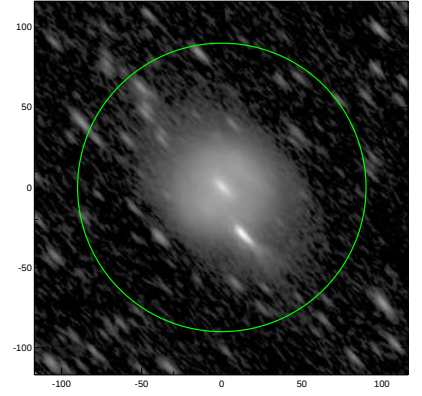
S4G: pa,inc= 132.8 70.5
