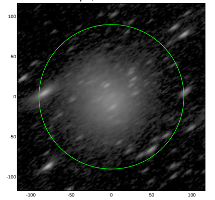
S4G: pa,inc= 34.2 70.4
