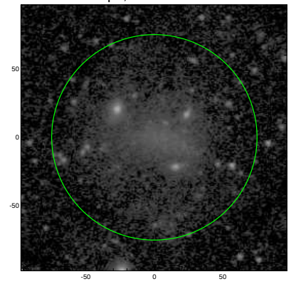
S4G: pa,inc= 179.6 15.5
