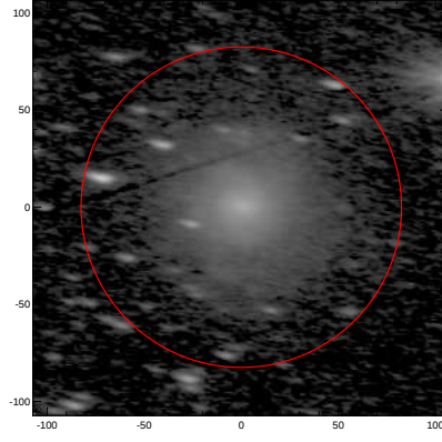
LEDA: pa,inc= 171.1 68.7
