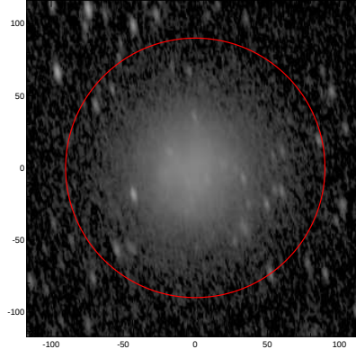
LEDA: pa,inc= 100.4 66.3
