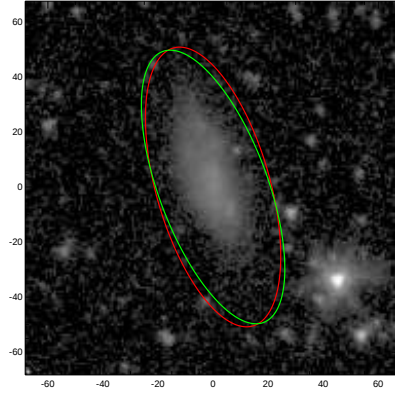
UGC01753
