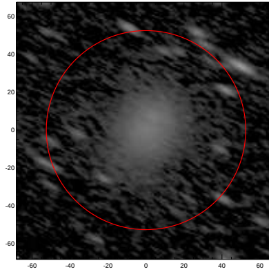
LEDA: pa,inc= 152.1 68.7
