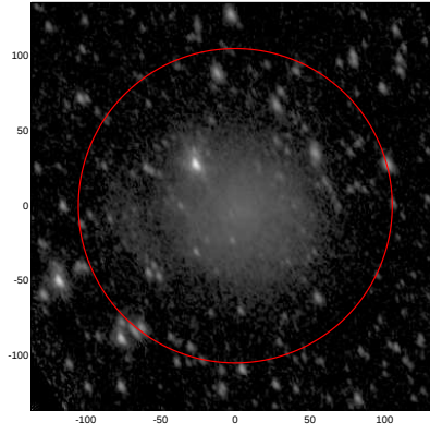
LEDA: pa,inc= 115.0 51.9
