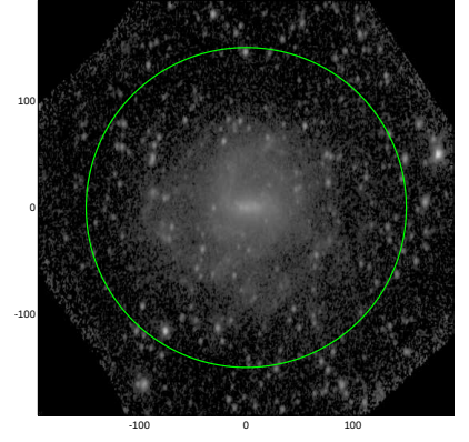
S4G: pa,inc= 87.0 48.5
