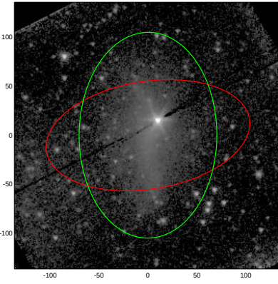
UGC08614
