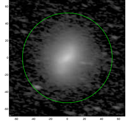
S4G: pa,inc= -11.7 65.1
