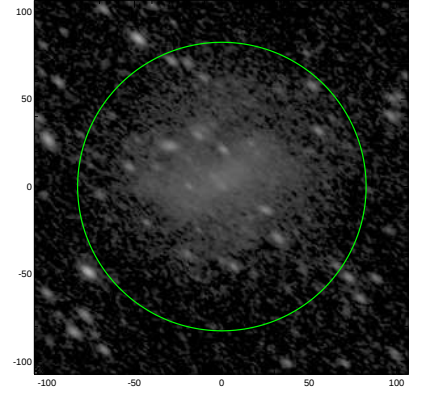
S4G: pa,inc= 144.3 56.7
