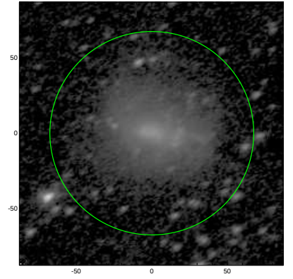
S4G: pa,inc= 28.2 50.6
