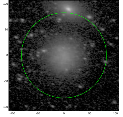
S4G: pa,inc= -13.4 52.7
