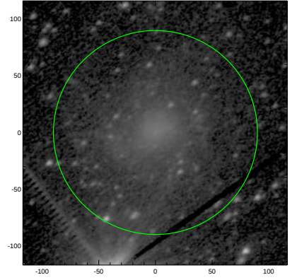
S4G: pa,inc= 33.8 45.7
