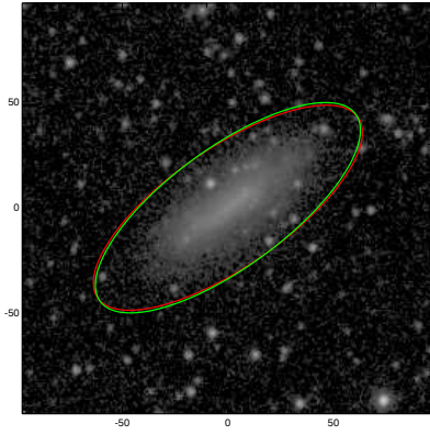
UGC11921
