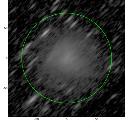
S4G: pa,inc= 43.8 76.1
