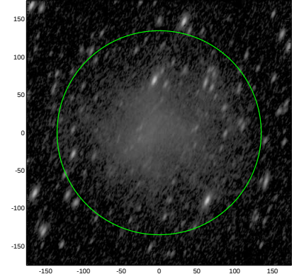
S4G: pa,inc= 64.9 66.5
