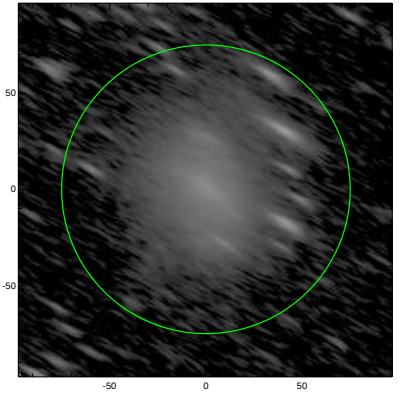
S4G: pa,inc= 150.7 76.8
