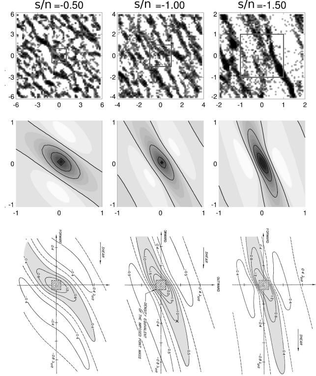
Figure 1.23 The upper row shows snapshots from simulation with different shear rates s : the physical width of the calculation region is fixed ( \sim 170 particle radii) and corresponds to 12, 8 , and 4\lambda_T for s/n = -0.5, -1.0 and -1.5 . The middle row shows 2D auto-correlation plots from the same simulations, covering 2\lambda_T \times 2\lambda_T . The lowermost row shows Julian-Toomre (1966) analytic calculations for the same shear rates of the wake response around an orbiting point mass-point: their graphs have been rotated to same orientation as our simulation plots. In the simulations \tau_D = 0.5 , constant \epsilon_n = 0.5 , r_h = 0.82 .
