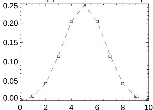
Gaussian approximation N= 10 p=0.
