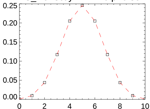
C_v directly N= 10 p=0.50
