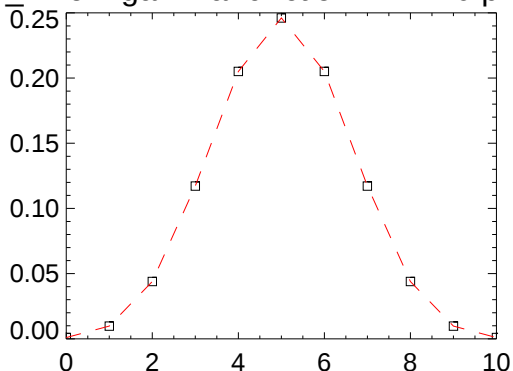
C_v from gamma-function N= 10 p=0.50
