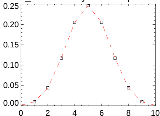
C_v recursively N= 10 p=0.50
