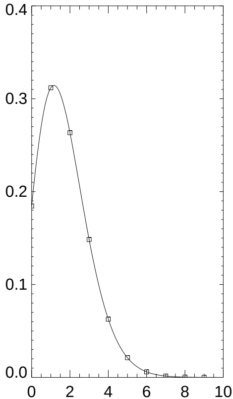
Poisson with \mu = 1.69000
