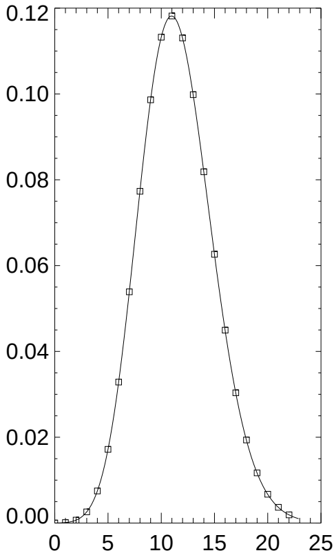
Poisson with \mu = 11.480
