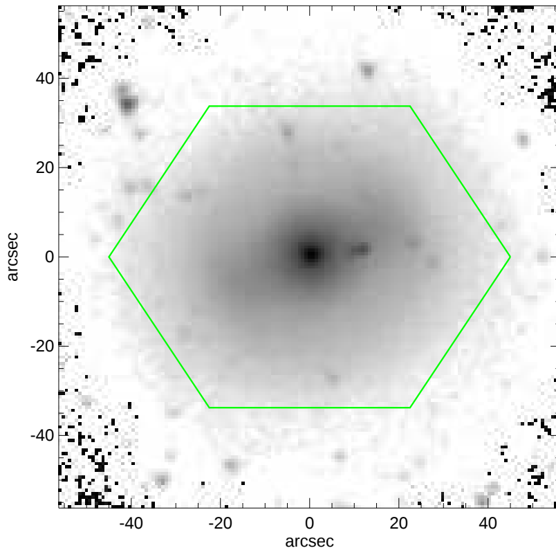
NGC5770
