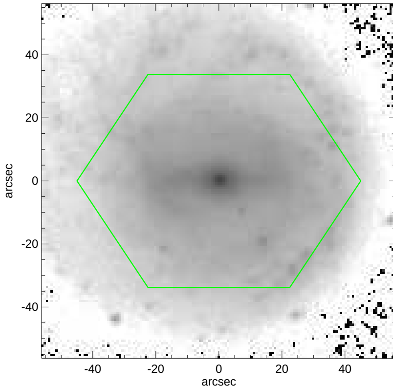
NGC7421
