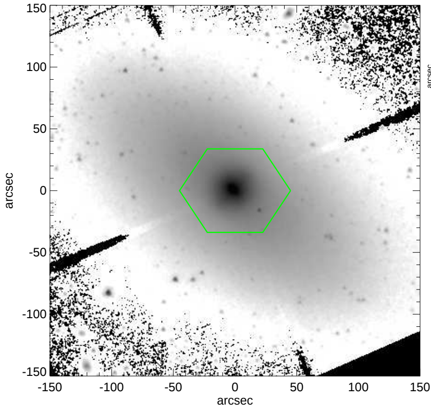
NGC3384
