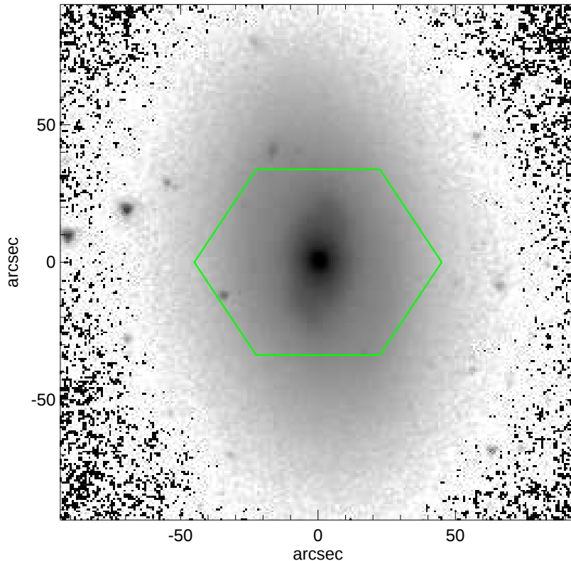
NGC3941
