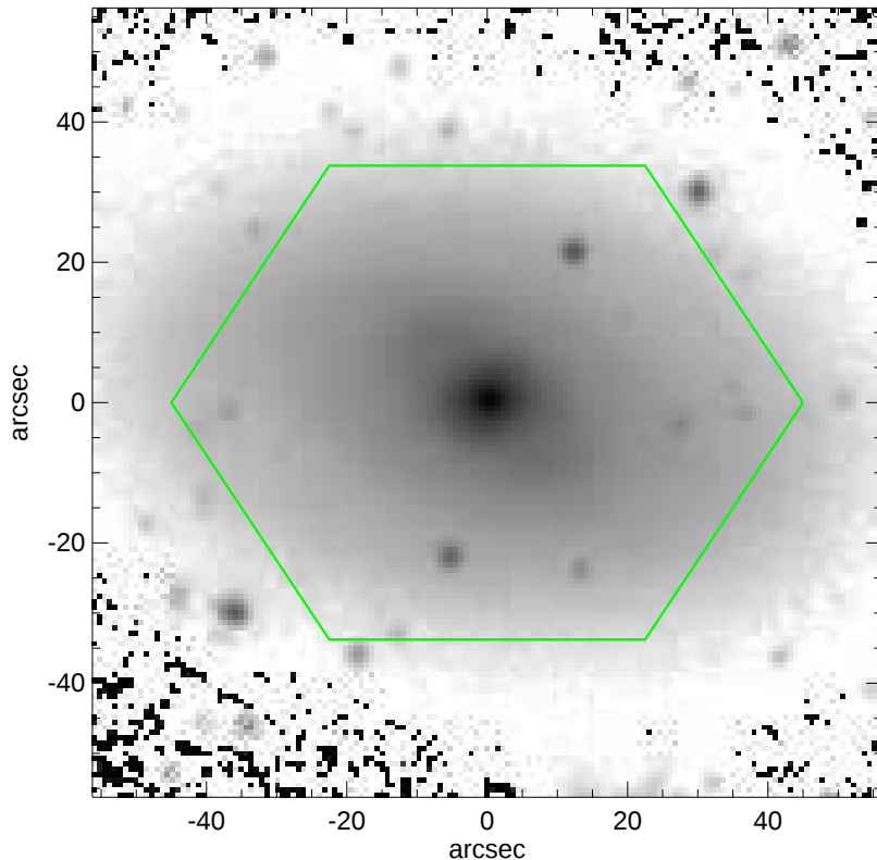
NGC7079
