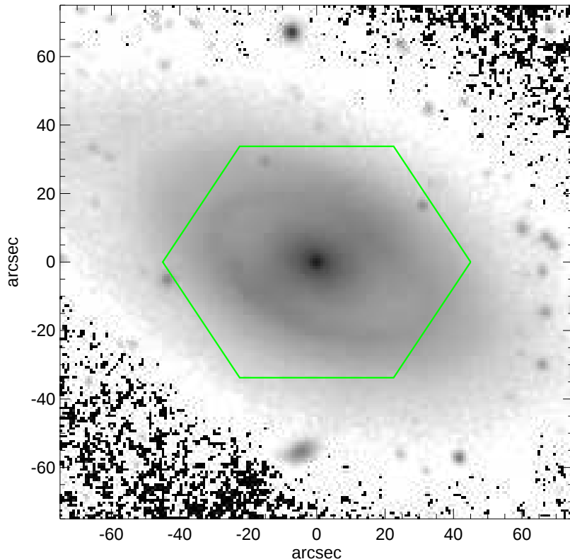
NGC5750
