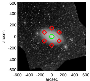
NGC3992
