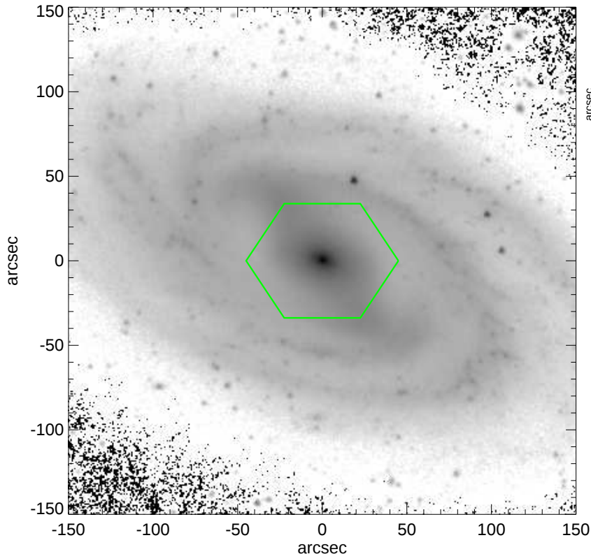
NGC3992
