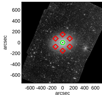
NGC1398
