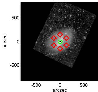
NGC1097
