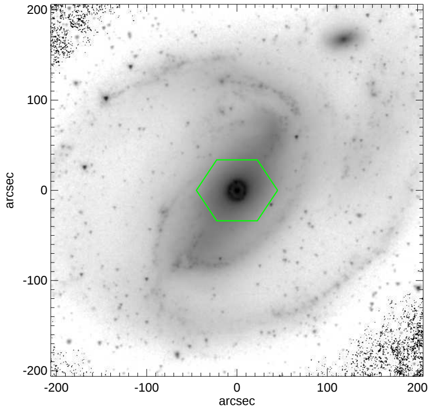
NGC1097
