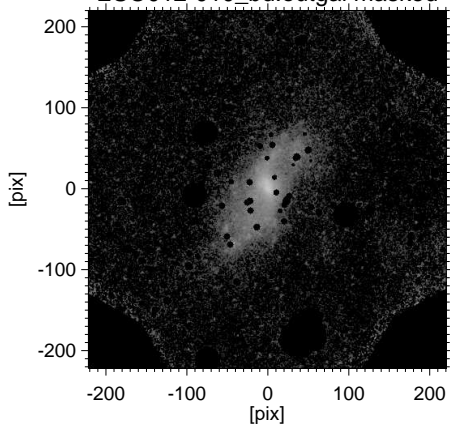
residual 9.78076
