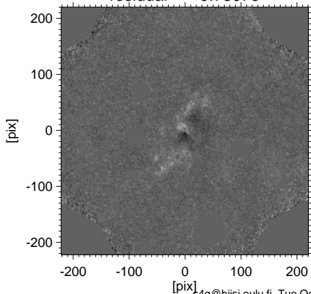
residual 9.78076
