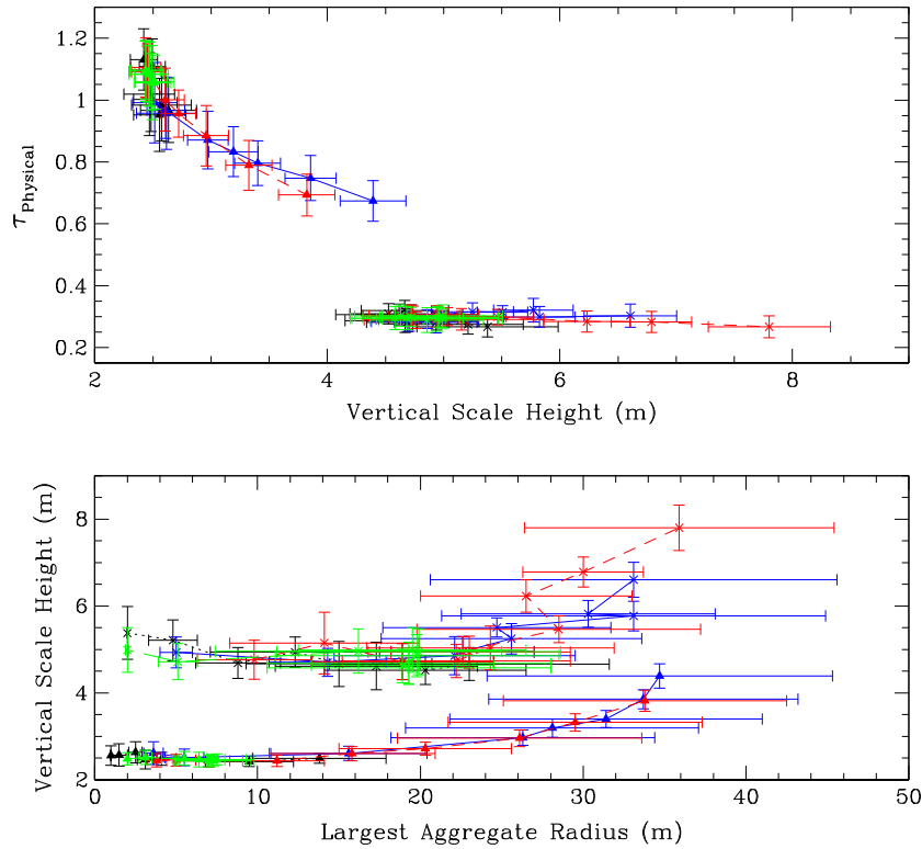
Fig. 11. Composite plot displaying physical optical depth ( \tau_{phys} ) vs. equilibrated vertical scale height ( h ) in the top pane, and h vs. the radius of the largest aggregate ( R_{max} ) in the bottom pane, for many of our simulation suites. Symbols distinguish A ring from B ring suites, with triangles for B ring, and x's for A ring. Colors distinguish which parameter was varied: merge limit suites with a lower fragmentation limit ( 1\nu_{esc} ) are dotted (black), merge limit suites with a higher fragmentation limit ( 2\nu_{esc} ) are solid (blue), fragmentation limit suites are dashed (red), and bond strength suites are long-dashed (green). See Section 3.8 for a discussion. (For interpretation of the references to color in this figure legend, the reader is referred to the web version of this article.)
