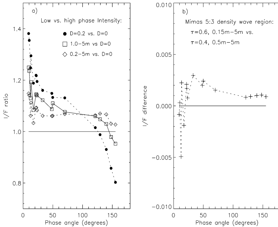
Fig. 21. In (a) the phase angle dependence of various models is shown relative to the \tau = 1.0, D = 0 multilayer model. The used values of \alpha, B , and B' correspond to those in Fig. 19: the scatter of points results from combining two set of solar elevations, not from any Monte Carlo uncertainty. Models include a homogeneous system with D = 0.2 and two size distribution models, with s_{\min} = 1.0 and 0.2 m. In (b) the difference of I/F for the Mimas 5:3 resonance site in comparison to its surroundings is modeled, by assuming that the surrounding region has \tau_{\text{dyn}} = 0.4 and a size distribution from 0.5 to 5 m. For the resonance site it is assumed that a q = 3 size distribution extends to 0.15 m, with correspondingly increased \tau_{\text{dyn}} = \log(5.0/0.15)/\log(5.0/0.5) \times 0.4 \approx 0.6 . Compare with Fig. 22 in Dones et al. (1993). In both frames A = 0.5 and the Callisto phase function are assumed.
