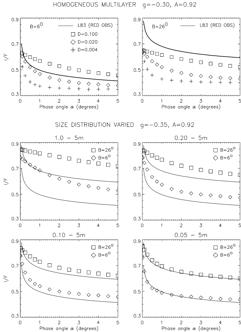
Fig. 14. In the uppermost row homogeneous systems with different D 's are compared to the observed B-ring phase curves. The observational curves for B' = B = 6^\circ and 26^\circ are constructed from Lumme et al. (1983) Eqs. (4), (5) and Table IIb, using I_{EZ}/F = 0.68 for the calibration of the brightness of Saturn's equatorial zone in the red ( \lambda = 620 nm, Lumme and Reitsema, 1978). The assumed albedo ( A = 0.92 ) and phase function (Henyeý-Greenstein law with g = -0.3 ) correspond to model A in Lumme et al. (1983), and \tau_{\text{dyn}} = 1 . In the two lower rows size distribution models with increasing width are compared ( \tau_{\text{dyn}} = 1.25 , except for the last model for which \tau_{\text{dyn}} = 1.5 ). The albedo is the same as in the homogeneous models, while g = -0.35 .
