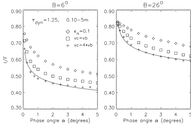
Fig. 22. Opposition effect due to mutual shadowing, calculated for dynamical simulations with different particle elasticities. Solid curves refer to Lumme et al. (1983) observations in red and the phase function and albedo are the same as in Fig. 14. In comparison to Fig. 14, which assumes v_c/v_B = 1 , s_{\min} = 0.05 m, the more elastic model with v_c/v_B = 4 yields an opposition phase curve close to the observed one for s_{\min} = 0.1 m instead of s_{\min} = 0.05 m.
