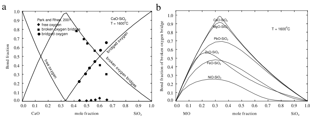
Fig. 39. Calculated silicate structure from Modified Quasichemical Model parameters. (a) Comparison of calculated bond fractions of O^{2-} , O^- and O^0 for the CaO-SiO_2 system with experimental data of Park and Rhee [206], and (b) calculated bond fractions of O^- for various binary silicate systems at 1600 °C.
