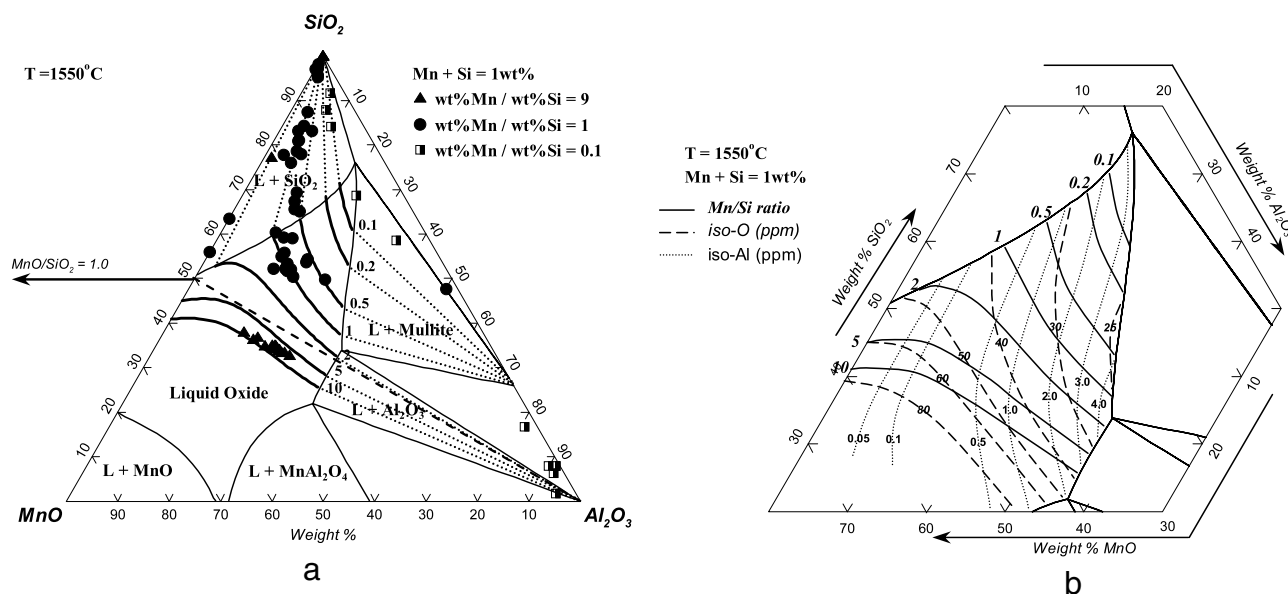
Fig. 9. Computed MnO-Al 2 O 3 -SiO 2 inclusion composition in equilibrium with Mn/Si deoxidized steels at 1550 °C [44,124]. The lines with values indicate the composition of Mn/Si deoxidized steel. (a) Calculated inclusion composition in comparison with experimental data, and (b) calculated Mn/Si ratio, iso-oxygen and iso-aluminum in steels.
