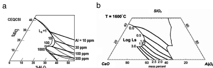
Fig. 23. Sulfur distribution ( L_s = (\text{wt}\%S)_{\text{slag}}/(\text{wt}\%S)_{\text{steel}} ) for a \text{CaO-SiO}_2\text{-Al}_2\text{O}_3 slag at 1600 °C in equilibrium with the \text{Fe-0.1C-0.7Mn-0.1Si-0.05Al-0.0005O-0.003S} (wt%) steel, calculated with (a) CEQCSI [150] and (b) FactSage [151].
