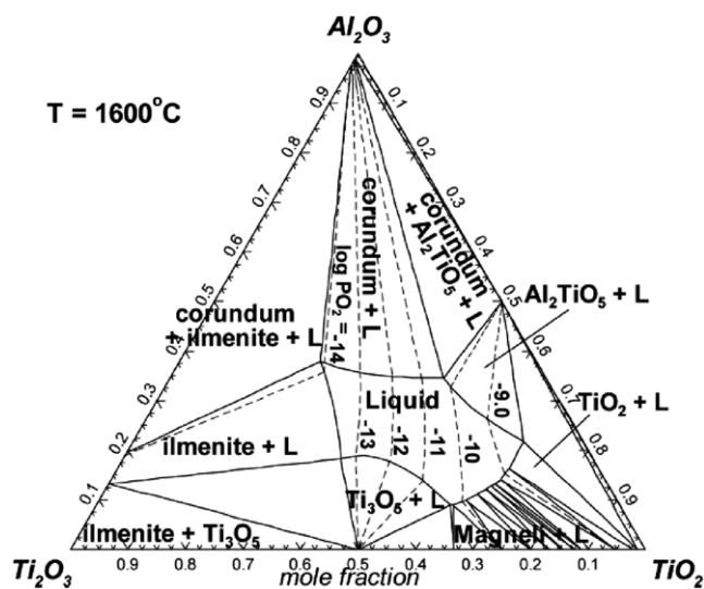
Fig. 14. Predicted phase diagram of the \text{Al}_2\text{O}_3 - \text{TiO}_2 - \text{Ti}_2\text{O}_3 system at 1600^\circ\text{C} with oxygen partial pressure isobars (bar) [134].
