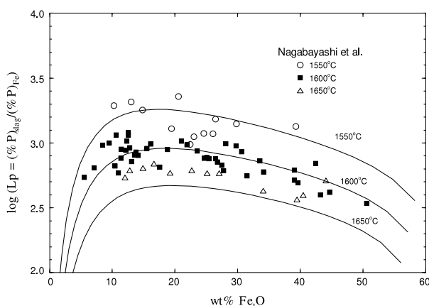
Fig. 25. The calculated phosphorus distribution ( L_p = (\text{wt}\%P)_{\text{slag}}/(\text{wt}\%P)_{\text{steel}} ) between the \text{CaO-saturated CaO-FeO-P}_2\text{O}_5 slag and molten \text{Fe-P} steel [151] in comparison with experimental results [159].
