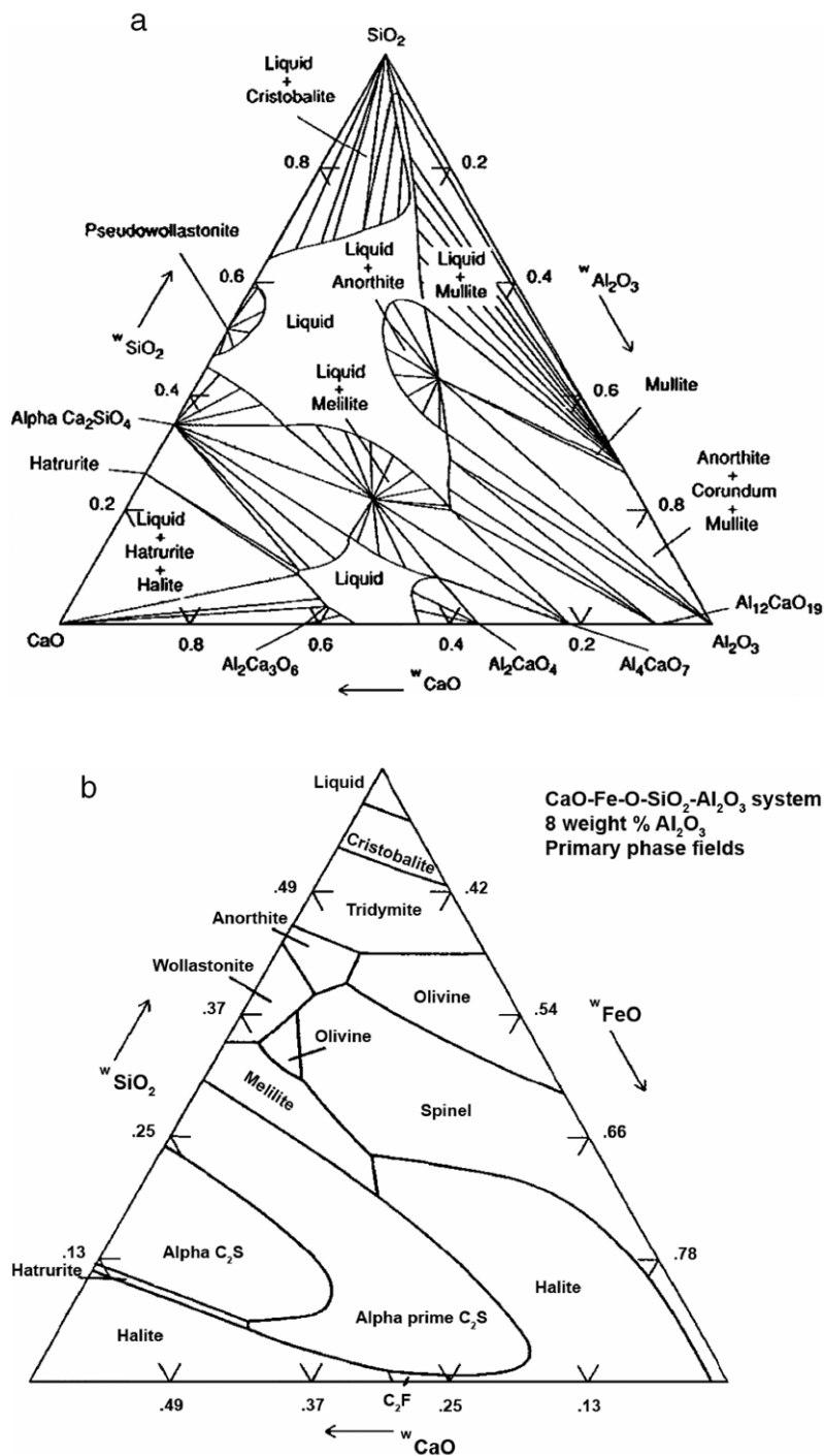
Fig. 5. Phase diagrams of (a) the \text{CaO}-\text{Al}_2\text{O}_3-\text{SiO}_2 [66] at 1500^\circ\text{C} and (b) the \text{CaO}-\text{FeO}-\text{SiO}_2-8\text{ wt}\%\text{Al}_2\text{O}_3 [67] systems, calculated with MTDATA [4].
