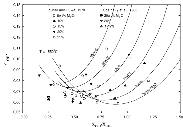
Fig. 26. Calculated water solubilities in \text{CaO-MgO-SiO}_2 slags at 1550 °C using the FactSage FToxid database [112] along with experimental data [160,161].
