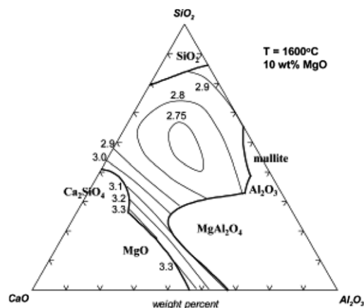
Fig. 27. Predicted iso-capacity lines of water for \text{CaO-Al}_2\text{O}_3\text{-SiO}_2\text{-10 wt}\% \text{MgO} at 1600 °C [112]. Values are \log (C_{\text{OH}} \times 10^4) .
