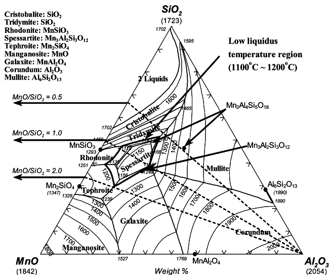
Fig. 8. Calculated liquidus surface of the MnO–SiO 2 –Al 2 O 3 system [44]. Temperature in °C.
