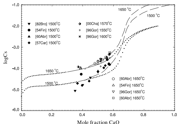
Fig. 24. Calculated sulfide capacities for the binary \text{CaO-SiO}_2 slags from FactSage [53] (solid and dotted lines) and MTDATA [67] (dashed lines) in comparison with experimental data [152–158].
