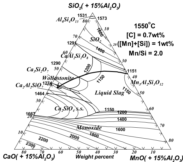
Fig. 11. Calculated change of composition of inclusions formed during Mn/Si deoxidation (as shown by arrows) when the Mn/Si ratio equals 2.0 for tire-cord steel ([C] = 0.7 wt%) by reaction with CaO-containing top slag at 1550 °C (top slag composition: 55CaO–15Al 2 O 3 –30SiO 2 in wt%). Predicted liquidus isotherms (T in °C) are also plotted [126].
