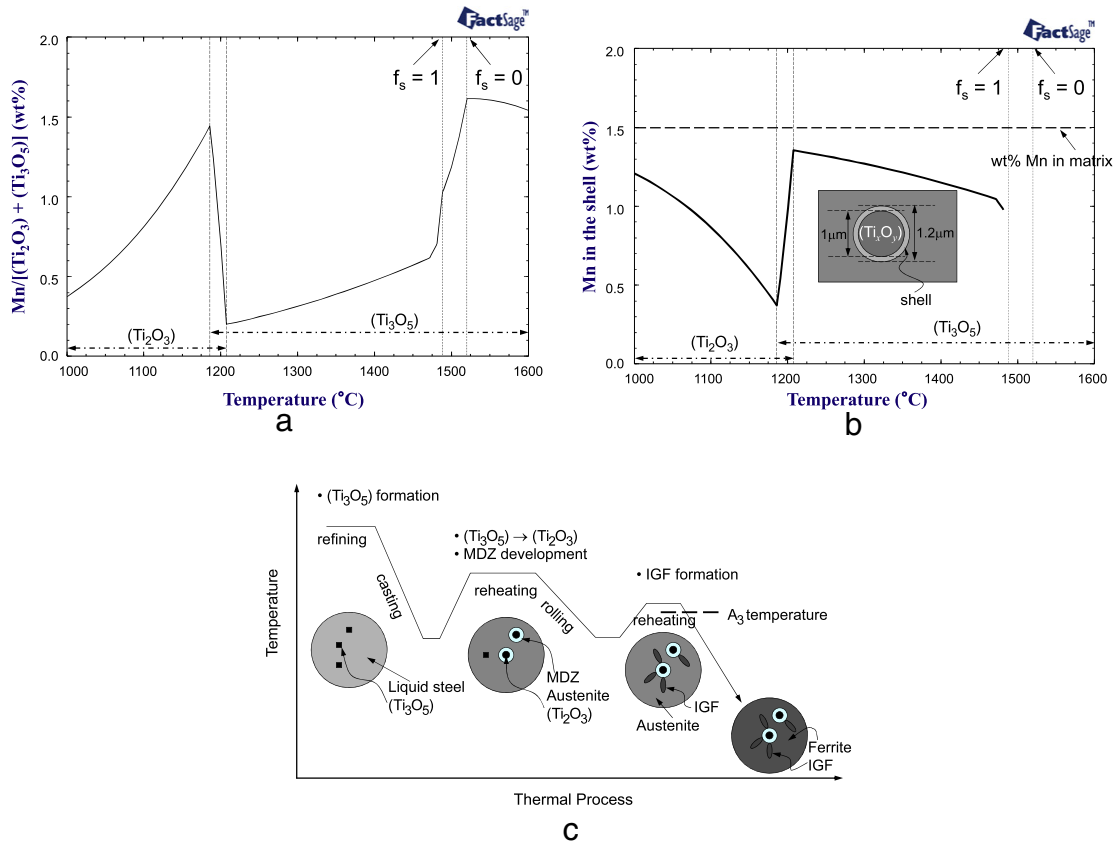
Fig. 19. Calculated Mn concentrations (a) in \text{TiO}_x inclusions and (b) in a shell around the \text{TiO}_x inclusion in equilibrium with Fe-0.1C-1.5Mn-0.1Si-0.007S-0.005O-0.015Ti (in wt%), and (c) proposed optimum thermal process in order to maximize IGF development associated with MDZs [141].
