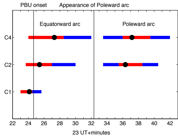
Fig. 4. Timeline of the C1, C2 and C4 crossings of the two arcs. Red (blue) horizontal bars denote upward (downward) FAC regions. Black dots denote times of maximum upward FACs. In addition, vertical lines show pseudo-breakup (PBU) onset time and the time when the poleward arc starts to form.
