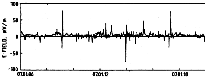
Figure 1 Measurements on ISEE-1 at 32 samples/sec of spiky electric fields of about 100 mV/m and a duration of 0.05 seconds of a bow shock crossing. This is a single axis measurement so that the direction relative to the magnetic field of the spikes is not known. Similarly no information of the phase velocity is available from this measurement. On Cluster the phase velocity could be determined if the potentials from each of the four probes were available at sampling rates of 10000 times/sec.
