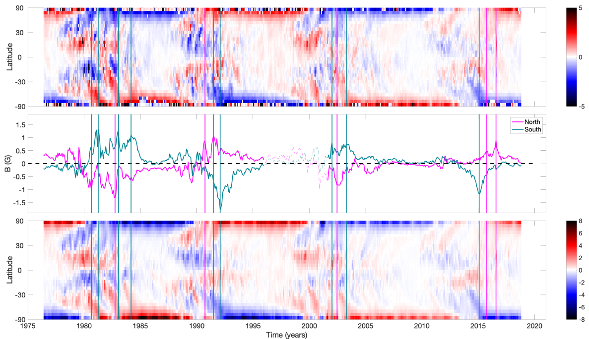
Fig. 1. Results for weak-field shifts from WSO synoptic maps. Top: Weak-field shifts calculated for each latitude bin and rotation, called here the shift butterfly diagram (positive shifts in red, negative in blue). Middle: Hemispheric shift values (north in pink, south in cyan). Bottom: Longitudinal means of the photospheric field for each latitude bin and rotation, i.e., the normal magnetic butterfly diagram (positive field in red, negative in blue). Vertical lines denote the shift extrema (north in pink, south in cyan).
