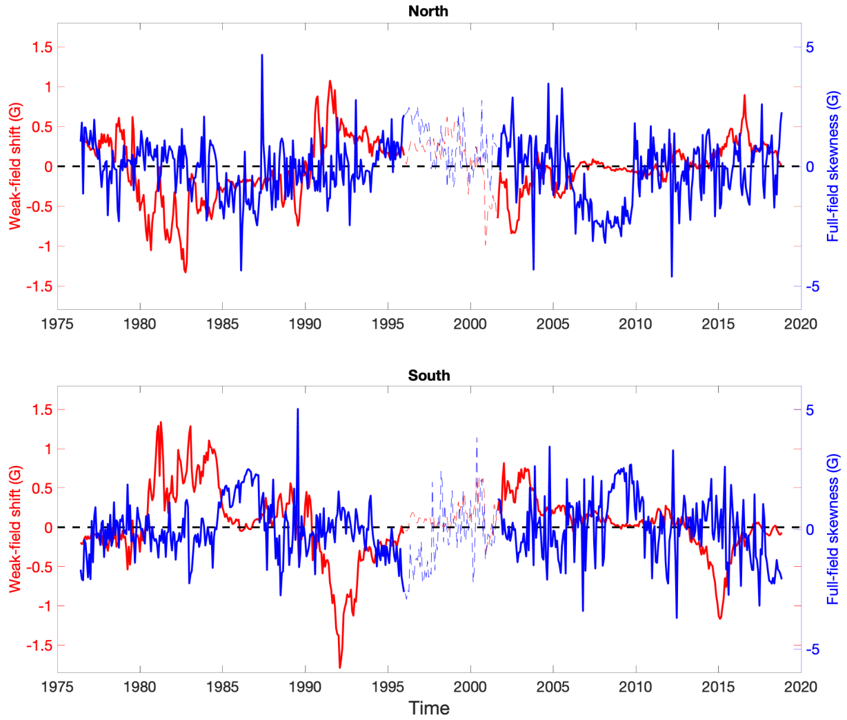
Fig. 4. Hemispheric weak-field shifts (red; left y-axis scale) and full-field skewnesses (blue; right y-axis scale) for each WSO synoptic map.
