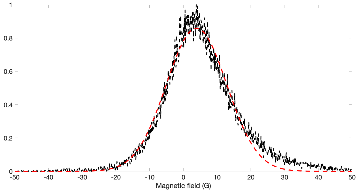
Fig. 6. Distribution of SOLIS high-resolution field values at high southern latitudes (poleward of -70 degrees) for CR 2052 (Jan. 2007; black dashed line), together with the Gaussian fit to weak field values (red dashed line).
