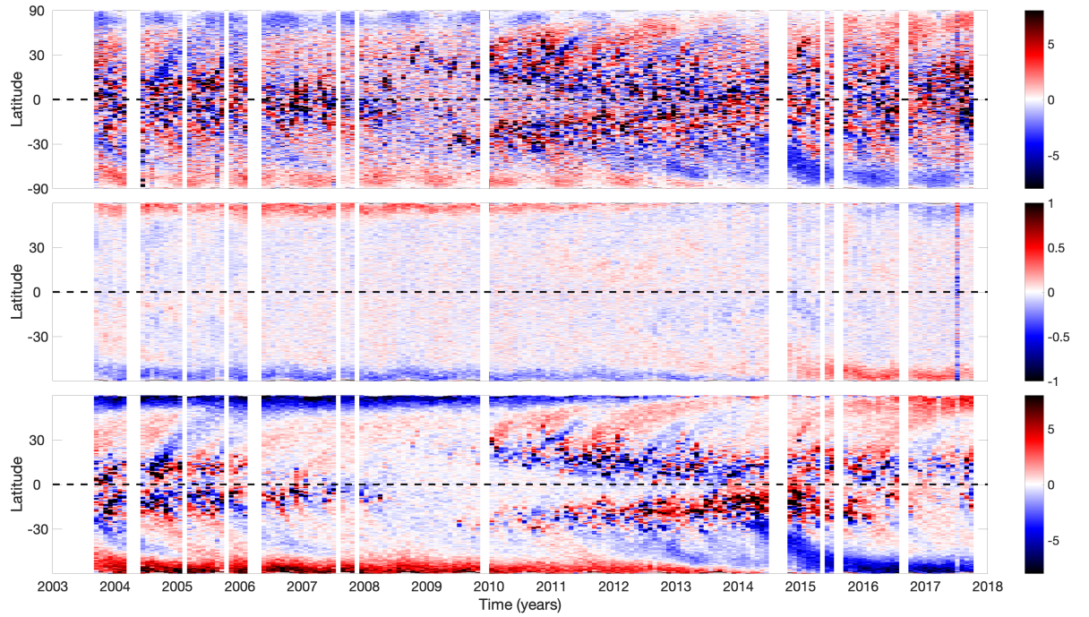
Fig. 5. Results for skewness from SOLIS/VSM synoptic maps. Top: Skewness calculated for each latitude bin and rotation using all field values, called here the full-field skewness butterfly diagram (positive skewness in red, negative in blue). Middle: Same as in top panel, but using only weak-field values to calculate skewness, called here the weak-field skewness butterfly diagram. Bottom: Longitudinal means of the photospheric field for each latitude bin and rotation, known as the normal magnetic butterfly diagram.
