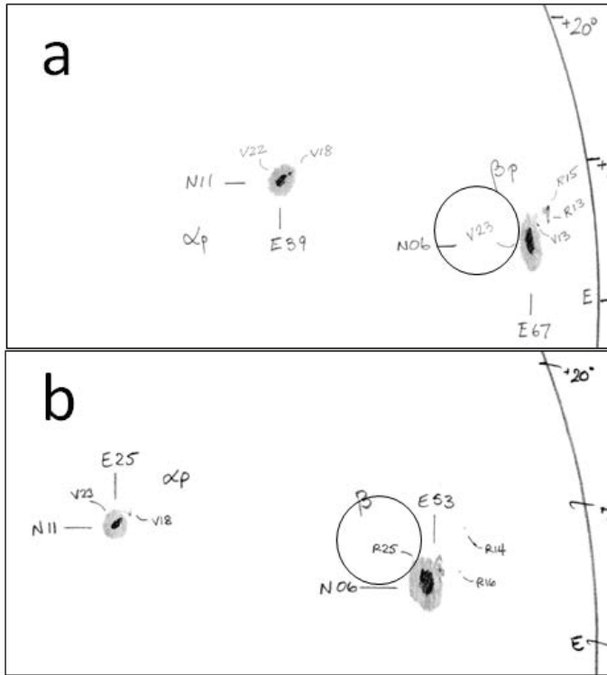
Fig. A.4. Example of incorrect measurement of sunspot polarity. Polarity of a sunspot observed on 13 November 2013 (panel a ) was determined as “V” (negative), but on all following days (panel b , 14 November 2013), the measured polarity was “R” (positive). The circles indicate the polarity measurement for this sunspot.
