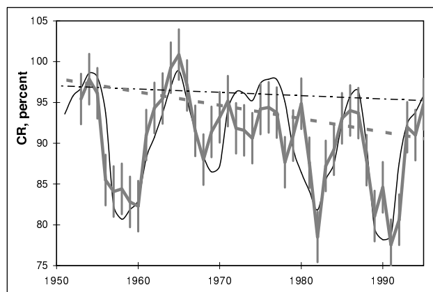
Fig. 2. Climax NM count rates in percent (count rate in May 1965 is 100%). Black thin curve depicts the actual count rates and the thick grey curve (including estimated errors) gives the count rate reconstructed from F_s . The dash-dotted black line and the grey dashed line give the trends for the respective series.
