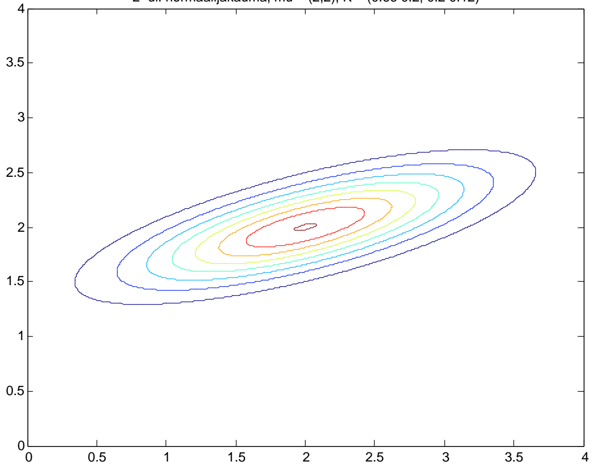
2-ul. normaalijakauma, \mu = (2,2) , K = \begin{pmatrix} 0.66 & 0.2 \\ 0.2 & 0.12 \end{pmatrix}
