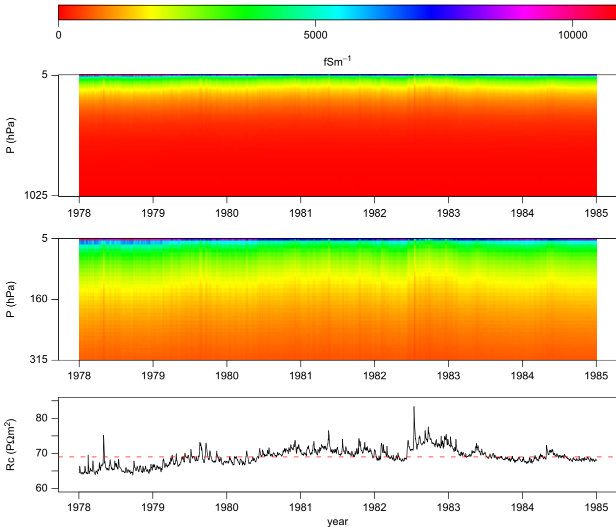
Fig. 2. Air conductivity profiles (against atmospheric pressure P ) for Lerwick 1978–1985 from the CRII cosmic ray ion-production model. Conductivity time series are shown for the troposphere (upper panel) with the upper troposphere (middle panel), both using the same conductivity scale (top bar). The lower panel shows the surface-stratosphere columnar resistance R_c derived from integrating the air conductivity profile with height, with the median R_c marked (dashed line).
