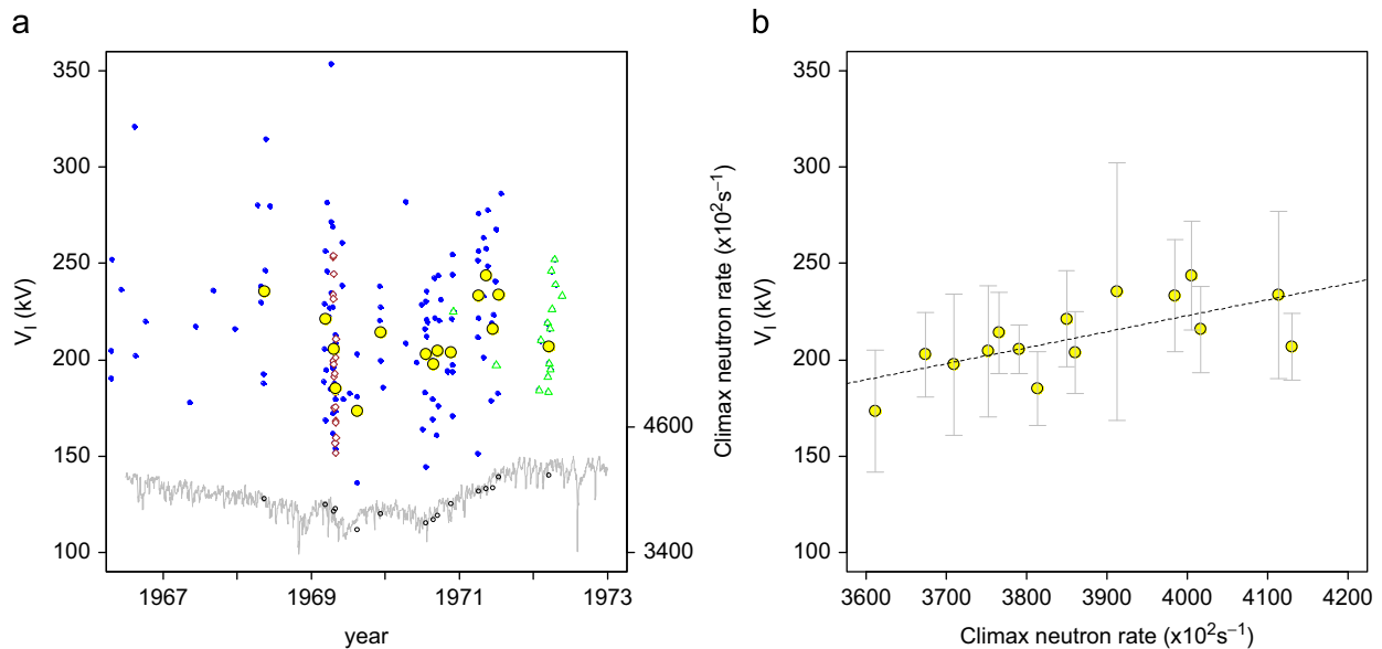
Fig. 4. Comparison of ionospheric potential ( V_i ) and neutron counter data at Climax (grey line), measured from 1966–1972. (a) V_i soundings of Mülheisen from Weissenau, Germany (points, individual soundings) and the Meteor research ship in the mid-atlantic (diamonds, individual soundings), and of Markson from the Bahamas (green triangles, daily averages). Large circles show monthly averages for months having 4 or more V_i points available, with the monthly neutron counter averages using the same days' data as for V_i . (b) Monthly-averaged V_i plotted against monthly average neutron count rate. Error bars represent two standard errors. (Individual Mülheisen V_i soundings have been corrected to equivalent daily values using the Carnegie curve, assuming the sounding to be representative of V_i at 3.5 h after launch time.)
