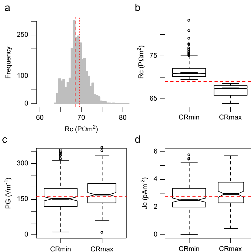
Fig. 3. (a) Histogram of calculated columnar resistances R_c for Lerwick with the upper and lower 40% quantiles marked to distinguish between “ CR_{min} ” (dotted line) and “ CR_{max} ” (dashed line), respectively. (b), (c), and (d) Comparisons of CR_{min} and CR_{max} columnar resistances R_c (b), with measured and seasonally corrected potential gradient (c) and conduction current density (d), from Lerwick. Dashed line shows the medians of the undivided dataset. (For the boxplots, the box width is proportional to the square root of the number of values in each interval; the box edges and the line in the centre of each box show the upper and lower quartiles and the median, respectively. Notches indicate the 95% confidence limits on the medians and the whiskers extend to 1.5 times the inter-quartile range.)
