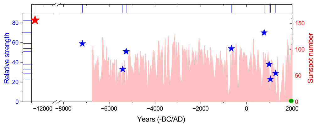
Fig. 8. Extreme solar storms (stars) known from cosmogenic isotopes, including the one of 12350 BC (the red star in the upper-left corner) and others as listed in Cliver et al. (2022). The strength of the events is normalized to that of the strongest directly observed SEP event of 23-Feb-1956 (Usoskin et al., 2020, green circle in the bottom-right corner). The red-shaded curve represents the decadal sunspot numbers (right-hand-side ordinate) reconstructed for the past nine millennia (Wu et al., 2018).
