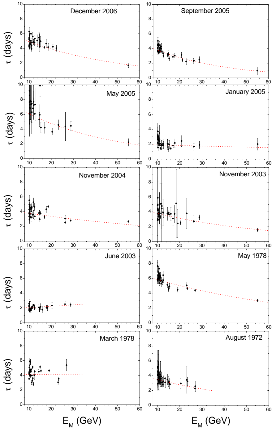
Figure 2: The recovery time \tau as a function of the median energy E_M of individual detectors. The dotted line represents the best fit exponential functions.
