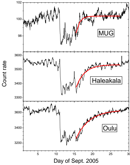
Figure 1: Count rates of MUG, Haleakala NM64 and Oulu NM for September 2005 together with the best-fit exponential recovery (thick lines) after the Forbush decrease.
