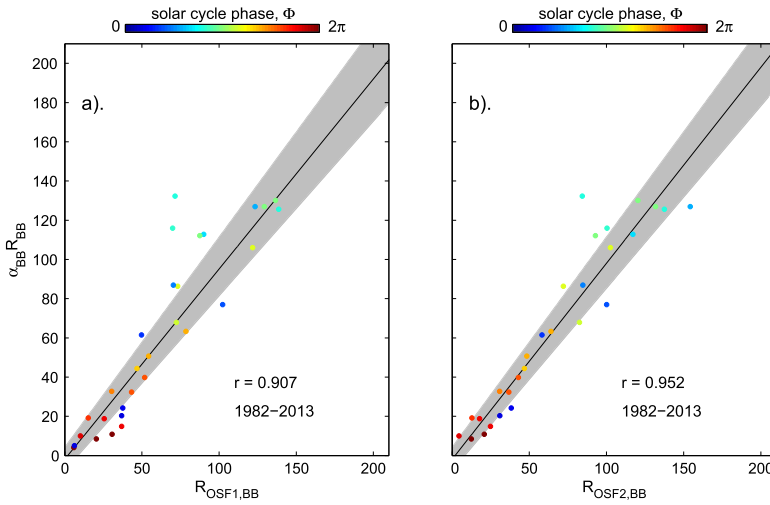
Figure 6 Scatter plots of \alpha_{BB} R_{BB} as a function of (a) R_{OSF1, BB} and (b) R_{OSF2, BB} , the estimates of R from the OSF reconstruction of Lockwood et al. (2014b) using OSF continuity and the OSF loss-rate formulations of Solanki, Schüssler, and Fligge (2000), and Owens and Lockwood (2012), respectively. The points are for the training interval and are coloured by the phase of the solar cycle according to the colour scale at the top of the figure. The black line shows the best-fit linear regression that minimises the mean square of the perpendicular deviations of the points from the line [ \langle d_{\perp}^2 \rangle ]. The grey area shows the range of fits for which \langle d_{\perp}^2 \rangle is larger than this minimum values by an amount smaller than the one- \sigma level, determined by the Student’s t -test.
