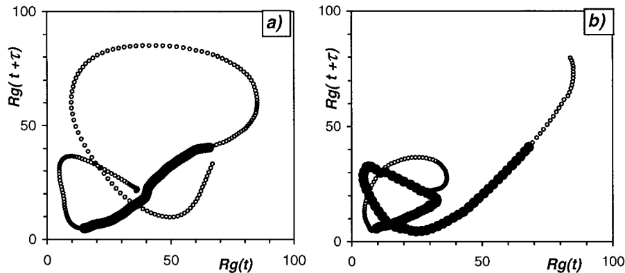
Figure 4. 2D projection of the phase evolution of sunspot activity around the Dalton minimum using the group sunspot numbers. Black dots denote the phase catastrophe in 1790–1798. (a) The standard sunspot number evolution depicting a phase catastrophe. (b) The same period but using the newly suggested lost cycle in 1793–1800 which removes the phase catastrophe.
