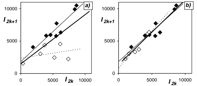
Fig. 3. Intensities of odd sunspot cycles vs. even cycles for a) standard cycle numbering; b) numbering suggested in the paper. Open (filled) diamonds correspond to the interval before (after) DM. Dotted, thin and thick solid lines give the linear fit (Eq. (1)) before and after DM, and for the entire period, respectively. Best fitting parameters are given in Table 1
