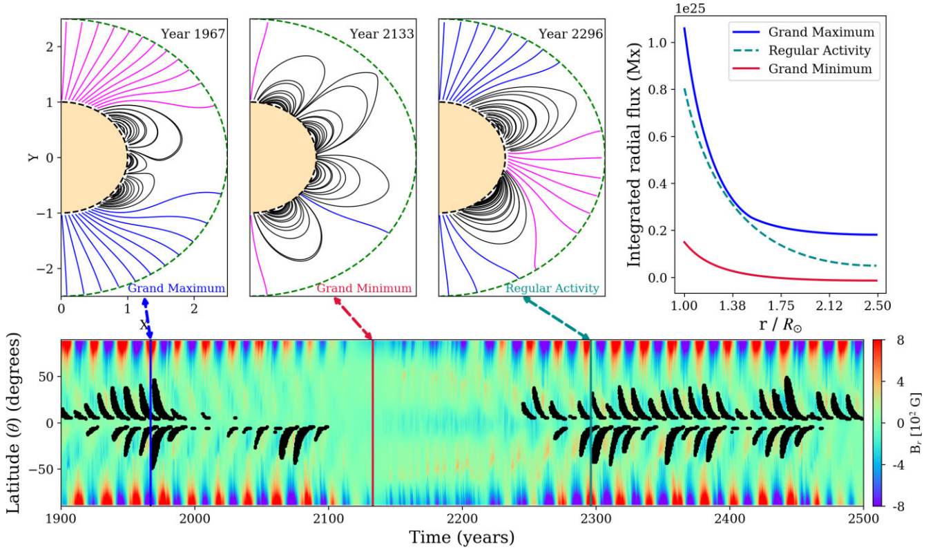
Figure 4. Reduction in magnetic field strength for different phases of solar activity. In our analysis, year 1967 corresponds to a grand maxima phase. Similarly, year 2133 and 2296 denote grand minima and regular solar activity phase. The integrated unsigned radial flux ( \int |B_r| 2\pi r^2 \sin \theta d\theta ) across different radial heights are plotted in the top-right-hand panel in blue (grand maxima), dashed dark cyan (regular activity), and red (grand minima). The decrease of over all flux from grand maxima to grand minima is observed for these three cases. In coronal magnetic field, configuration plots source surface ( r = 2.5R_\odot ) is denoted by green-dashed line. Distribution of closed and open magnetic fields for different phases (grand maximum, grand minimum, and regular) is provided with radially outward/inward open field lines plotted in blue/magenta. On the butterfly diagram (in the bottom panel), these phases are marked in solid lines for ease of understanding.
